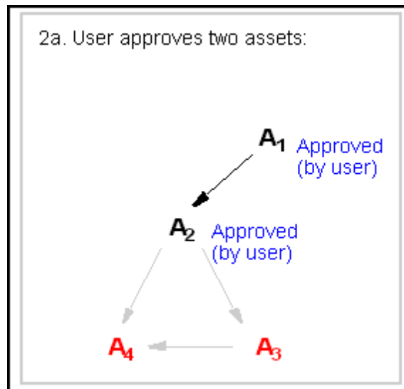
Figure 17-13 Dependency Model
