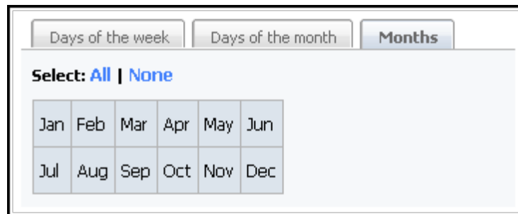
Figure 16-2 Months Tab
