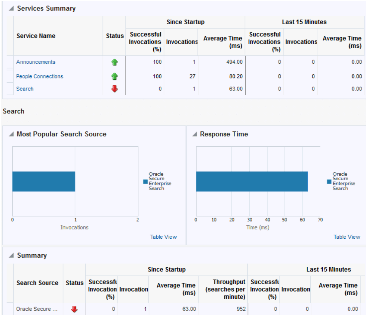
Figure 22-28 Search Metrics
