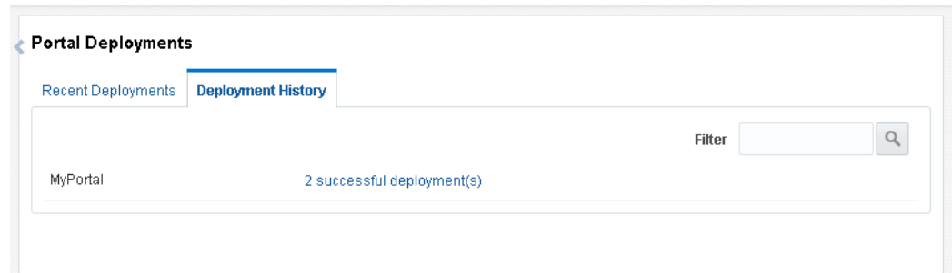
Figure 34-5 Deployment History
