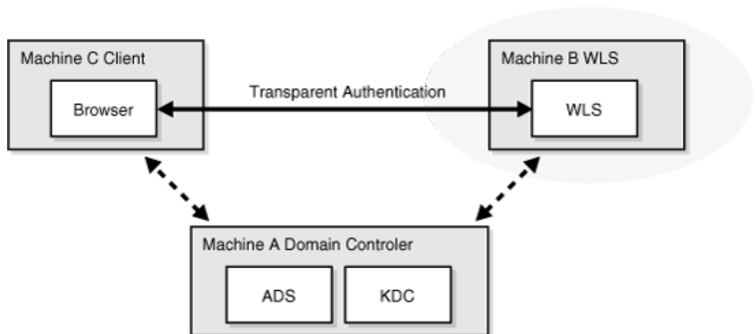
Figure 28-7 SPNEGO-based Authentication
