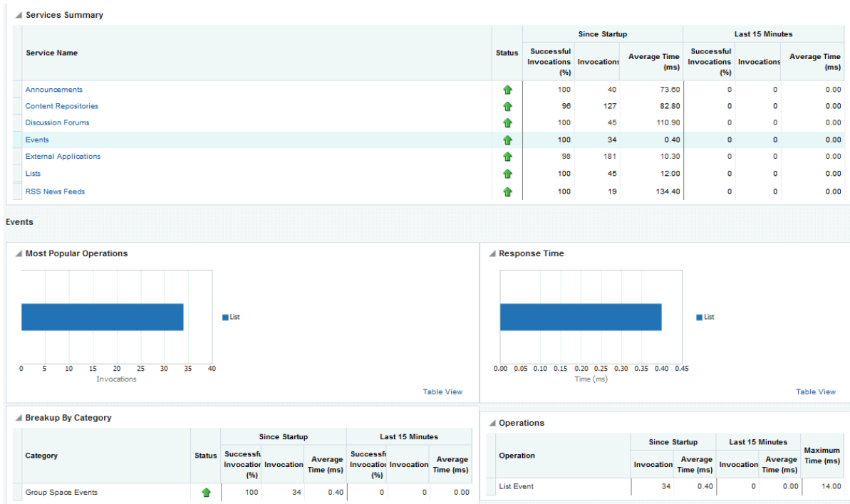
Figure 22-18 Events Metrics
