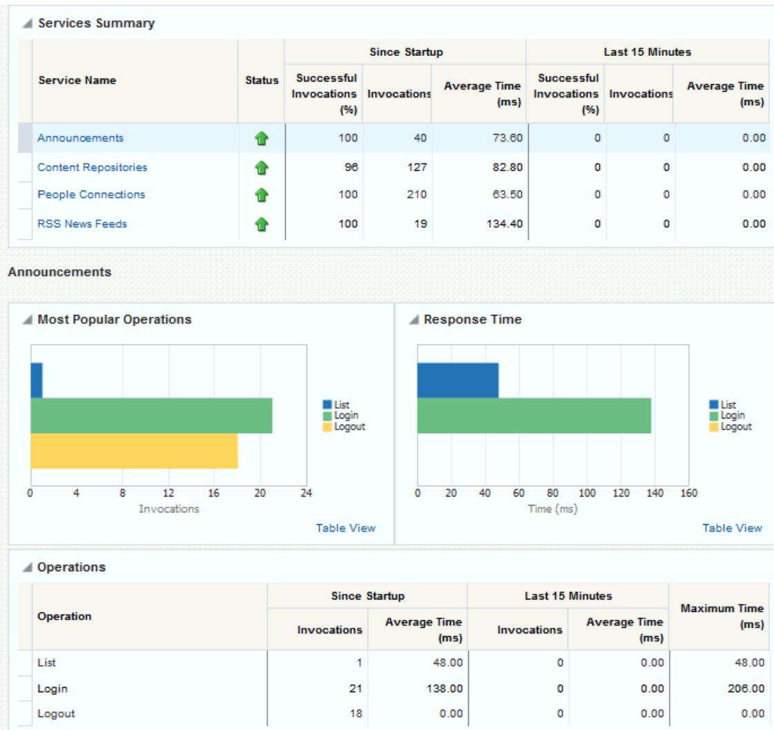
Figure 22-14 Announcements Metrics
