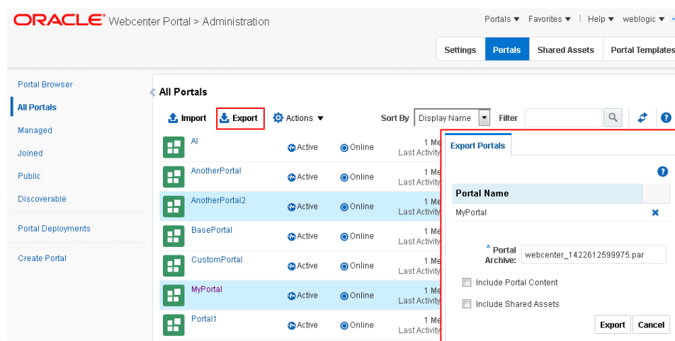
Figure 34-10 Exporting Portals
