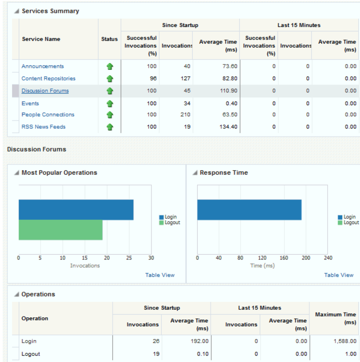
Figure 22-17 Discussion Metrics
