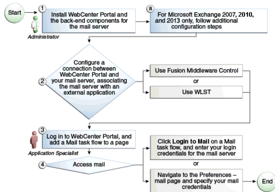
Figure 12-1 Configuring Mail
