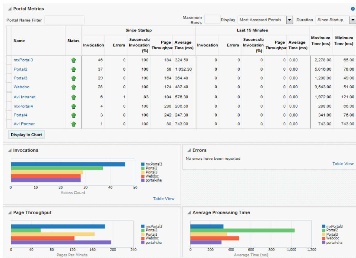
Figure 22-13 Portal Metrics
