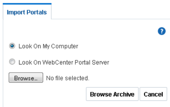
Figure 34-12 Importing Portals
