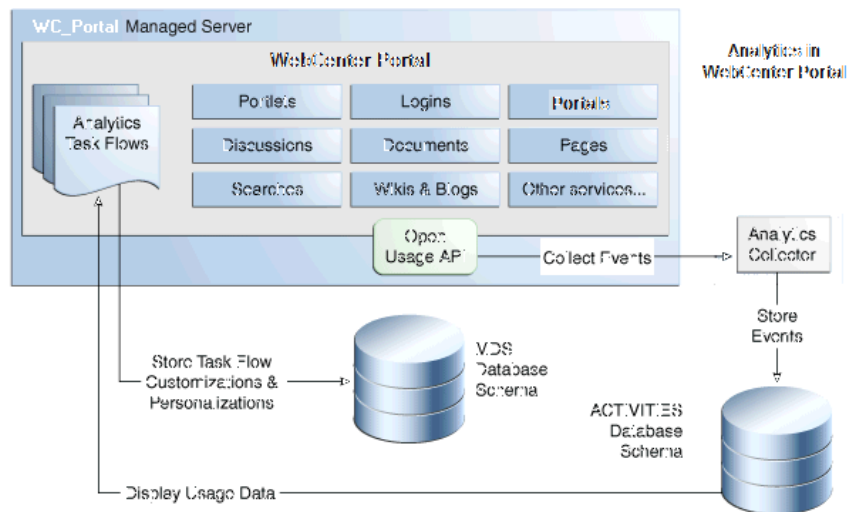
Figure 7-1 Analytics Components
