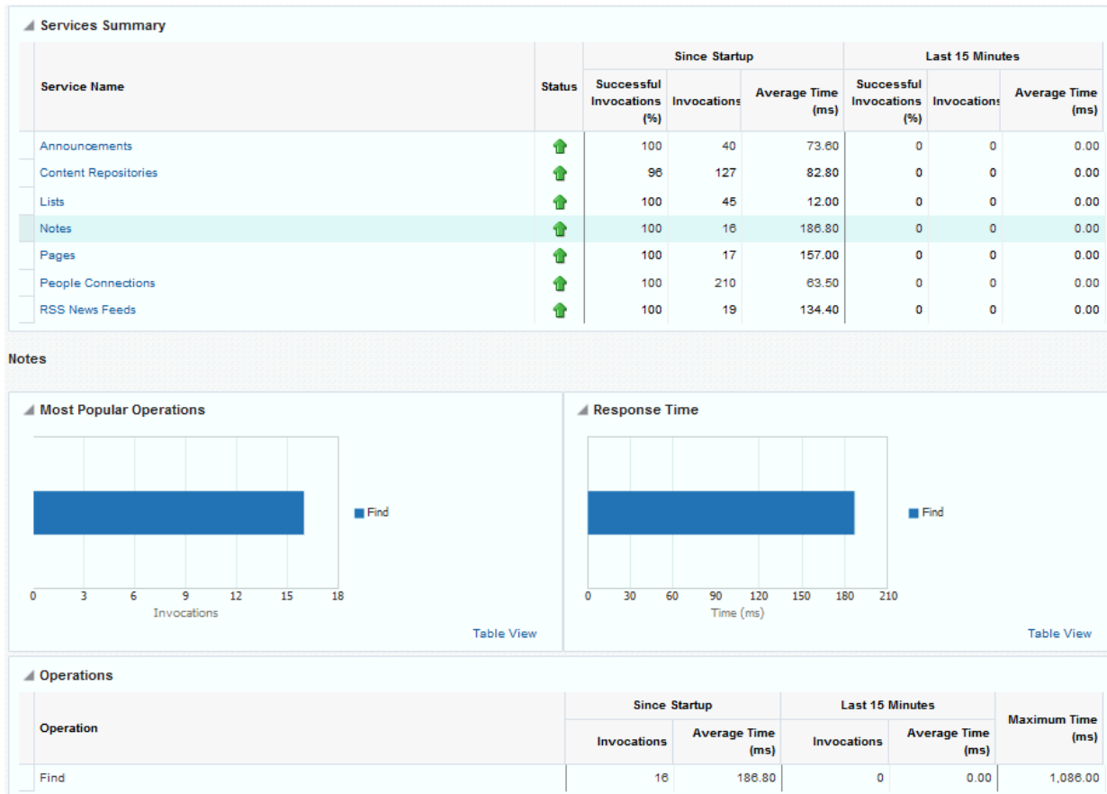
Figure 22-24 Notes Metrics
