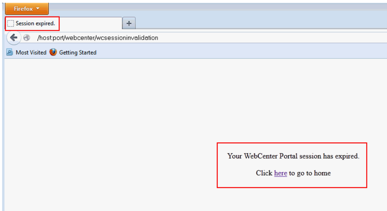
Figure 39-21 Timeout Page
