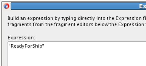
Figure 4-18 ReadyForShip Expression
