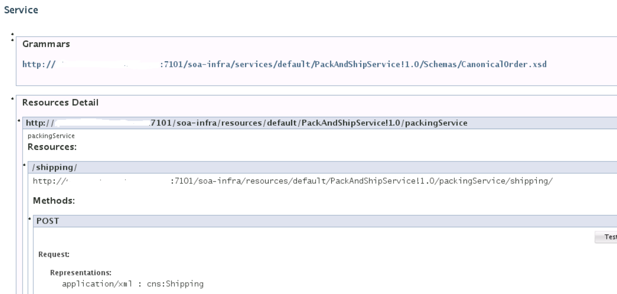
Figure 6-10 Service Dialog
