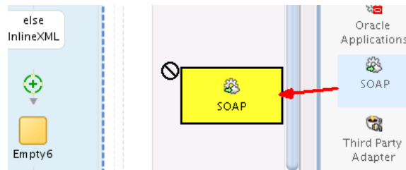
Figure 9-14 SOAP Reference
