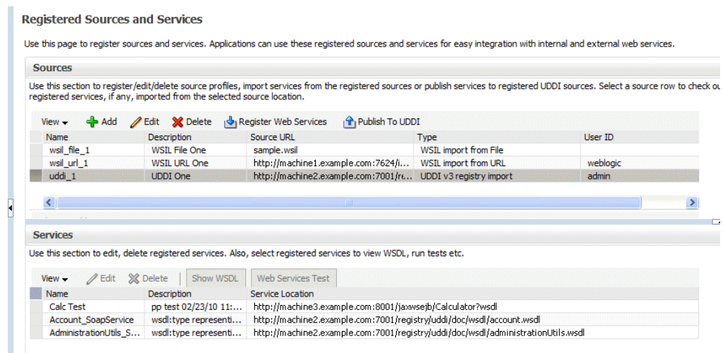
Figure 9-1 Viewing Registered Sources and Services
