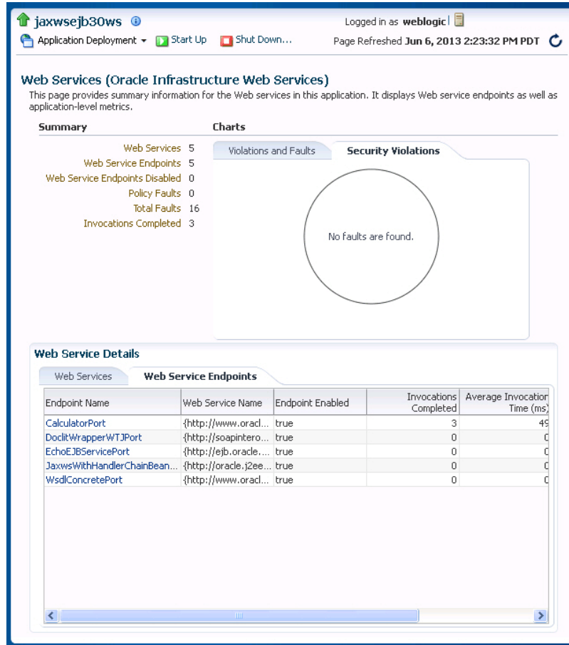
Figure 4-2 Web Services Summary Page for ADF and WebCenter Applications
