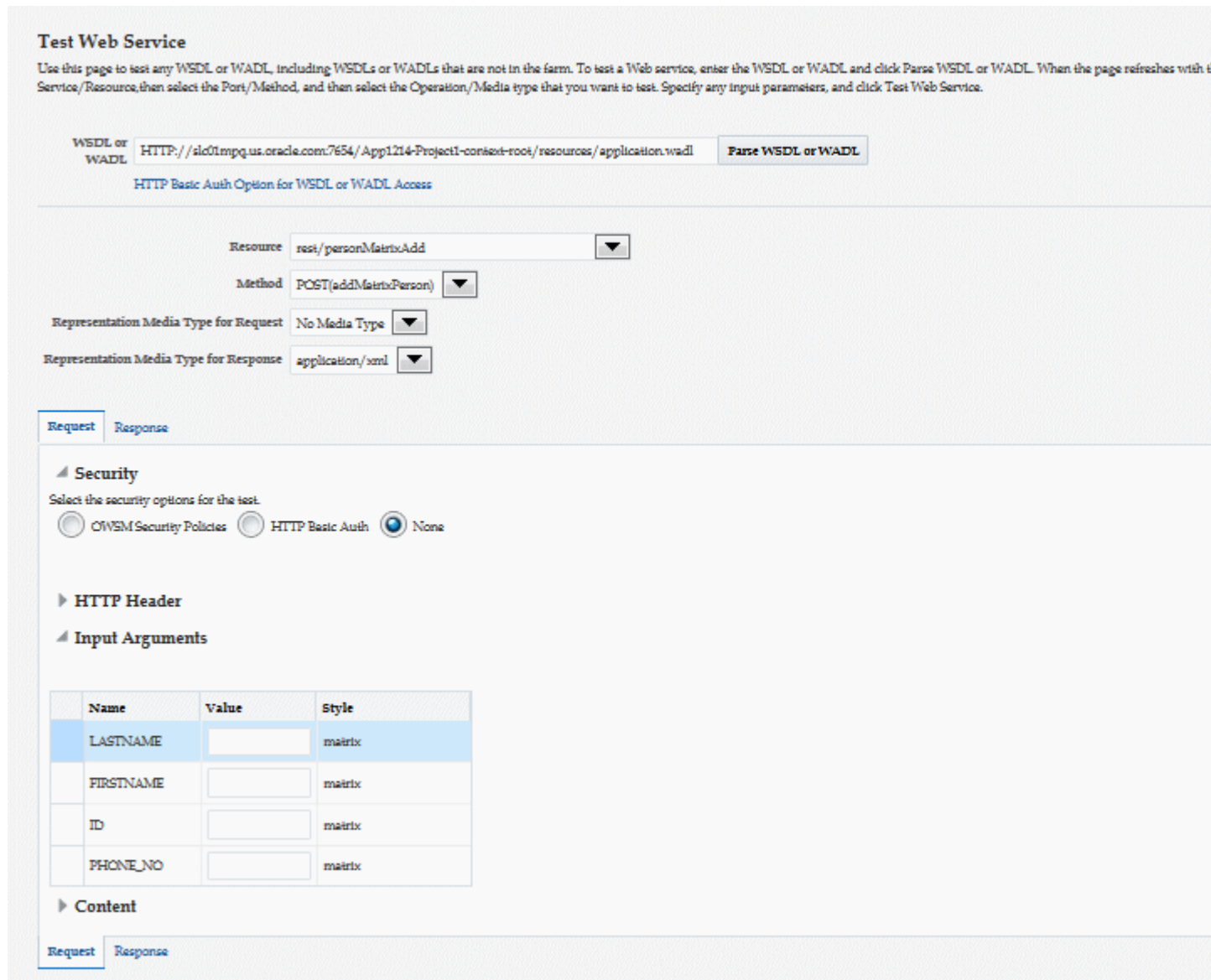
Figure 5-8 Test Web Service Page for a WADL
