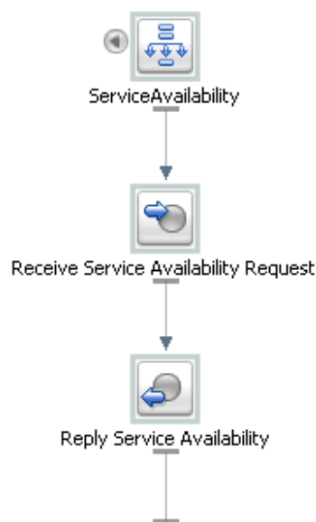
Figure 10-5 New Split-Join
