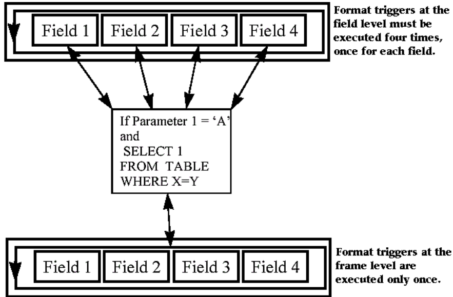
Figure 24–1 Format Triggers
