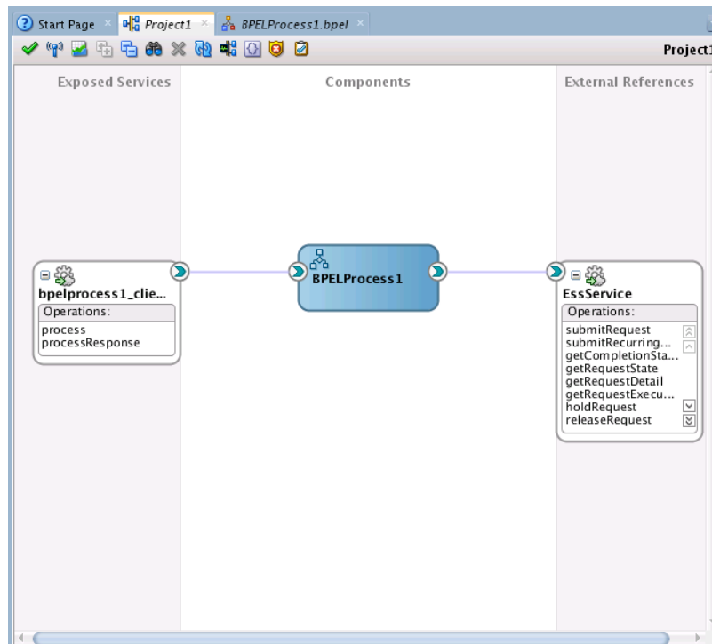
Figure 16-10 The Project Editor Tab
