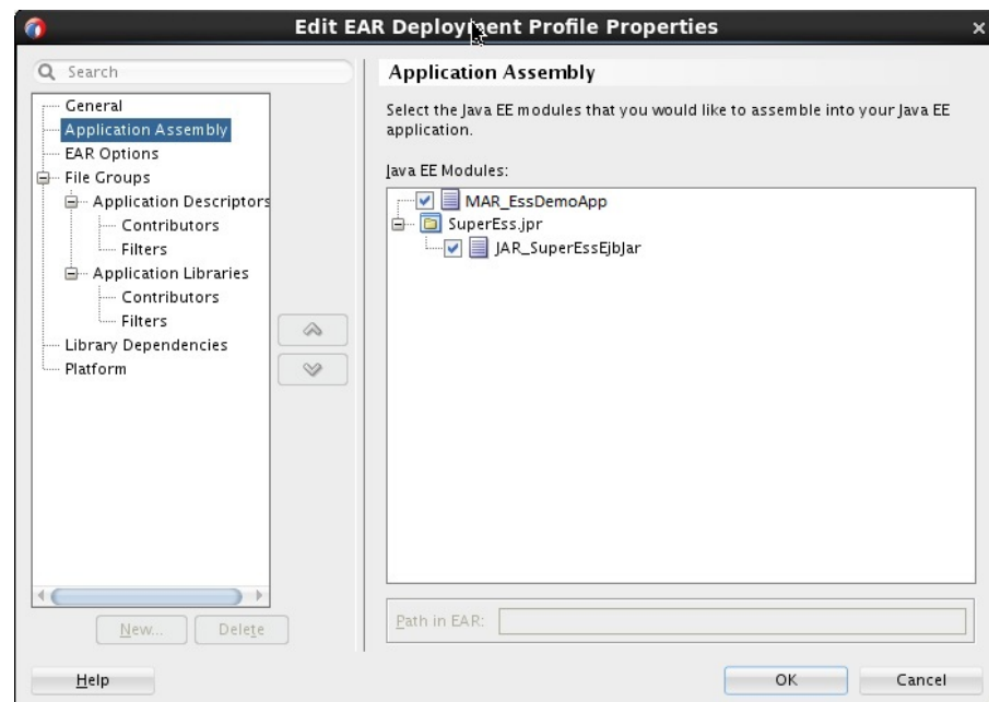
Figure 7-21 Edit EAR Deployment Profile Properties
