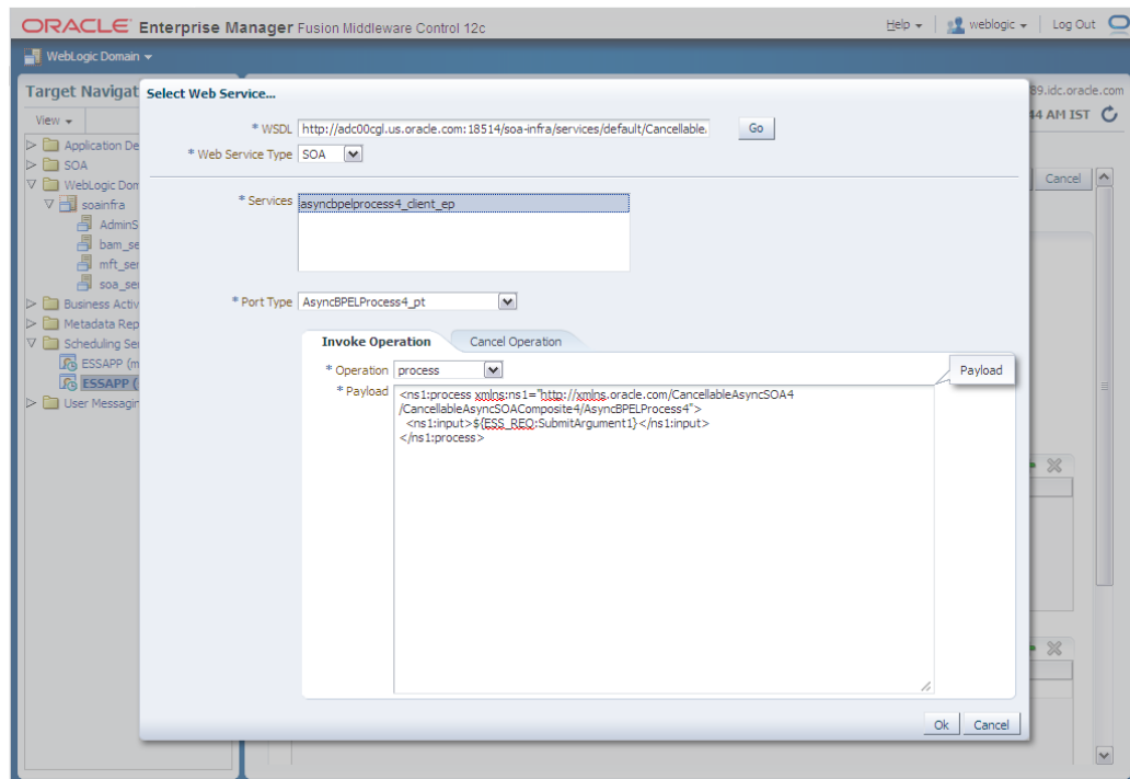
Figure 13-7 Fusion Middleware Control Console: Select Web Service Pop-up
