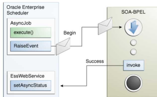
Figure 21-5 BPEL Call from Oracle Enterprise Scheduler Asynchronous Job
