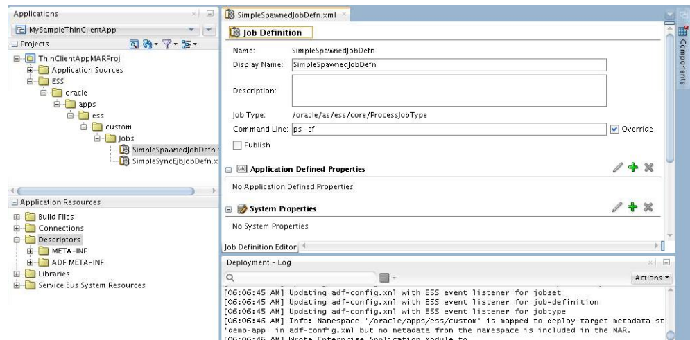
Figure 6-9 SimpleSpawnedJobDefn.xml Tab
