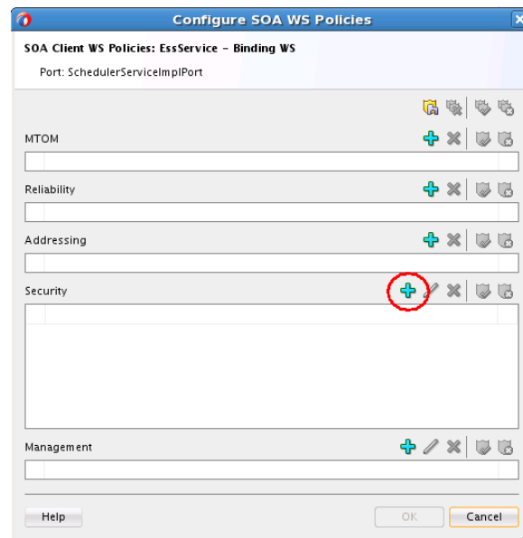
Figure 16-13 The Configure SOA WS Policies Dialog
