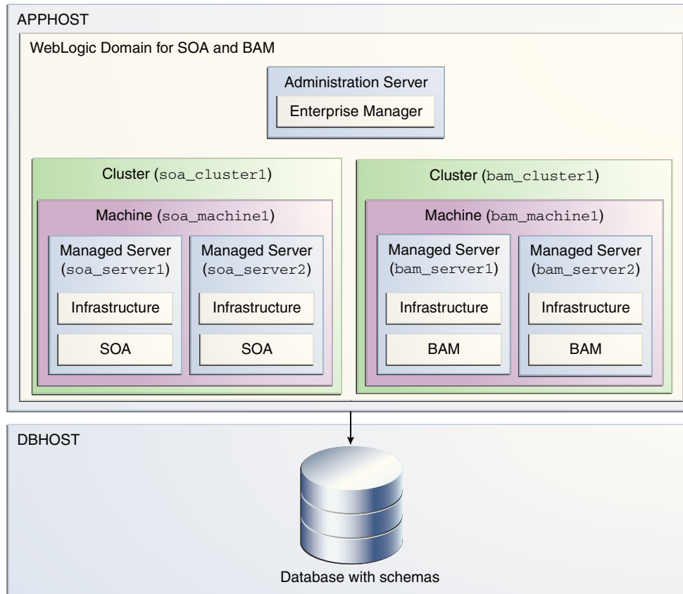
Figure 1-2 BAM Standard Installation Topology
