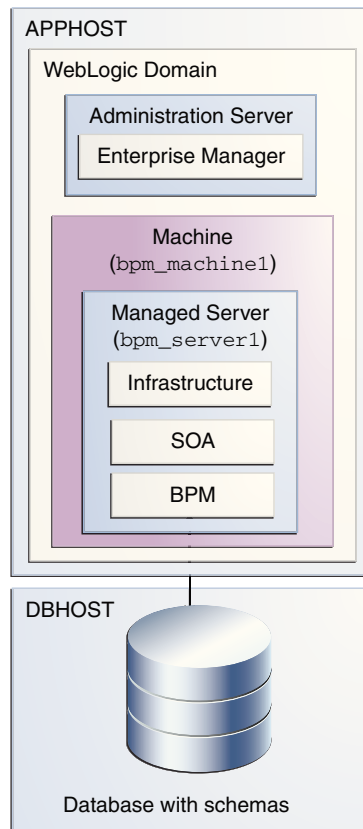
Figure A-1 Oracle Business Process Management Standalone Topology
