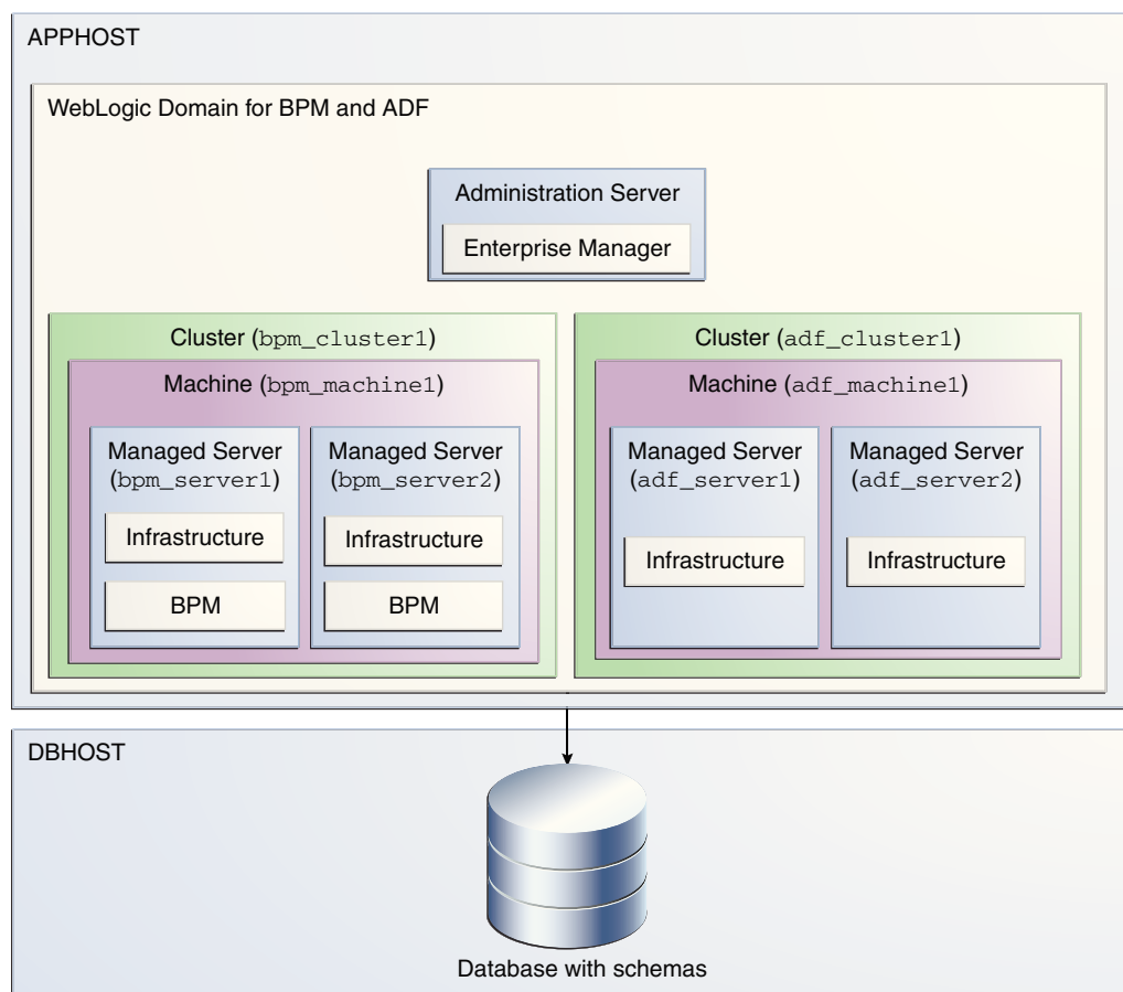
Figure A-3 BPM and ADF Topology
