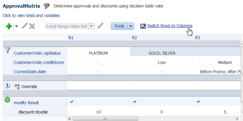
Figure 12-48 A Sample Decision Table
