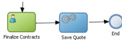
Figure A-19 The Service Task within the Sales Quote Example Process
