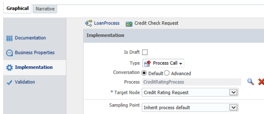
Figure 7-9 Activity Properties - Implementation
