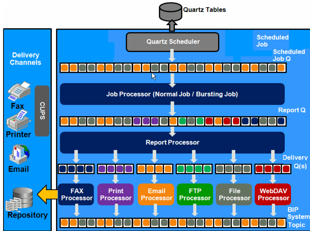
Figure 7-1 Scheduler Architecture
