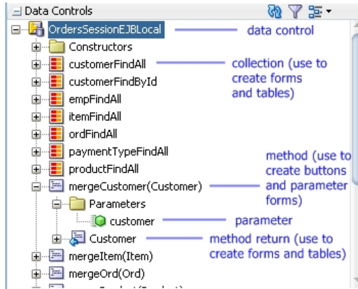
Figure 2-3 Data Controls Panel Main Nodes
