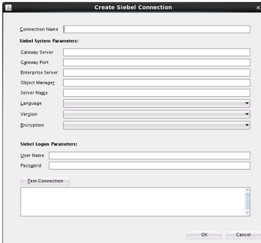
Figure 16-3 Siebel Adapter Configuration Wizard — Create Siebel Connection Screen
