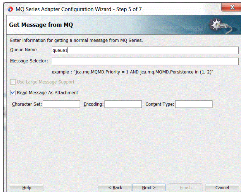
Figure 10-34 Configuring Inbound MQ Adapter to Read Message as Attachment
