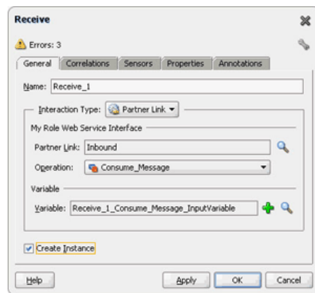
Figure 8-22 The Receive Dialog
