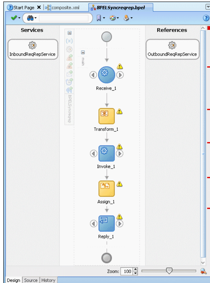
Figure 10-70 The BPELSyncreqrep.bpel Page
