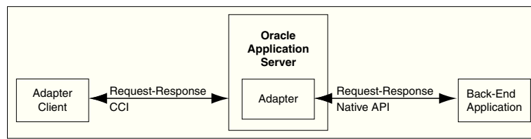
Figure 1-16 Request-Response Service
