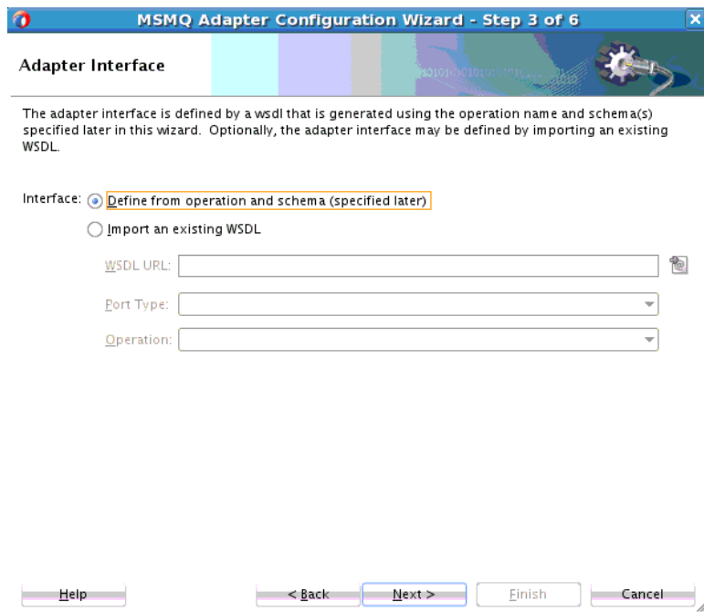
Figure 13-3 MSMQ Adapter Configuration Wizard Adapter Interface Screen
