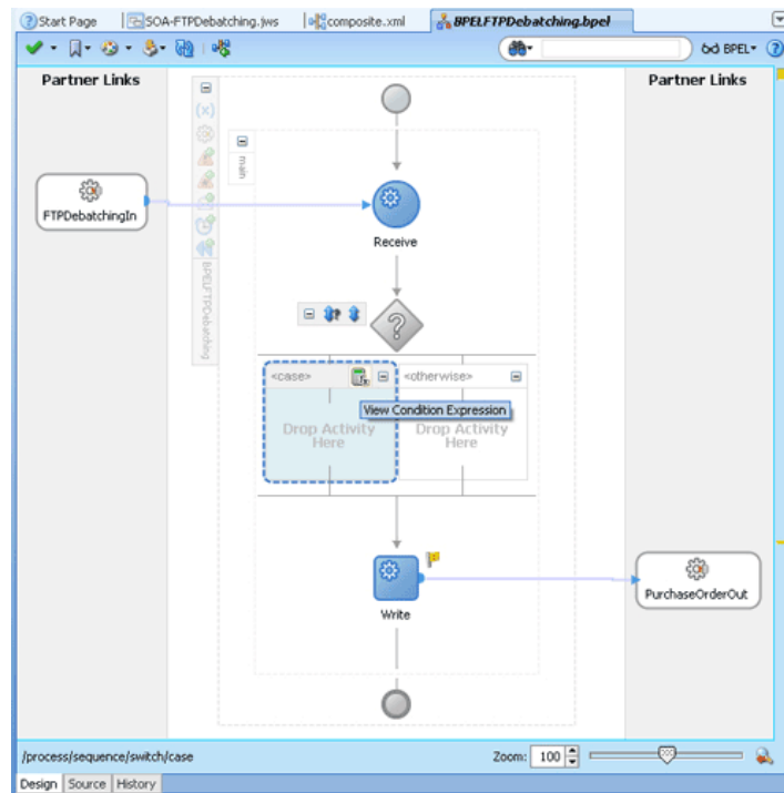
Figure 4-163 BPELFTPDebatching.bpel Page
