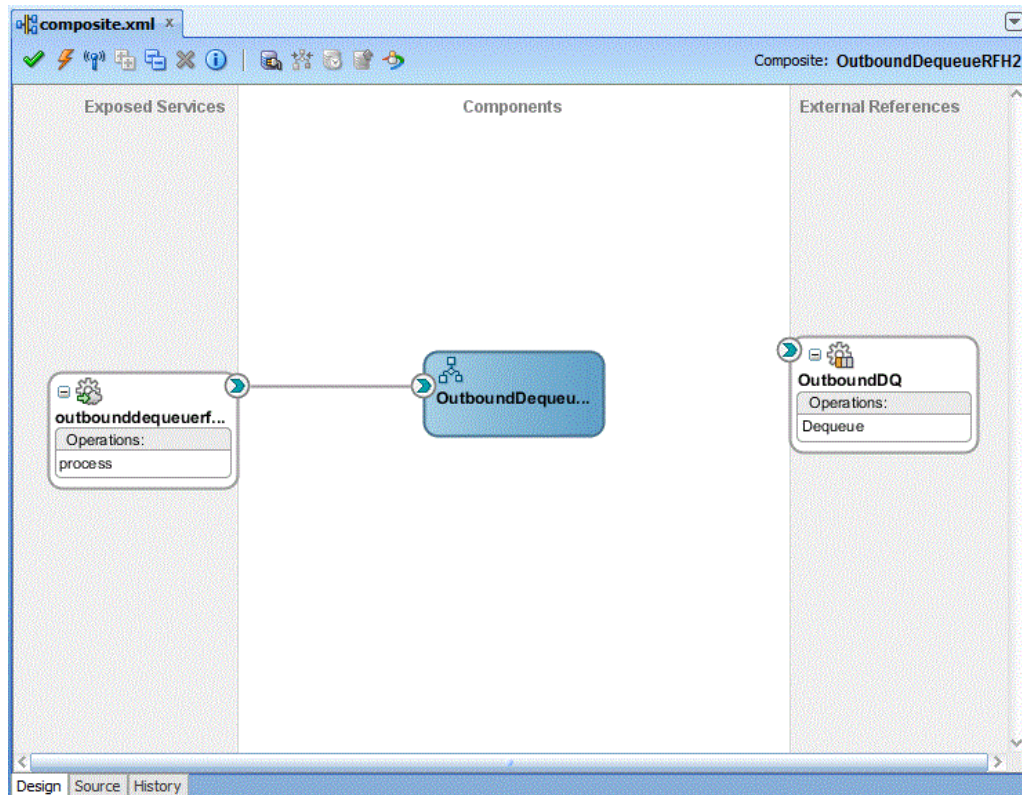
Figure 10-103 The JDeveloper-composite.xml
