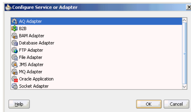
Figure 3-7 Adapter Types
