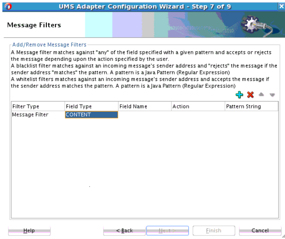
Figure 11-14 UMS Adapter Message Filters Screen
