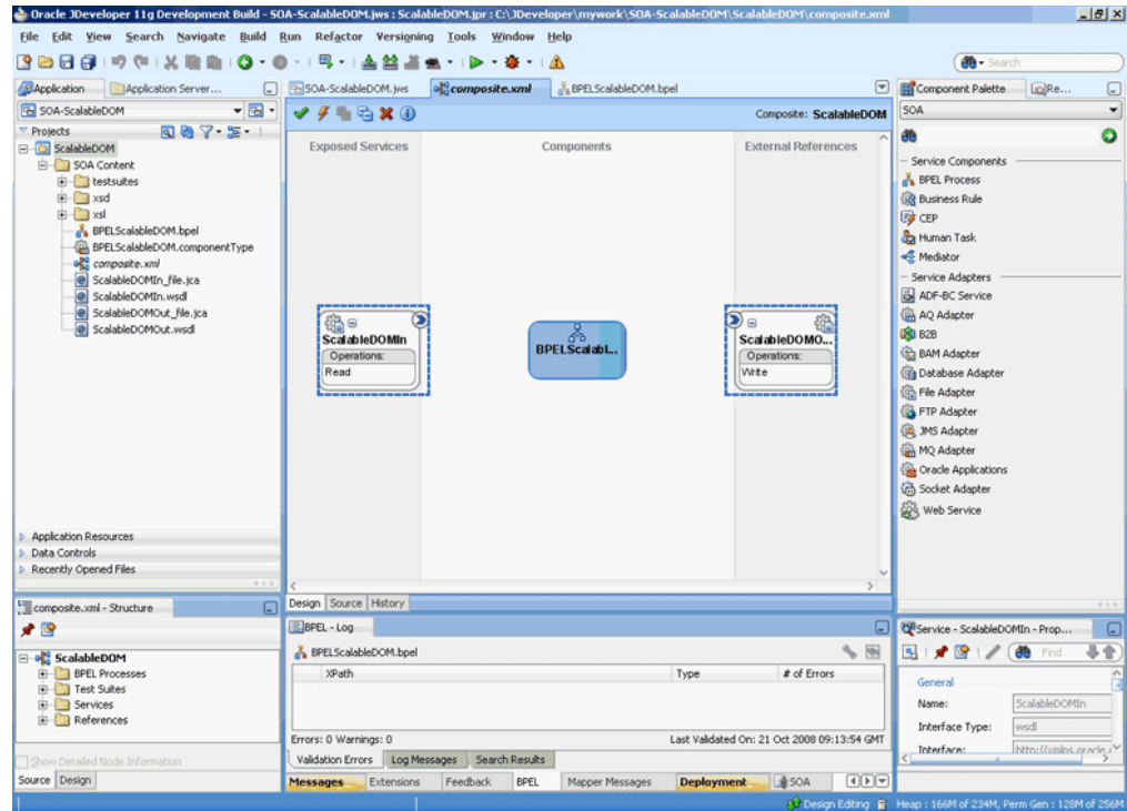
Figure 4-101 The JDeveloper - Composite.xml
