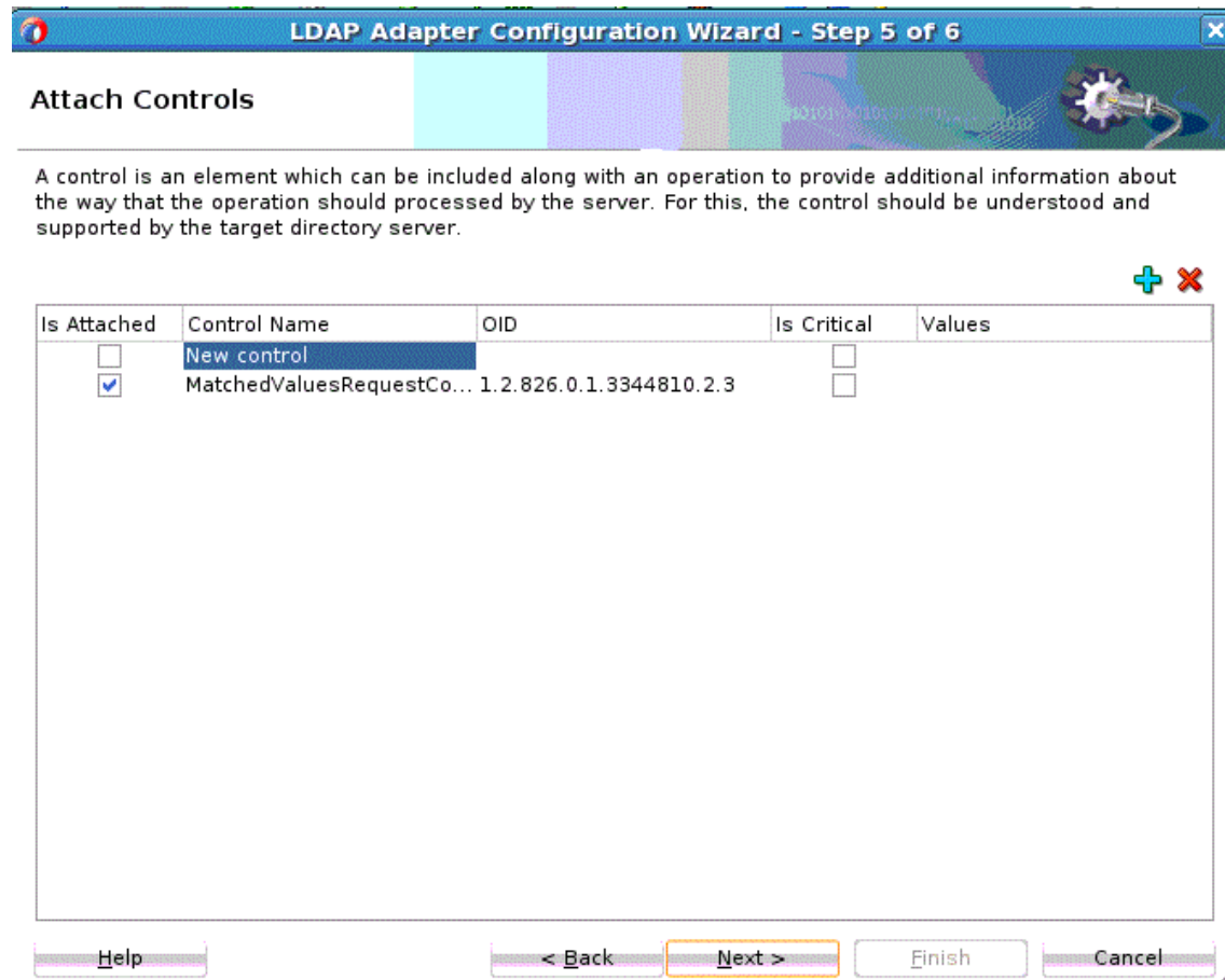
Figure 12-15 LDAP Configuration Wizard Attach Controls Page
