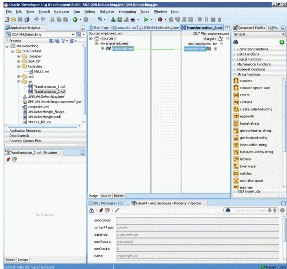
Figure 4-87 The JDeveloper - Transformation_2.xsl
