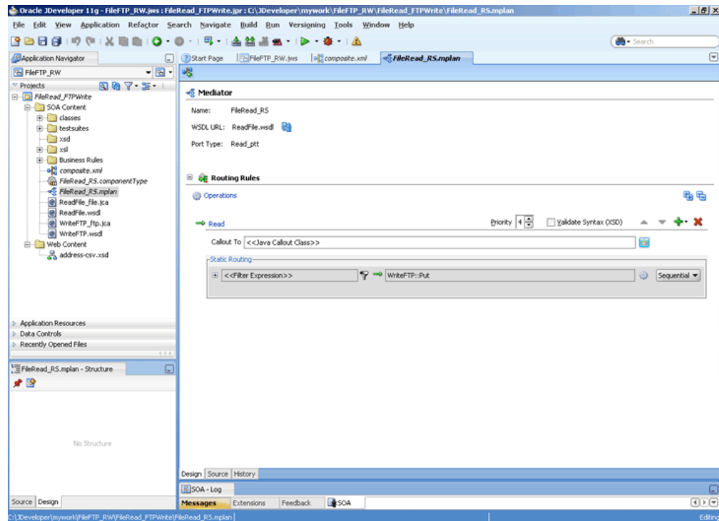
Figure 4-97 The JDeveloper - ReadFile_RS Routing Service Page
