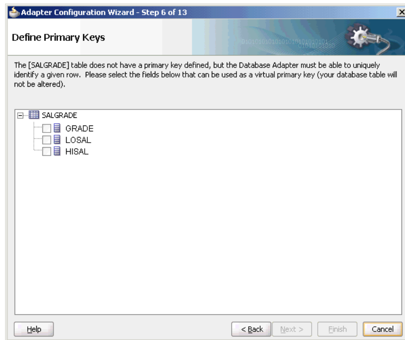
Figure 9-11 The Adapter Configuration Wizard: Define Primary Keys Page
