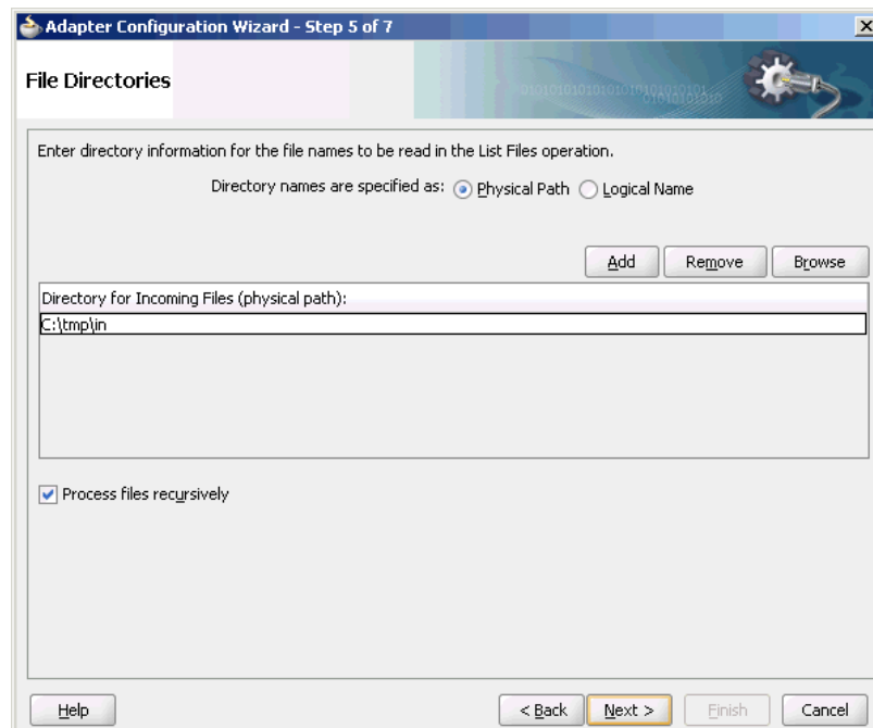
Figure 4-41 The Adapter Configuration Wizard-Specifying Incoming Files
