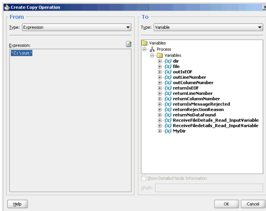
Figure 4-34 Create Copy Operation Dialog
