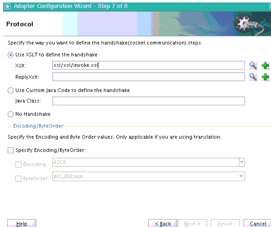
Figure 5-8 Defining a Protocol with the Handshake Mechanism By Using a Style Sheet
