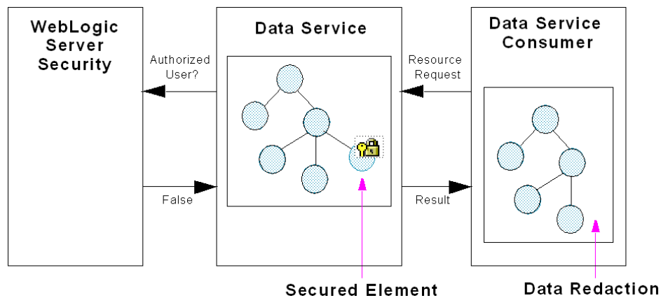
Figure 5–1 Data Redaction
