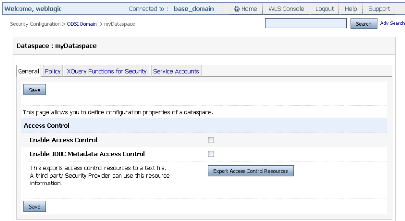
Figure 5–3 General Tab
