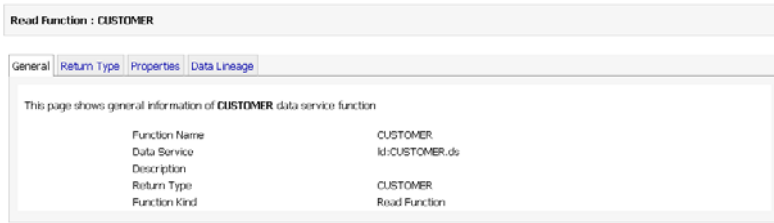
Figure 7–6 Function Metadata
