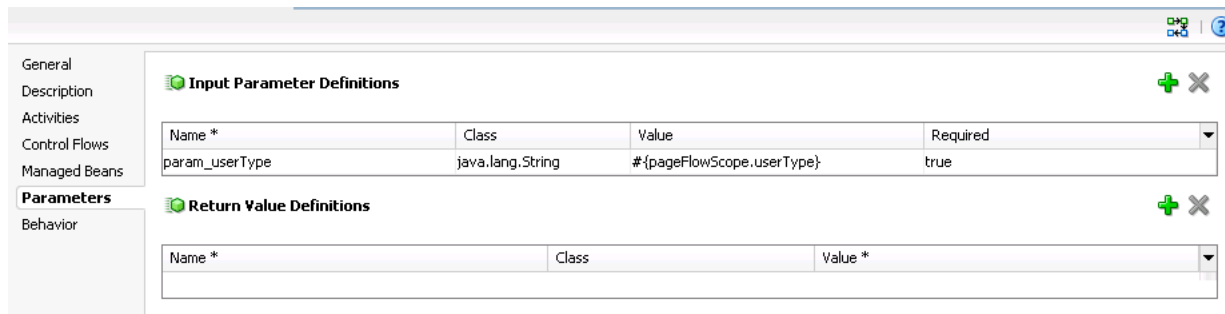
Figure 22–1 Task Flow Defining an Input Parameter
