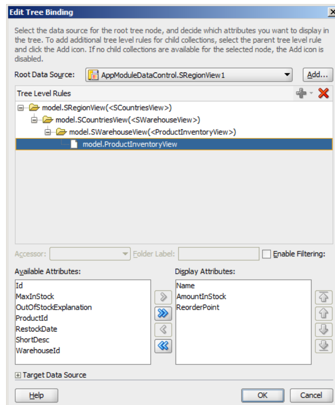
Figure 39–33 Edit Tree Binding Dialog
