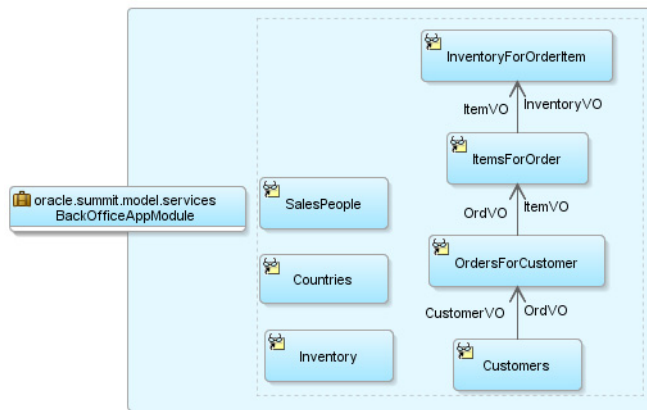
Figure 13–16 Partial UML Diagram of Application Module
