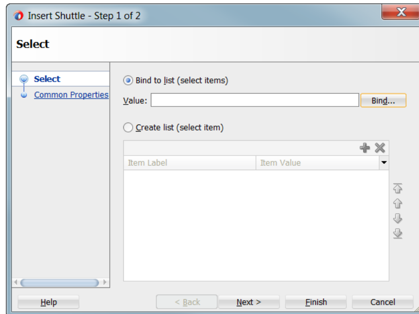
Figure 32–8 Insert SelectManyShuttle Wizard
