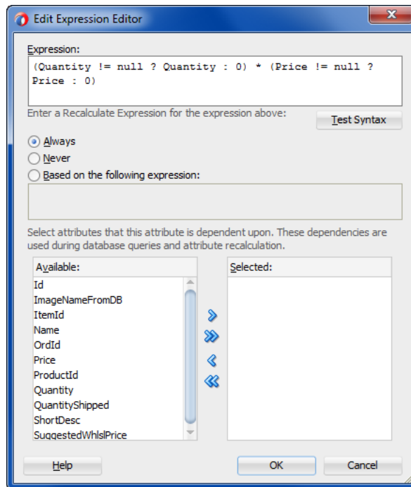
Figure 3–12 Dialog to Edit Expression for Default Attribute Values
