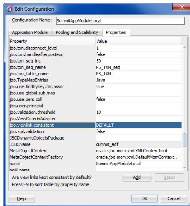
Figure 9-1 jbo.viewlink.consistent Property Setting
