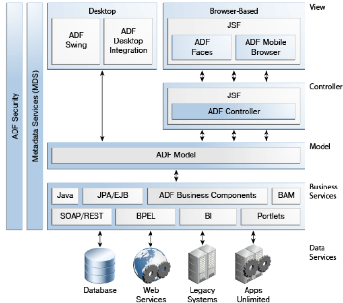
Figure 1–2 Simple Oracle ADF Architecture
