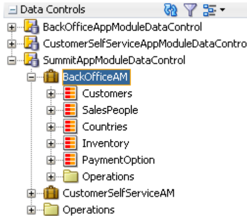
Figure 17-7 How Nested Application Modules Appear in the Data Controls Panel
