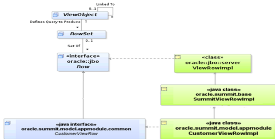
Figure 13–25 Custom View Row Interface Extends the Base Row Interface
