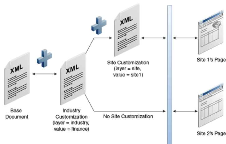
Figure 45–1 Example of Layered Customization
