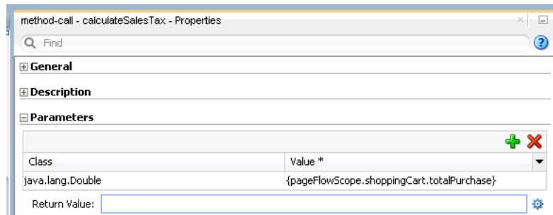
Figure 21–9 Method Parameters in a Method Call
