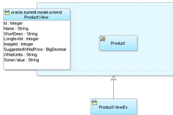
Figure 16–10 ADF Business Components Can Extend Another Component
