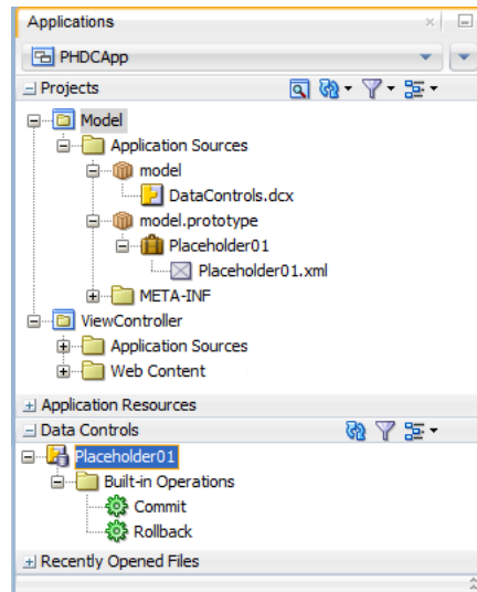
Figure 19–2 Applications Window and Data Controls Panel
