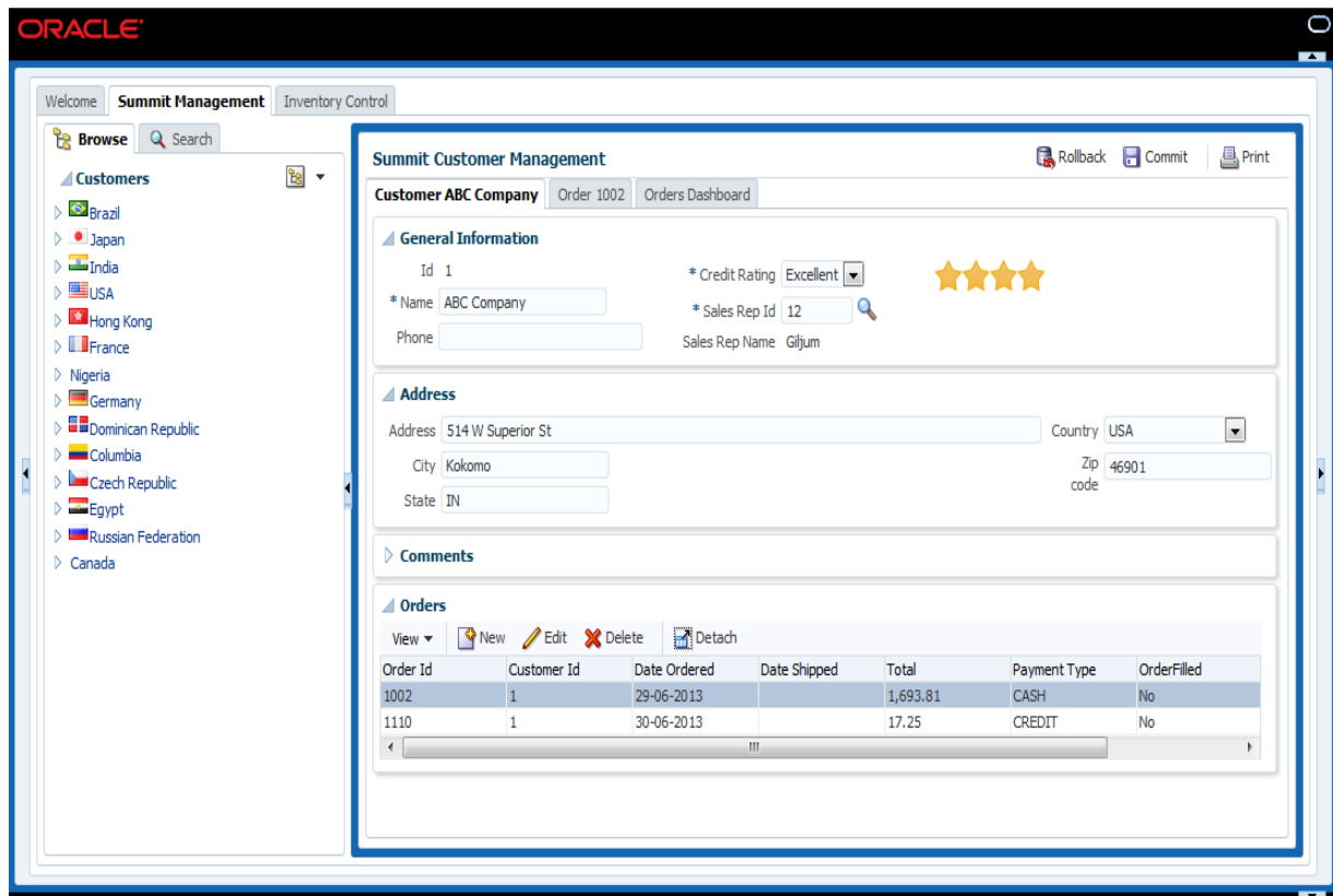
Figure 2-7 Index Page with Multiple Regions
