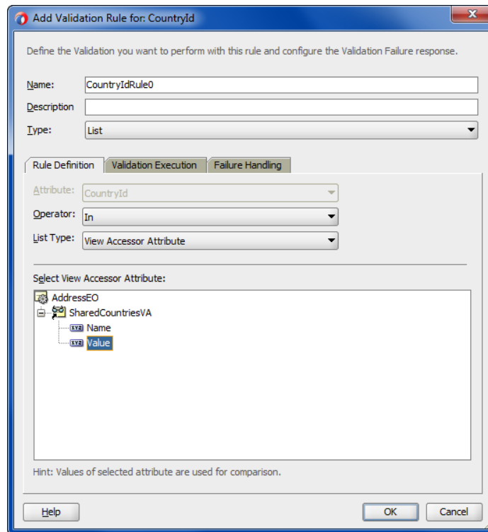
Figure 14–7 List Validator Using a View Accessor
