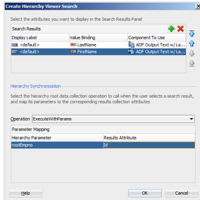
Figure 39–21 Create Hierarchy Viewer Search Dialog
