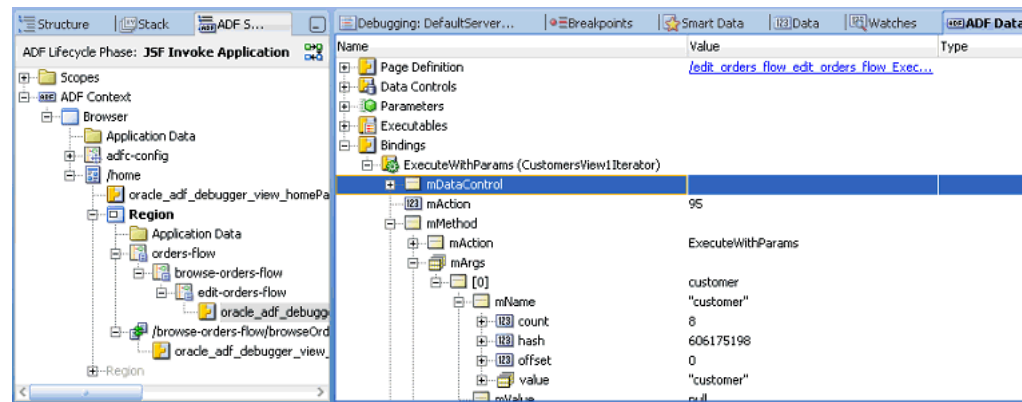
Figure 42–47 Method Bindings Selected for the ADF Data Window
