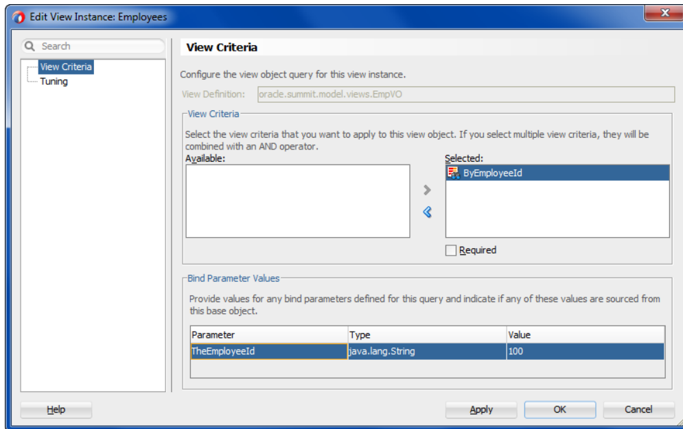
Figure 6–13 View Criteria Filters View Instance
