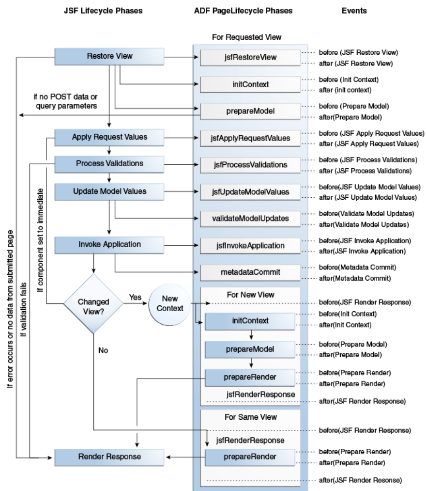
Figure 27-3 Lifecycle of a Page Request in a Fusion Web Application
