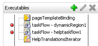
Figure 42–24 ADF Declarative Breakpoint Enabled on a Contextual Event in the Page Definition File
