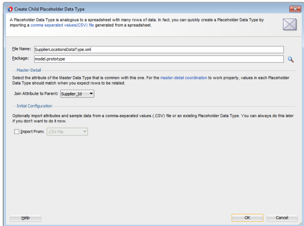
Figure 19–8 Create Child Placeholder Data Type Dialog
