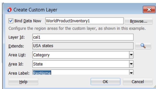
Figure 37–39 Create Custom Layer Dialog
