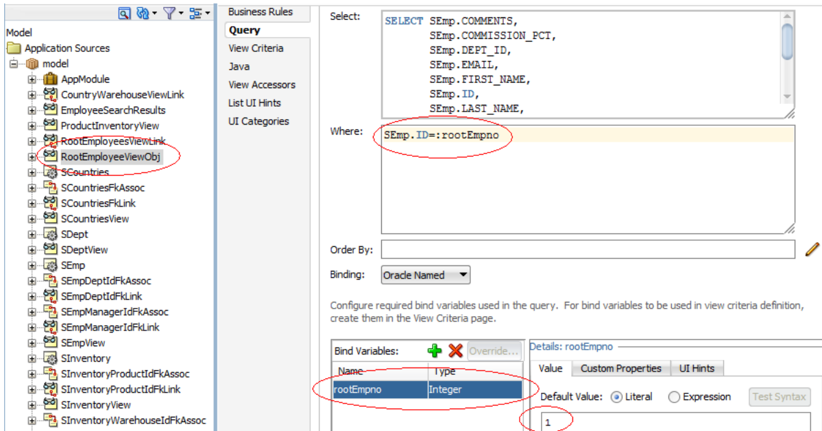
Figure 39–6 RootEmployeeViewObject Sample for Hierarchy Viewer
