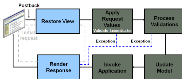
Figure 27-2 JSF and ADF Page Lifecycles
