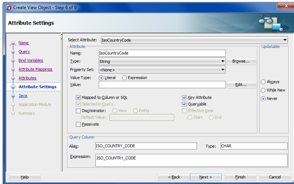
Figure 5–25 Create View Object Wizard, Attribute Settings Page
