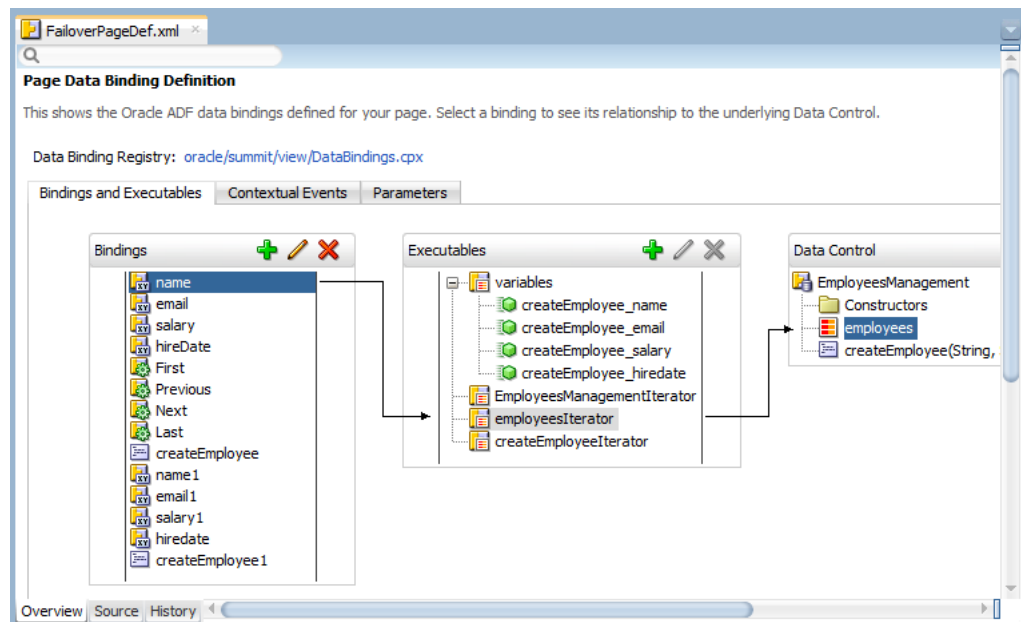
Figure 43–1 Page Data Binding Definition Overview Tab
