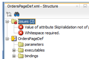
Figure 42–1 The Structure Window Displays XML Errors
