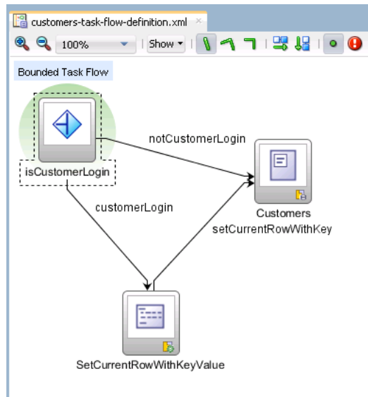
Figure 21–6 Router for Alternate Control Flow Cases
