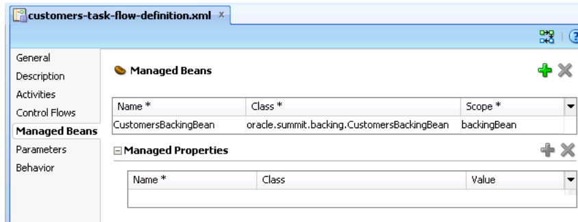
Figure 20–10 Managed Bean Registered With Task Flow
