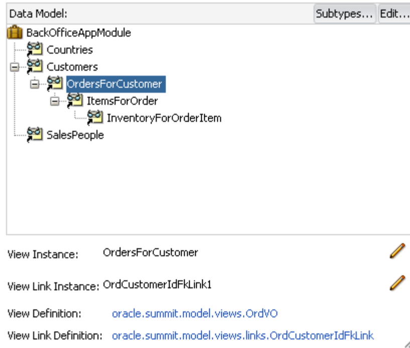
Figure 31–4 View Link between CustomerVO and OrdVO View Objects
