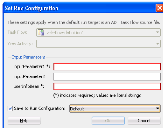
Figure 20–16 Set Run Configuration dialog
