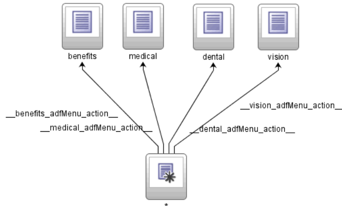
Figure 24–23 Updated Unbounded Task Flow
