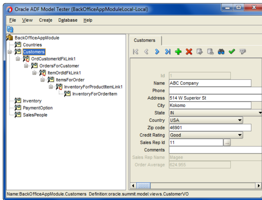
Figure 14–9 Testing the Data Model in the Oracle ADF Model Tester
