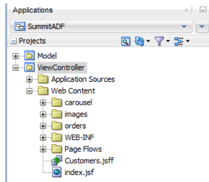
Figure 2–6 The ViewController Project of the SummitADF Workspace
