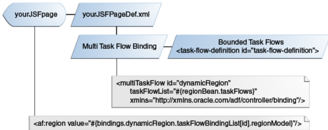
Figure 23–16 ADF Regions Derived from a Multi Task Flow Binding
