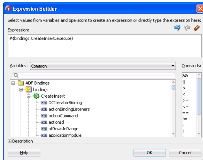
Figure 21-8 EL Expression for Method in Expression Builder Dialog
