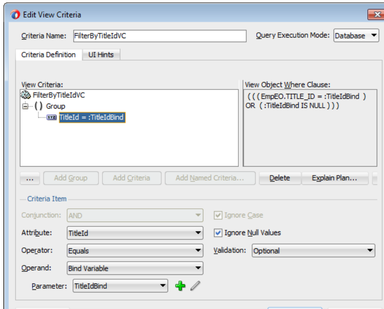
Figure 33–16 View Criteria with Named Bind Variable
