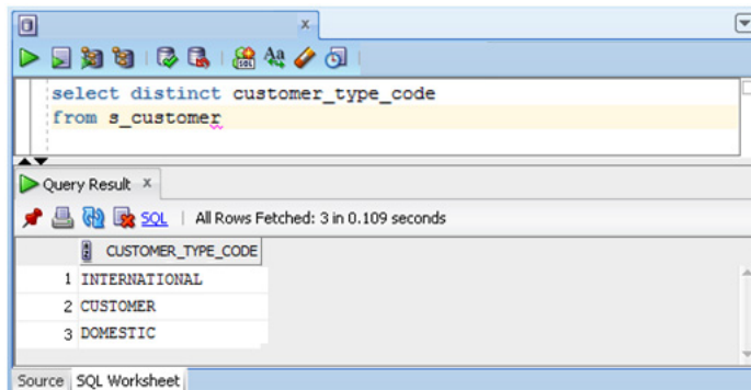
Figure 4–19 Using the SQL Worksheet to Find Distinct Discriminator Column Values
