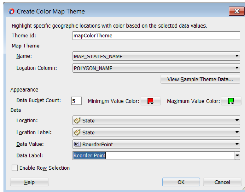
Figure 37–13 Create Color Map Theme for Product Popularity By State
