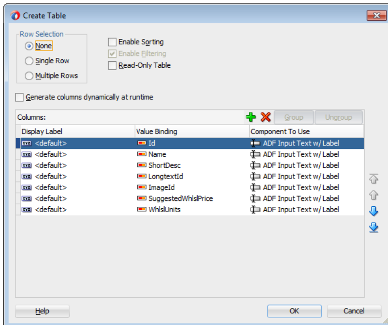
Figure 33–24 Edit Table Columns Dialog for Filtered Table
