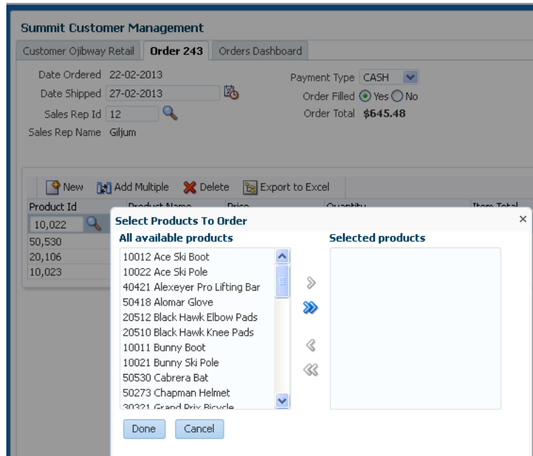
Figure 24-4 Task Flow Transaction
