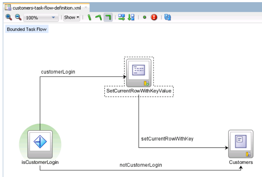
Figure 21–2 Customers Task Flow in the Summit ADF Task Flow Sample Application
