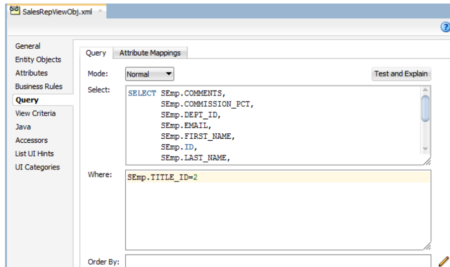
Figure 39–14 Sales Representatives View Object Using the Summit ADF Schema
