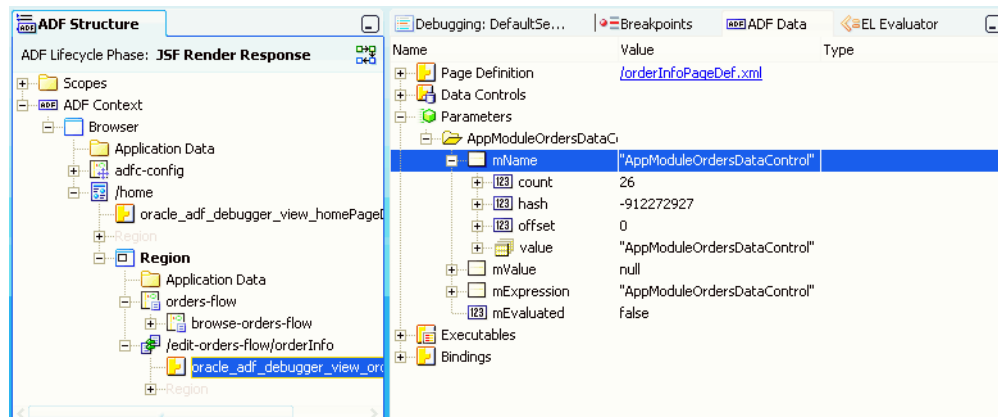
Figure 42-44 Parameters Selected for the ADF Data Window
