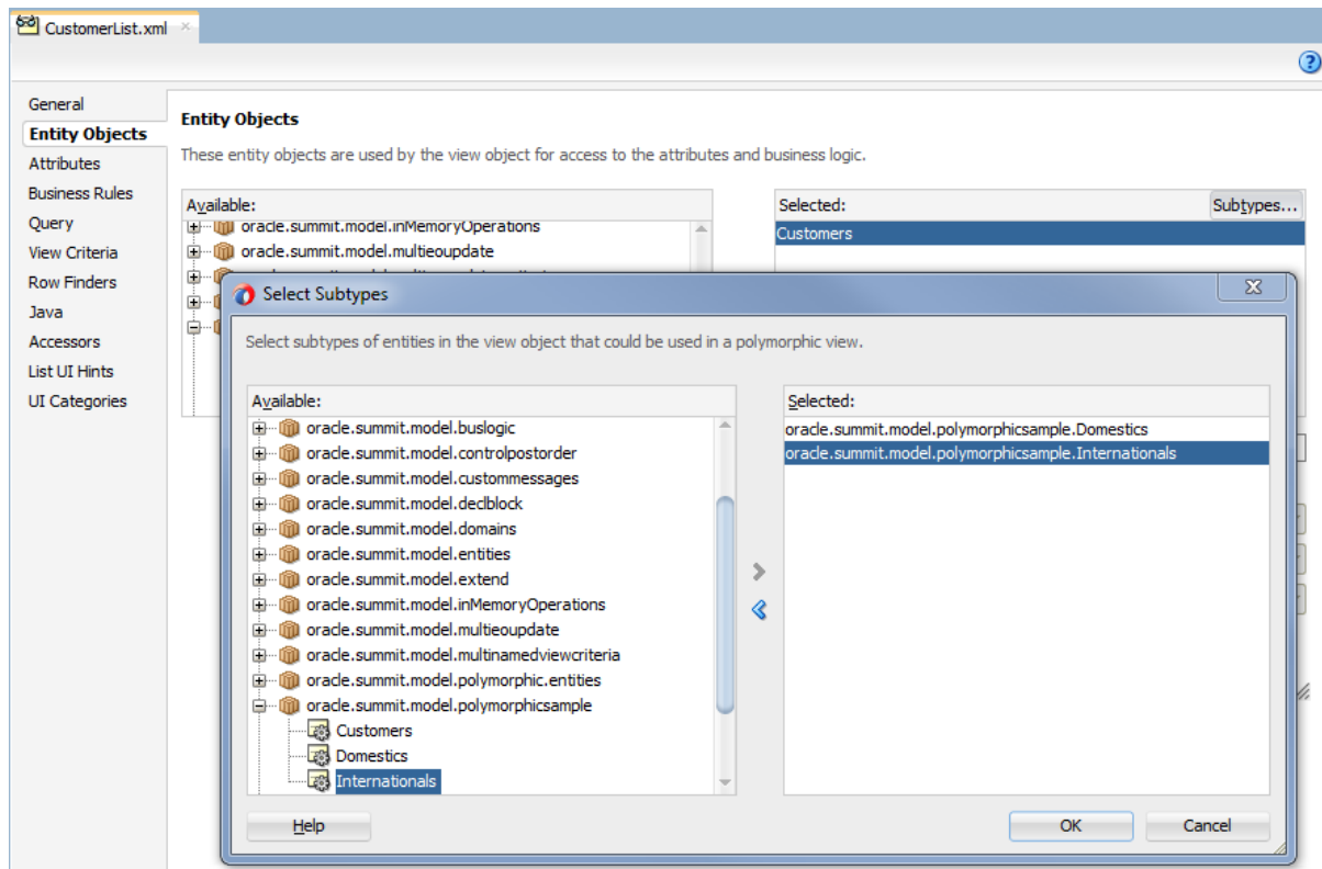
Figure 7–2 Entity Subtypes Define Possible Subtype View Objects
