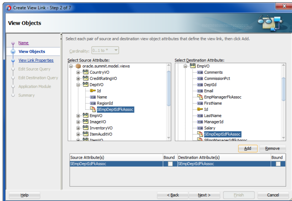
Figure 6–3 Master and Detail Related by an Association Selection
