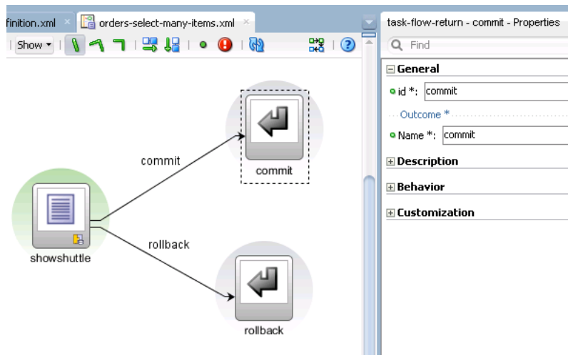
Figure 21–11 Multiple Task Flow Return Activities
