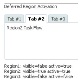
Figure 23–10 Deferred Activation of ADF Regions
