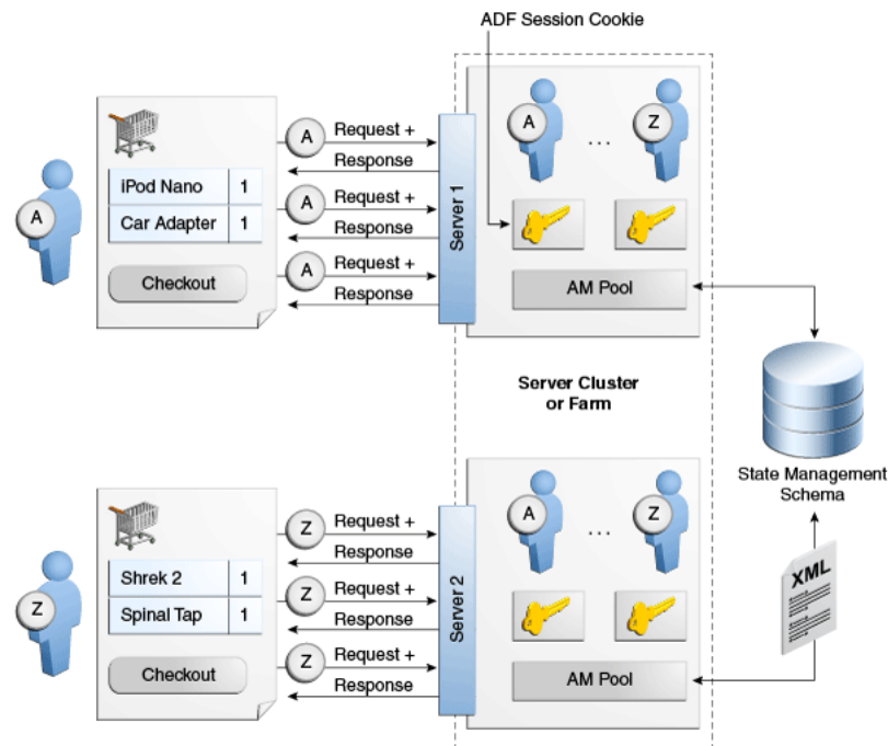
Figure 50–1 ADF Provides Generic, Database-Backed State Management
