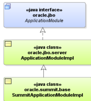
Figure 13–21 Your Custom Application Module Class Extends ApplicationModuleImpl
