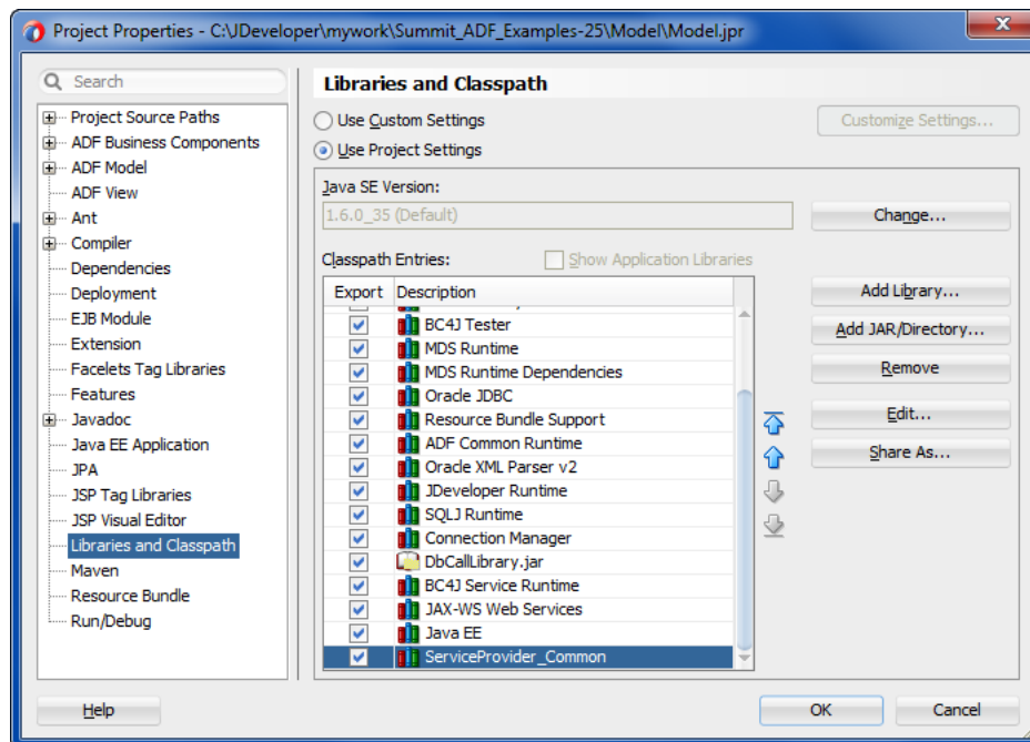
Figure 15–19 SDO Client Library Classpath Entry
