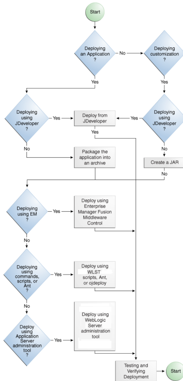
Figure 49–5 Application Deployment Flow Diagram
