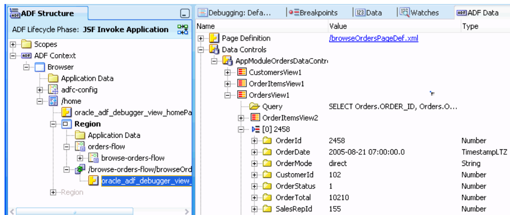
Figure 42-43 Binding Container (Business Components) Selected for the ADF Data Window
