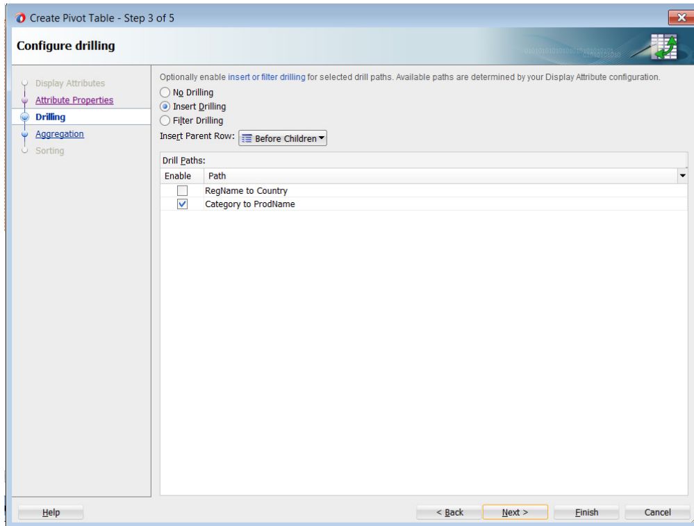
Figure 36–8 Configure Drilling Page of Create Pivot Table Wizard
