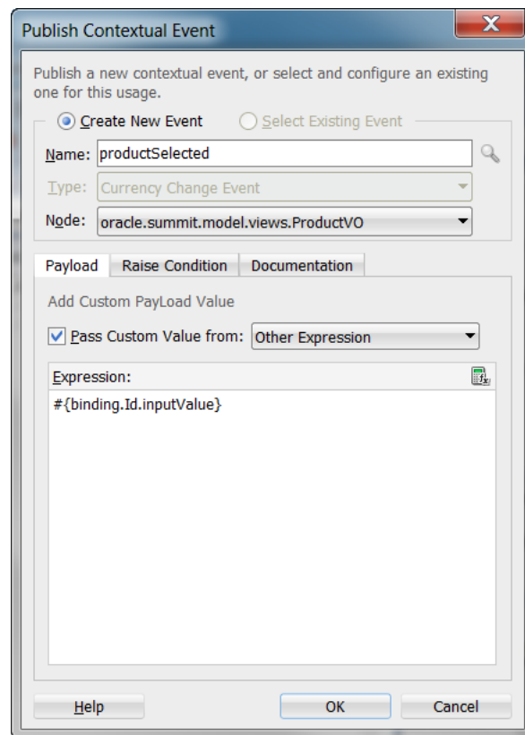
Figure 40–4 Publish a Contextual Event
