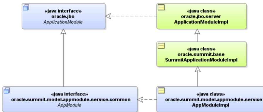
Figure 13–23 Custom Client Interface Extends the Base ApplicationModule Interface
