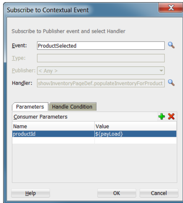
Figure 40–5 Subscribe to a Contextual Event
