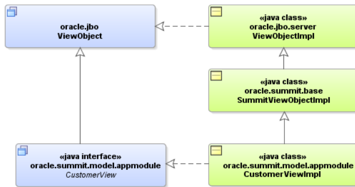
Figure 13–24 Custom View Object Interface Extends the Base ViewObject Interface
