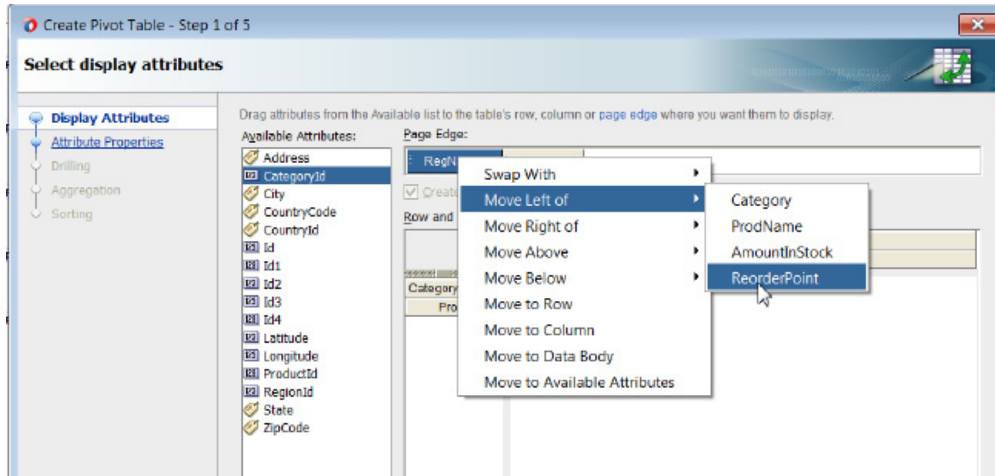
Figure 36-3 Display Attributes Context Menu
