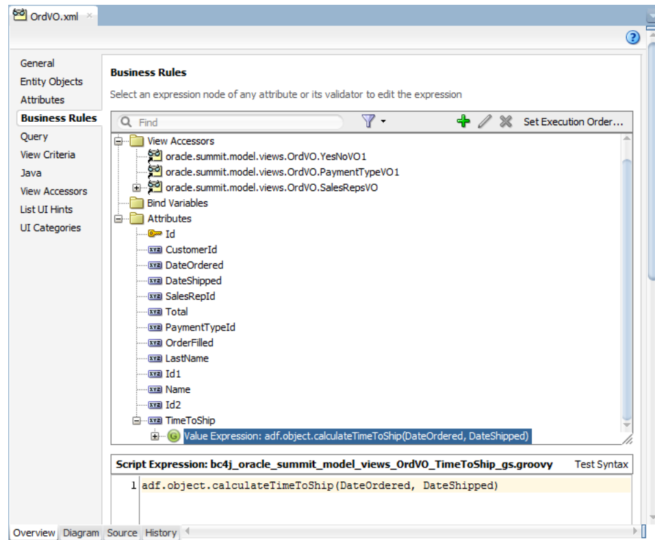
Figure 3–13 Overview Editor’s Business Rules Page Shows All Expressions Used by a Business Component
