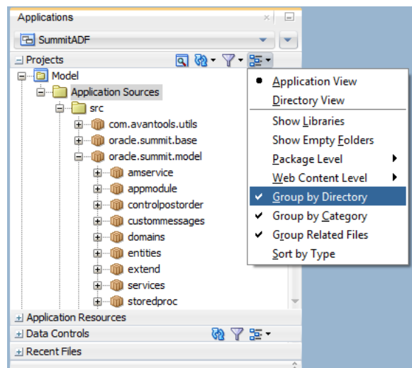
Figure 4–10 Toggleing the Display of Separate Content Path Directories
