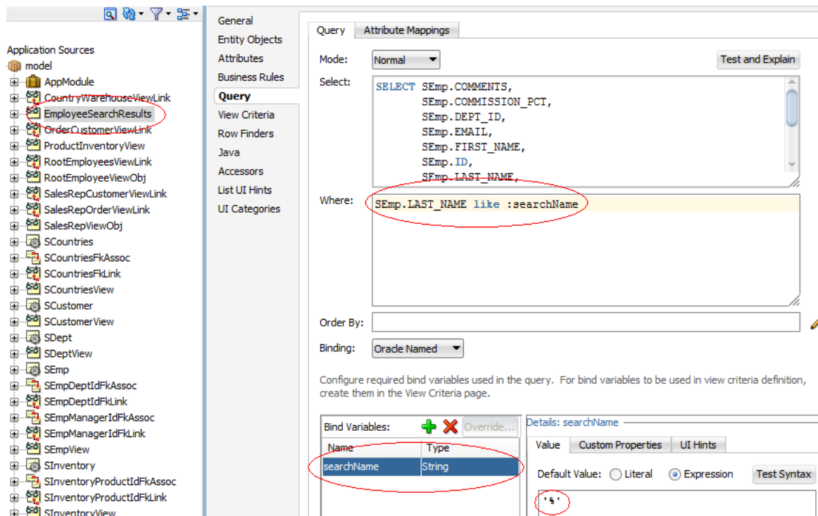
Figure 39–19 EmployeeSearchResults View Object
