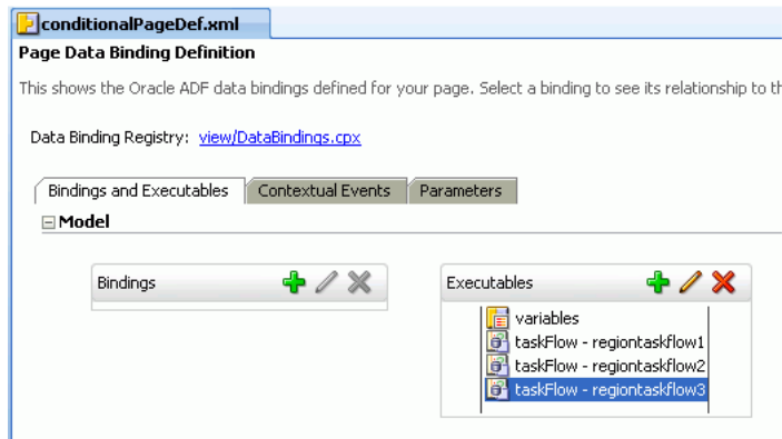
Figure 23–8 Task Flow Bindings for ADF Region Configured for Activation
