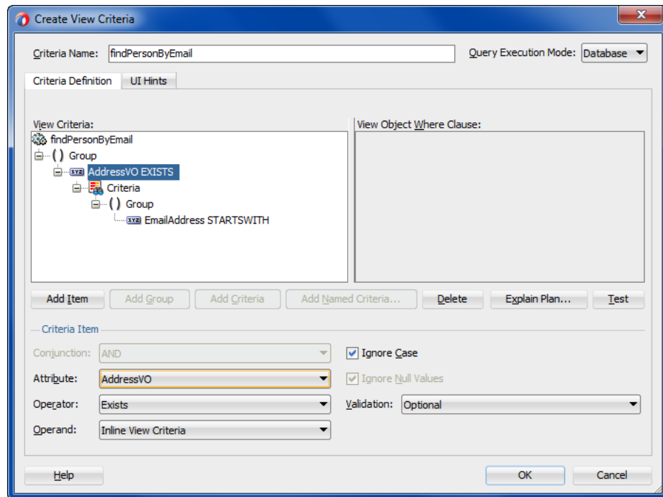
Figure 6–15 Edit View Criteria Dialog with Inline View Criteria Specified
