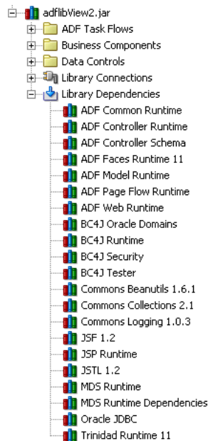
Figure 44-4 Resources Window Showing adflibView2.jar Extension Libraries
