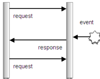
Figure 47-5 Long Polling Mode
