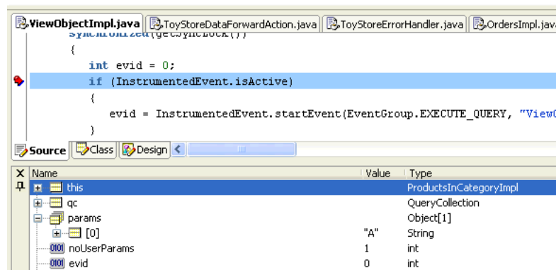
Figure 42–51 Symbol Information Displayed in the Debugger
