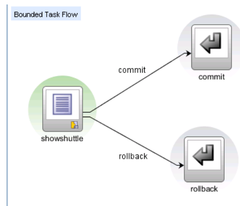
Figure 24–3 Task Flow Return Activities in Called Bounded Task Flow
