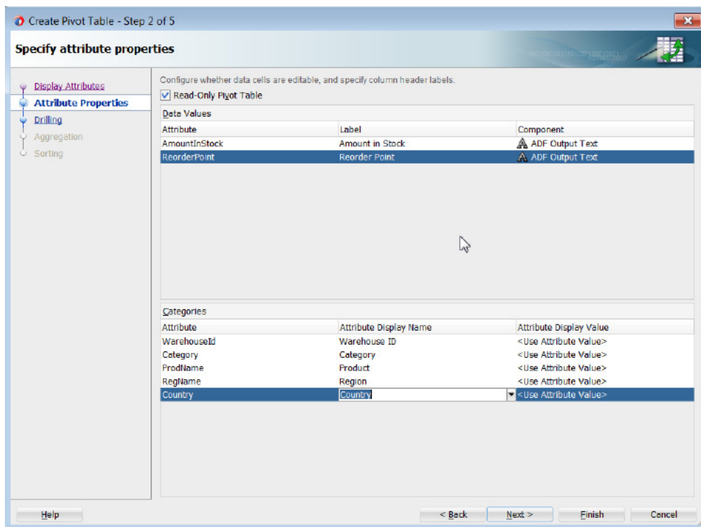
Figure 36-5 Specify Attribute Properties Page of Create Pivot Table Wizard
