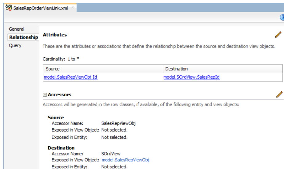
Figure 39–15 View Link Between Summit Sales Representatives and Orders
