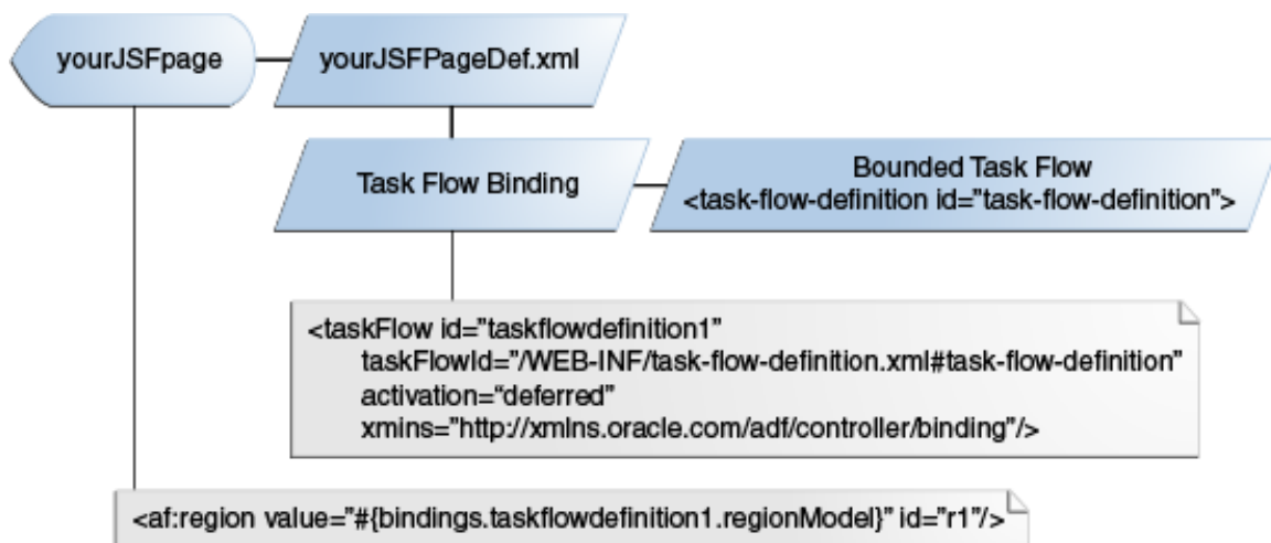
Figure 23–1 ADF Region Referencing a Bounded Task Flow
