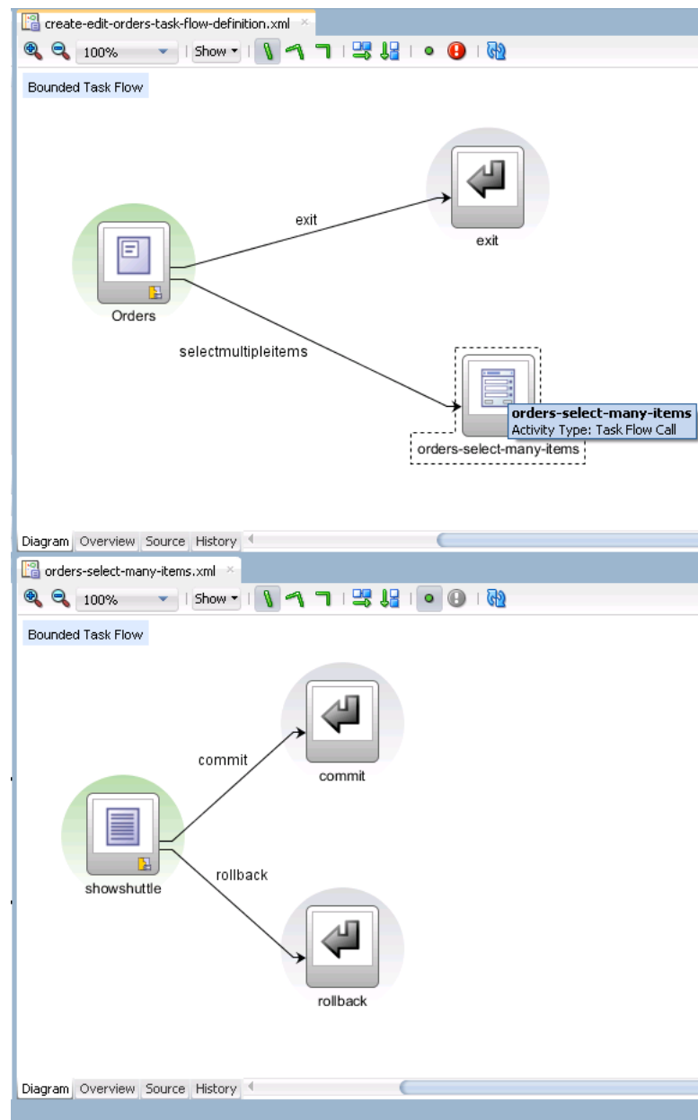
Figure 25–1 Task Flow Activities to Invoke a Modal Dialog in Summit ADF Sample Application
