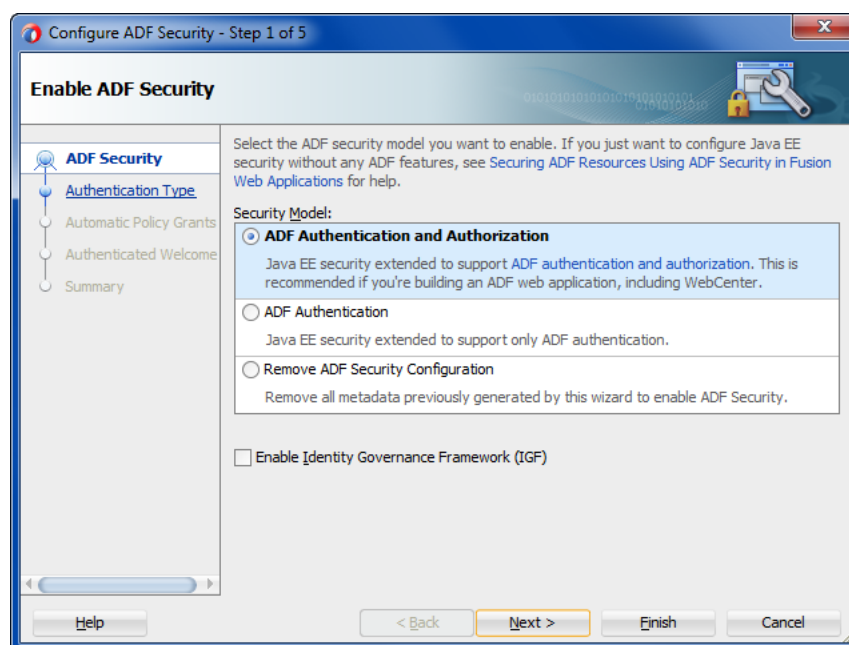
Figure 41–2 Using the Configure ADF Security Wizard to Enable Security-Aware Resources
