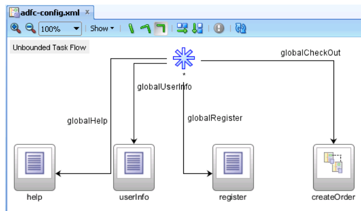
Figure 20–6 Wildcard Control Flow Rule With Single Wildcard
