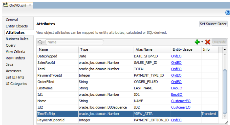
Figure 35–4 OrdVO View Object in Summit ADF Sample Application
