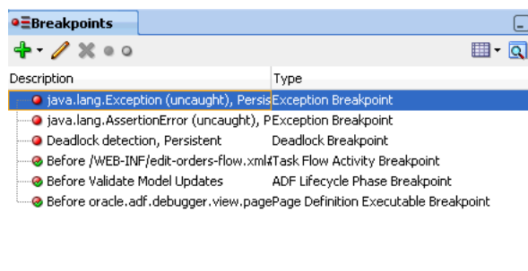
Figure 42–30 Breakpoints Window Showing ADF Declarative and Java Code Breakpoints
