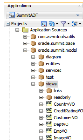
Figure 1–11 View Objects in the Summit ADF Sample Application
