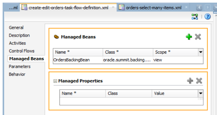
Figure 26–1 Managed Beans in the create-edit-orders-task-flow-definition
