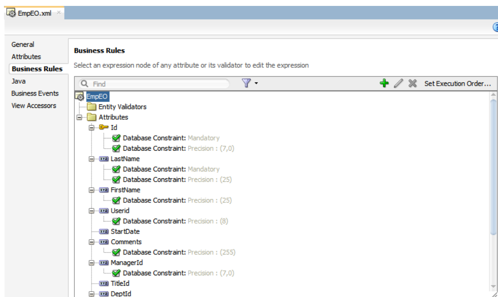
Figure 1–15 Setting Validation in the Overview Editor
