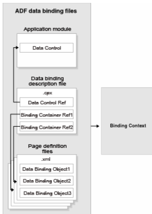
Figure 17–13 ADF File Binding Runtime Usage
