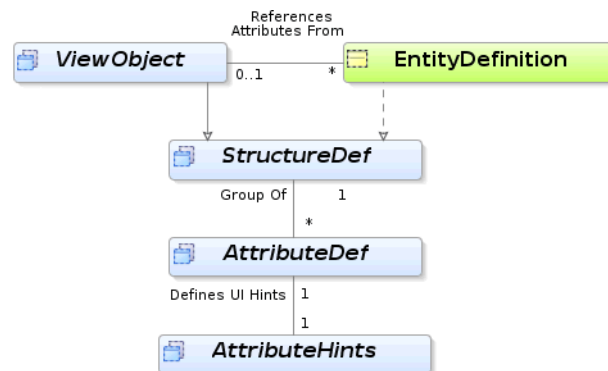
Figure 16–7 Runtime Metadata Available for View Objects and Entity Objects
