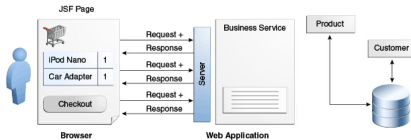
Figure 50-2 Web Applications Use the Stateless HTTP Protocol
