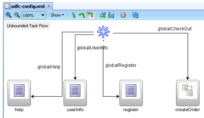
Figure 20–3 Unbounded Task Flow
