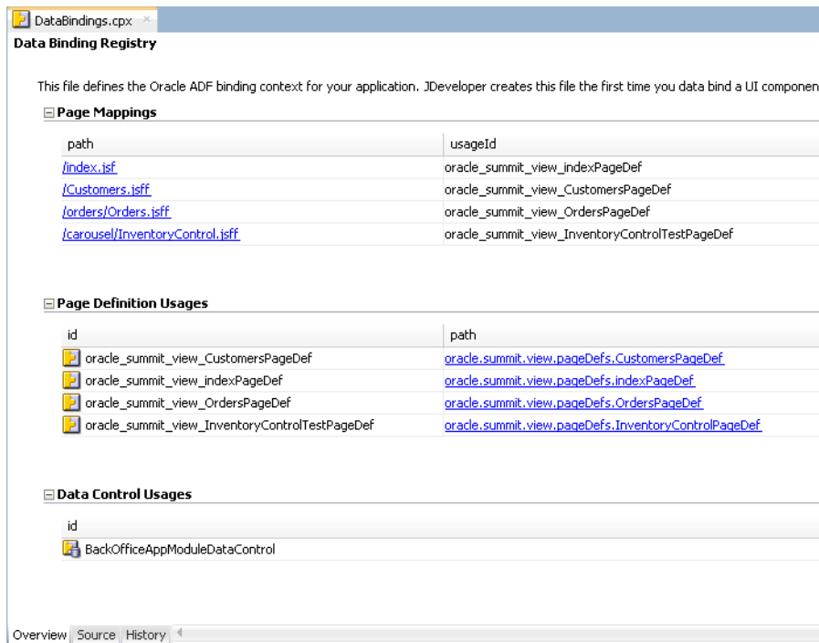
Figure 17–14 DataBindings.cpx File in the Overview Editor
