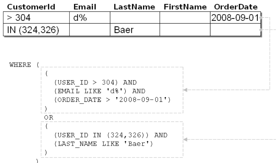
Figure 5-33 View Object Automatically Translates View Criteria Groups into Additional Runtime WHERE Filter
