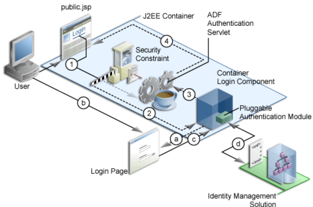
Figure 41–28 ADF Security Explicit Authentication
