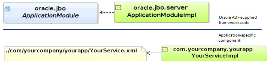
Figure 3–11 Component with Custom Java Class
