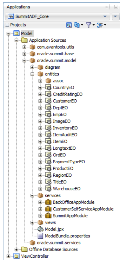
Figure 3–7 Organization of ADF Business Components in the Core Summit ADF Sample Application
