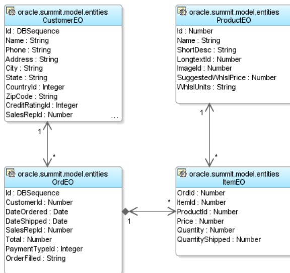
Figure 4–9 UML Diagram of Business Domain Layer
