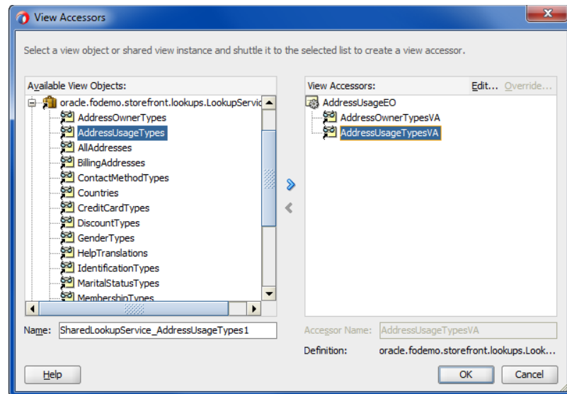
Figure 14–6 Defining a View Accessor on an Entity Object
