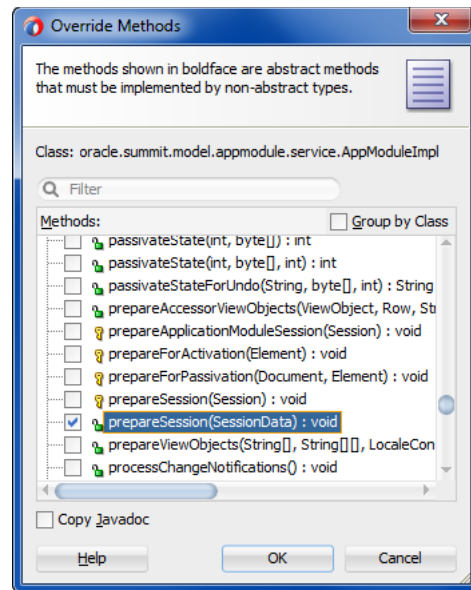
Figure 13–27 Overriding a Built-in Framework Method
