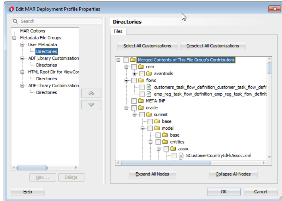
Figure 49–4 Selecting Items for the MAR Deployment Profiles
