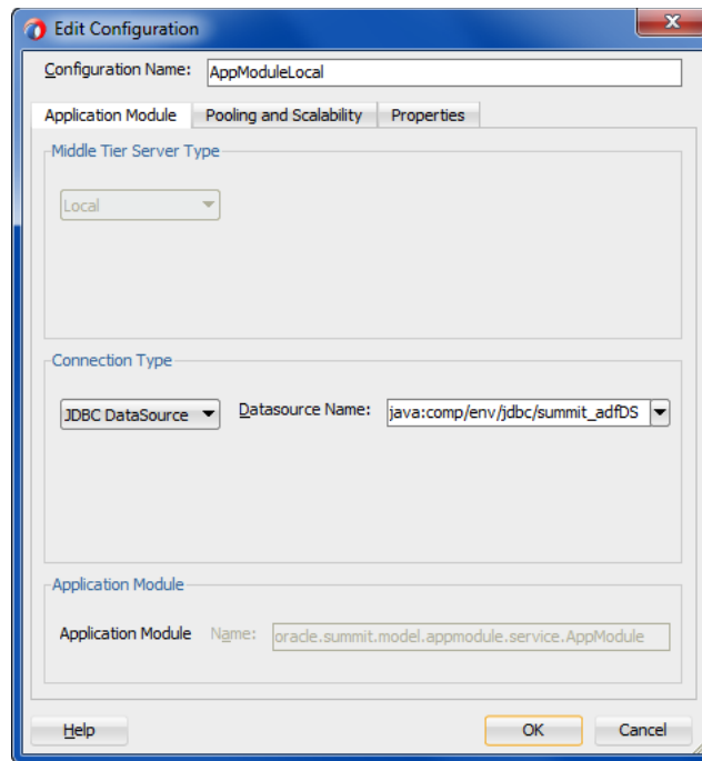
Figure 13–13 bc4j.xcfg File Configurations Displayed by Edit Configuration Dialog
