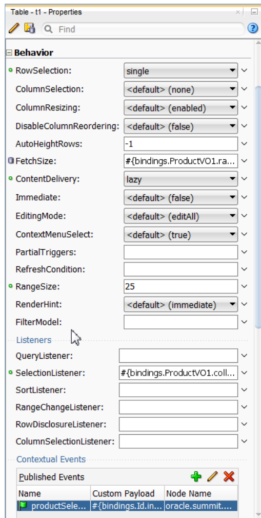
Figure 40–2 Contextual Events Panel in the Properties Window
