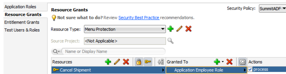
Figure 41–35 Creating a Grant for a Custom Resource in the Overview Editor
