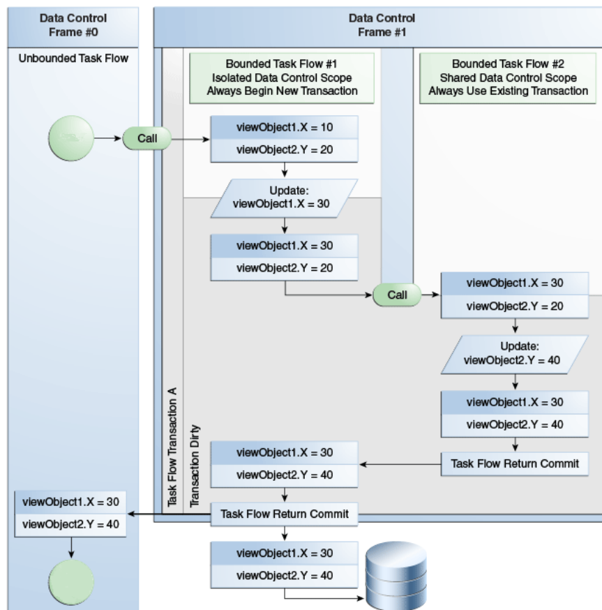
Figure 24–6 Guaranteed Joined Transactions
