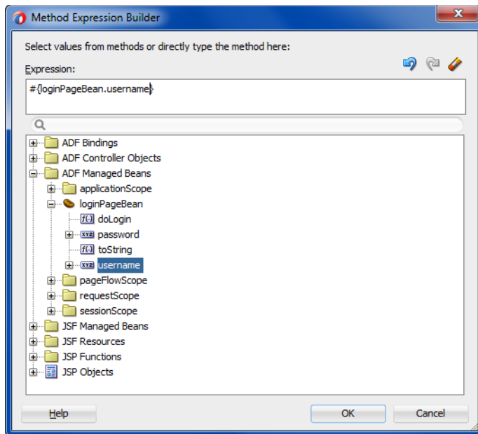
Figure 41–22 username Selection in Expression Builder Dialog
