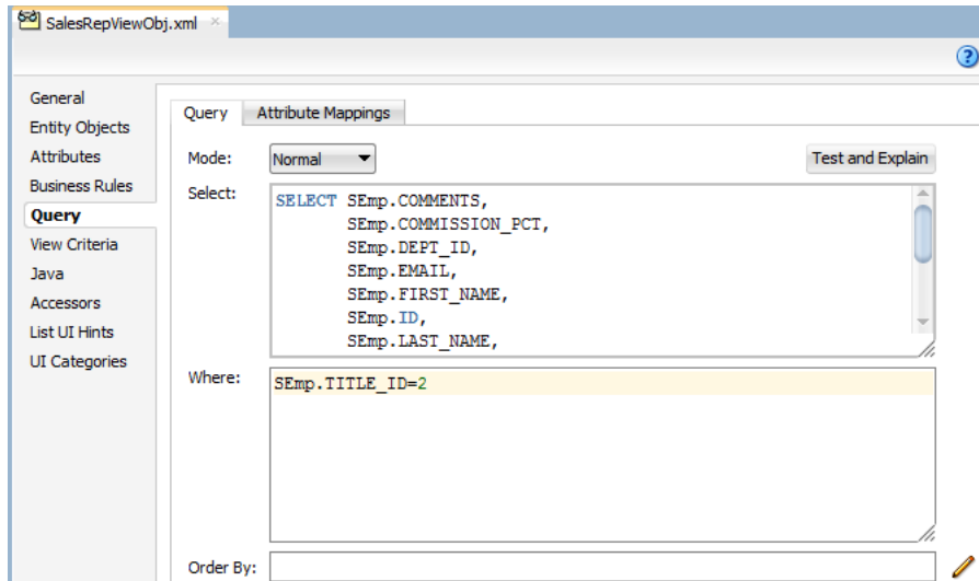
Figure 35–12 SalesRepViewObj View Object in Summit DVT Sample Application
