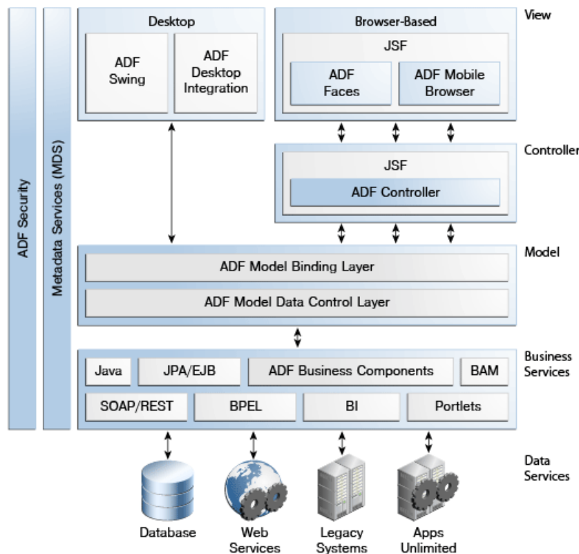
Figure 17-1 ADF Model within the ADF Architecture
