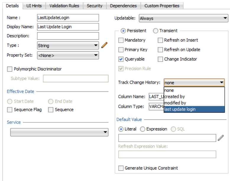
Figure 4–16 New History Types in the Overview Editor
