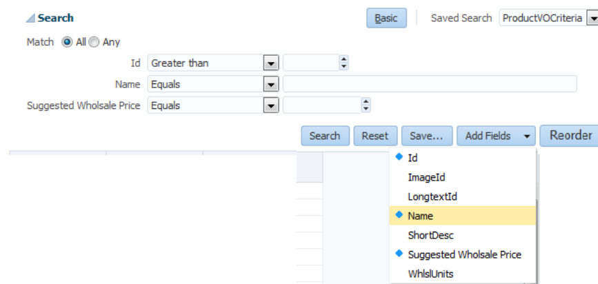
Figure 33–7 Dynamically Adding Search Criteria Fields at Runtime
