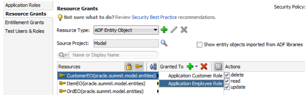
Figure 41–14 Granting to an Application Role for an ADF Entity Object in the Overview Editor
