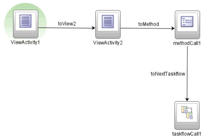
Figure 20–5 Task Flow with Activities and Control Flow Cases
