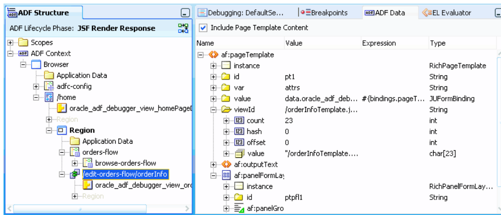
Figure 42–41 Page Selected for the ADF Data Window
