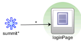
Figure 20–7 Wildcard Control Flow Rule with Trailing Wildcard
