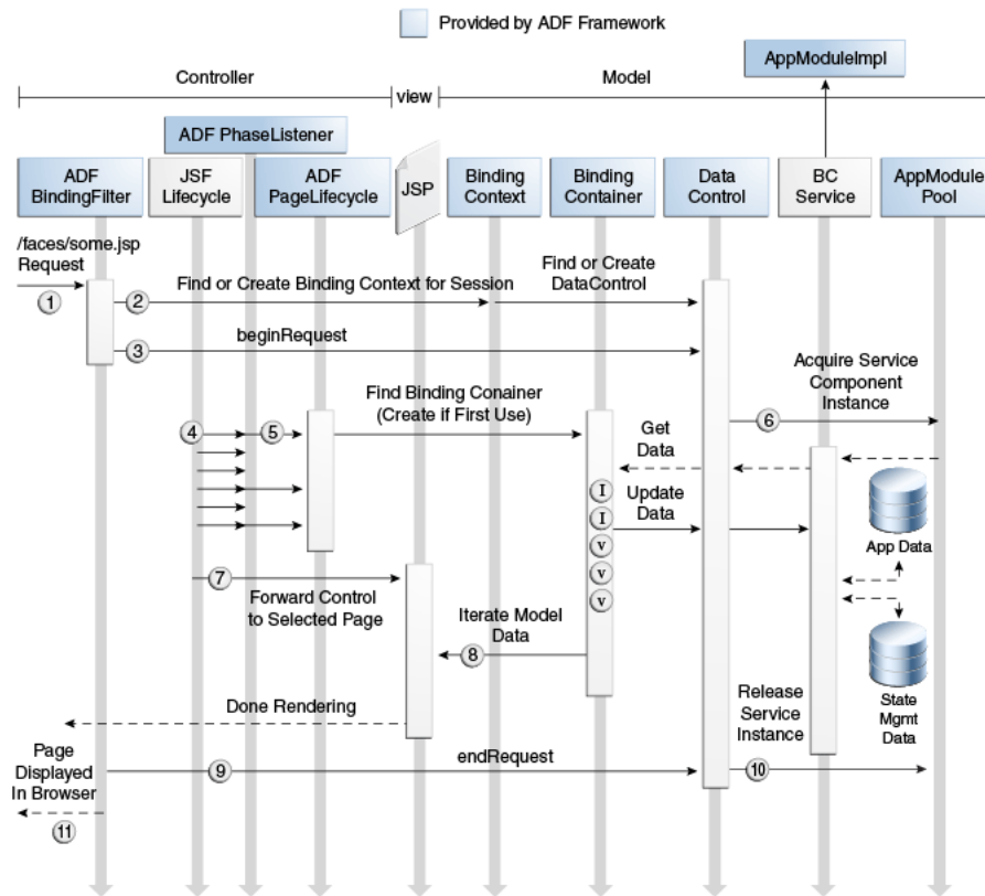
Figure 27-1 Lifecycle of a Web Page Request Using JSF and Oracle ADF
