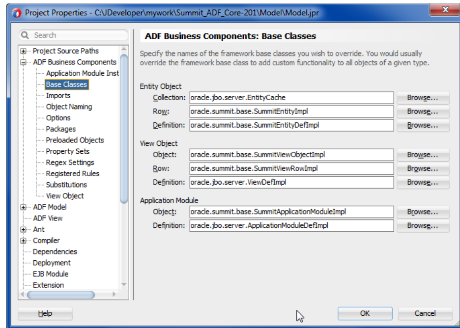
Figure 16–3 Setting Project-Level Preferences for Business Component Base Classes
