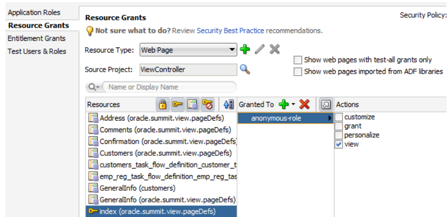
Figure 41–10 Granting to an Application Role for an ADF Page Definition in the Overview Editor
