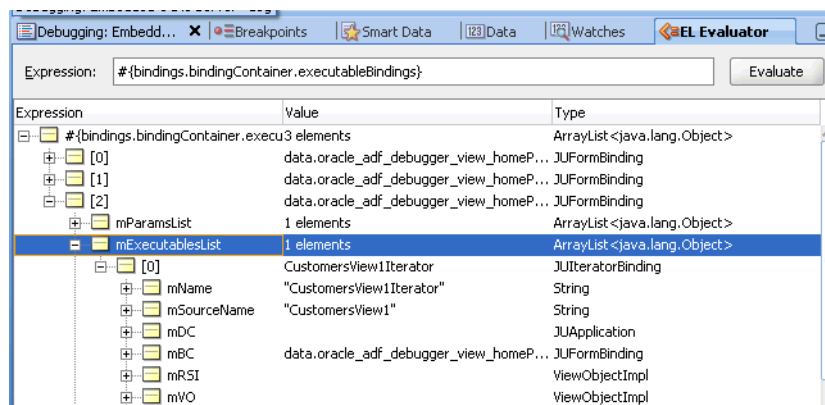
Figure 42–14 EL Expression Evaluated
