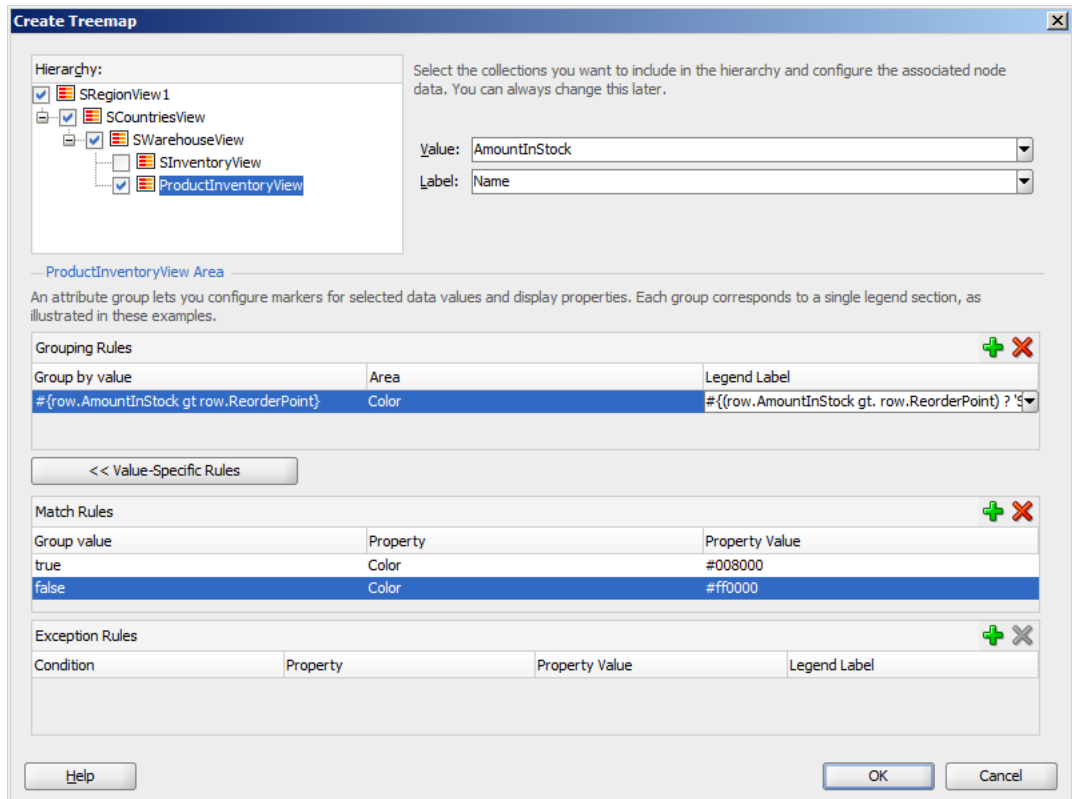
Figure 39–30 Treemap Showing Match Rules for an Attribute Group
