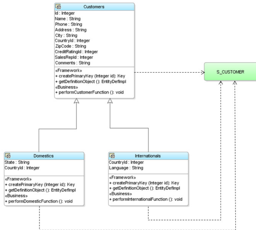
Figure 4–18 Distinguishing Customers, Domestics, and Internationals Using Inheritance
