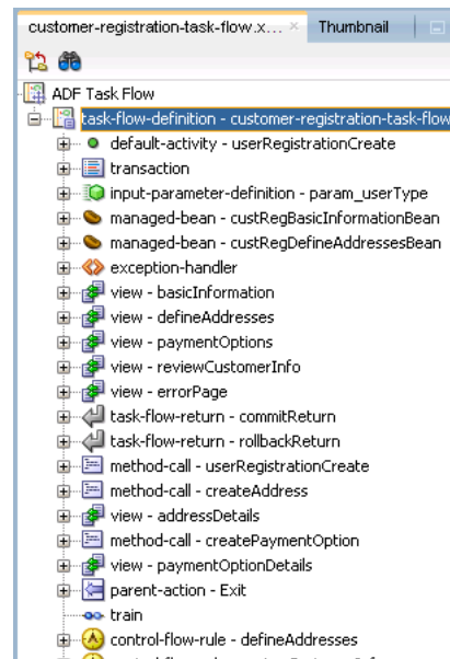
Figure 24–1 Task Flow in the Structure Window
