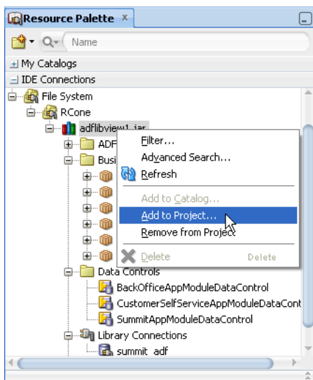
Figure 44–16 Adding the ADF Library JAR to the Project
