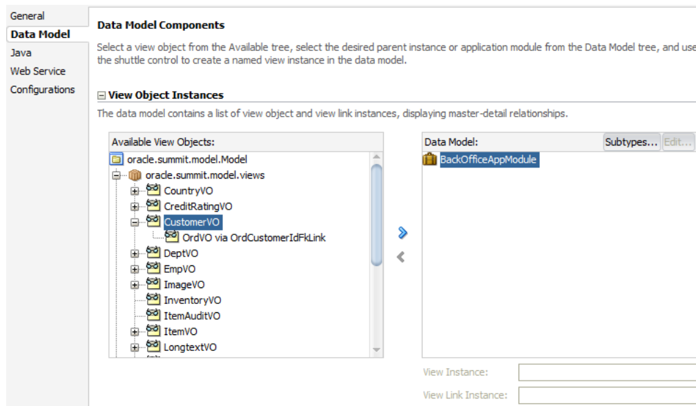
Figure 13-4 Master View Object Selected
