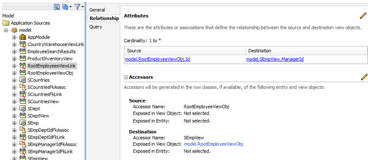
Figure 39–7 RootEmployeesViewLink in the Summit ADF DVT Sample Application
