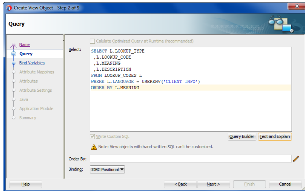
Figure 14–3 Create View Object Wizard, SQL Query for Lookup Table
