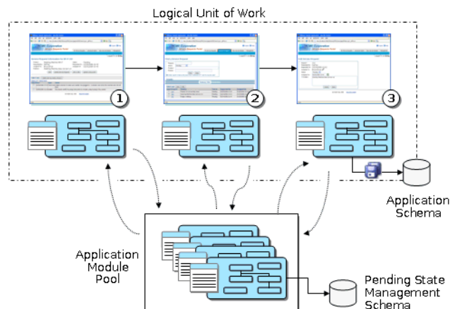
Figure 13–19 Using Pooled Application Modules Throughout a Multipage, Logical Unit of Work
