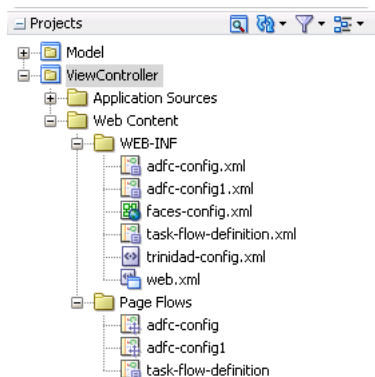
Figure 20–11 Application with Two Unbounded Task Flow XML Source Files
