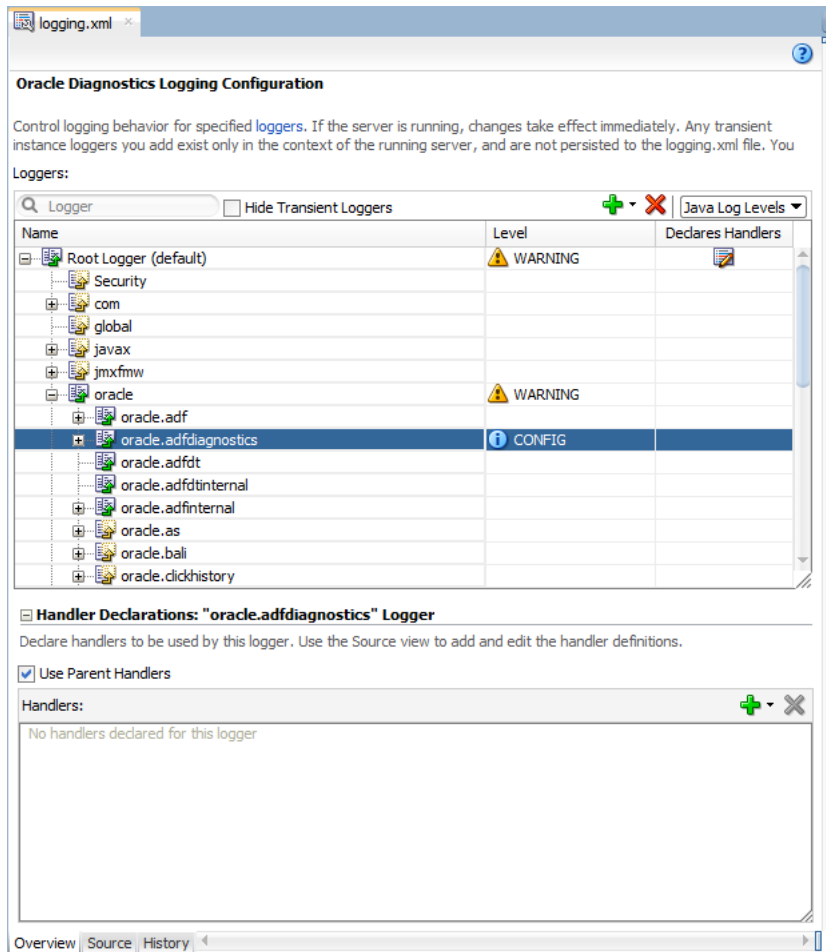
Figure 42–4 Editor for Oracle Diagnostic Logging Configuration
