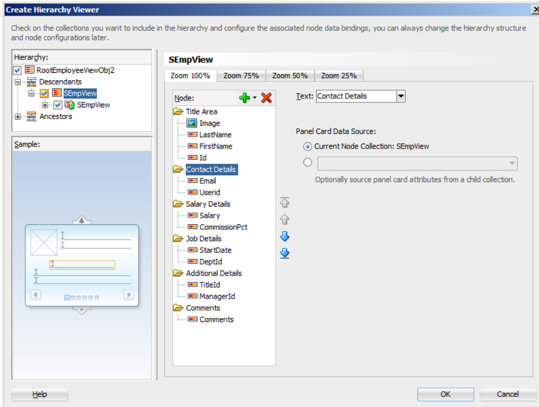
Figure 39–10 Hierarchy Viewer Configured With Default Panel Card Data Source
