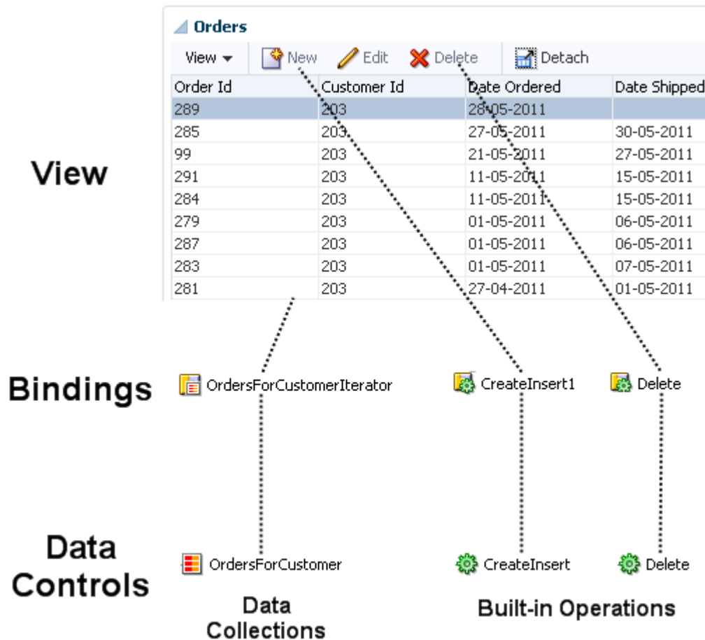
Figure 17-2 Bindings Connect UI Components to Data Controls
