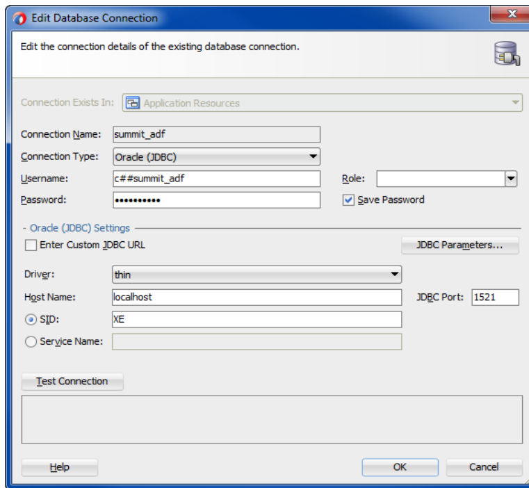
Figure 2–3 Edit Database Connection Dialog for a Summit ADF Sample Application
