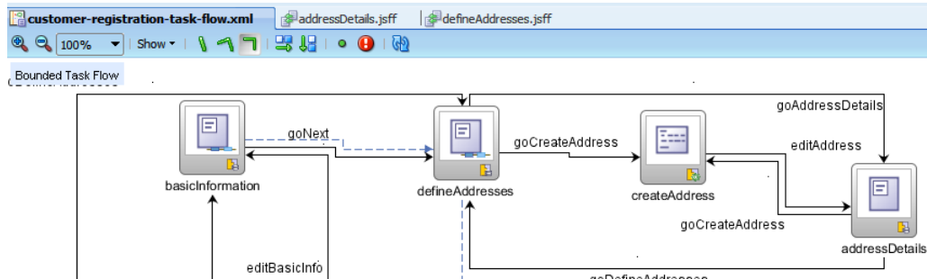
Figure 24–11 Task Flow Activities Grouped into One Train Stop
