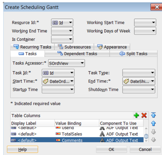
Figure 38–11 Create Scheduling Gantt Dialog
