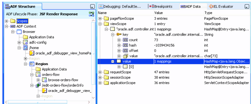
Figure 42–37 Scopes Node Selected in the ADF Structure Window
