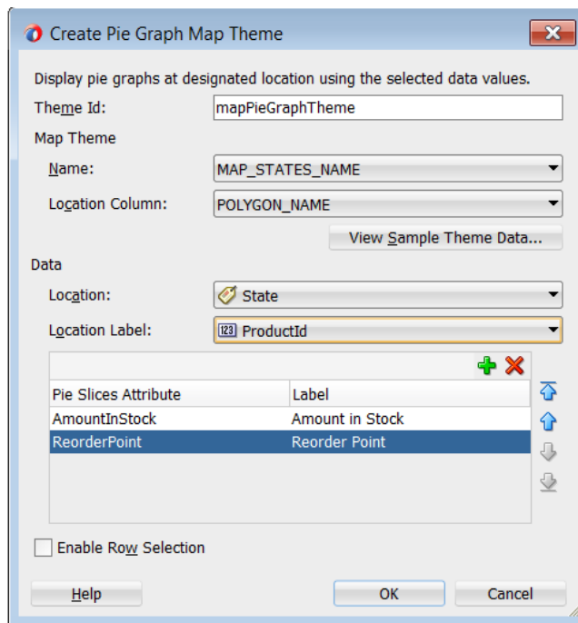
Figure 37–17 Create Pie Graph Map Theme for Inventory Levels by Product
