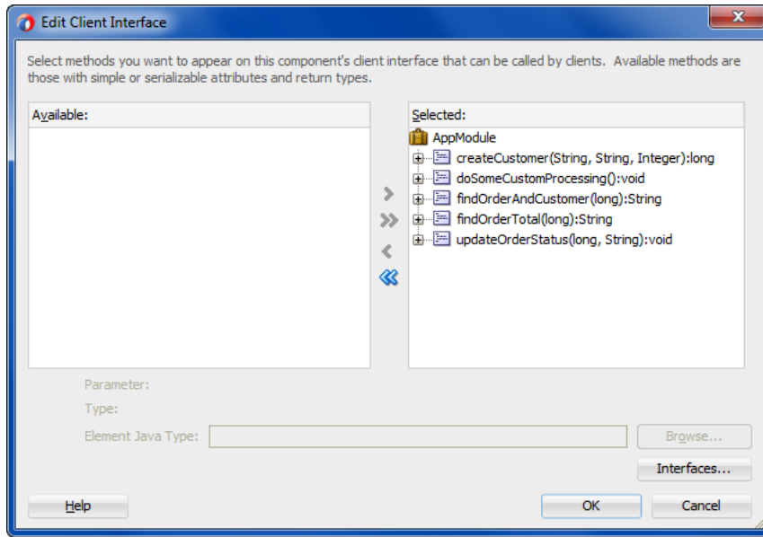
Figure 13–22 Public Methods Added to an Application Module's Client Interface
