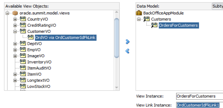
Figure 8–5 Master-Detail-Detail Hierarchy Created
