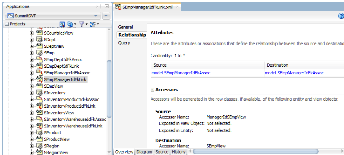
Figure 39–4 View Link Between Managers and Employees in the Summit ADF DVT Sample Application
