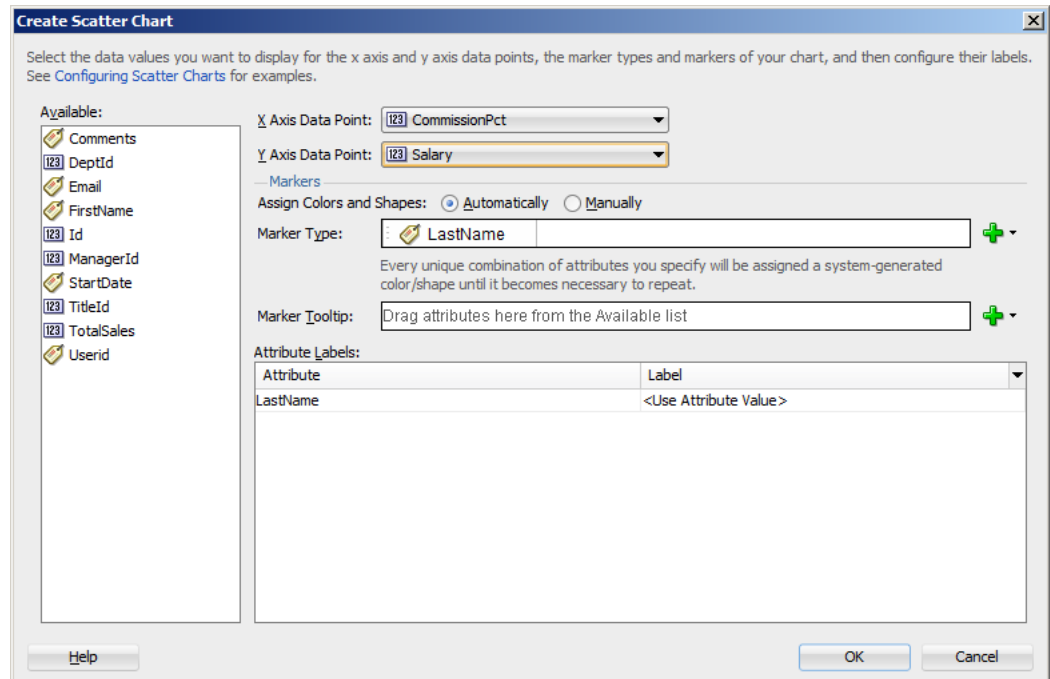
Figure 35–16 Create Scatter Chart Dialog
