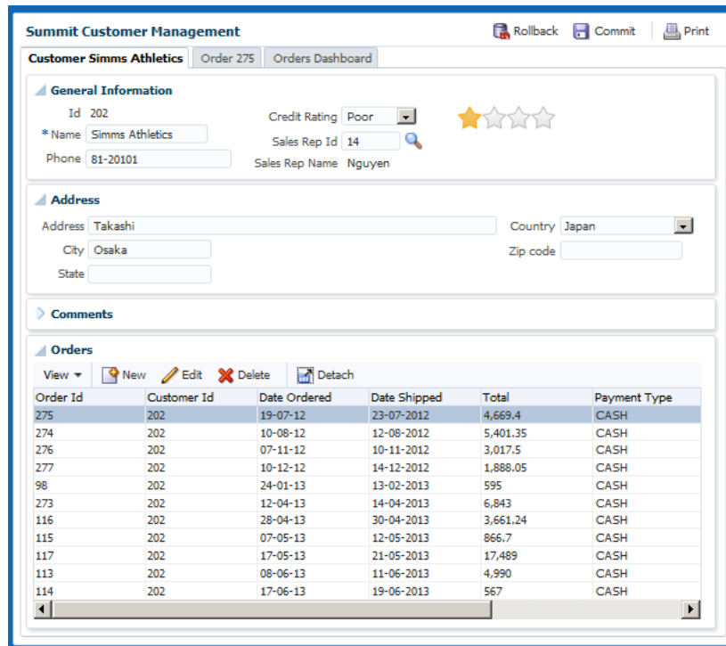
Figure 35–28 Rating Gauge in Summit ADF Sample Application
