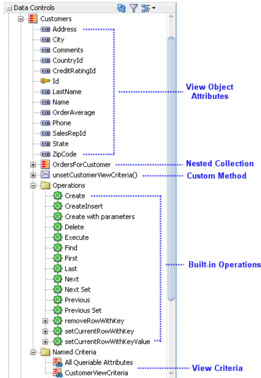
Figure 17-6 How View Objects Appear in the Data Controls Panel
