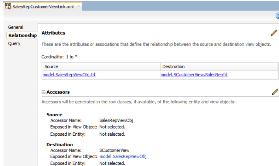
Figure 39–16 View Link Between Sales Representatives and Customers in the Summit ADF DVT Sample Application
