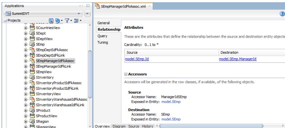
Figure 39–3 Association Between Manager and Employees in the Summit ADF DVT Sample Application
