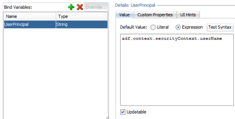
Figure 5–32 Groovy Expression Used to Set userPrincipal Bind Variable
