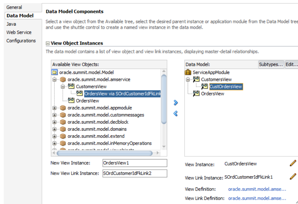
Figure 15–18 Data Model Contains Service View Instances
