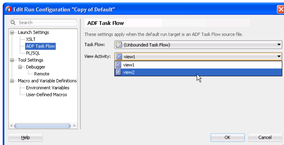
Figure 20-17 Edit Run Configuration Dialog
