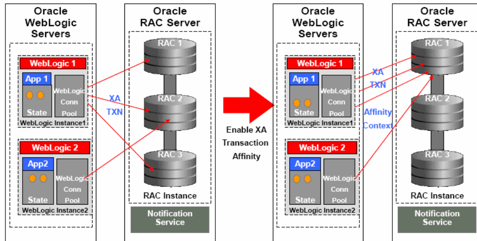
Figure 5-5 XA Affinity
