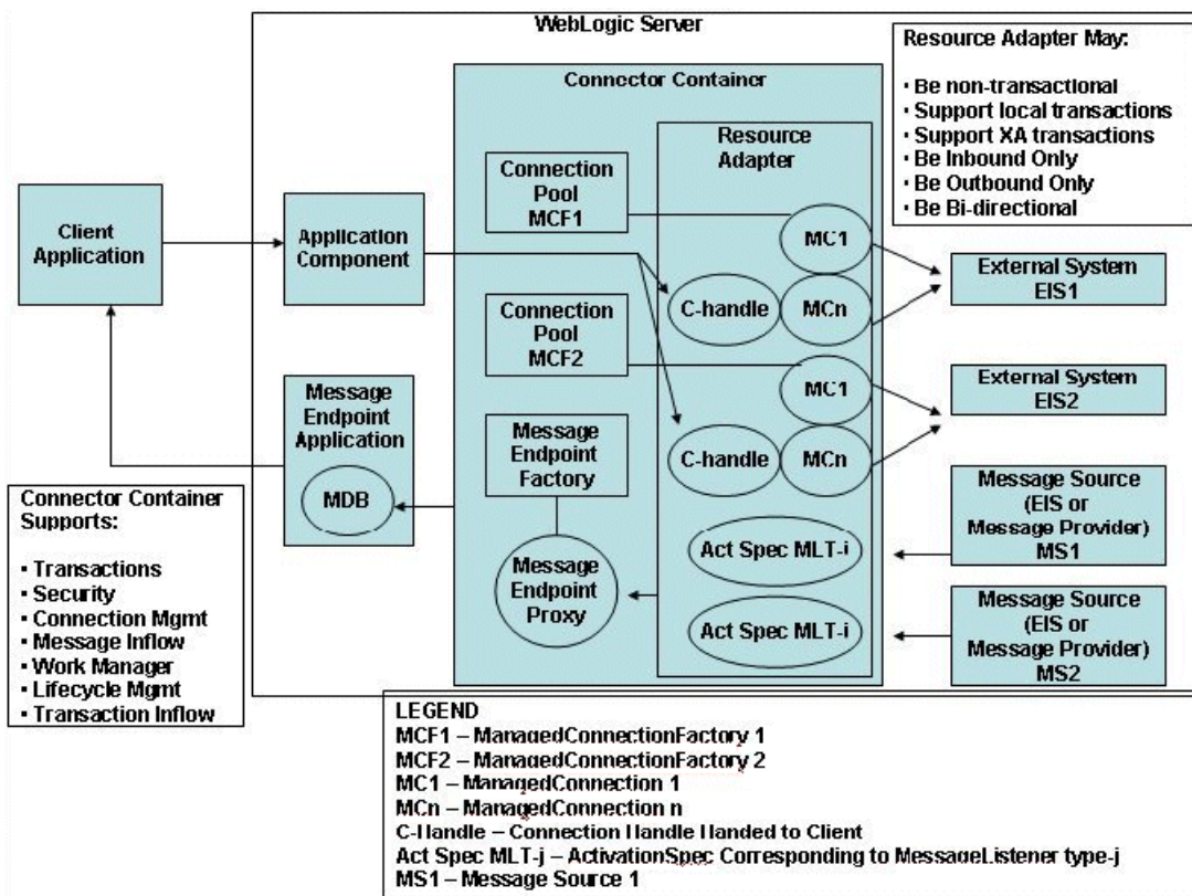
Figure 2–1 Connector Architecture Overview
