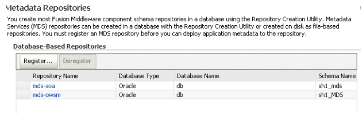
Figure 16-2 Registering an OWSM Repository
