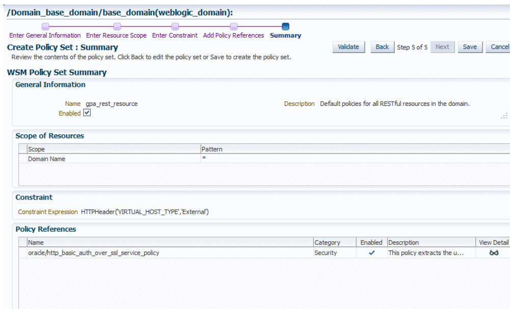
Figure 4–10 Summary Page in Create Policy Set Wizard
