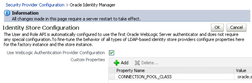
Figure 9–3 Identity Store Configuration Page
