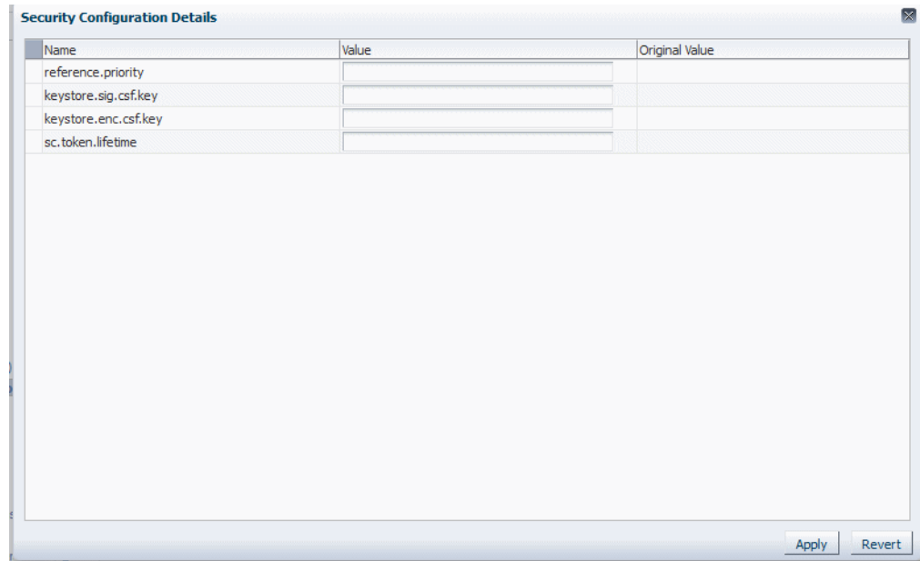
Figure 5-1 Overriding a Policy Configuration Property
