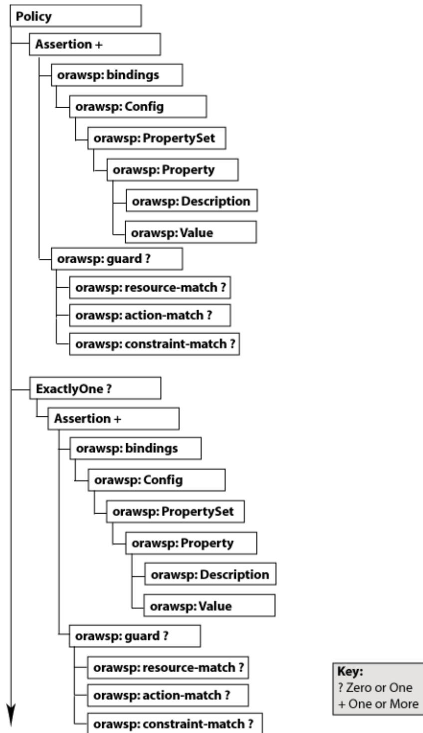
Figure B-1 Element Hierarchy of an Assertion
