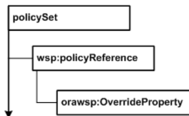
Figure C-1 Element Hierarchy of the Policy Set
