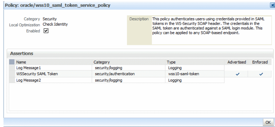
Figure 4-3 Viewing Details about a Policy
