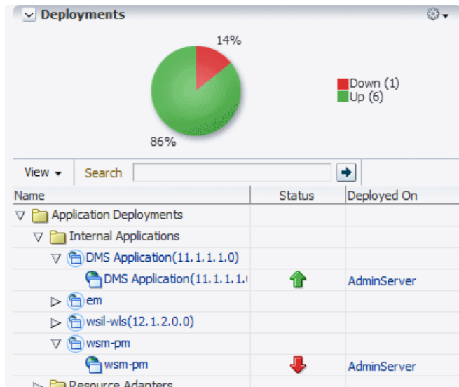
Figure 17–2 OWSM Policy Manager Shutdown (Farm Page)
