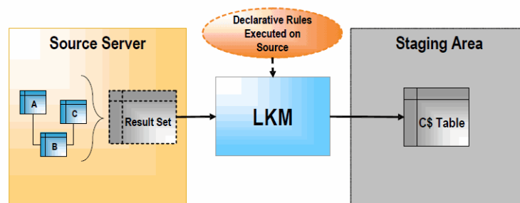
Figure 1–4 Loading Knowledge Module
