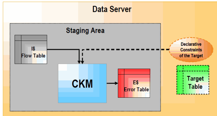
Figure 1–3 Check Knowledge Module (FLOW_CONTROL)
