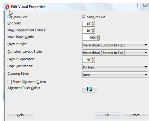
Figure 5-4 Class Diagram General Preferences for Visual Properties
