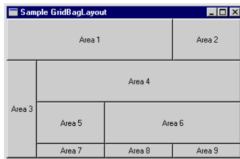
Figure 15–5 GridBagLayout
