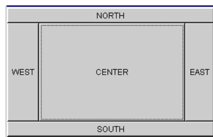
Figure 15–2 BorderLayout
