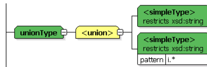
Figure 22–10 Union Component
