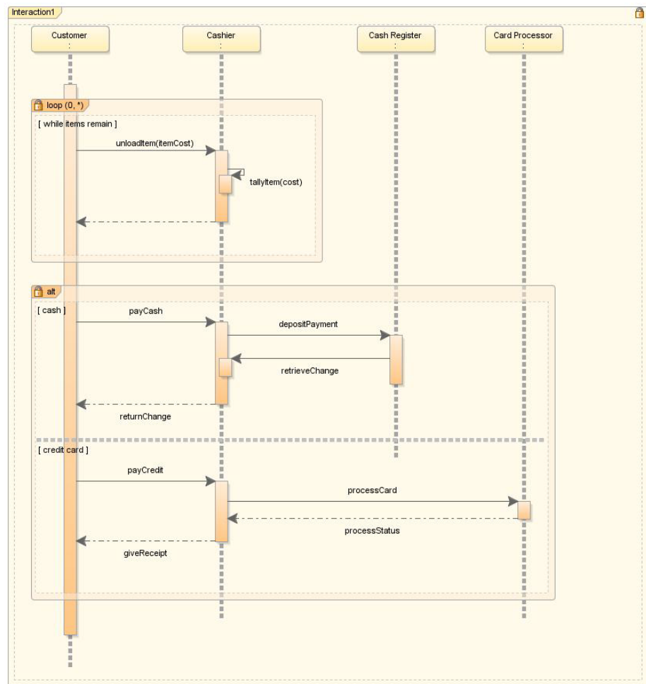
Figure 5–41 Typical Sequence Diagram with Combined Fragments
