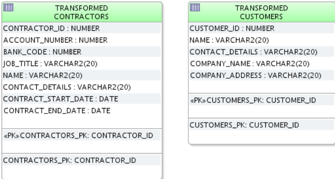
Figure 5–20 Leaf Classes Transformed Inheriting From Generalized Classes
