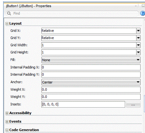
Figure 15–6 Layout Properties in Properties Window
