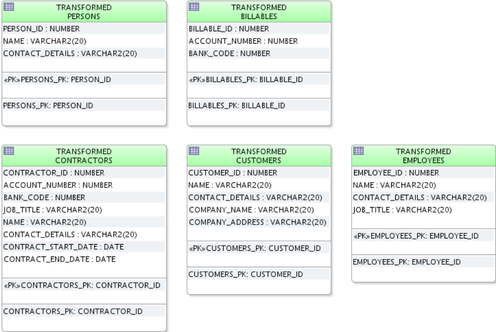
Figure 5–21 All Classes Transformed, Inheriting from Generalized Classes
