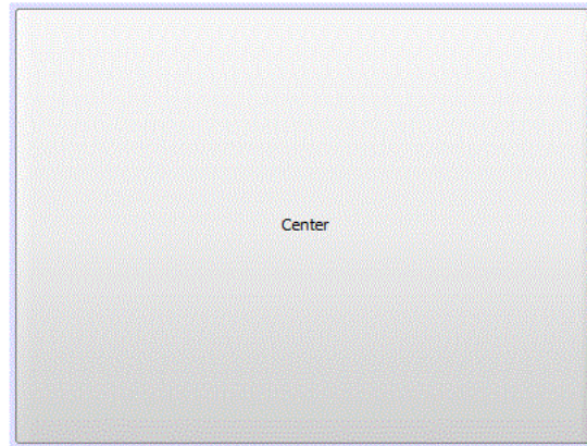
Figure 15–3 Card layout
