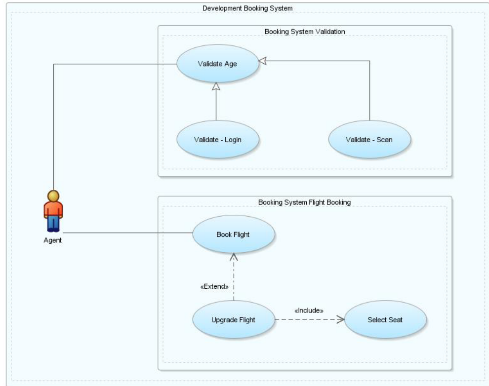
Figure 5–43 Typical Use Case Diagram
