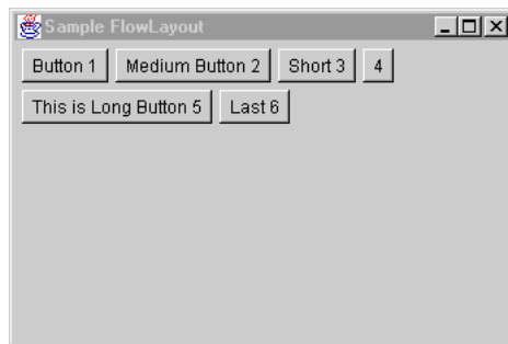
Figure 15–4 FlowLayout
