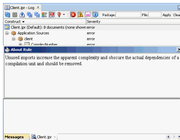
Figure 13–3 About Pop-up
