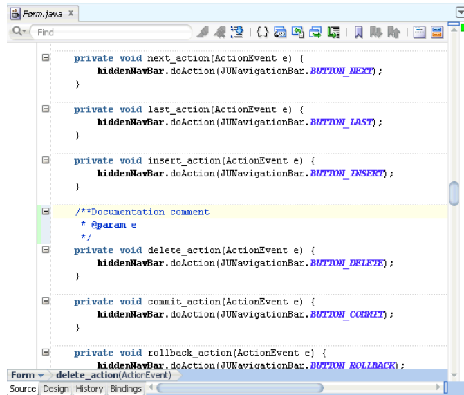
Figure 11–8 Javadoc Comments
