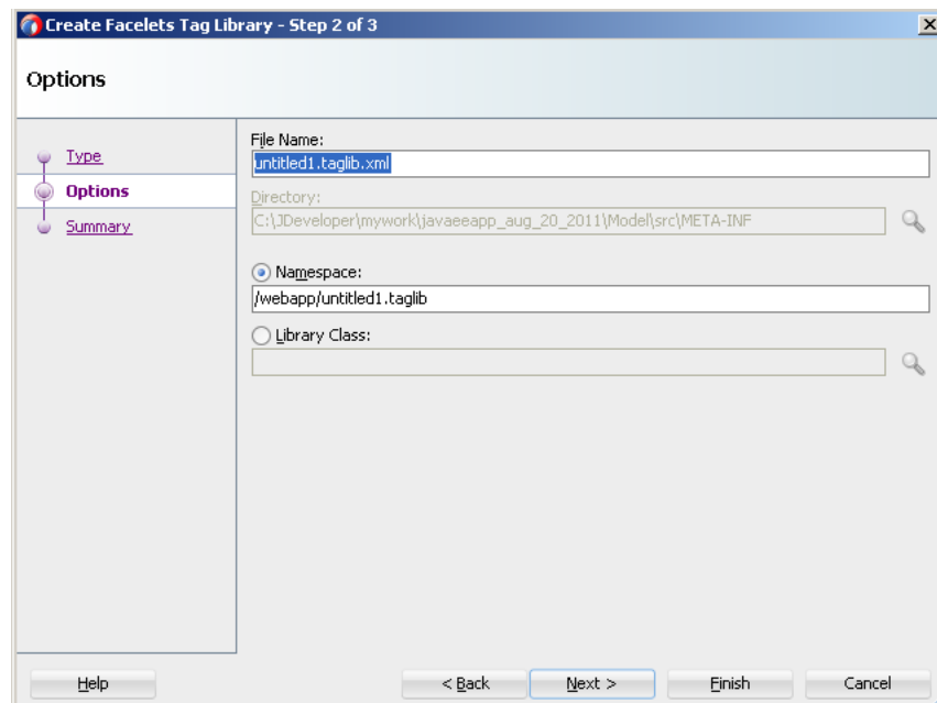
Figure 18–24 Facelets Tag Library Wizard
