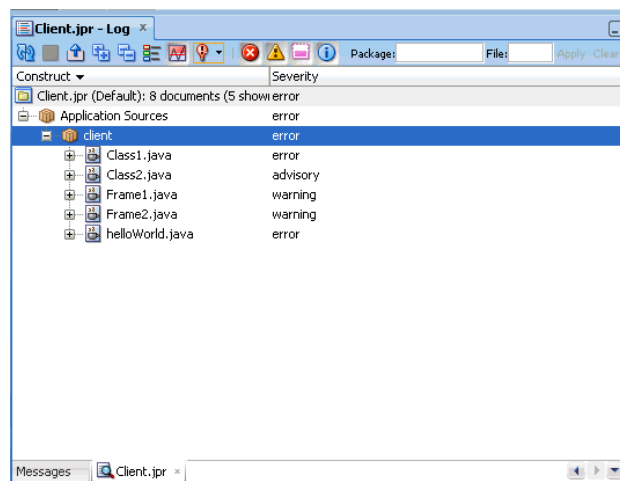
Figure 13–2 Audit Report
