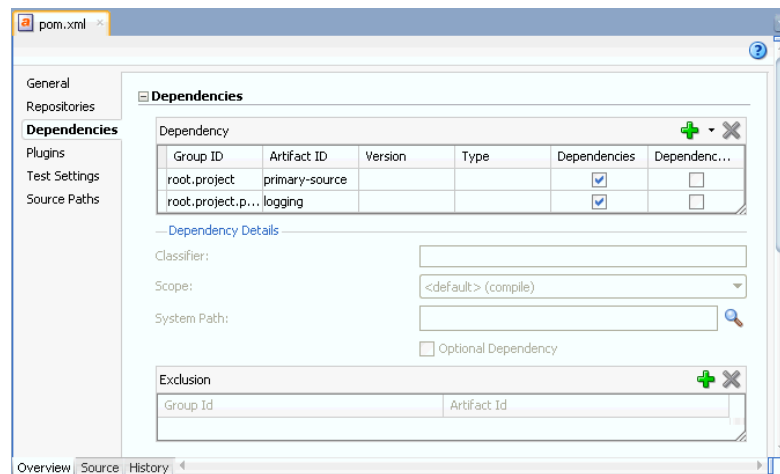
Figure 12–2 Maven Dependencies
