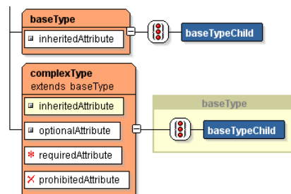
Figure 22–8 complexType Component
