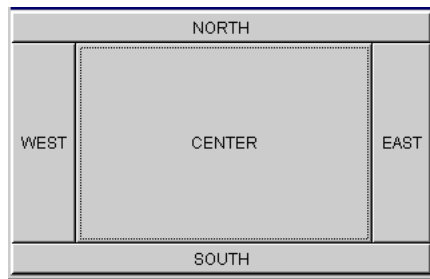
Figure 15–1 BorderLayout
