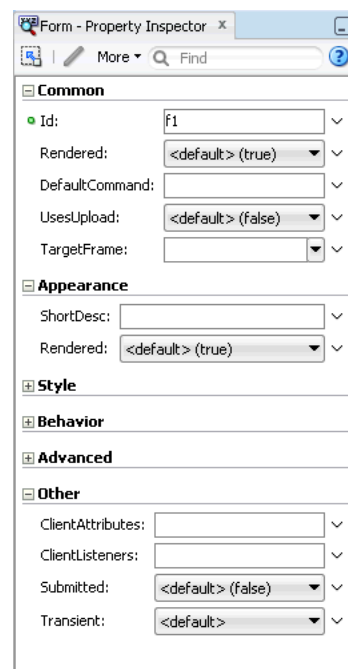
Figure 18–5 Properties Window
