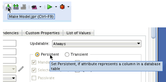
Figure 10–2 InfoTips
