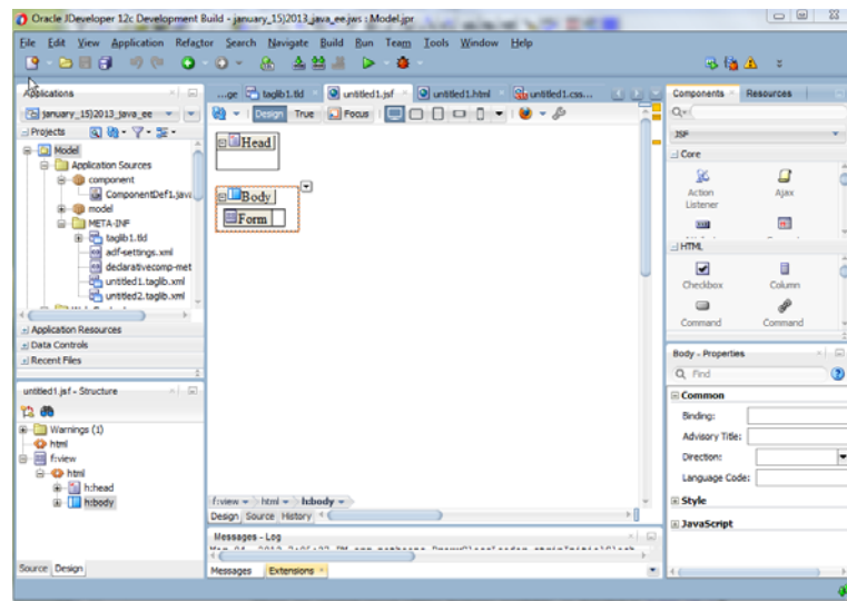
Figure 18–2 Visual Editor For a JSF Page
