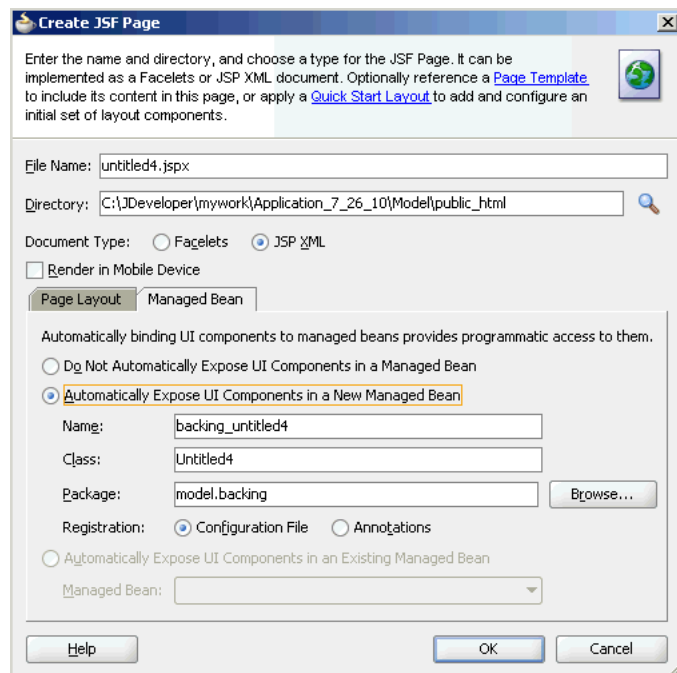
Figure 18–14 Create JSF Dialog - Create Managed Bean Tab
