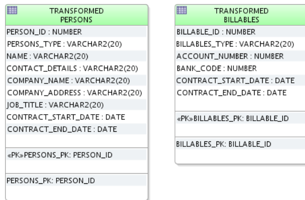
Figure 5–19 Transformed Root Classes
