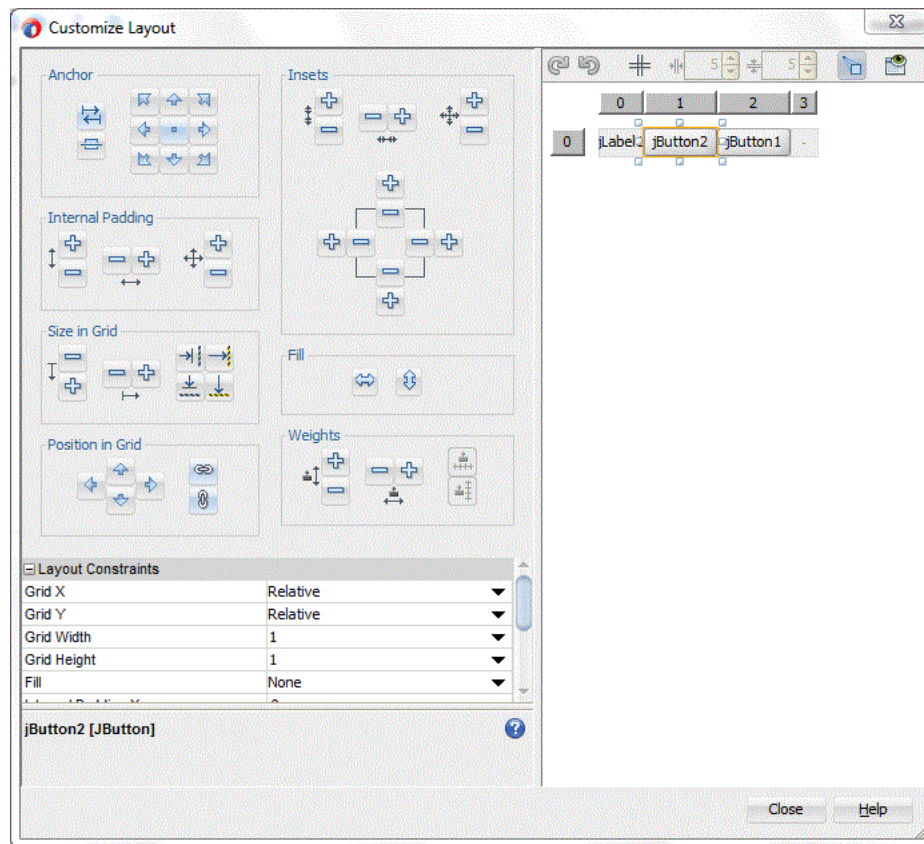
Figure 15–7 Customize Layout Dialog
