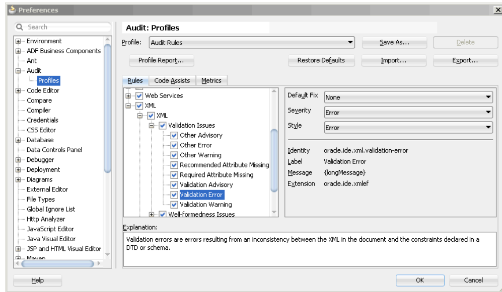
Figure 13–1 Audit Profiles Page
