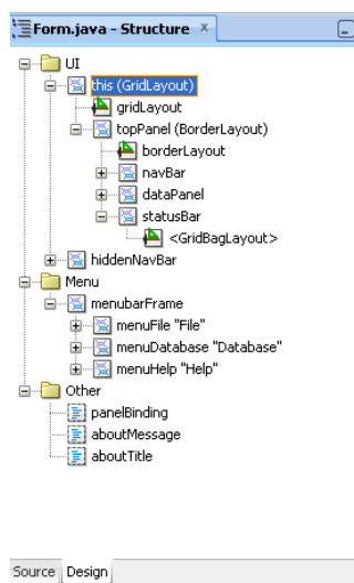
Figure 11–6 Structure Window for Java File
