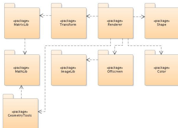
Figure 5–8 Grid Diagram Layout Example
