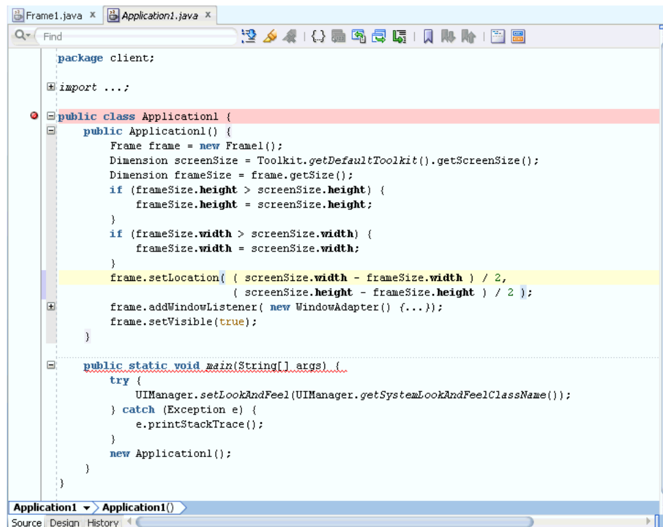
Figure 14-7 Breakpoint in Source Editor
