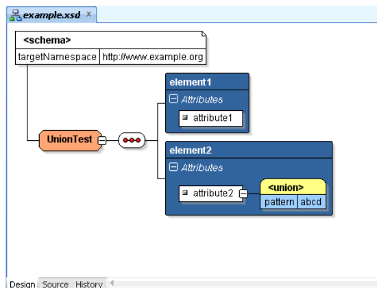
Figure 22-2 Schema in XSD Visual Editor
