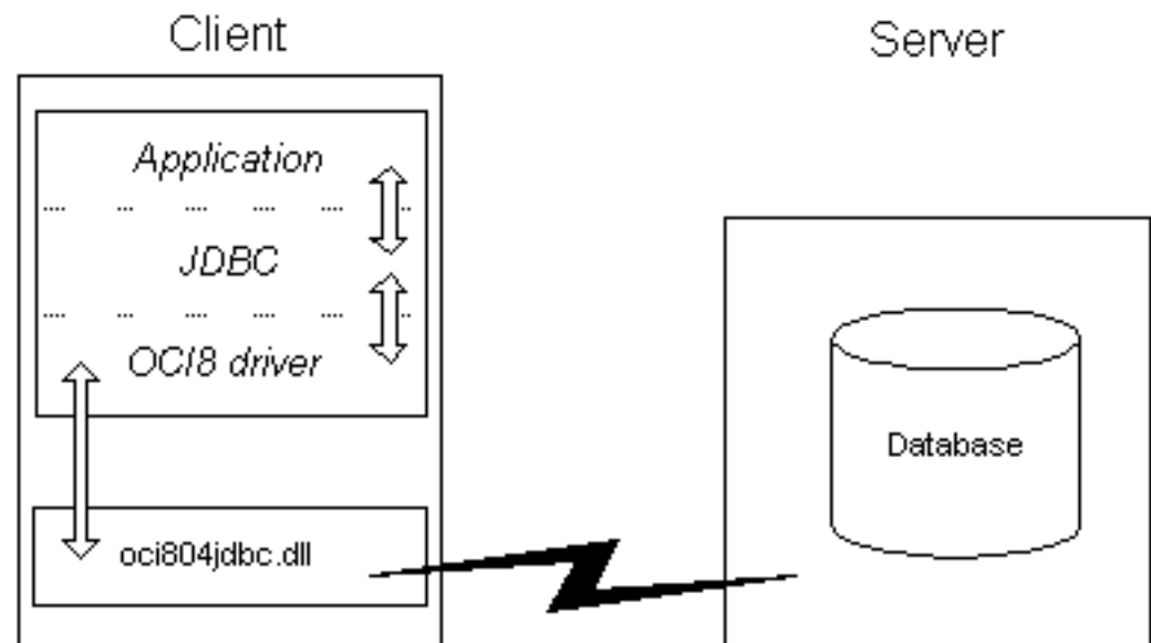
Figure 28–2 Oracle JDBC OCI Drivers
