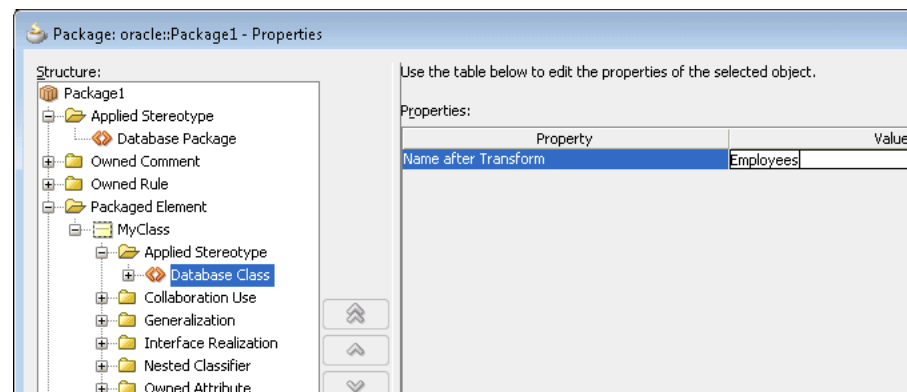
Figure 5–28 Package Properties Dialog Showing Resulting Class Name for UML Transformation
