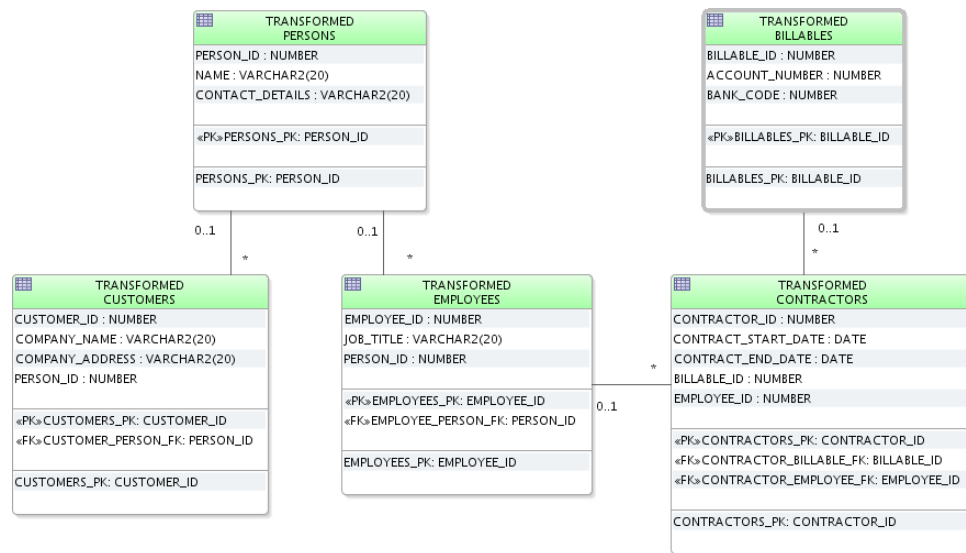
Figure 5–22 All Classes Transformed with Foreign Keys
