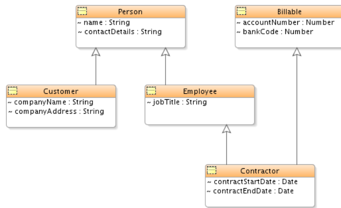
Figure 5–18 Diagram Showing Two Root and Three Leaf Classes
