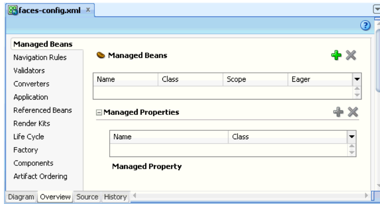
Figure 18–7 Overview Editor for JSF Configuration File
