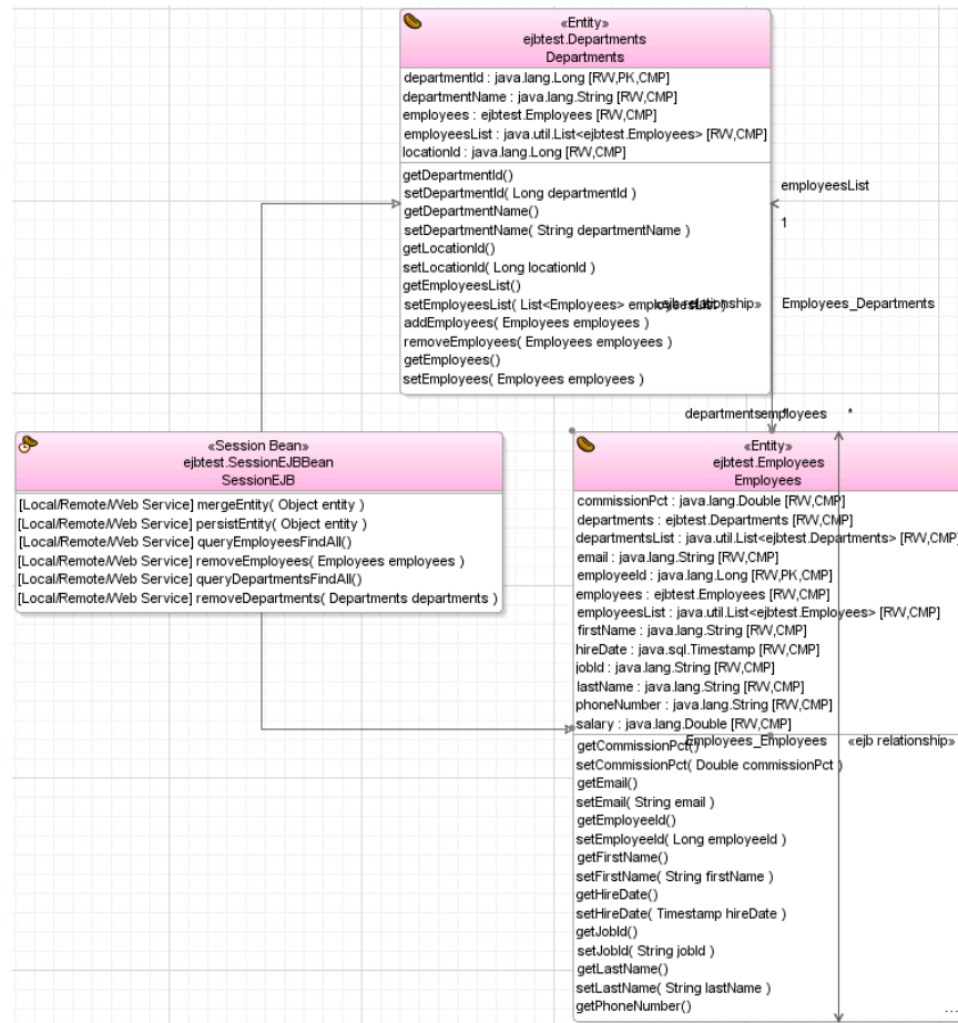
Figure 5–35 EJB/JPA Components Diagram
