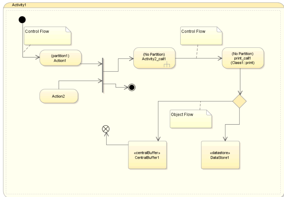
Figure 5–37 Sample Activity Diagram Showing Elements
