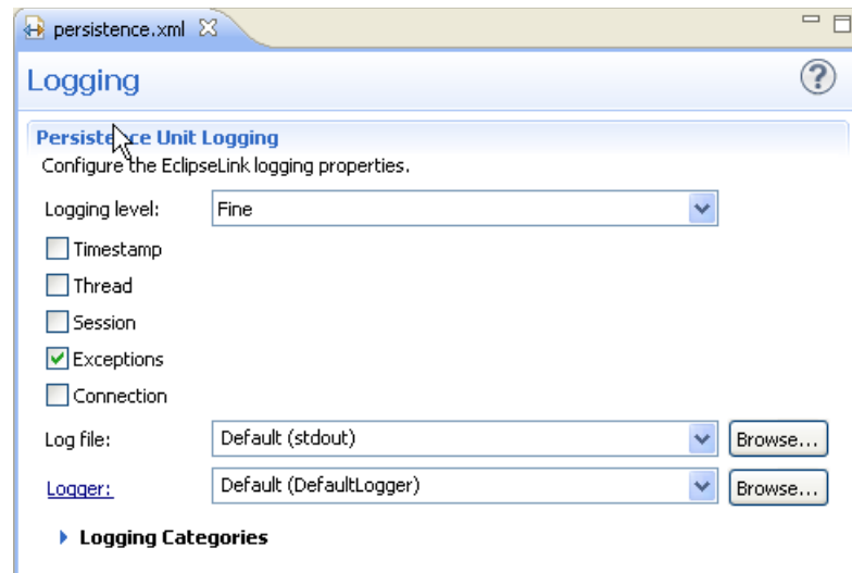
Figure 8–17 Logging Tab in the persistence.xml Editor
