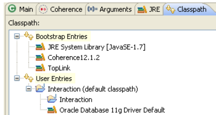
Figure 9-4 Classpath for the DatabaseCache Program
