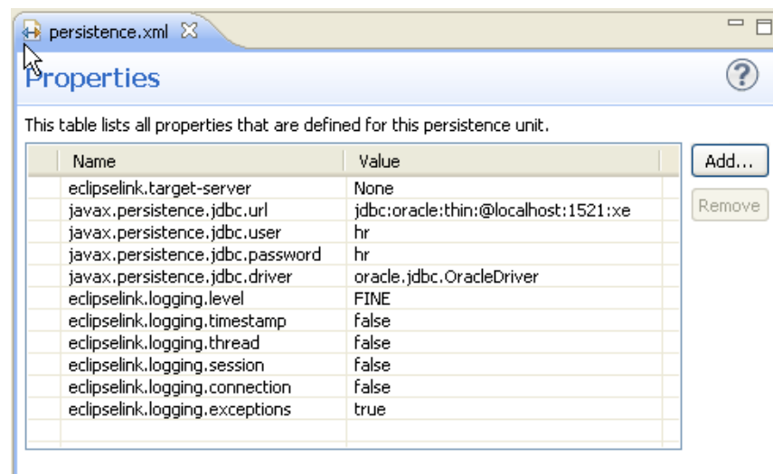
Figure 8–18 Properties Tab in the persistence.xml Editor
