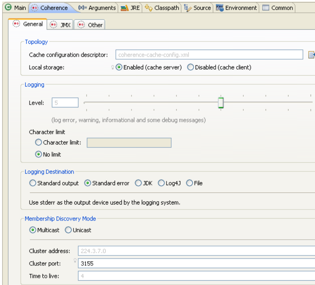
Figure 2–10 Coherence Tab of the Run Configurations Dialog Box
