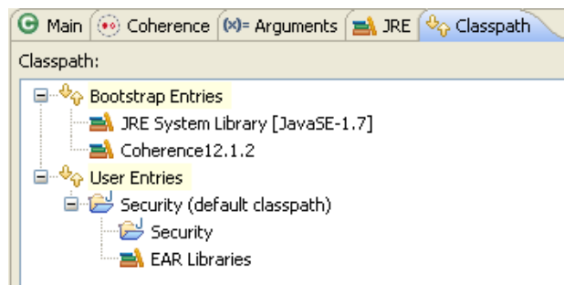
Figure 10-1 Class Path for the Security Cache Server
