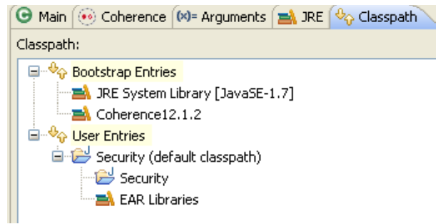
Figure 10–5 Classpath Tab for the AccessControlExample Program
