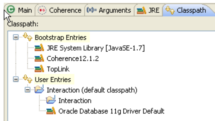
Figure 9–1 Classpath for the CoherenceCacheServer Executable
