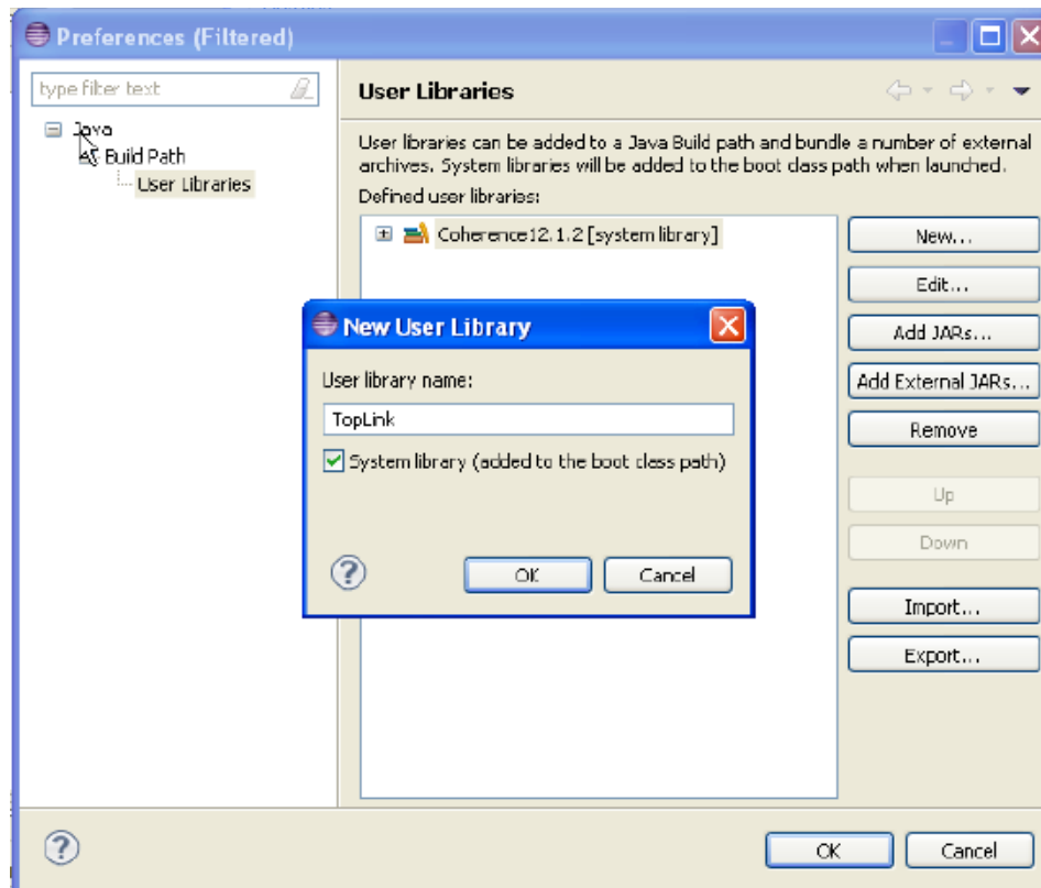
Figure 8–5 Adding the EclipseLink JPA Library
