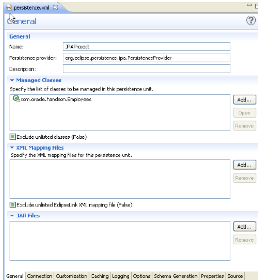
Figure 8–15 General Tab in the persistence.xml Editor
