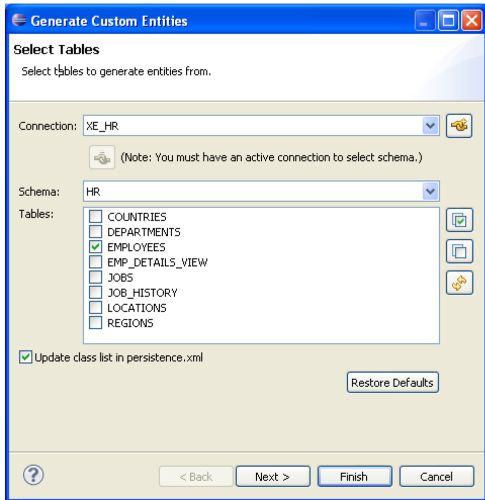
Figure 8–11 Selecting the Database Tables
