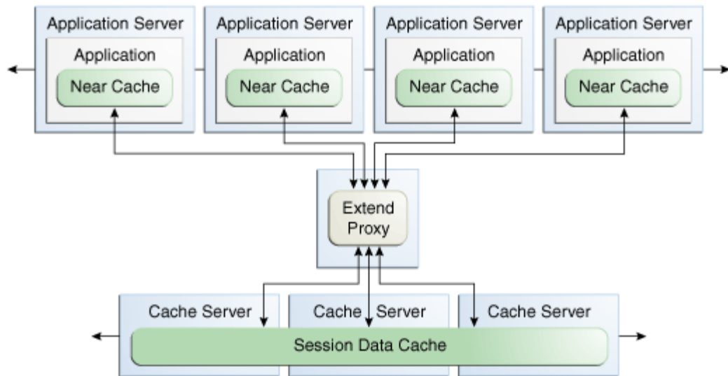
Figure 5–11 Out-of-Process with Coherence*Extend Deployment Topology
