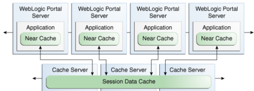
Figure 10-3 Out-of-Process Deployment Topology for WebLogic Portal
