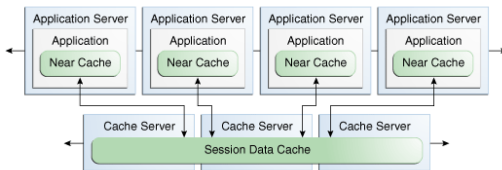
Figure 5–10 Out-of-Process Deployment Topology
