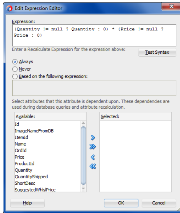
Figure 3–11 Dialog to Edit Expression for Default Attribute Values
