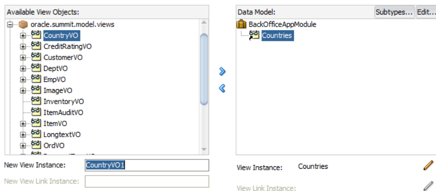
Figure 13–4 Master View Instance Created
