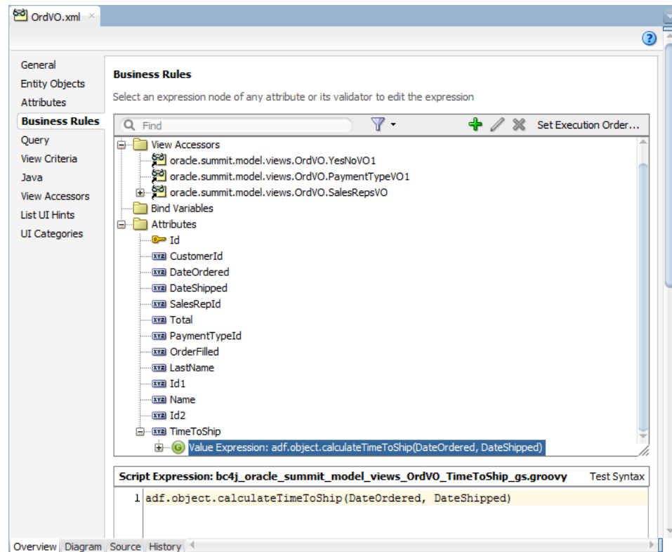
Figure 3–12 Overview Editor's Business Rules Page Shows All Expressions Used by a Business Component
