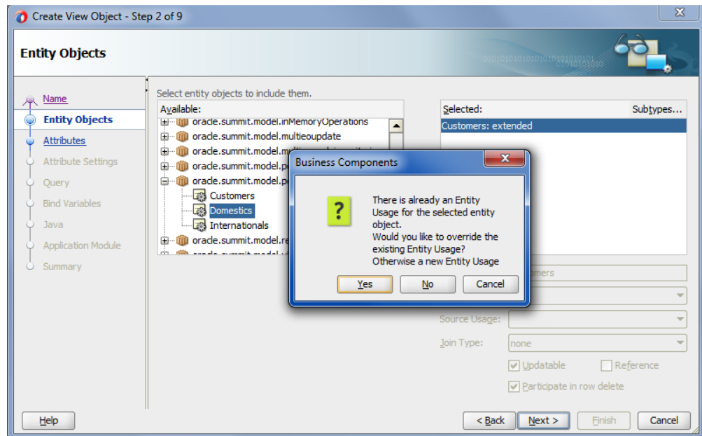
Figure 7-3 View Object with a Polymorphic Entity Subtype Selection
