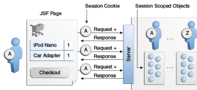
Figure 49–2 Tracking State Using a Session Cookies and Server-Side Session
