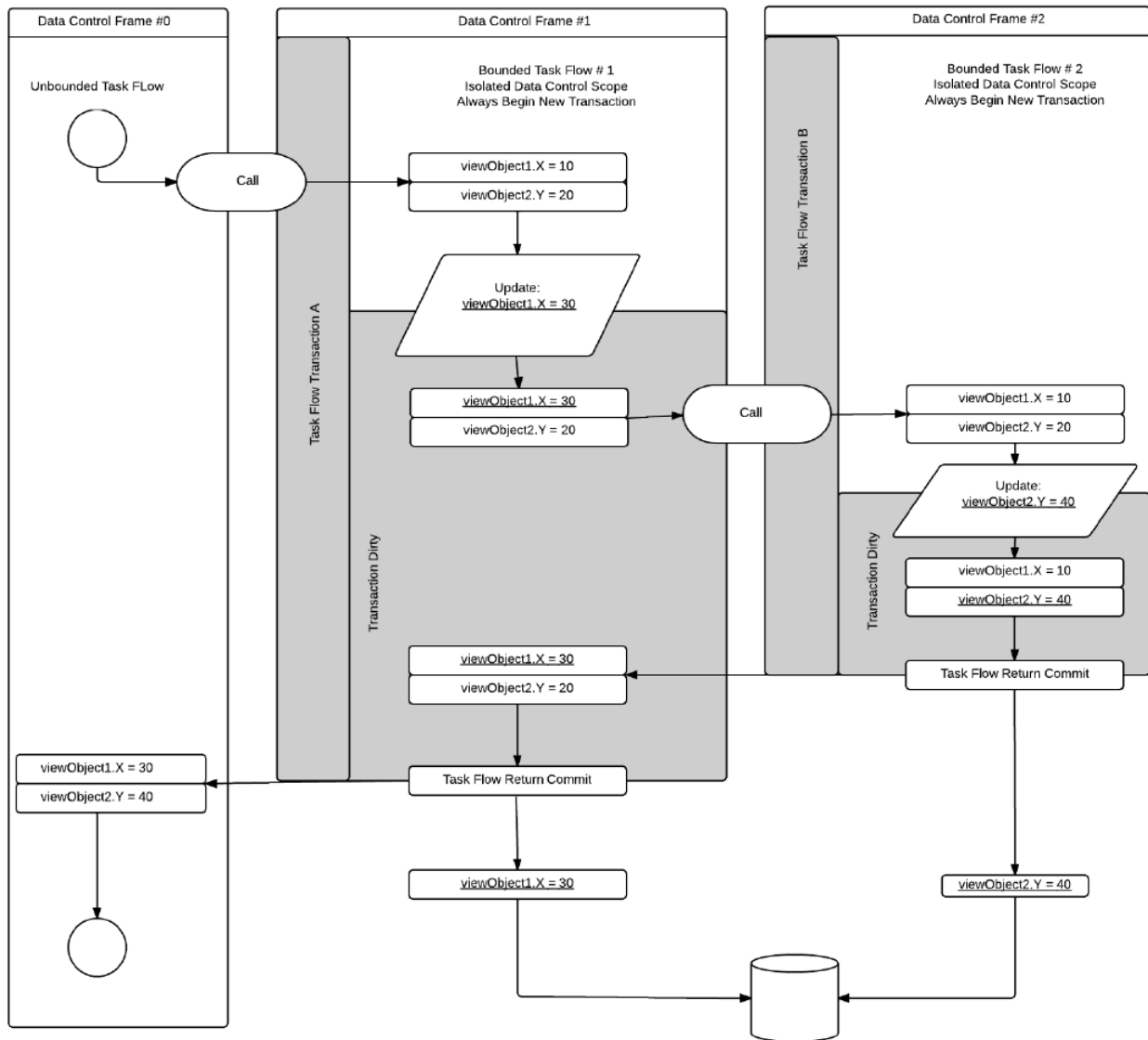
Figure 24–5 Completely Separate Transactions
