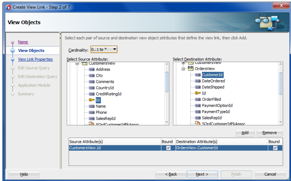
Figure 15-14 One to Many Relationship Defined in Create View Link Wizard
