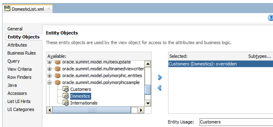
Figure 7-6 View Object Editor Shows Entity Subtype is Overridden
