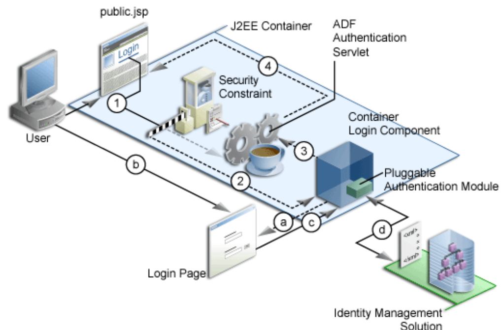
Figure 41–28 ADF Security Explicit Authentication
