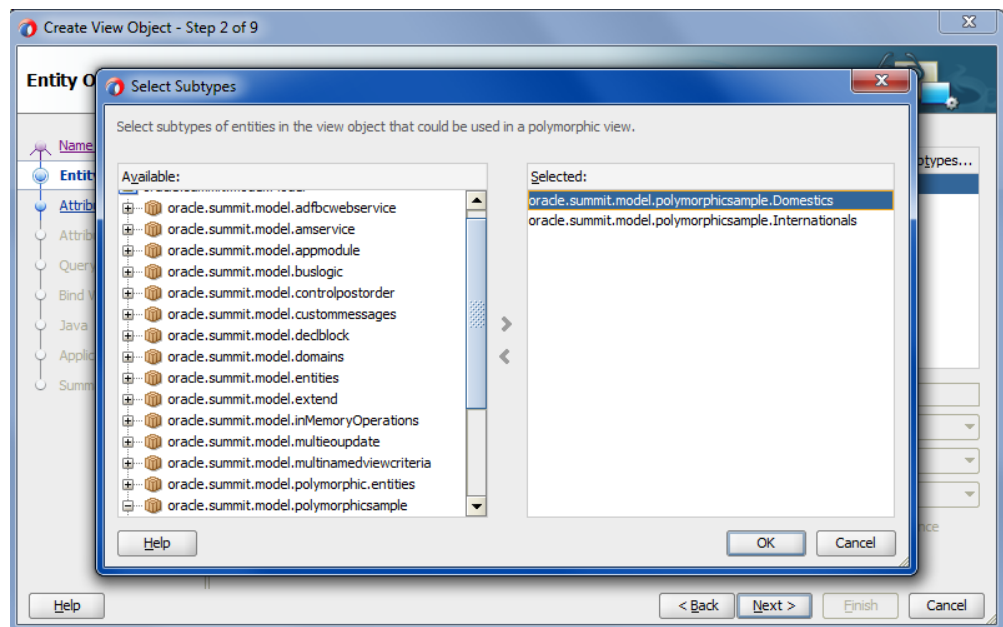
Figure 7-4 View Object with a Entity Subtype Selection
