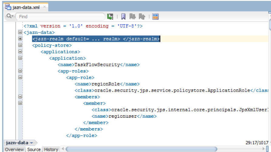
Figure 41–31 Selecting the <jazn-realm> Element in the XML Editor
