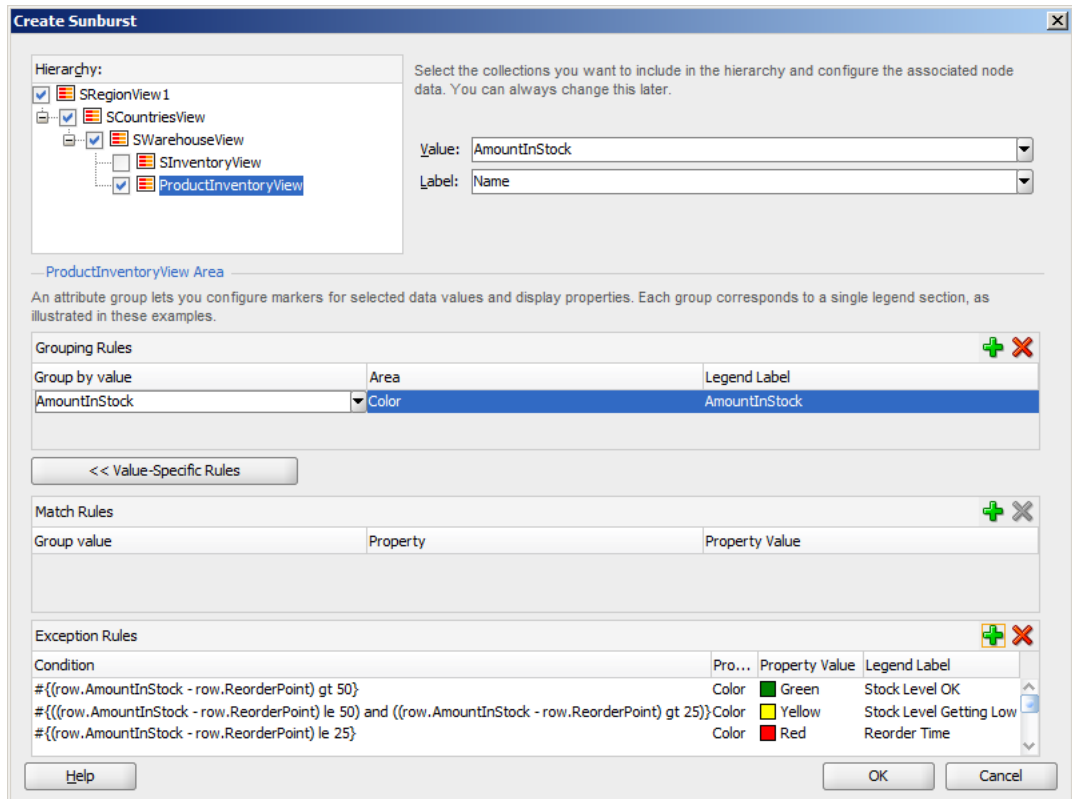
Figure 39–31 Sunburst Showing Exception Rules Creation Dialog
