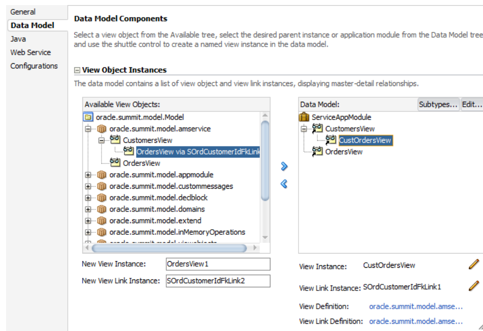
Figure 15–15 Data Model Contains Service View Instances
