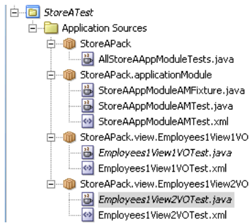
Figure 42–57 Business Components Test Suite in the Applications Window
