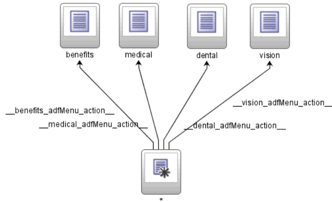
Figure 24-23 Updated Unbounded Task Flow
