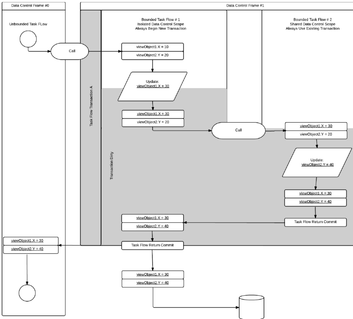
Figure 24–6 Guaranteed Jointed Transactions
