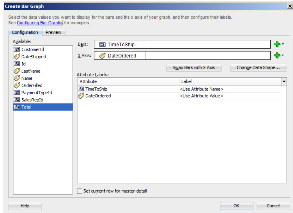
Figure 35–4 Create Bar Graph Dialog for Time to Ship Graph
