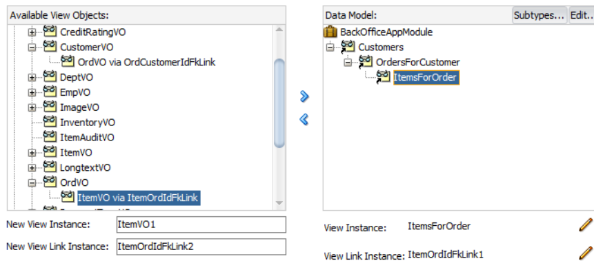
Figure 13–7 Master-Detail-Detail Hierarchy Created
