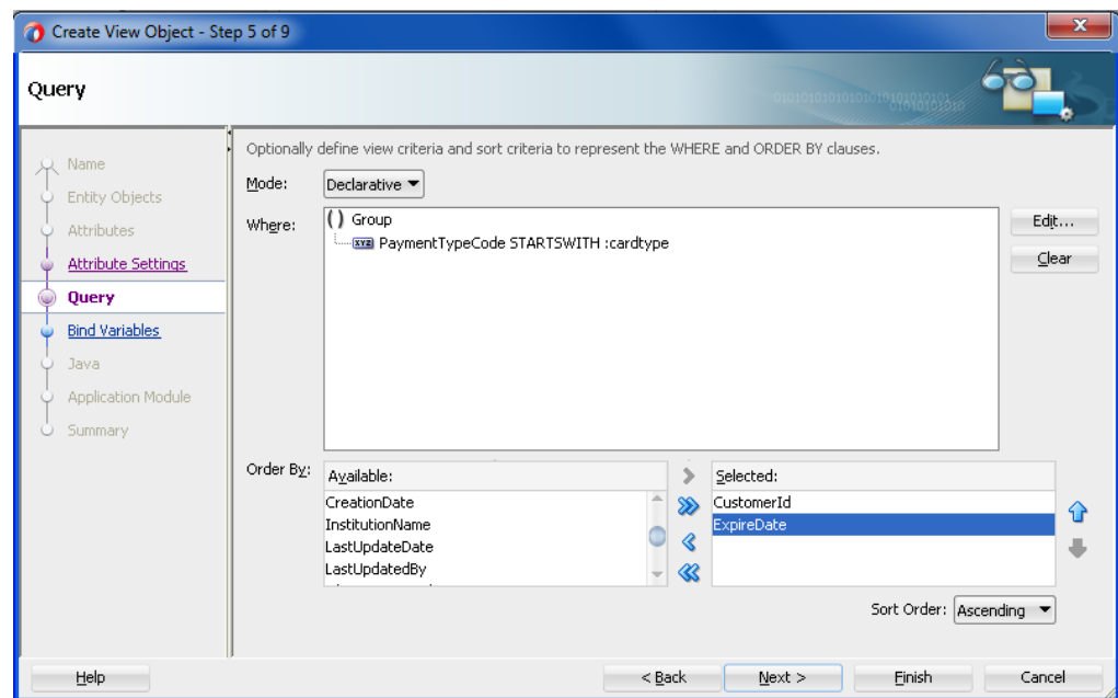
Figure 5–22 Creating View Object Wizard, Query Page with Declarative Mode Selected
