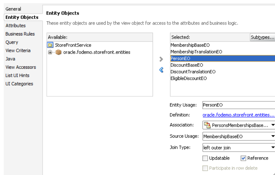
Figure 5–19 Setting an Outer Join to Return NULL Rows from Joined Entities
