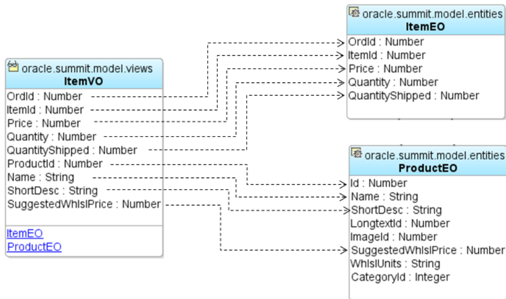
Figure 5-20 View Object Maps Attributes of Multiple Entity Objects
