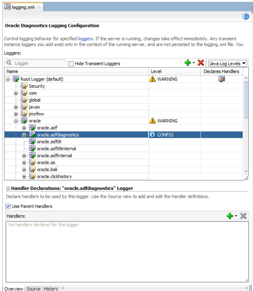
Figure 42–4 Editor for Oracle Diagnostic Logging Configuration
