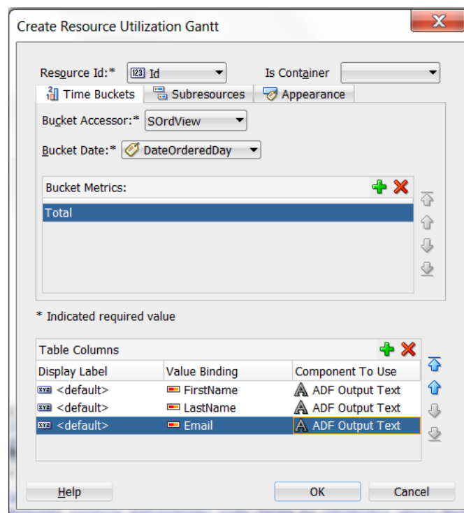
Figure 38–7 Create Resource Utilization Gantt Chart Dialog
