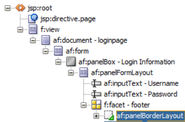
Figure 41-24 Login Page Structure with Panel Border Layout
