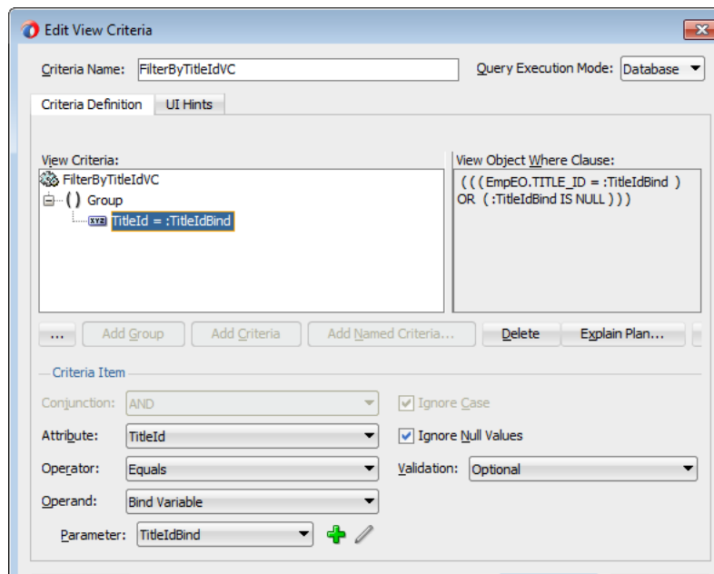
Figure 33–14 View Criteria with Named Bind Variable
