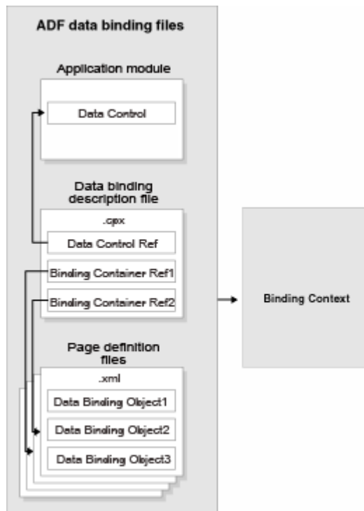
Figure 17–13 ADF File Binding Runtime Usage
