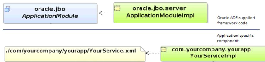
Figure 3–10 Component with Custom Java Class
