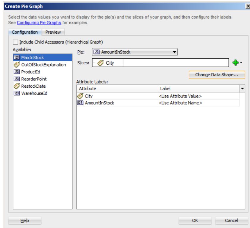
Figure 35–17 Create Pie Graph for InventoryForOrderItem
