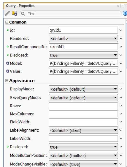
Figure 33–18 Properties window for a Query Component
