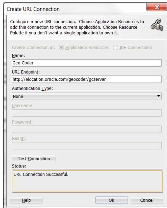
Figure 37–4 Create Geocoder URL Connection
