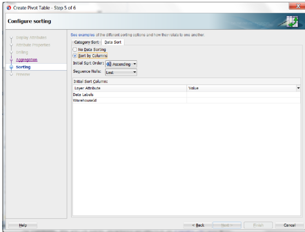
Figure 36–13 Data Sort Page of the Create Pivot Table Wizard
