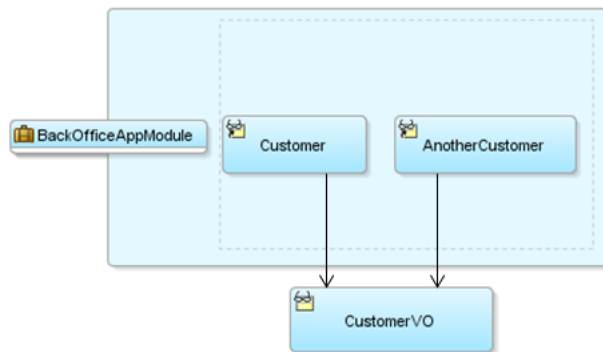
Figure 13–9 Application Module Containing Two Instances of a View Object Component
