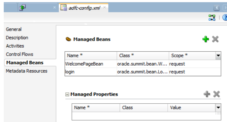
Figure 26-3 Managed Beans in the adfc-config.xml File
