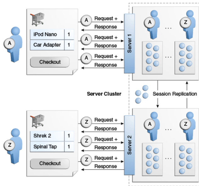
Figure 49-3 Session Replication in a Server Cluster
