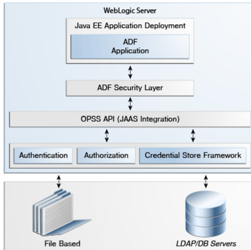
Figure 9–2 ADF Security Architecture
