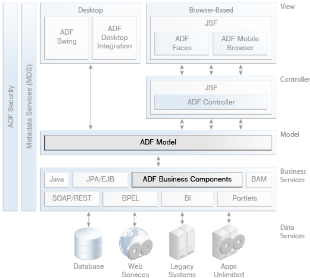
Figure 4–1 ADF Architecture with Business Components
