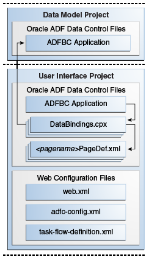
Figure 3–5 Files Used in Data Binding
