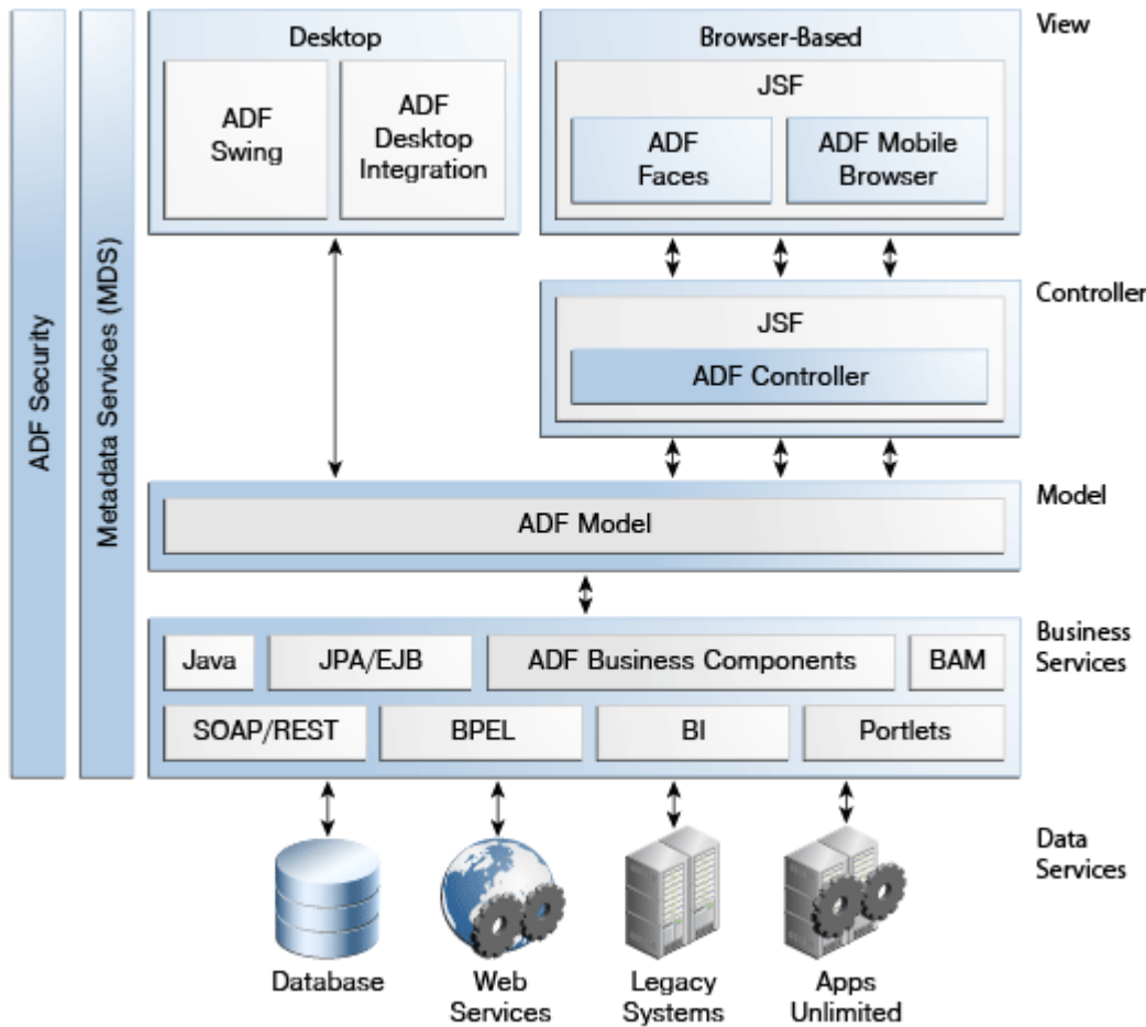
Figure 1-1 ADF Architecture
