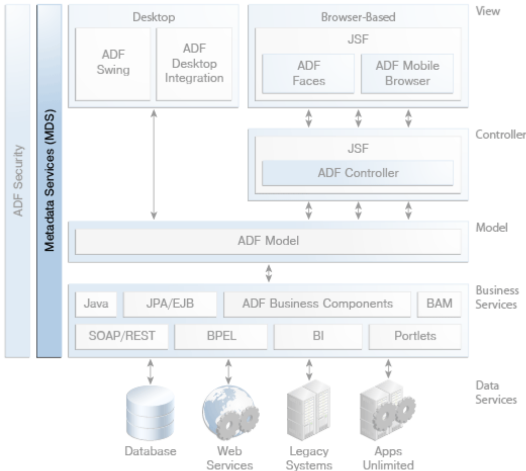
Figure 10–1 ADF Architecture with Metadata Services
