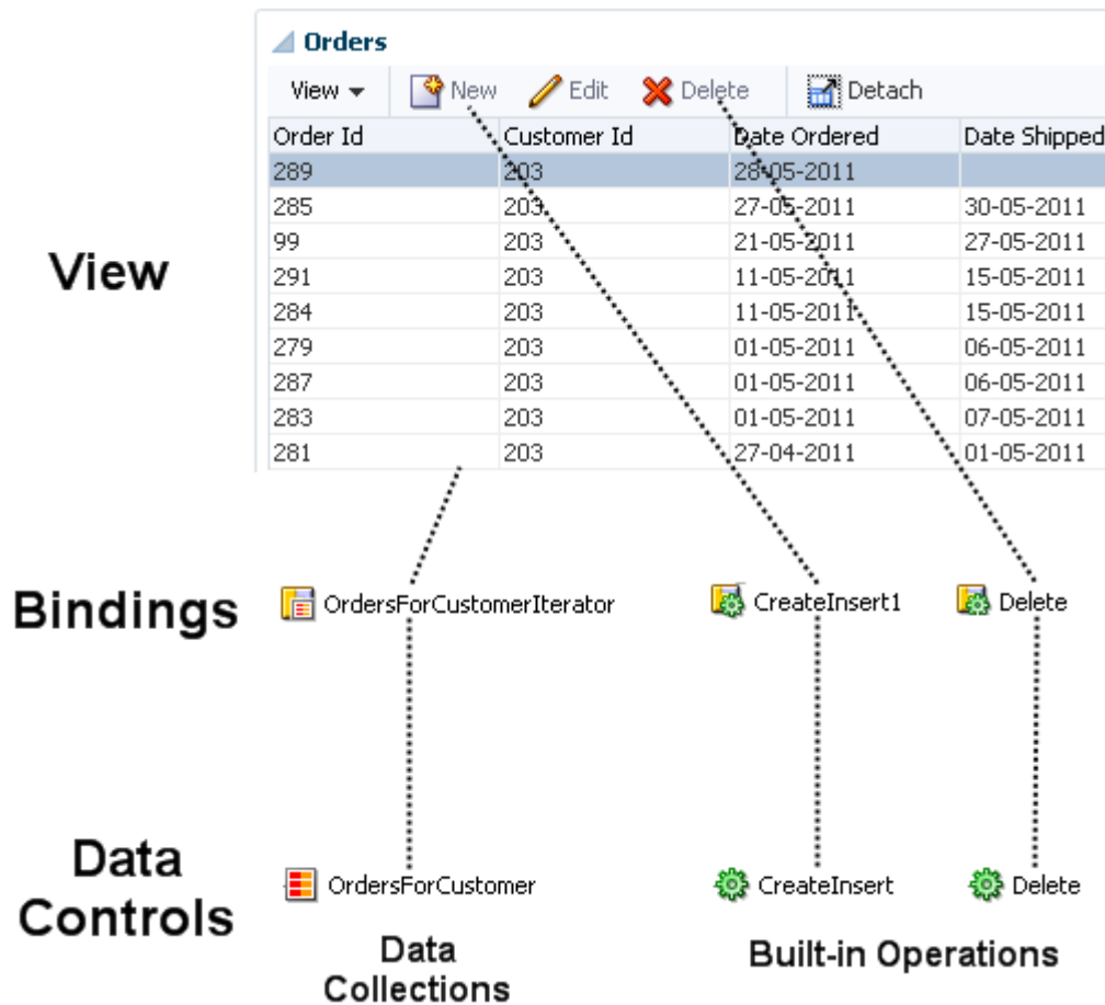
Figure 3–6 Binding Data Sources to UI Components Using ADF Model
