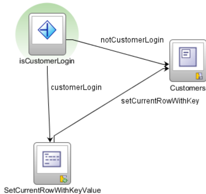
Figure 2–2 ADF Task Flow
