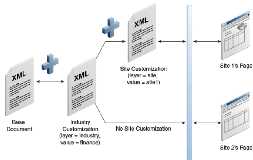
Figure 10–2 Base Application and Customization Layers
