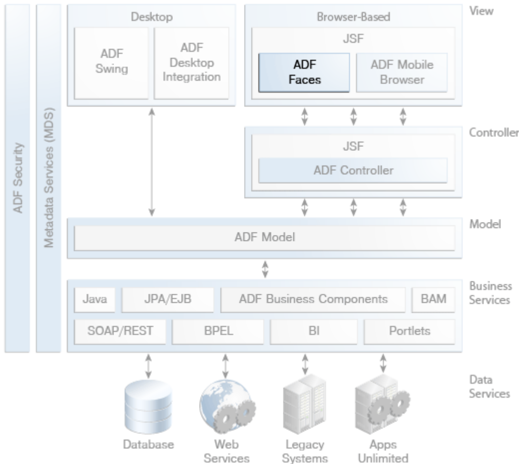
Figure 6–1 Overall Application Architecture with ADF Faces
