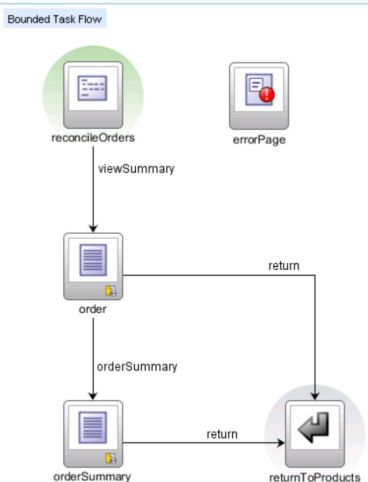
Figure 5-2 ADF Bounded Task Flow
