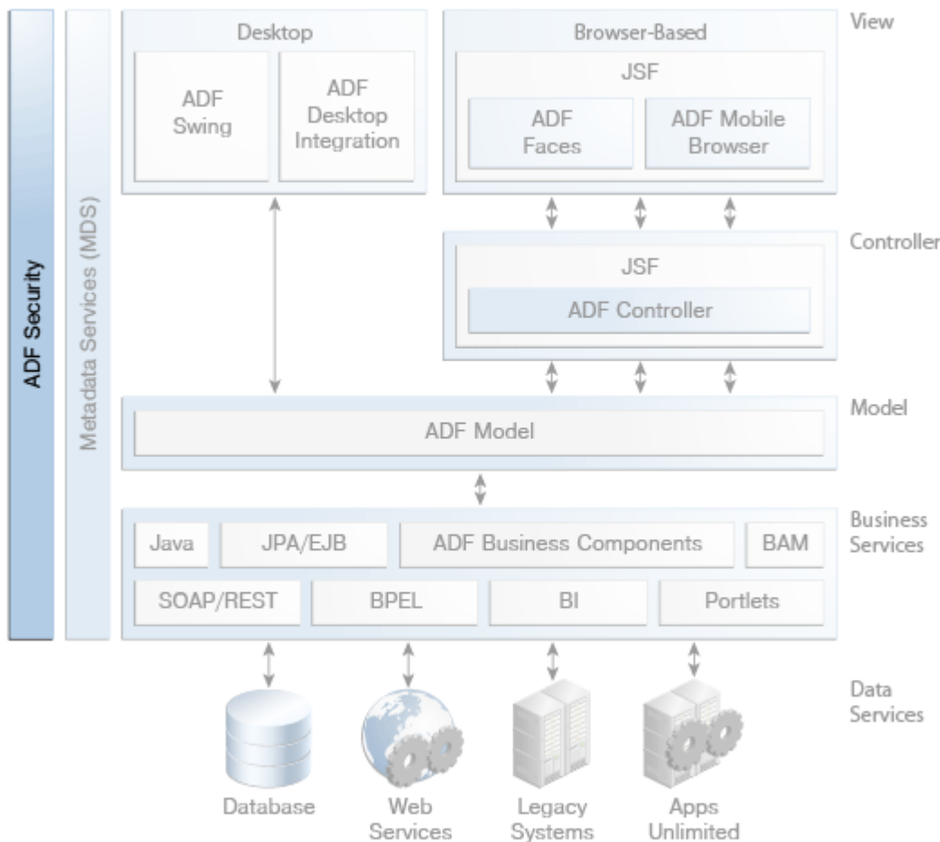
Figure 9–1 ADF Architecture with ADF Security
