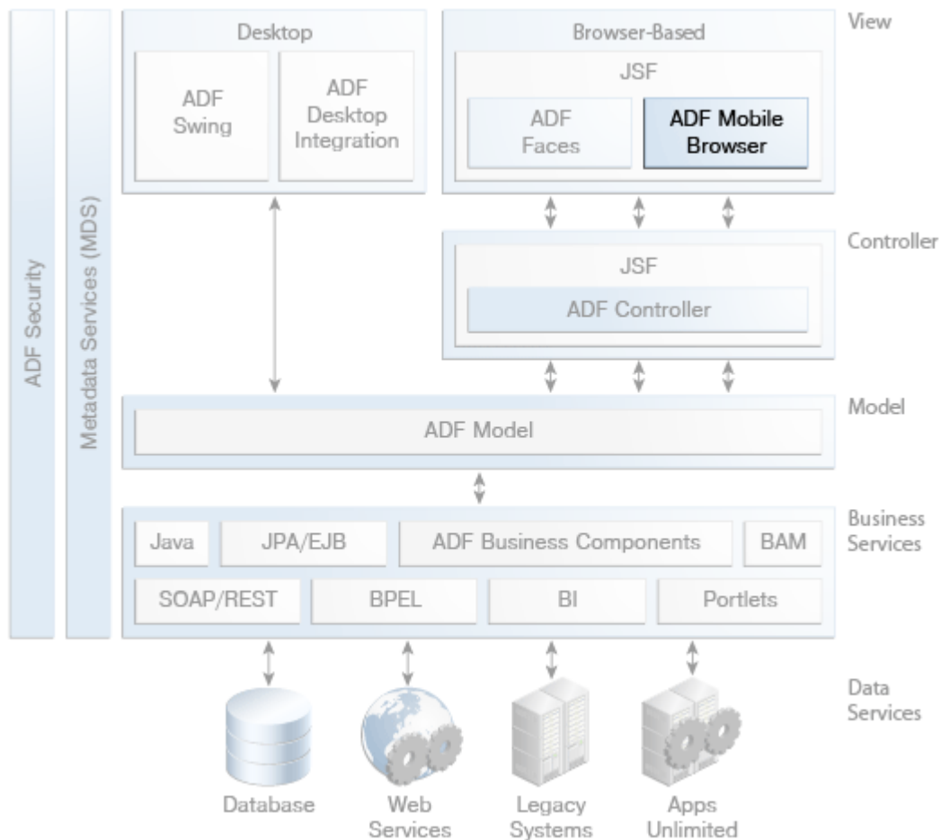
Figure 7-1 ADF Architecture with ADF Mobile Browser
