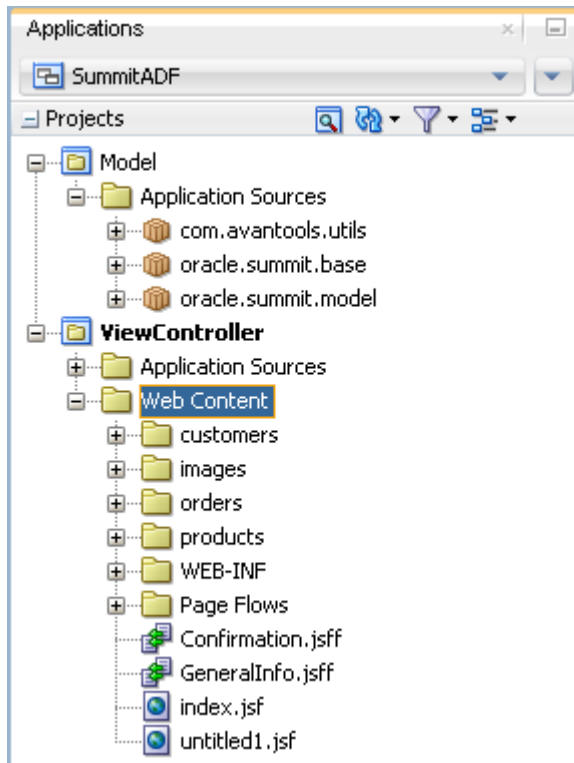
Figure 2–1 Applications Window in JDeveloper
