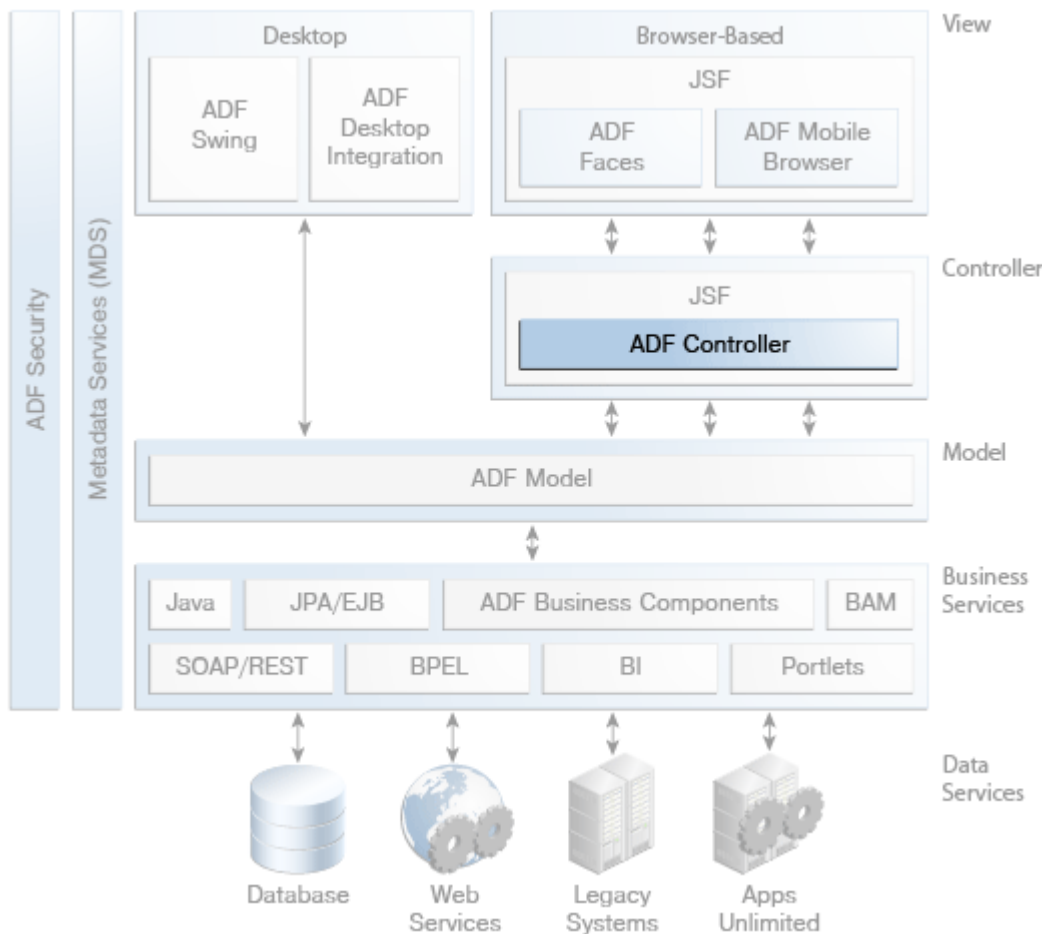
Figure 5–1 Overall Application Architecture with ADF Controller
