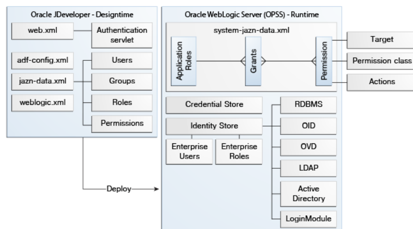
Figure 9–3 ADF Security Configuration and Deployment
