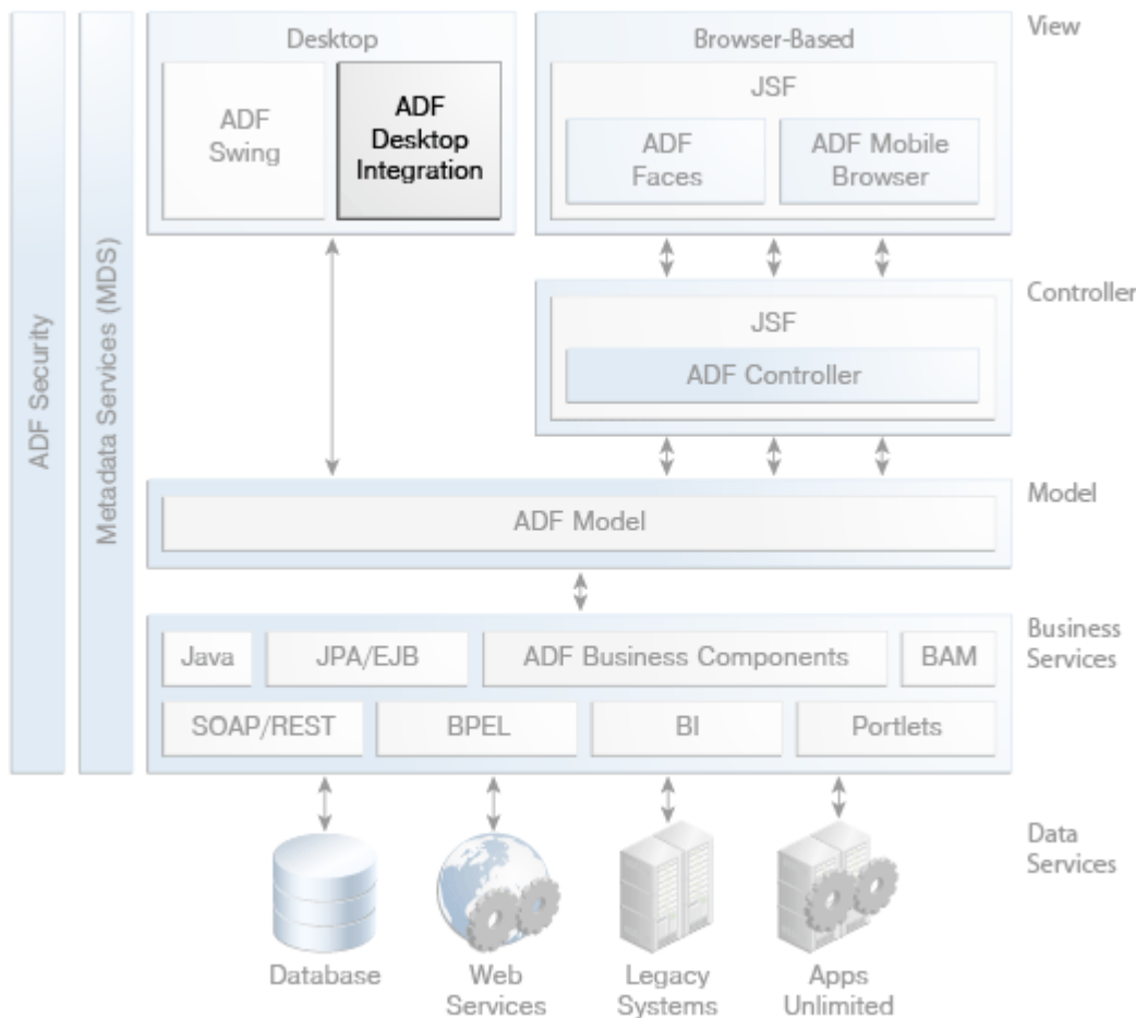
Figure 8–1 ADF Architecture with ADF Desktop Integration
