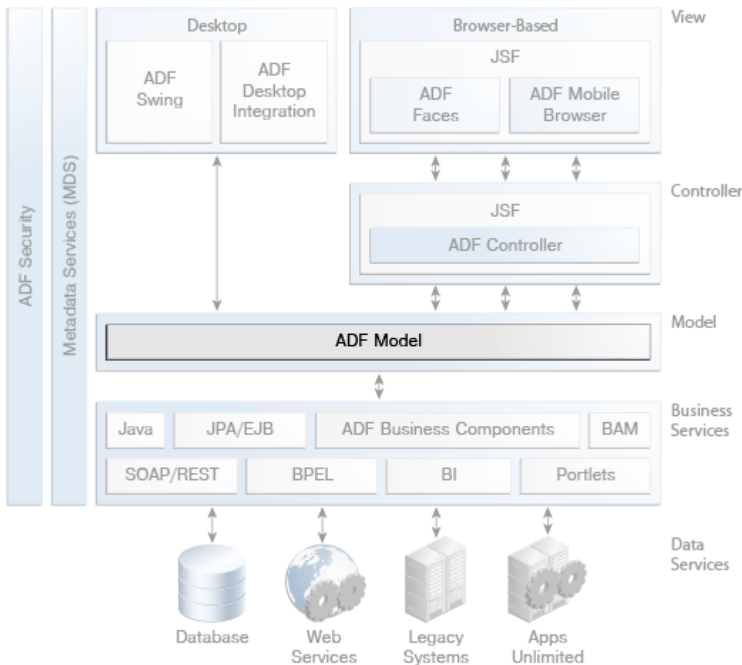
Figure 3–1 Overall Application Architecture with ADF Model
