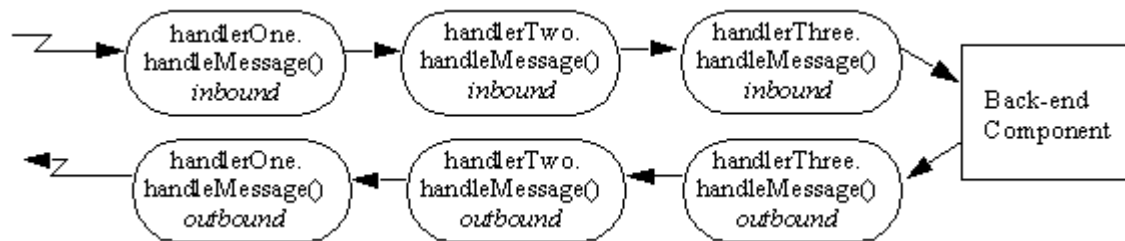
Figure 17–1 Order of Execution of Handler Methods
