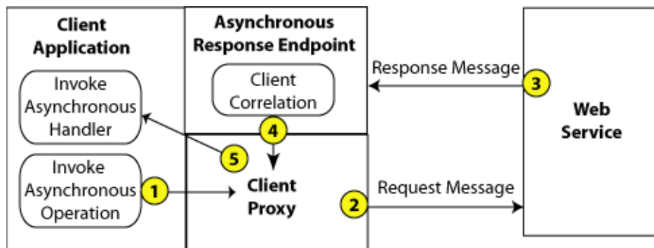
Figure 4–1 Asynchronous Client Transport Feature
