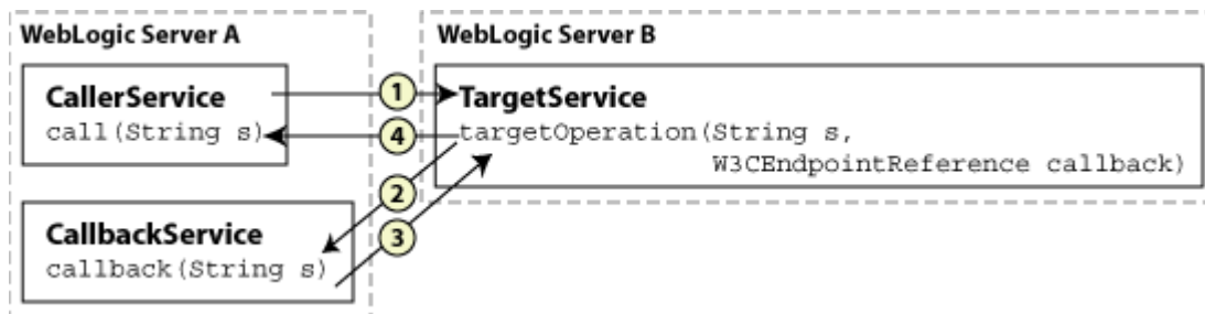
Figure 12–1 Example Callback Implementation
