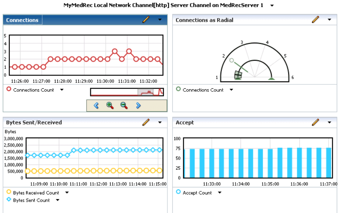
Figure 15–4 View Containing Four Charts
