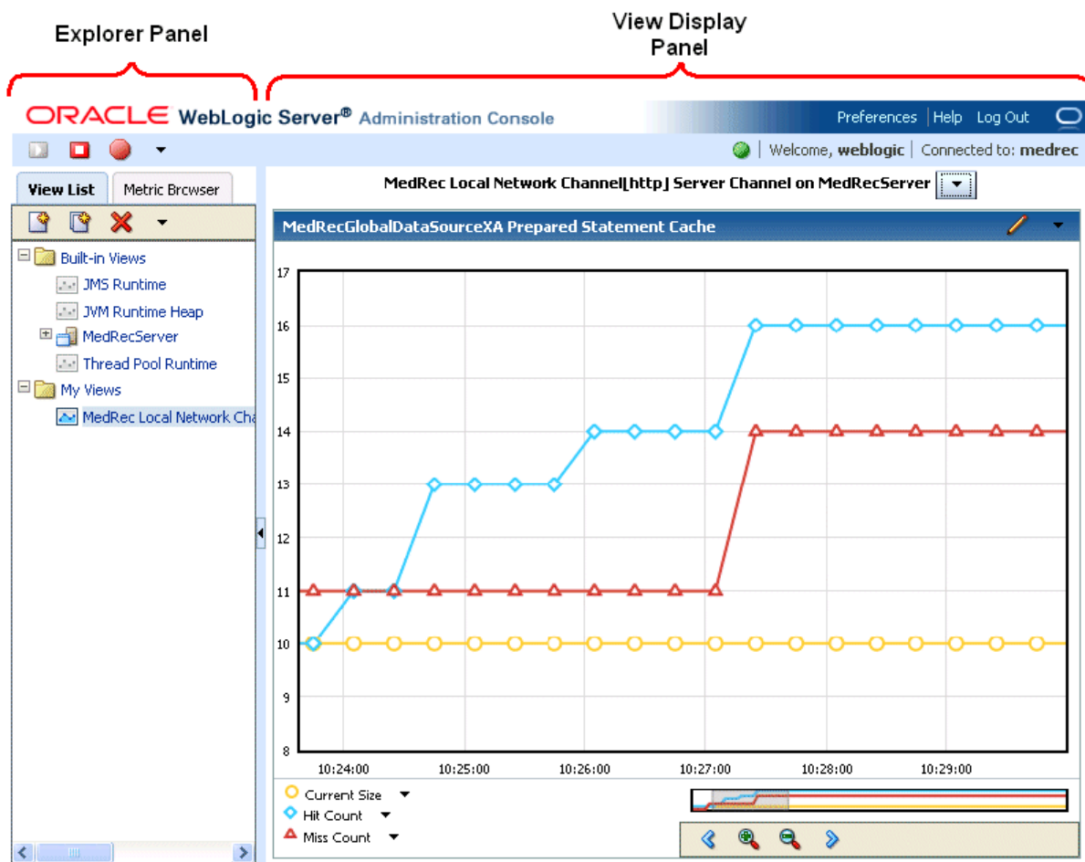
Figure 15–1 Monitoring Dashboard Panels
