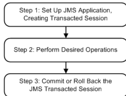
Figure 12–1 Setting Up and Using a JMS Transacted Session
