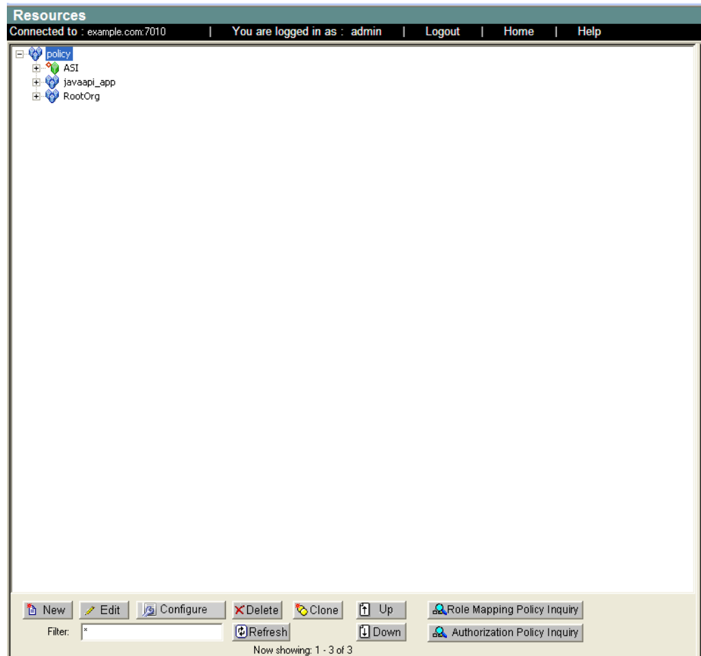
Figure 31-9 Resources Page
