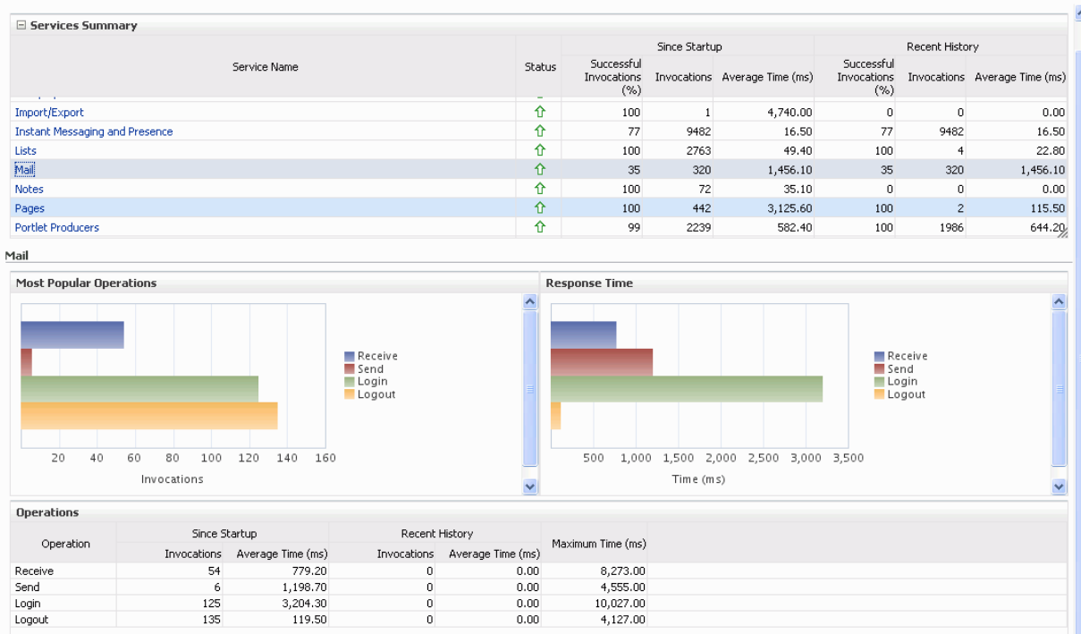
Figure 27–29 Mail Metrics
