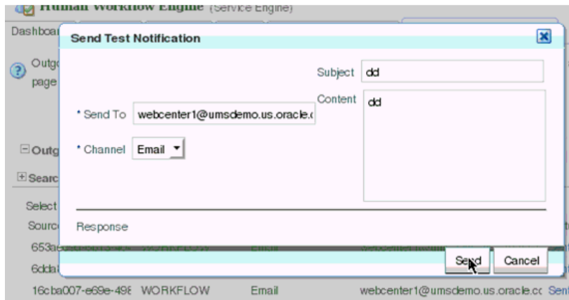
Figure 20–13 Test Notification
