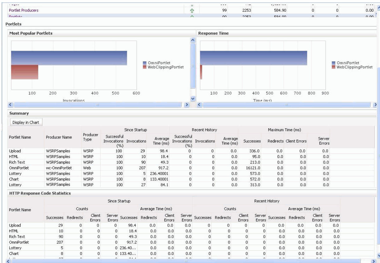
Figure 27-12 Portlet Metrics
