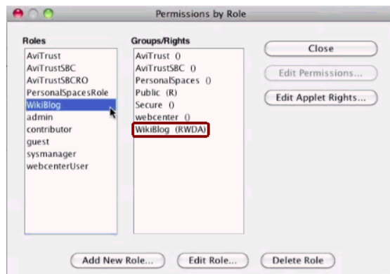
Figure 9–3 RWDA Permissions
