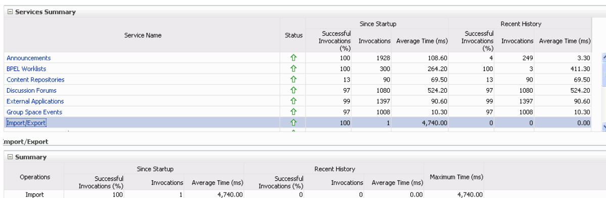
Figure 27–27 Import/Export Metrics
