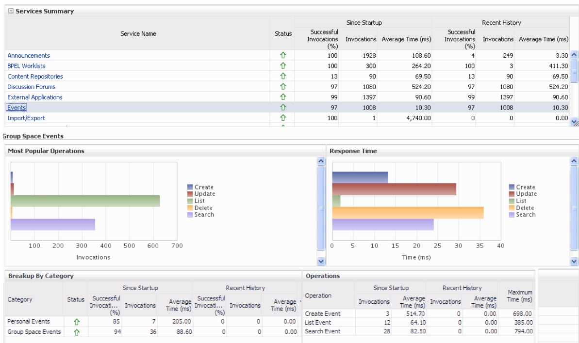
Figure 27–23 Events Metrics
