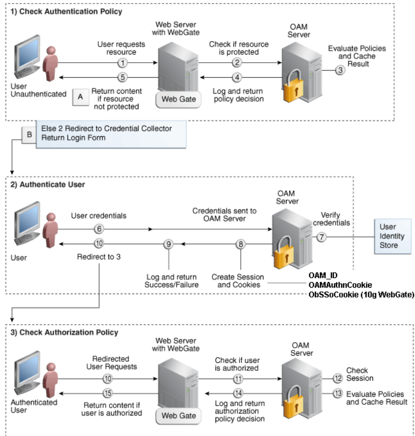
Figure 33–2 OAM Single Sign-on Process Flow
