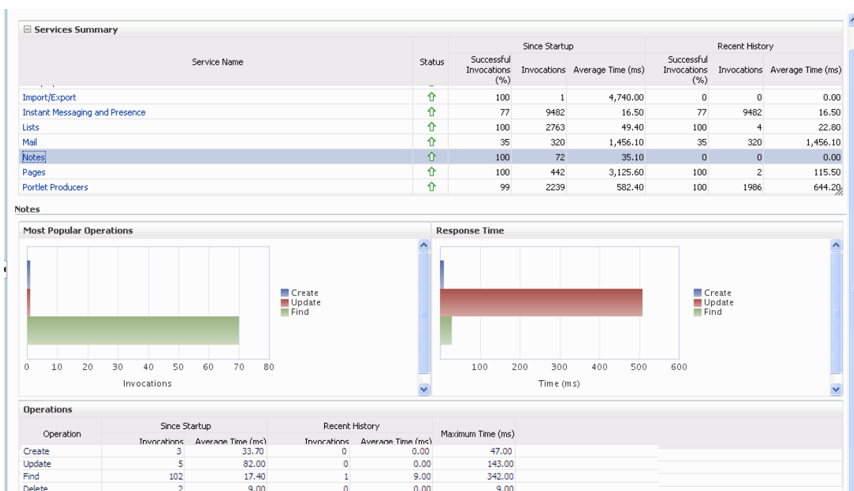
Figure 27–30 Notes Metrics
