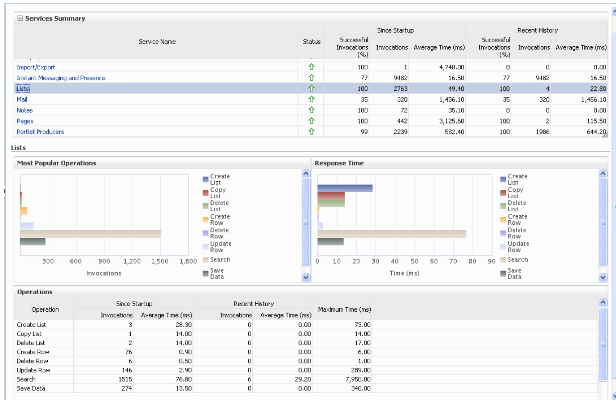
Figure 27–28 List Metrics
