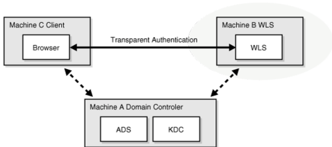
Figure 33–11 SPNEGO-based Authentication
