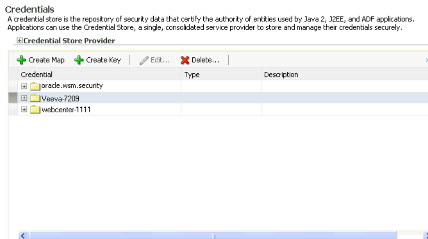
Figure 42-18 Credentials Pane
