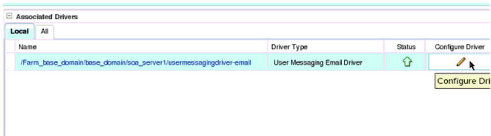
Figure 20–7 Associated Drivers
