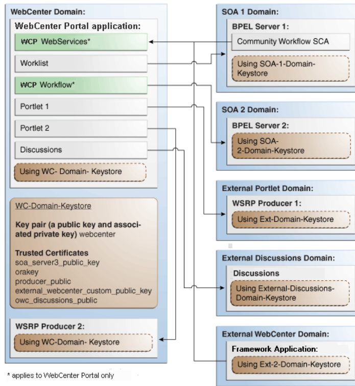
Figure 36–11 WS-Security for a Complex Configuration
