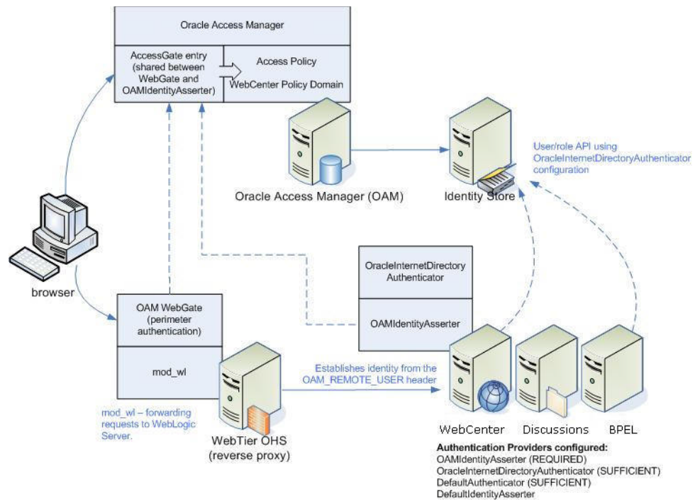
Figure 33–1 OAM Single Sign-On Components and Topology
