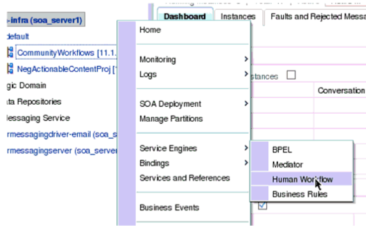
Figure 20–11 Human Workflow
