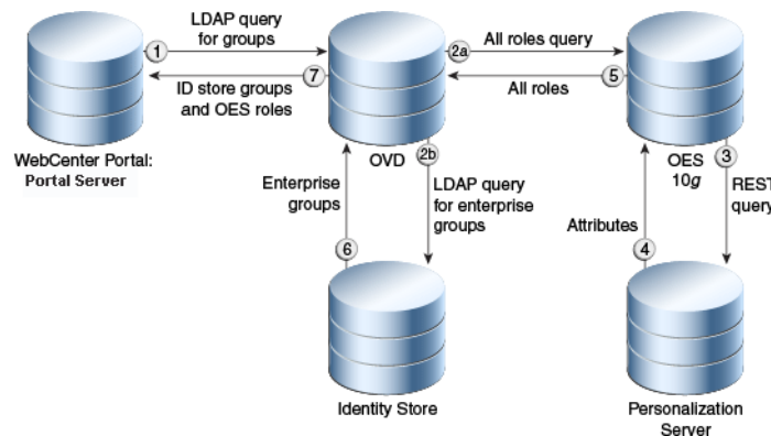
Figure 31-8 Group Query
