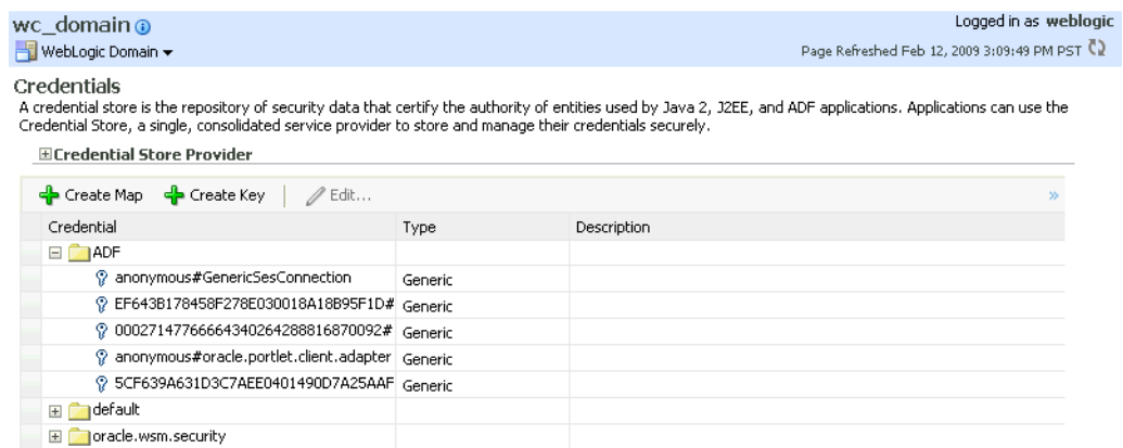
Figure 37-6 Credentials Pane
