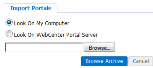
Figure 40–8 Importing Portals
