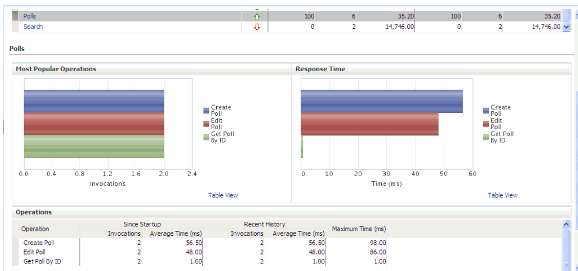
Figure 27–33 Poll Metrics
