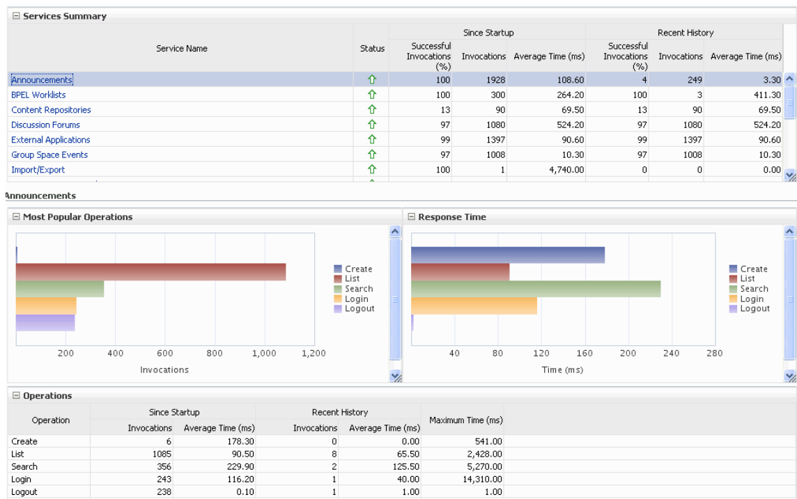
Figure 27–18 Announcements Metrics
