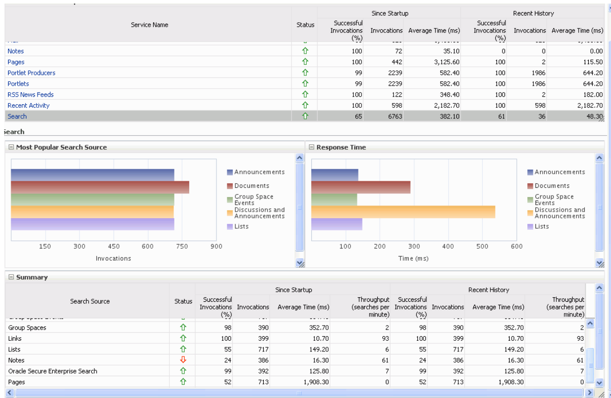
Figure 27–36 Search Metrics
