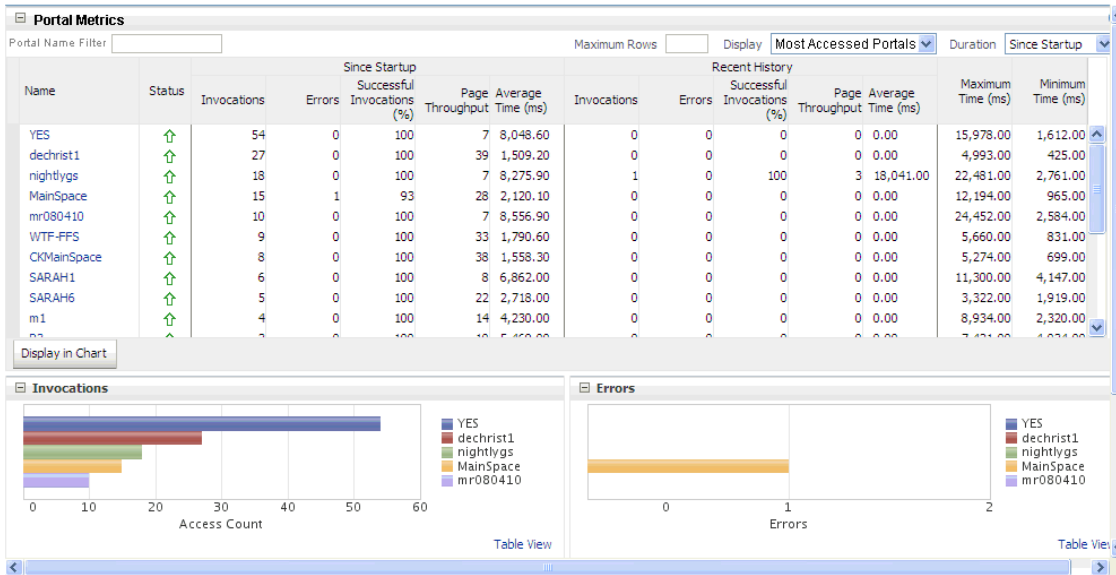
Figure 27–17 Portal Metrics
