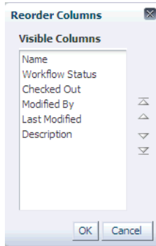
Figure 43–41 Columns - Reorder
