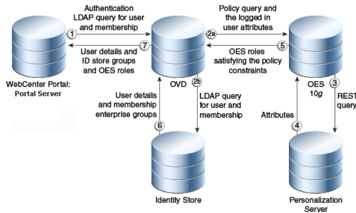
Figure 31-7 Login Process
