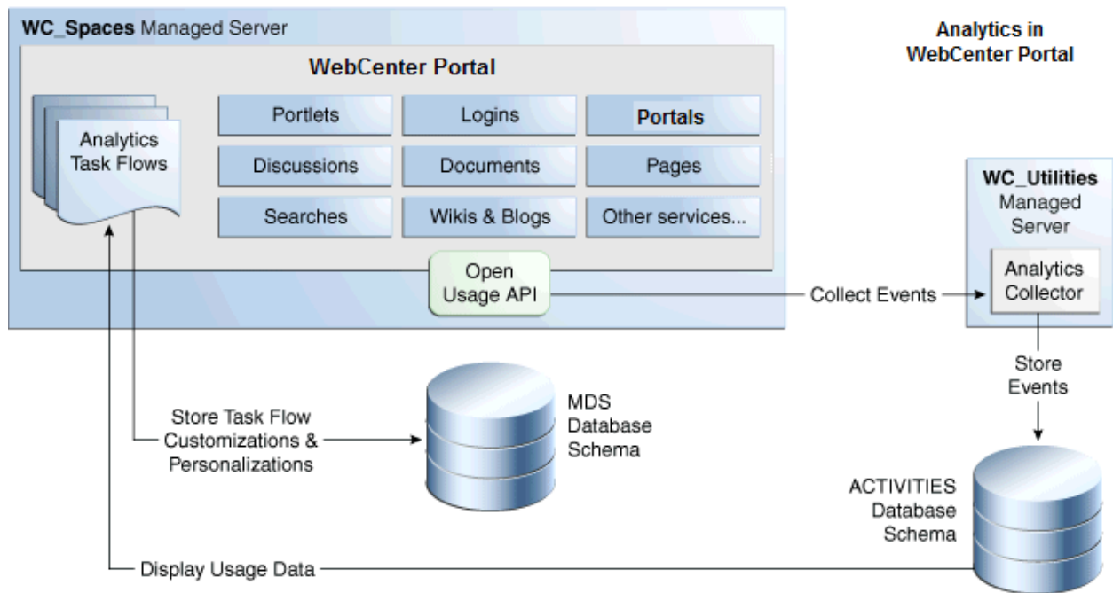
Figure 11–1 Analytics Components
