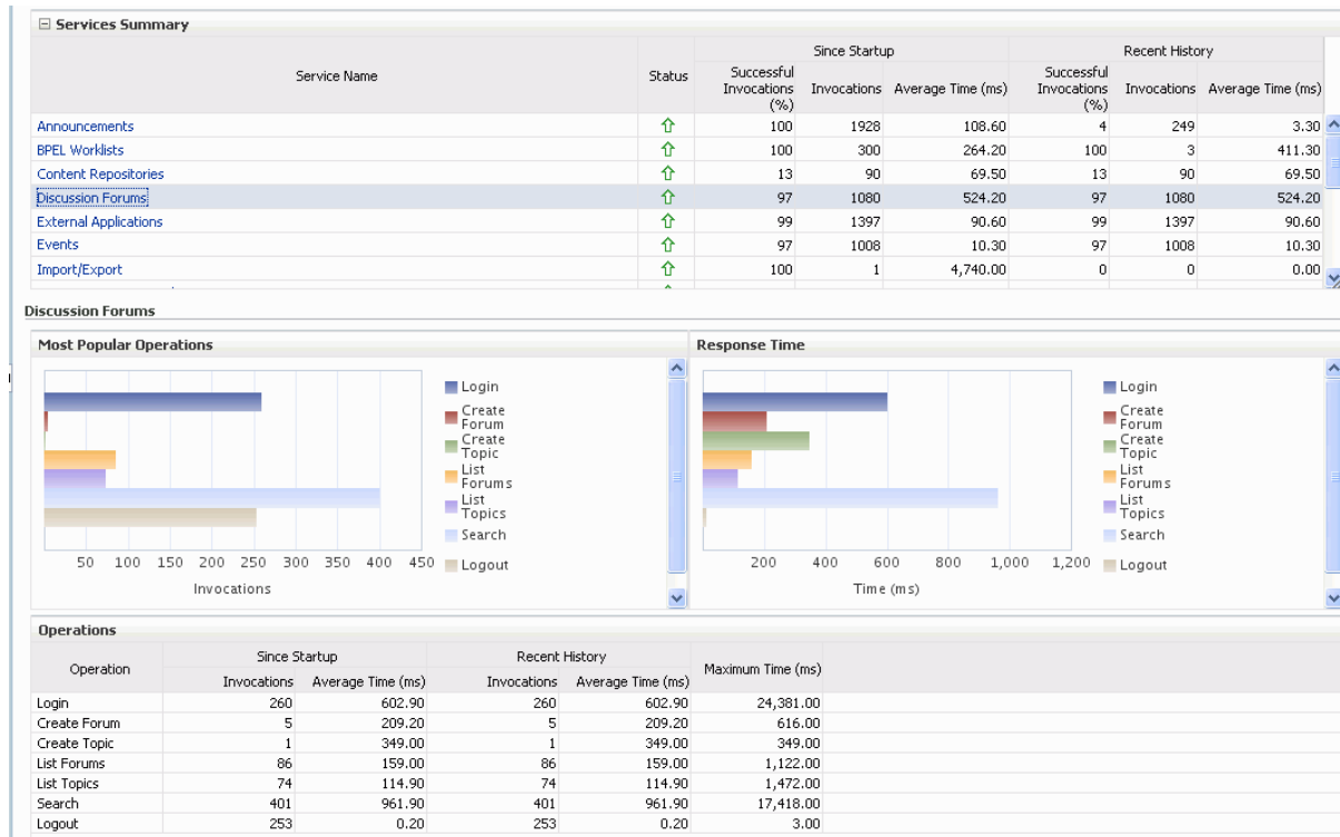
Figure 27–22 Discussion Metrics
