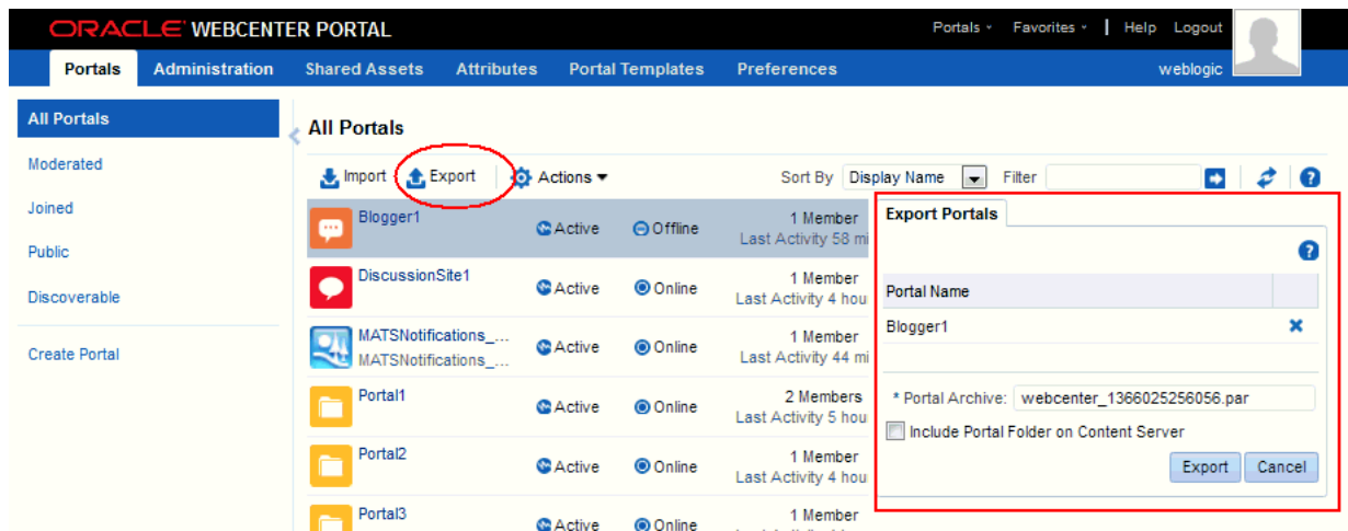
Figure 40–5 Exporting Portals
