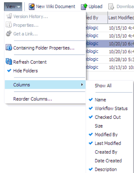
Figure 43–40 Columns - Show
