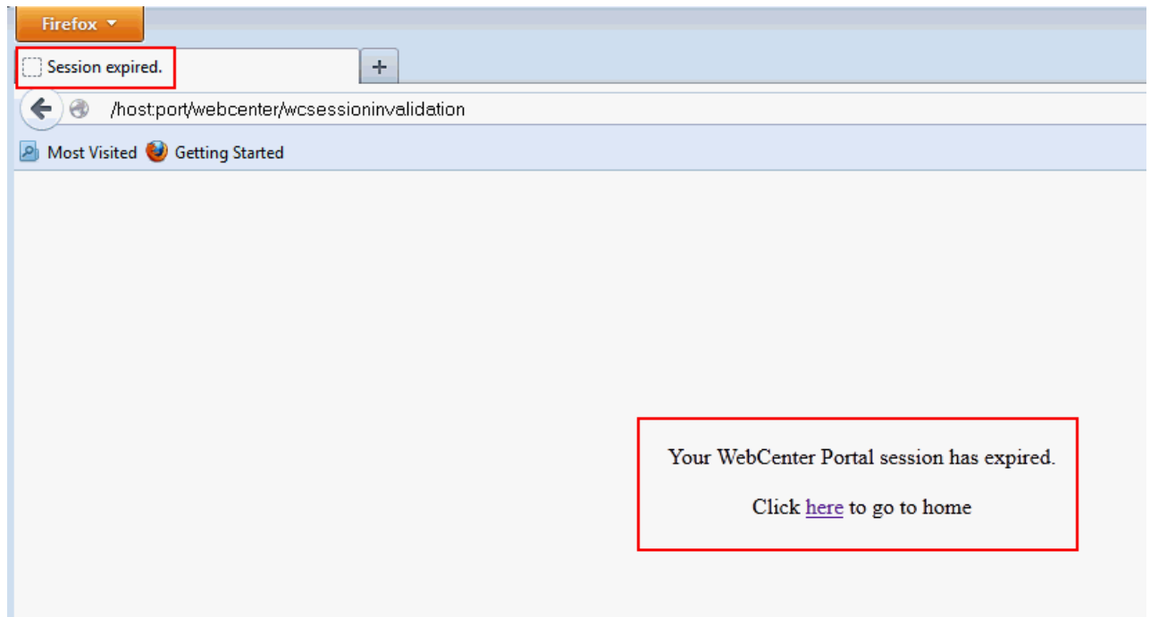
Figure 48-22 Timeout Page
