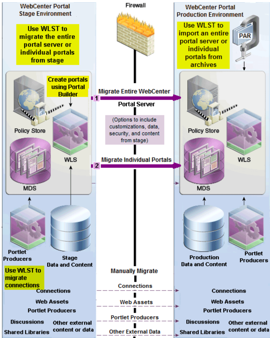
Figure 39–1 Flow from WebCenter Portal Staging to Production Environments
