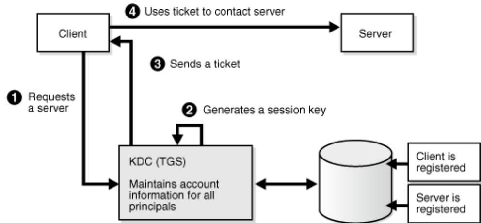
Figure 33–10 Connecting to a Server Through a Key Distribution Center
