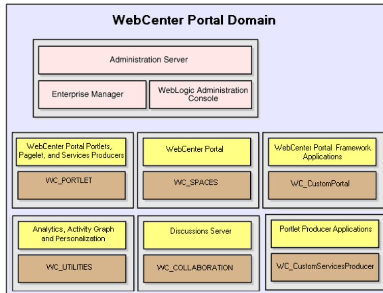
Figure 1–3 Oracle WebCenter Portal Topology Out-of-the-Box
