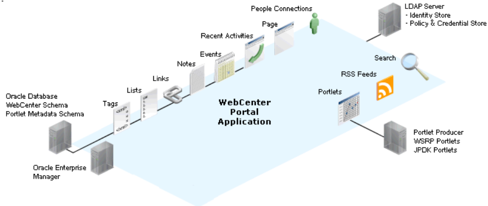
Figure 30–1 Basic WebCenter Portal Application Architecture
