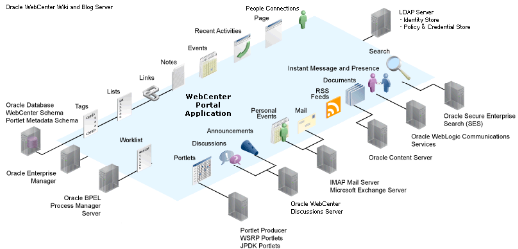
Figure 30–2 WebCenter Portal Application Architecture with Back-end Server Connections
