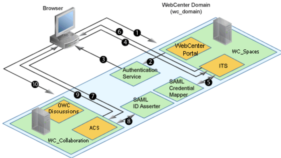
Figure 33–9 SAML Single Sign-on Components and Topology (POST Profile Configured)
