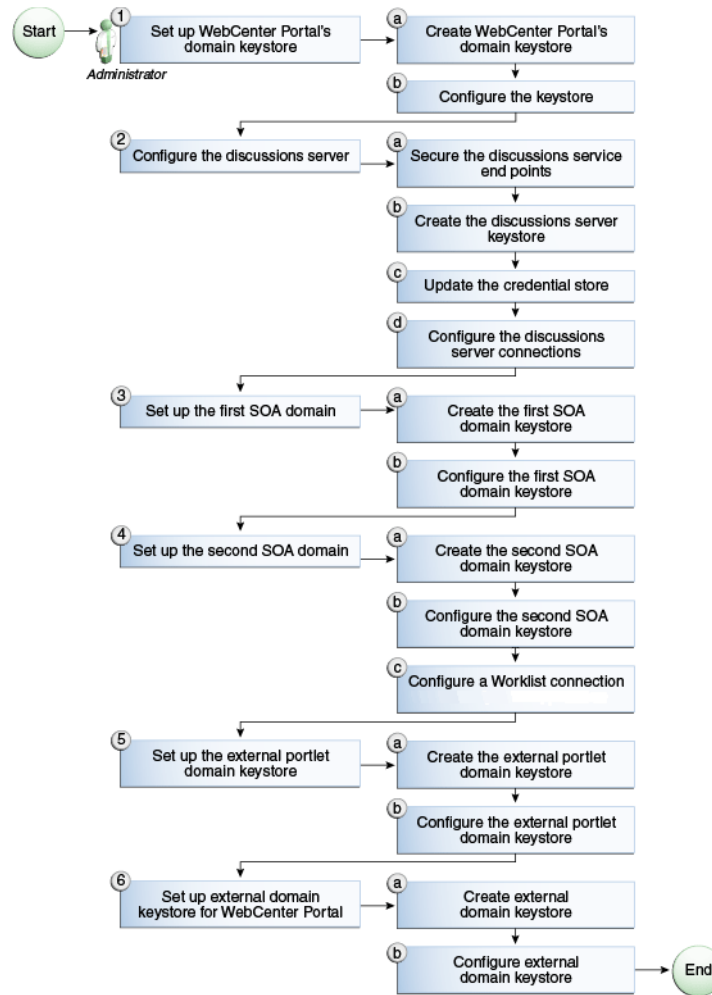
Figure 36–12 Configuring WS-Security for a Complex Topology
