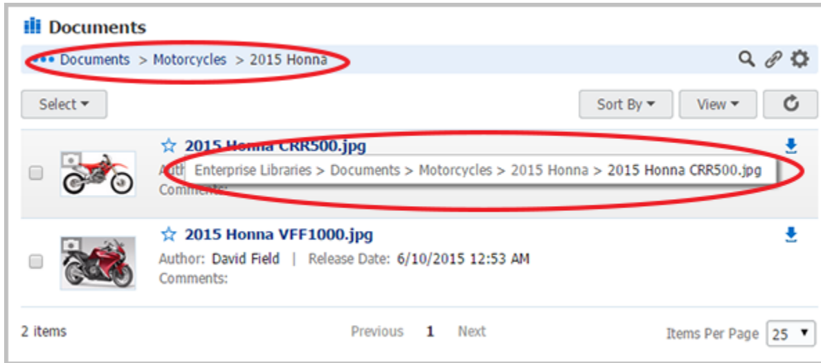
Figure 11-1 Document Context
