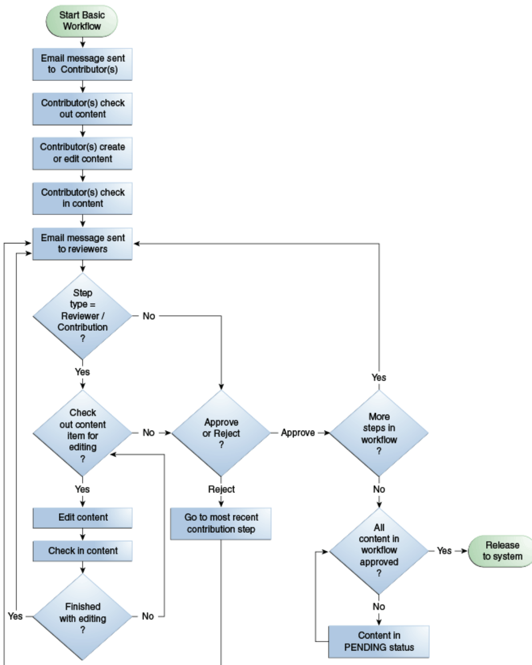
Figure 6–2 Basic Workflow Process
