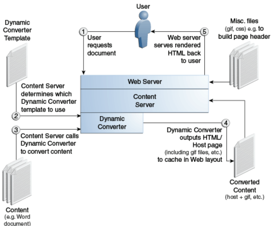
Figure 27–1 Basic Dynamic Converter Process
