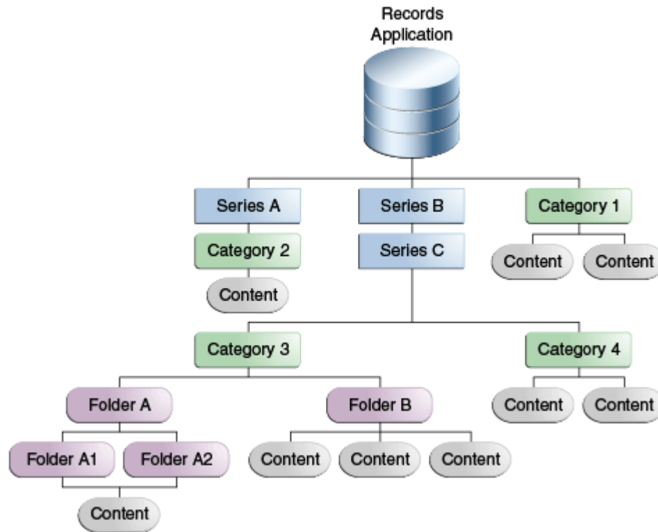
Figure 12-3 Sample Retention Schedule Hierarchy
