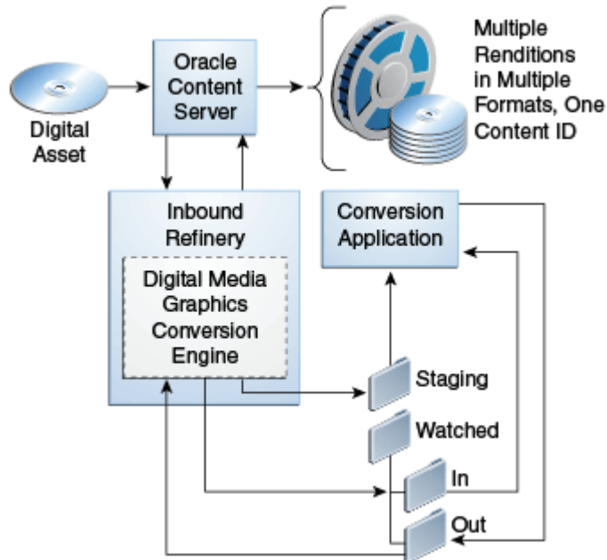
Figure 24–1 Rendering a Video Asset
