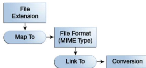
Figure 21–1 Mapping File Formats to a Conversion
