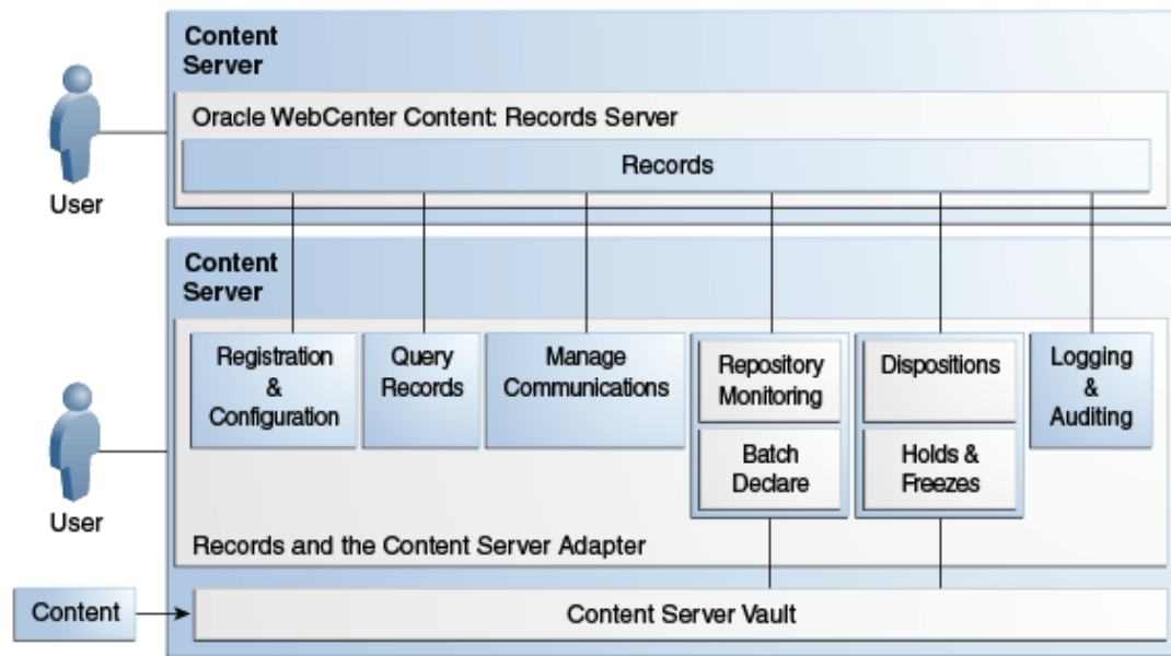
Figure 15–1 Content Server Adapter Retention Functions Overview
