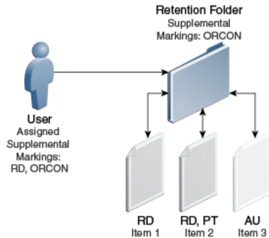
Figure 13–5 User Must Match At Least One Supplemental Marking
