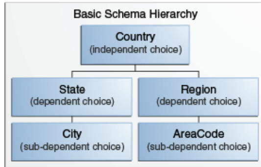
Figure 7-1 Basic Schema Hierarchy Example
