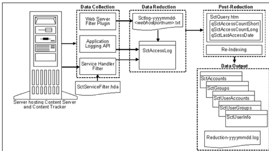
Figure 9–1 Data Reduction Process with Activity Metrics
