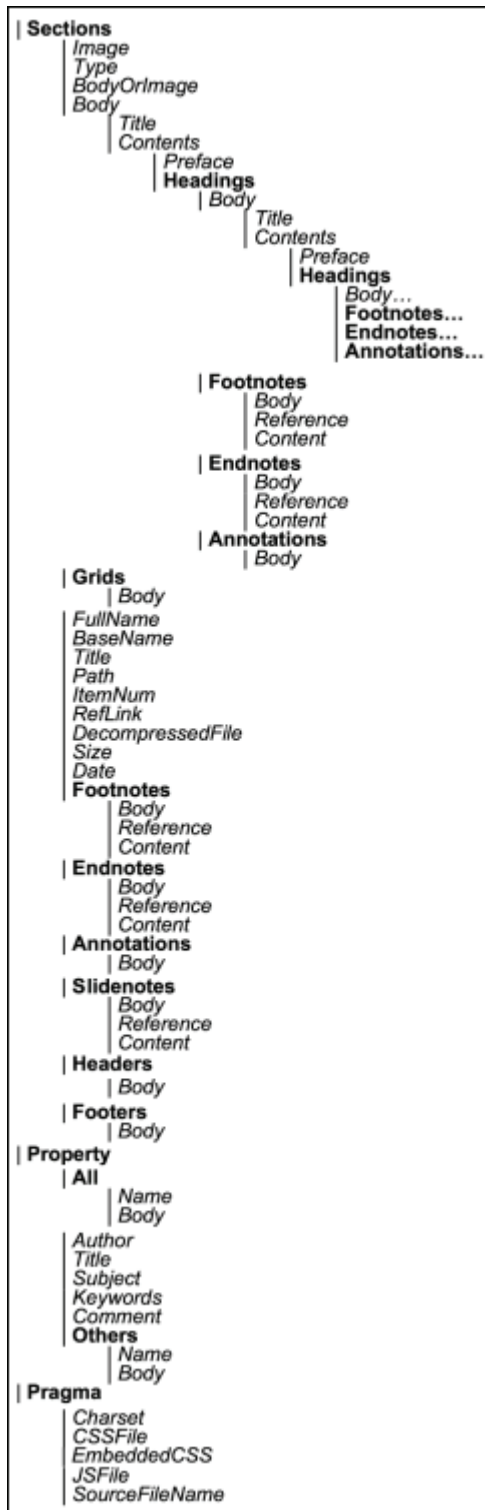
Figure 33-1 Example of an Element Tree
