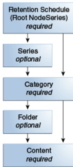
Figure 12-1 Basic Retention Schedule Hierarchy
