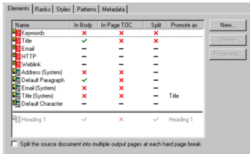
Figure 31–3 Elements in Template Editor
