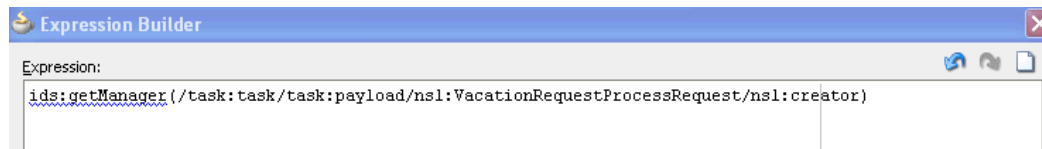
Figure 31–8 XPath Expression
