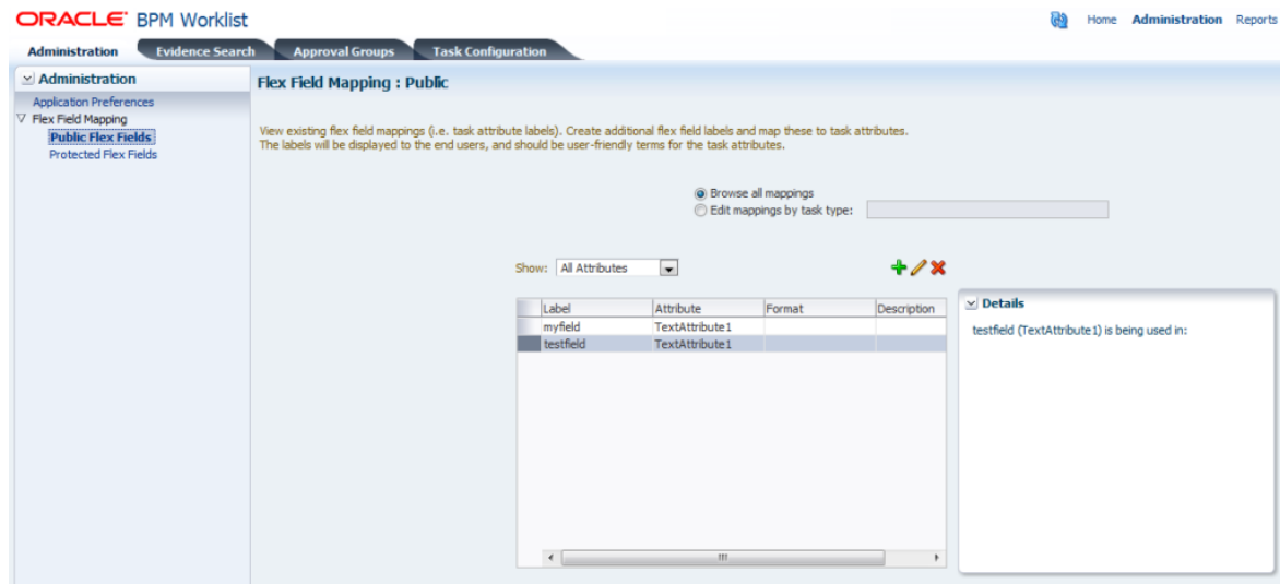
Figure 32–56 Browsing Mappings
