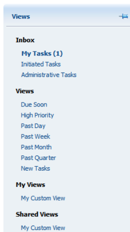
Figure 32–11 Worklist Views
