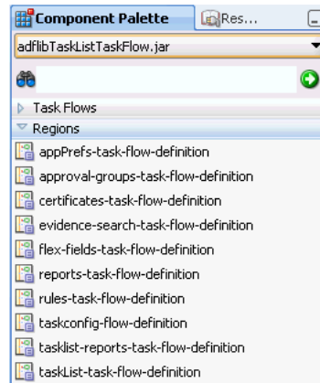
Figure 32–69 Component Palette
