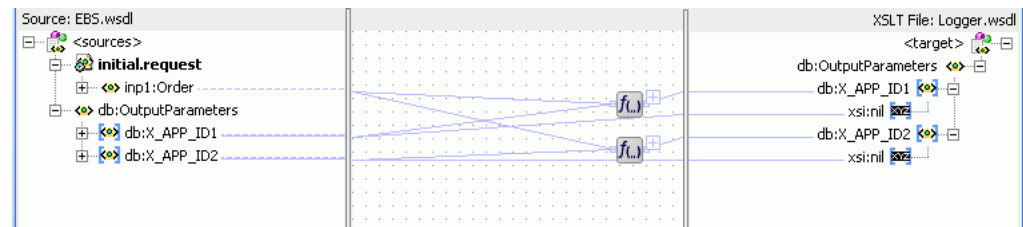
Figure 49–60 EBS_TO_COMMON_INSERT.xsl Transformation
