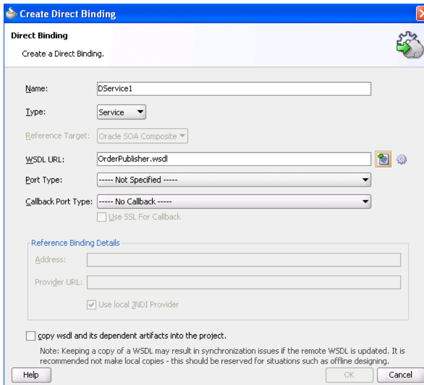
Figure 39–4 Create Direct Binding Dialog
