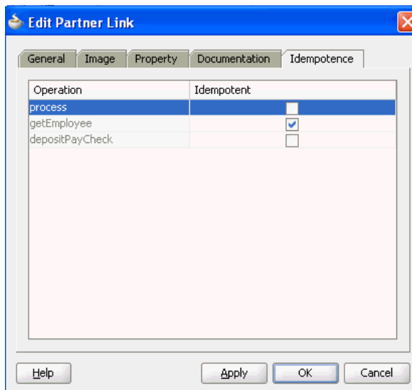
Figure 12–19 Idempotence Tab of Edit Partner Link Dialog
