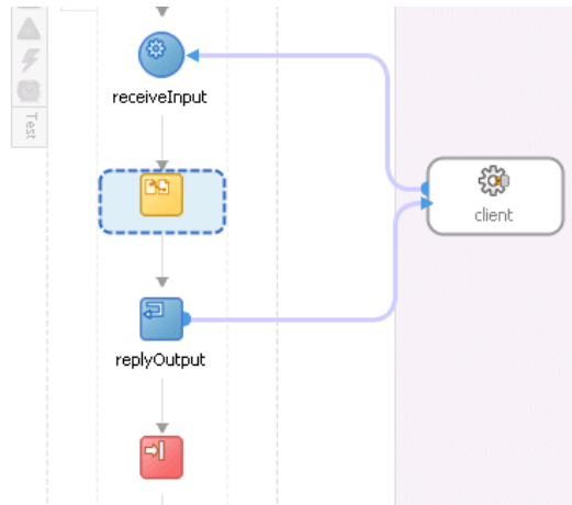
Figure 12–30 Exit Activity in a BPEL Process
