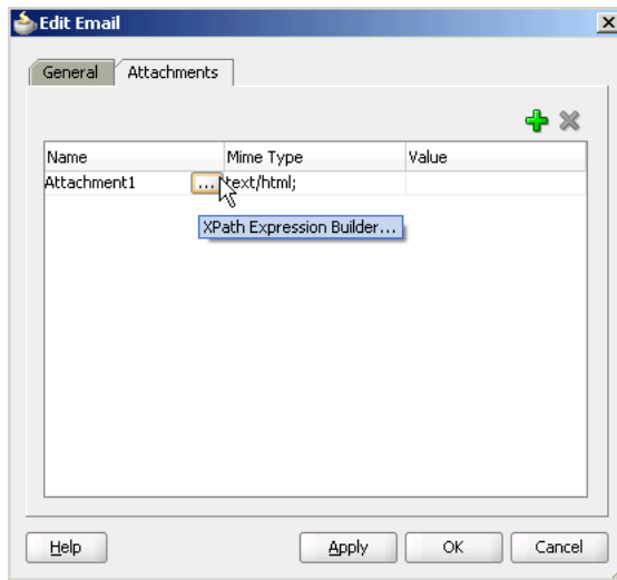
Figure J-29 Edit Email Window
