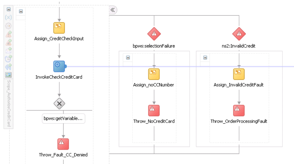
Figure 12–17 Scope Activity After Design Completion
