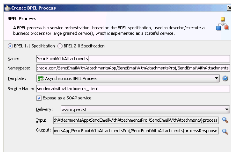
Figure J-24 Creating the BPEL Process
