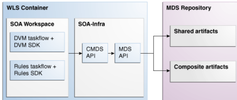
Figure 48–1 Oracle SOA Composer High-Level Deployment Topology
