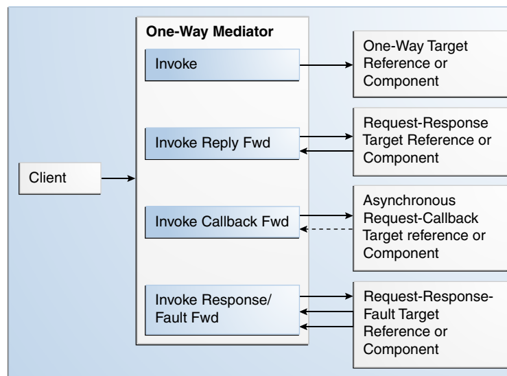
Figure 24-1 One-way Message Exchange Pattern
