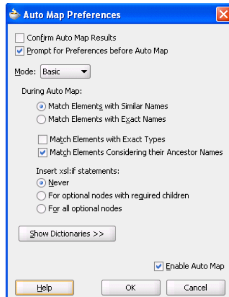
Figure 40–31 Auto Map Preferences
