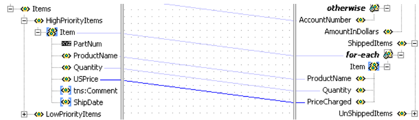
Figure 40–28 Creating Loops with xsl:for-each
