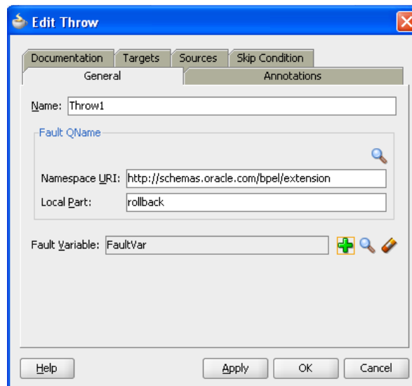
Figure 12–13 Throw Activity with bpelx:rollback Extension
