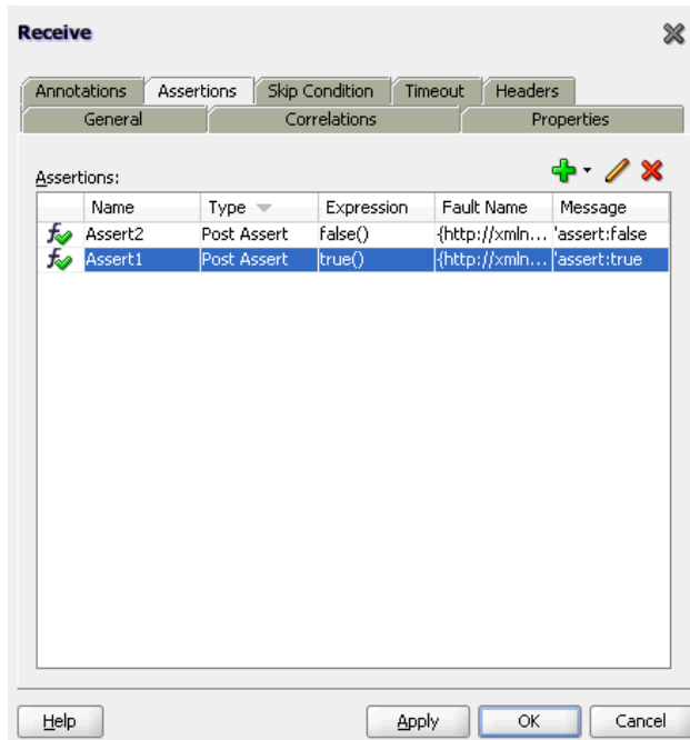
Figure 12–34 Assertions Tab with Data
