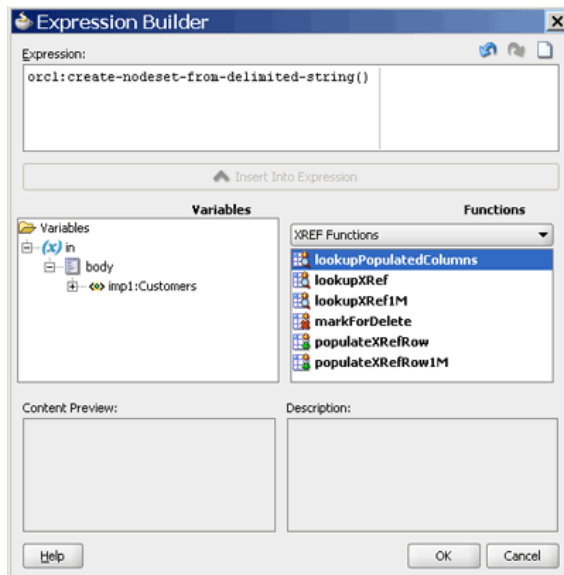
Figure 49–6 Expression Builder Dialog with Cross Reference Functions
