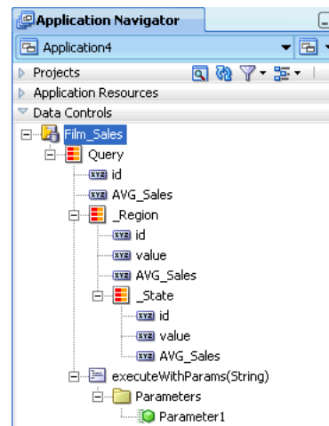
Figure 54–1 Data Controls Panel in Oracle JDeveloper
