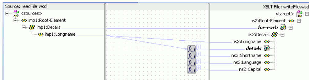
Figure 47-28 Complete imp1:Root-Element To ns2:Root-Element Transformation
