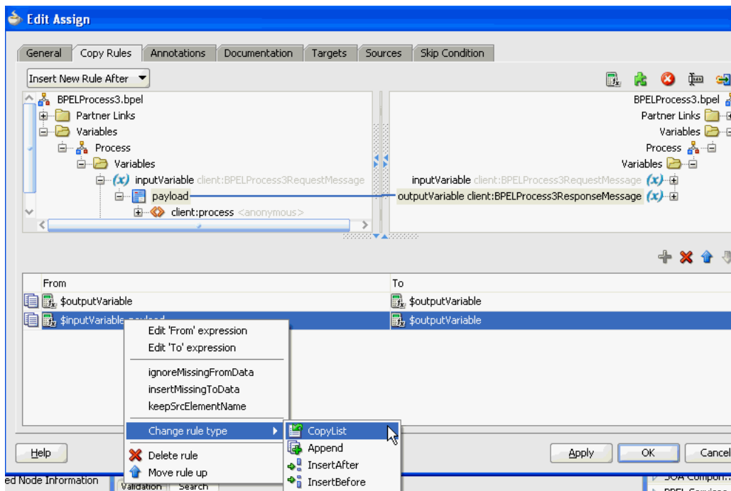
Figure 6–11 Copy Rule Converted to bpelx Extension in BPEL 2.0
