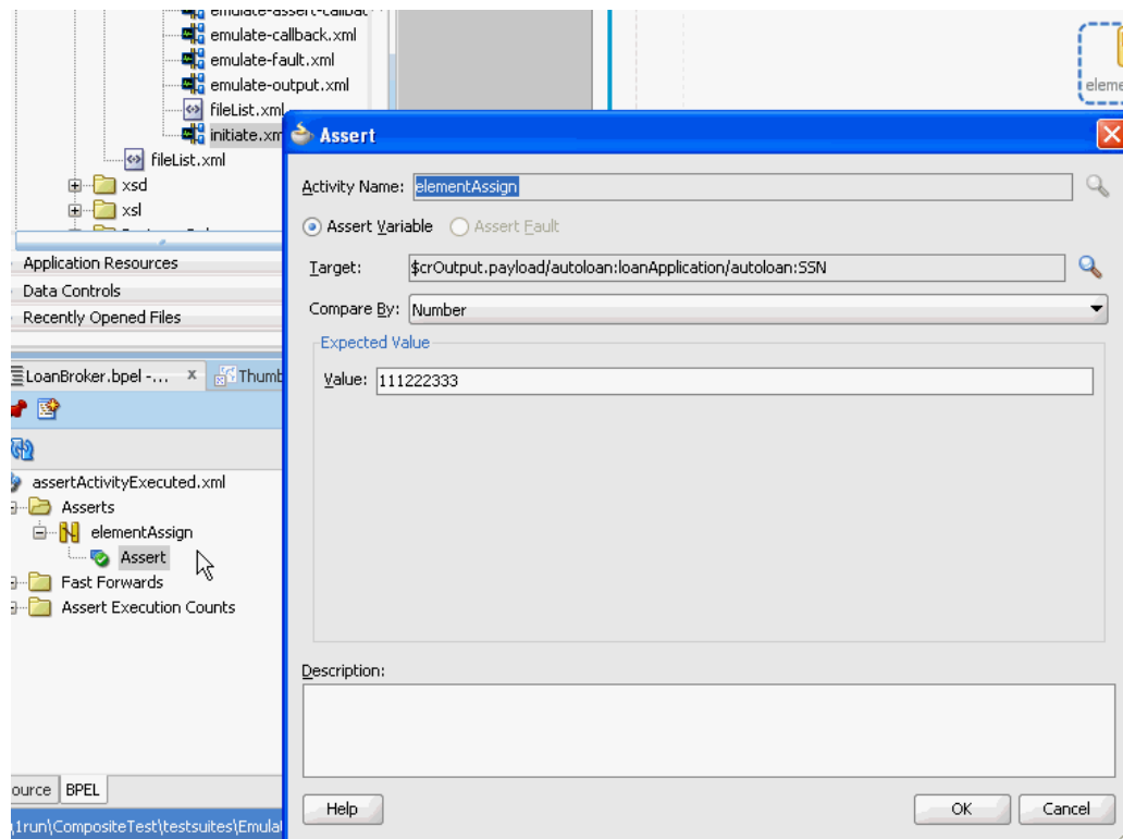
Figure 44–24 Assert Folder in Structure Window
