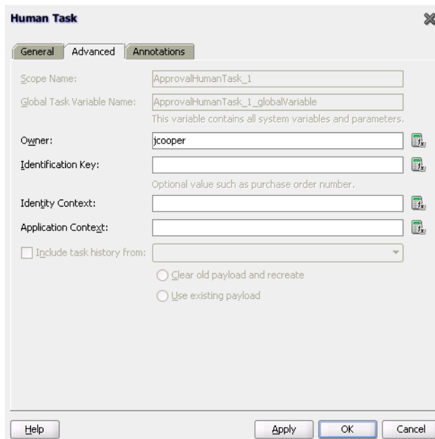
Figure 28–11 Create Human Task — Advanced Tab
