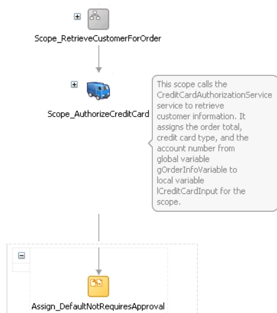
Figure 12–18 Scope with Descriptive Note and Modified Image
