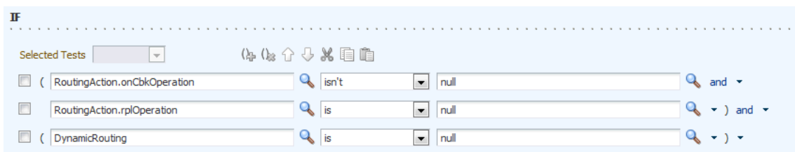
Figure 26–8 Nested Rules Support
