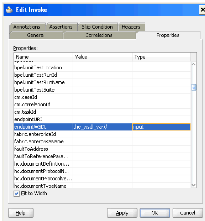
Figure 8–10 endpointWSDL Normalized Message Property of Invoke Activity
