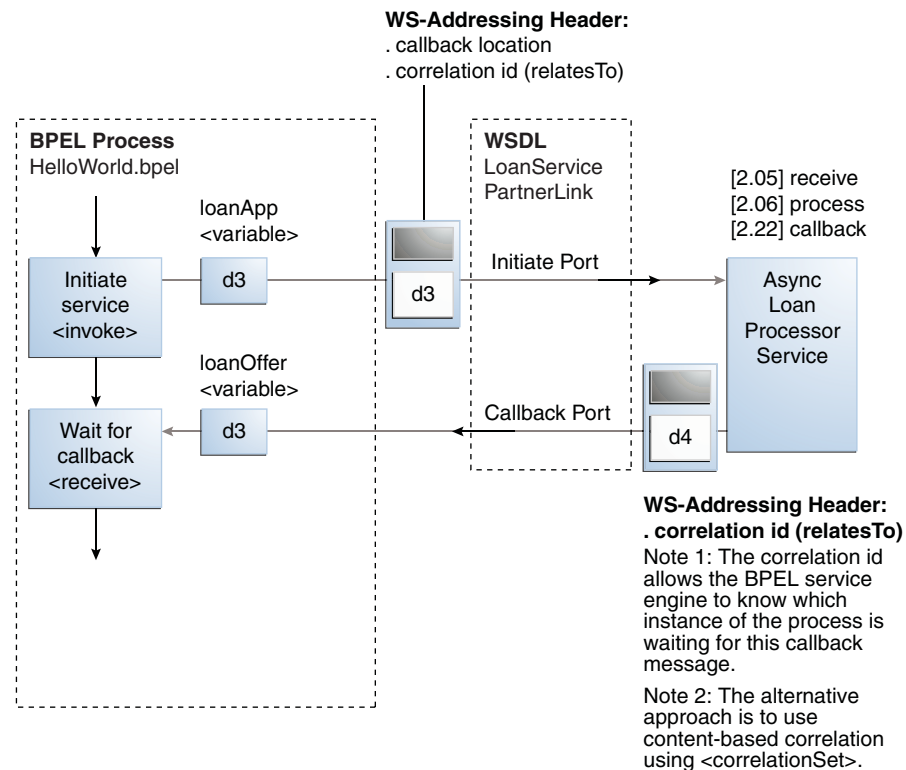
Figure 8–11 Callback with WS-Addressing Headers
