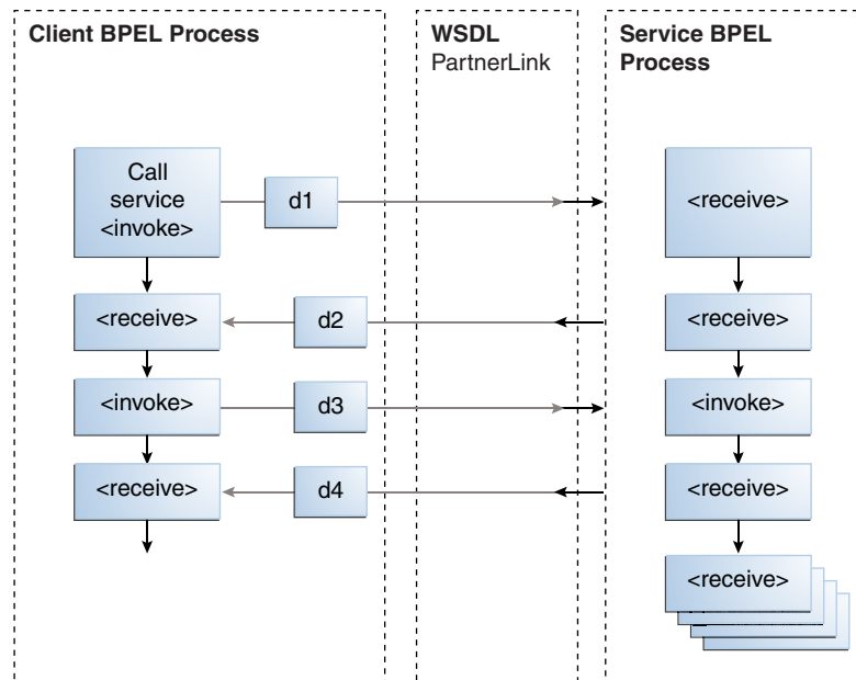
Figure 5–9 Partial Processing
