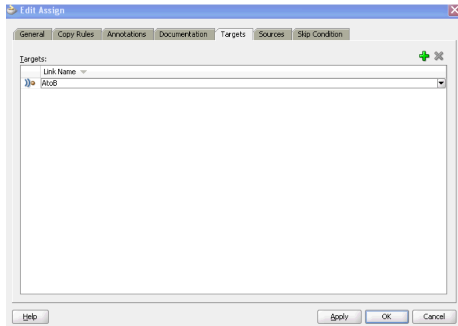
Figure 10–7 Target Activity
