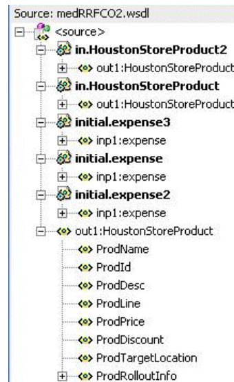
Figure 40–10 Reply Part
