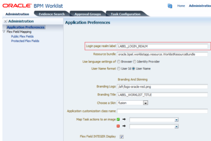
Figure 32-73 Application Preferences
