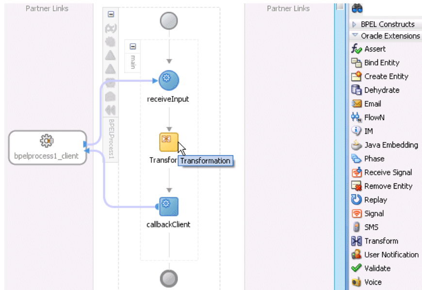
Figure 40–4 Transform Activity
