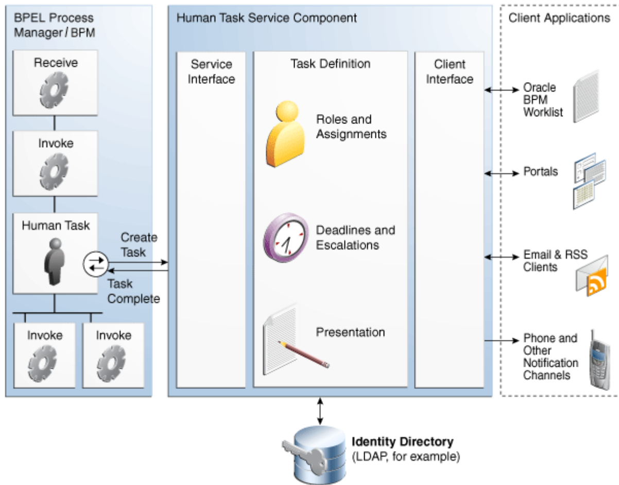
Figure 27-1 Human Workflow
