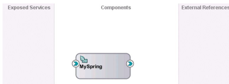
Figure 52-7 Reference Handle
