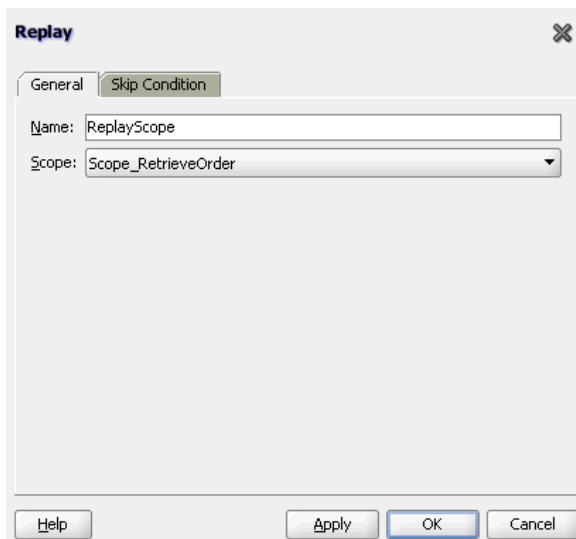
Figure 12–24 Replay Dialog
