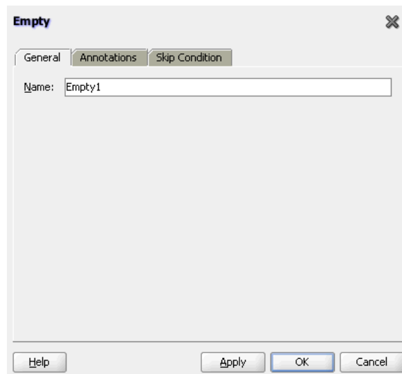
Figure 12–23 Empty Activity
