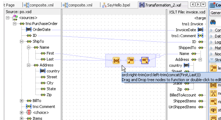
Figure 40–20 Chaining Functions
