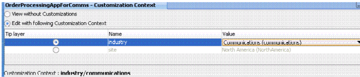
Figure 46–4 Customization Context
