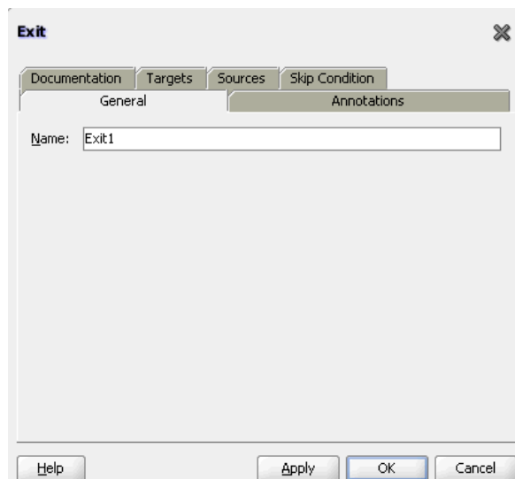
Figure 12–29 Exit Activity
