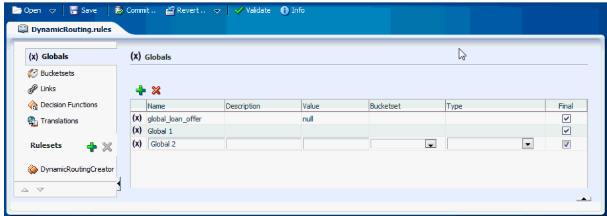
Figure 26–29 Globals Editor
