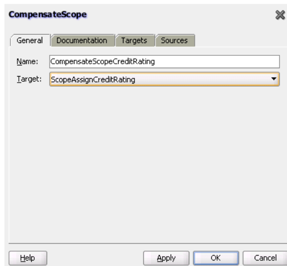
Figure 12–27 CompensateScope Activity
