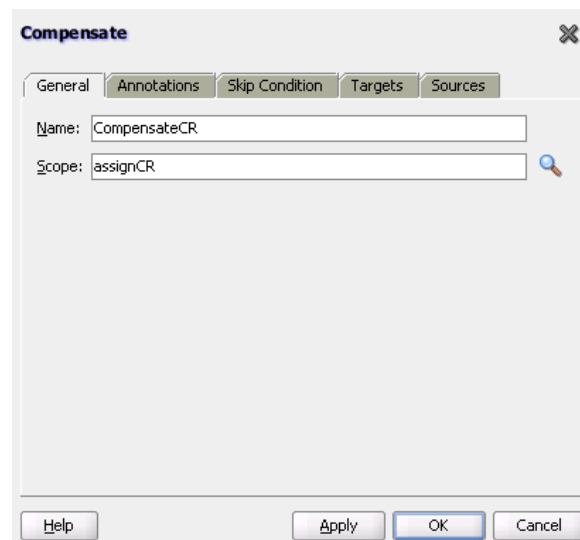
Figure 12–26 Compensate Activity
