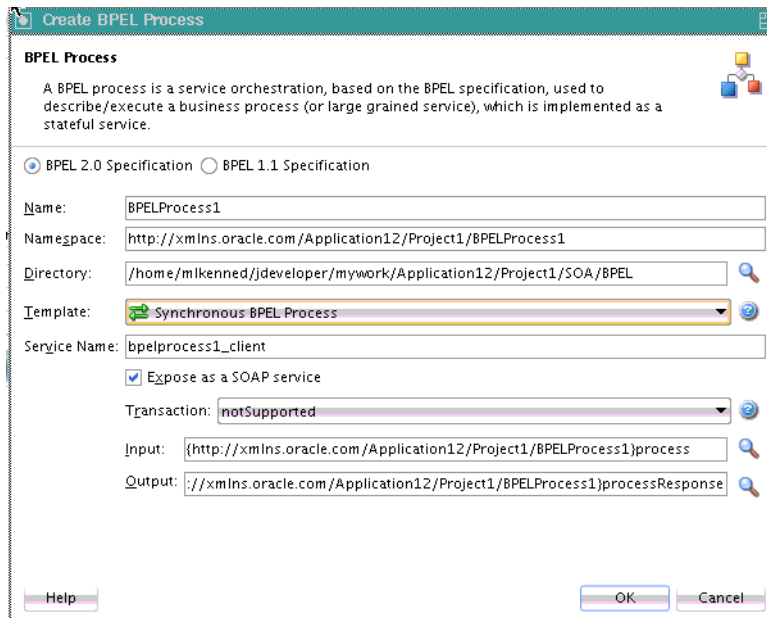
Figure 13–1 Create BPEL Process Dialog
