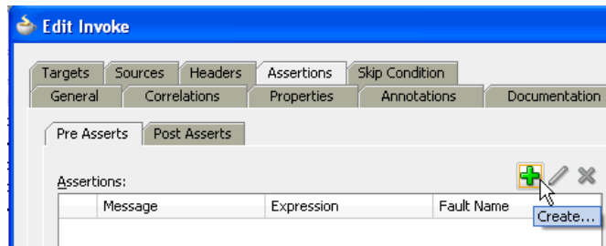
Figure 12–32 Add Icon of Assertions Tab in BPEL 2.0
