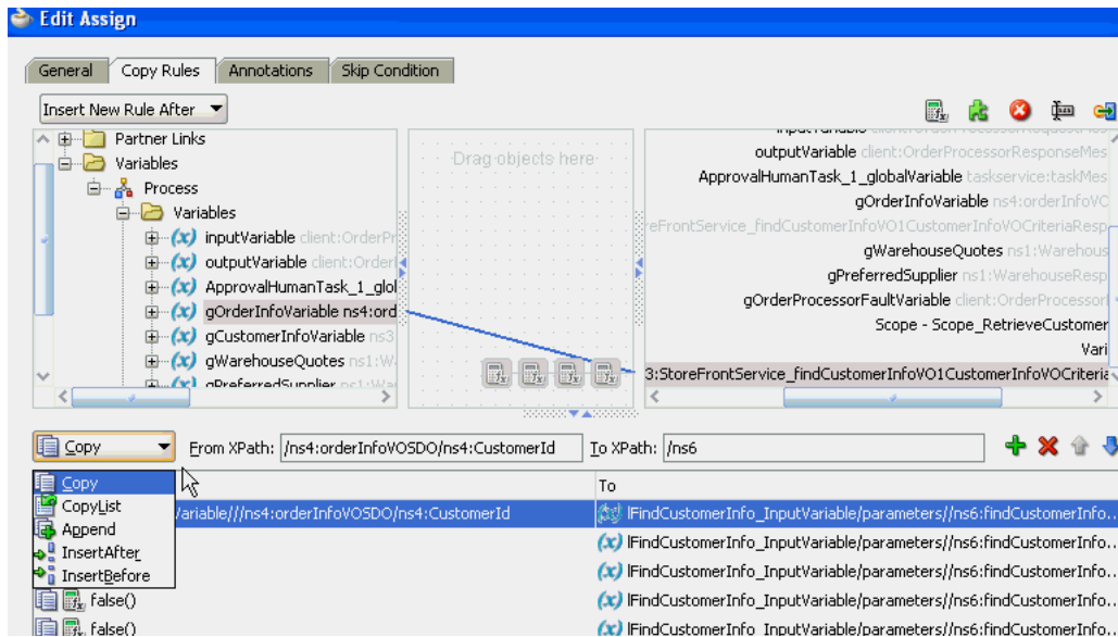
Figure 6–10 Copy Rule Converted to bpelx Extension in BPEL 1.1
