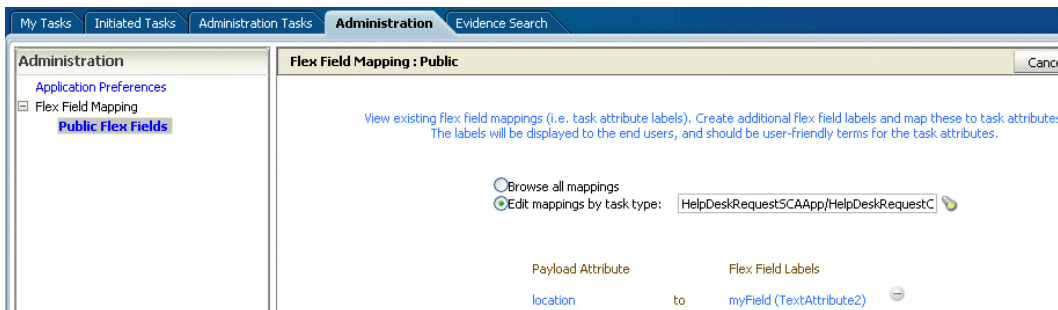
Figure 32–59 Mapped Attribute Mapping Created
