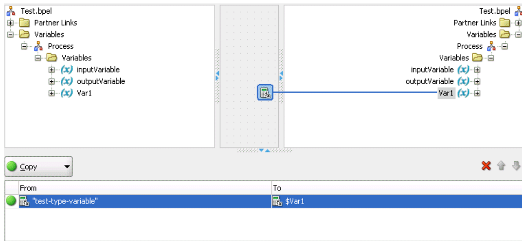
Figure 6–16 Assign Activity
