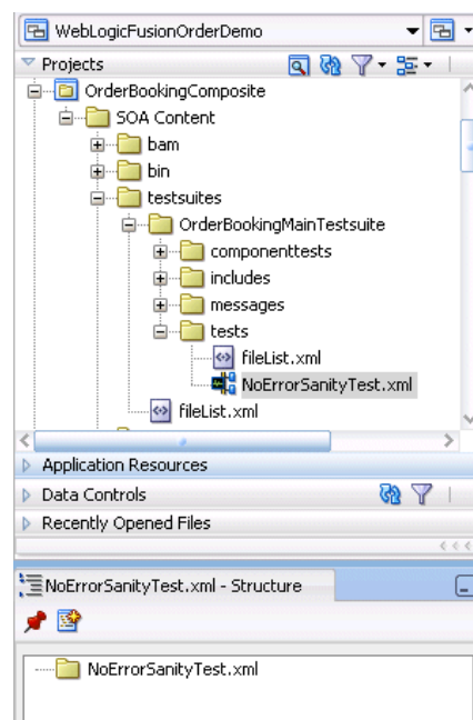
Figure 44-4 NoErrorSanityTest.xml Folder
