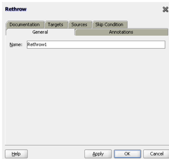
Figure 12–14 Rethrow Dialog
