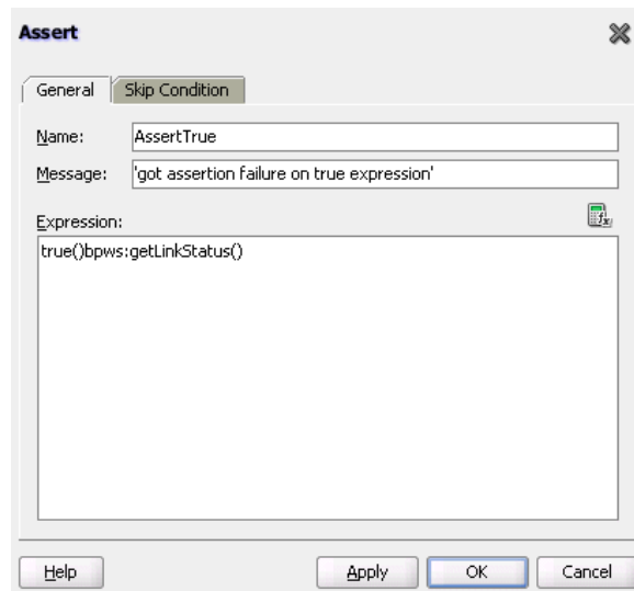
Figure 12–36 Assert Dialog
