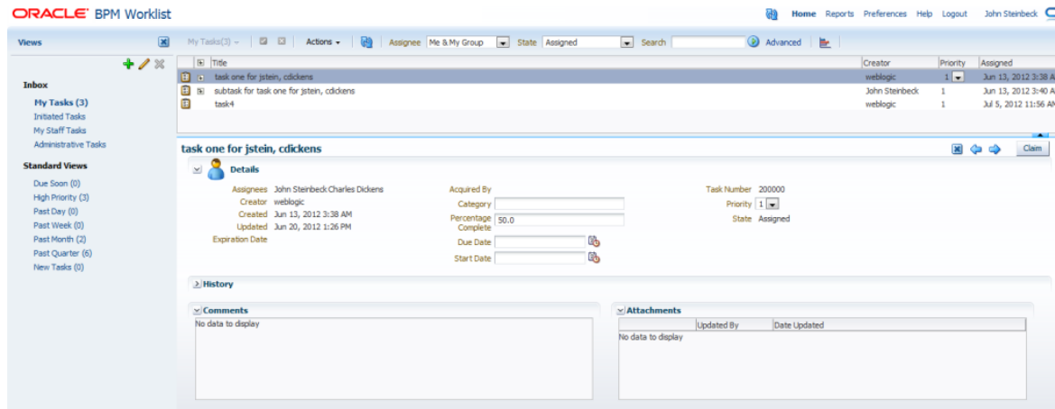
Figure 32–70 Task List
