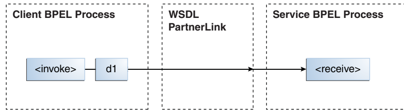
Figure 5–1 One-Way Message
