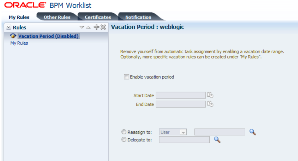
Figure 32-75 Vacation Period
