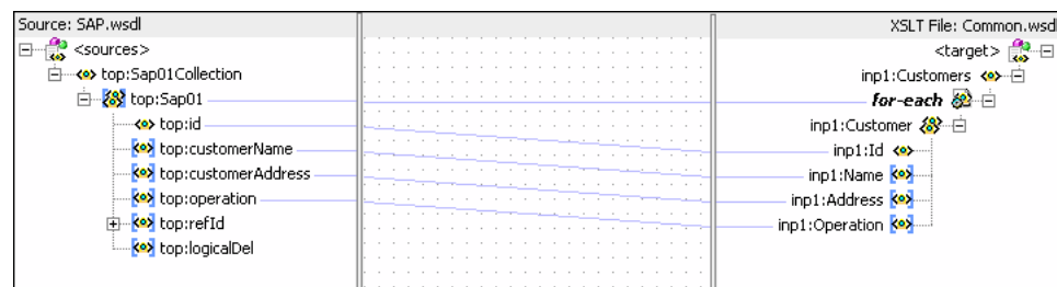
Figure 49-24 SAP_TO_COMMON_INSERT.xml Transformation
