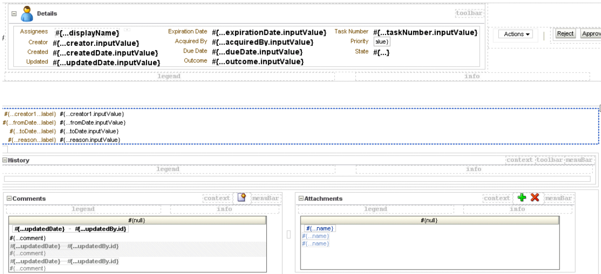
Figure 30–30 The Task Form (taskDetails.jspx)
