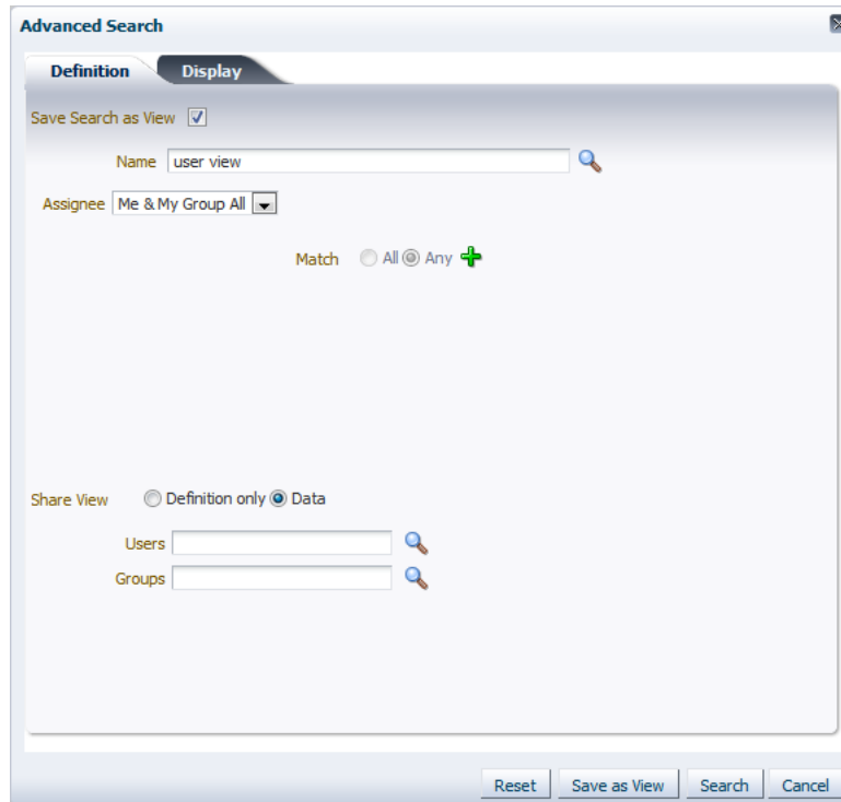
Figure 32-5 Worklist Advanced Search—Definition Tab
