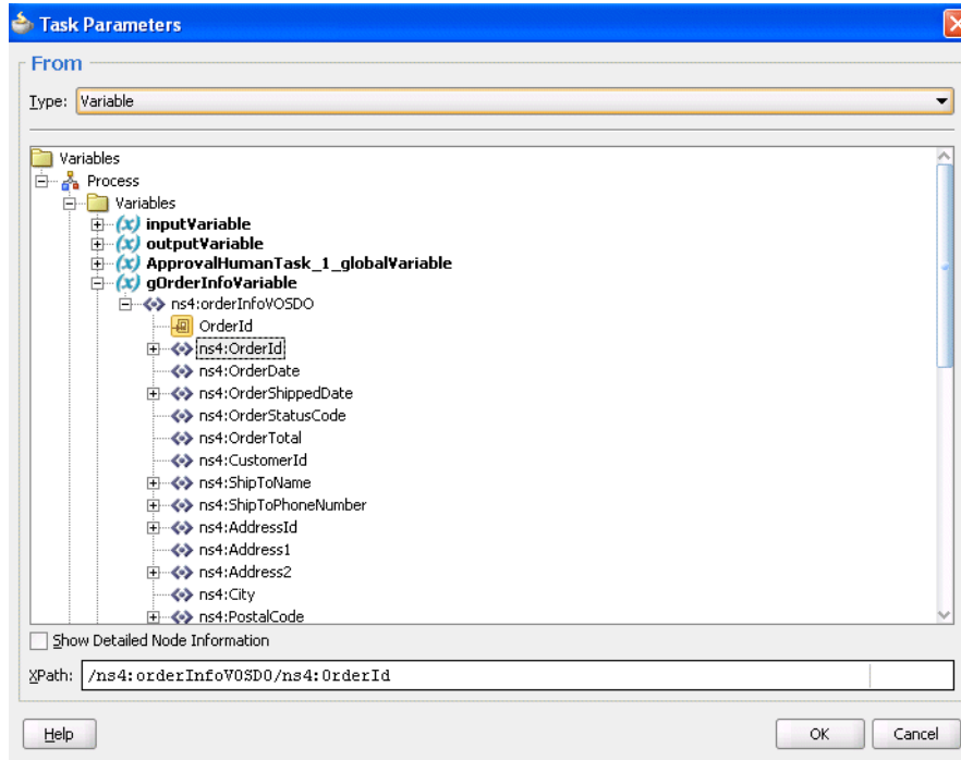
Figure 28–9 Variables Tree
