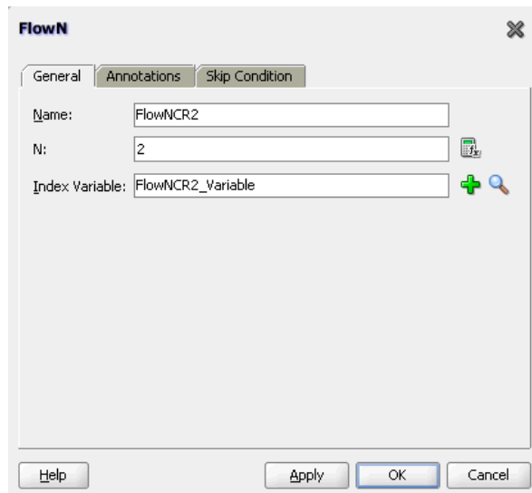
Figure 10–10 FlowN Dialog
