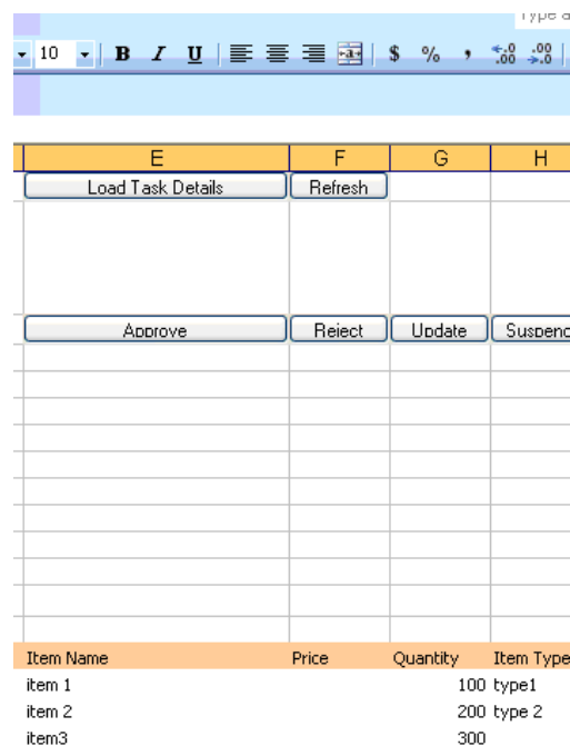
Figure 35–22 Task Actions
