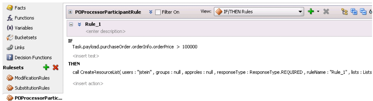
Figure 29–31 Business Rules
