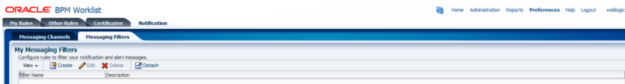
Figure 32–52 Messaging Filters
