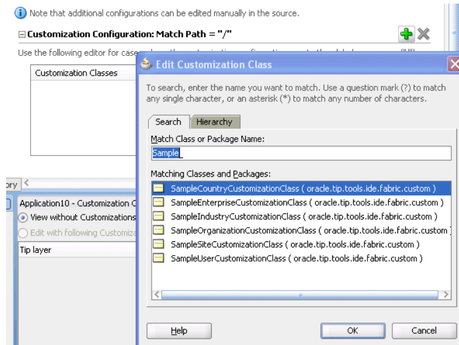
Figure 46–1 Customization Classes
