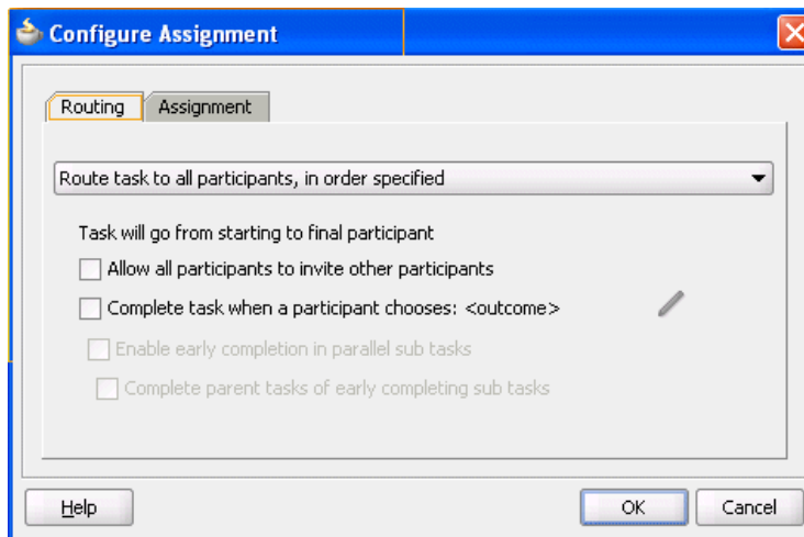
Figure 29–41 Configure Assignment
