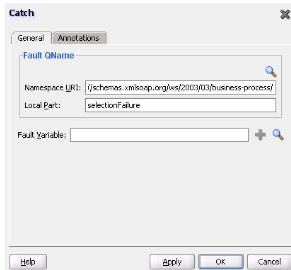
Figure 12–21 Catch Dialog
