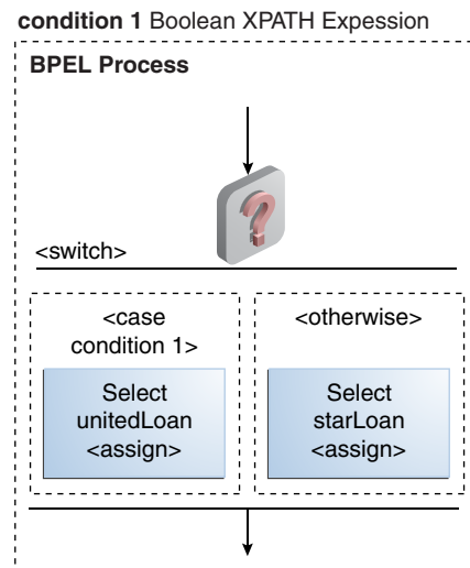
Figure 11–1 Conditional Branching
