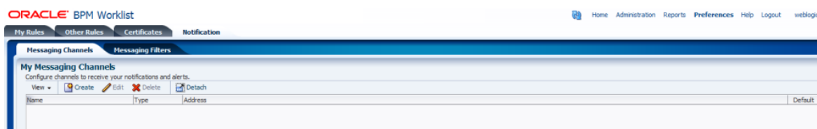
Figure 32–51 Messaging Channels
