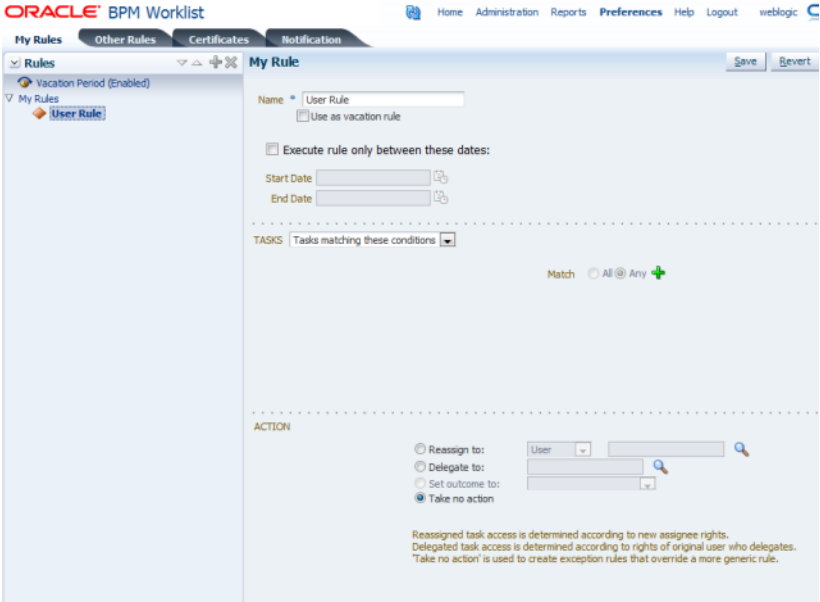
Figure 32-76 My Rule
