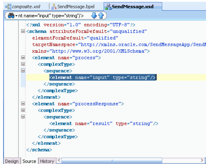
Figure J-6 Modifying the Inputs in the SendMessage.xsd File
