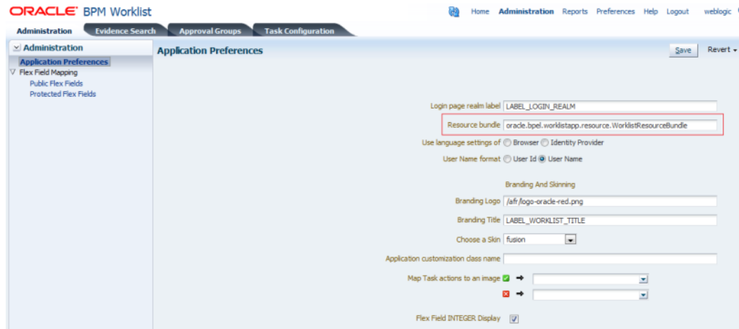
Figure 32–43 Specifying the Resource Bundle
