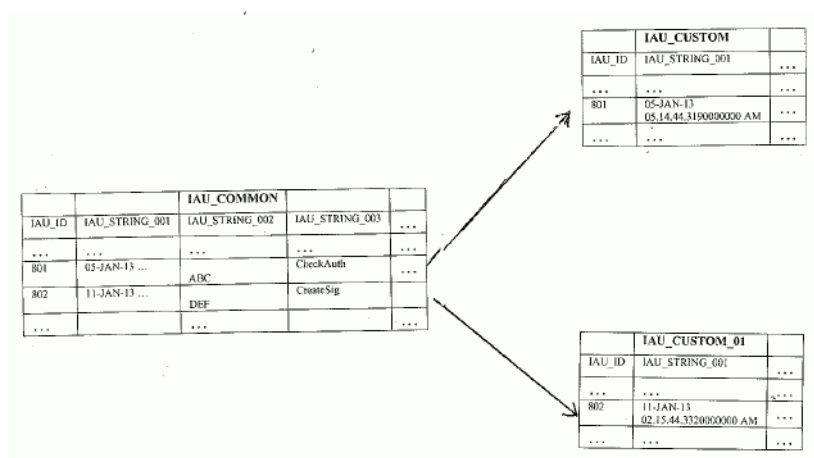
Figure 13–1 Common and Custom Audit Tables
