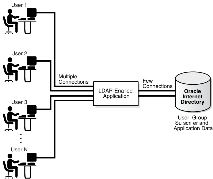
Figure 1-1 A Directory-Enabled Application
