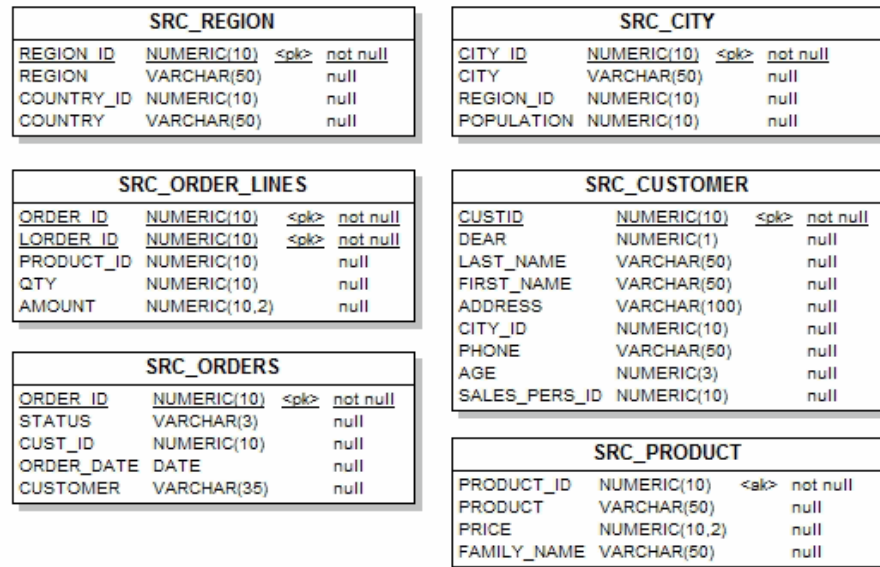
Figure 3–2 Orders Application Schema Diagram
