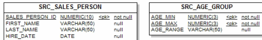
Figure 3–3 Parameters Schema Diagram
