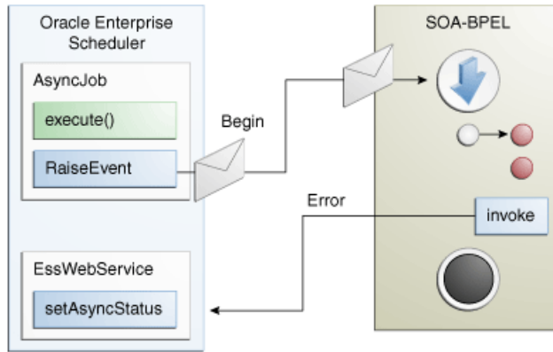
Figure 16–13 BPEL Handling Error
