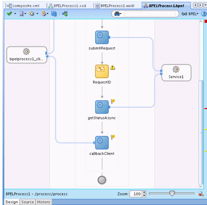
Figure 11-18 Adding RequestID Assign Activity
