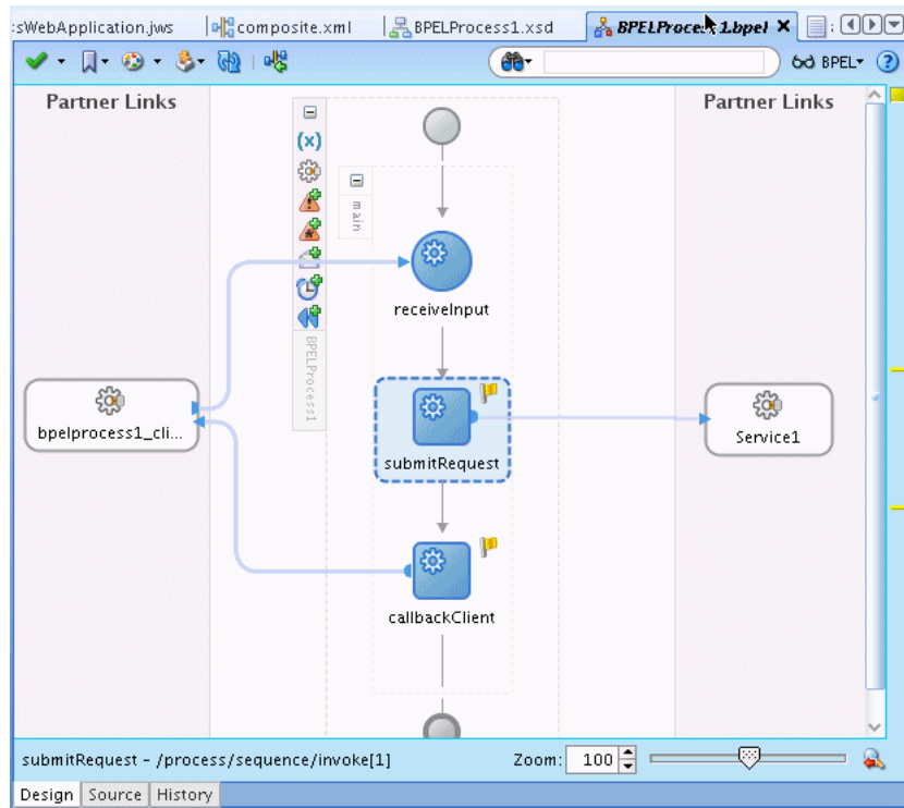
Figure 11-9 Adding the submitRequest Invoke Activity
