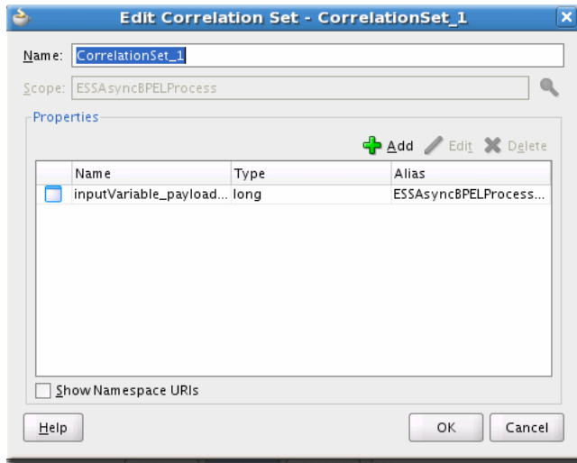
Figure 16–15 Edit Correlation Set
