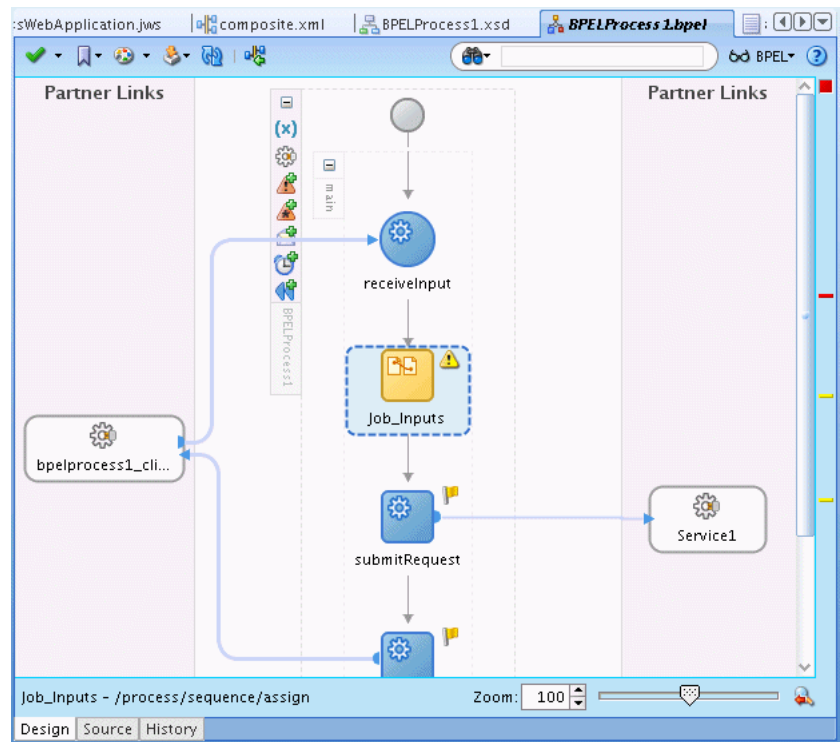
Figure 11–10 Adding an Assign Activity to BPEL
