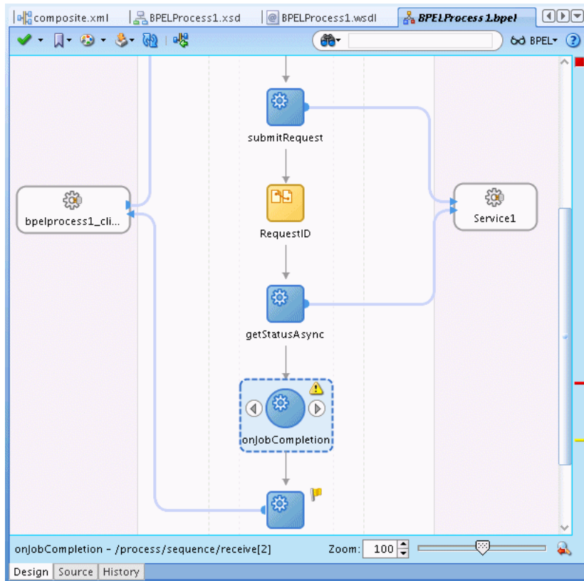
Figure 11–21 Adding Receive Activity to BPEL Process
