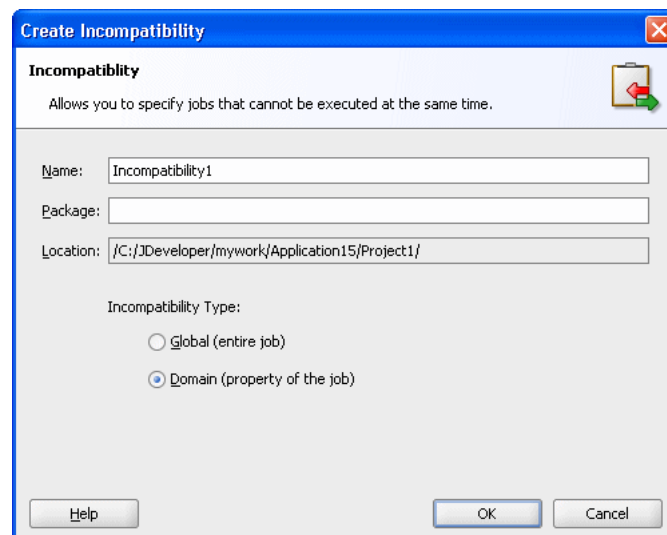
Figure 13-4 Create Incompatibility Window
