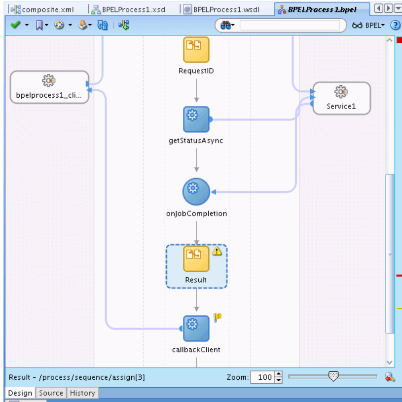
Figure 11-24 Adding Assign Activity for Output to Client
