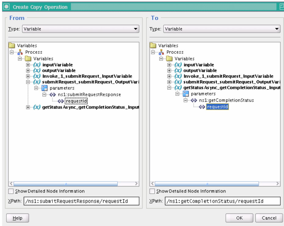
Figure 11–19 Edit Copy Operation Window for Request ID Assign
