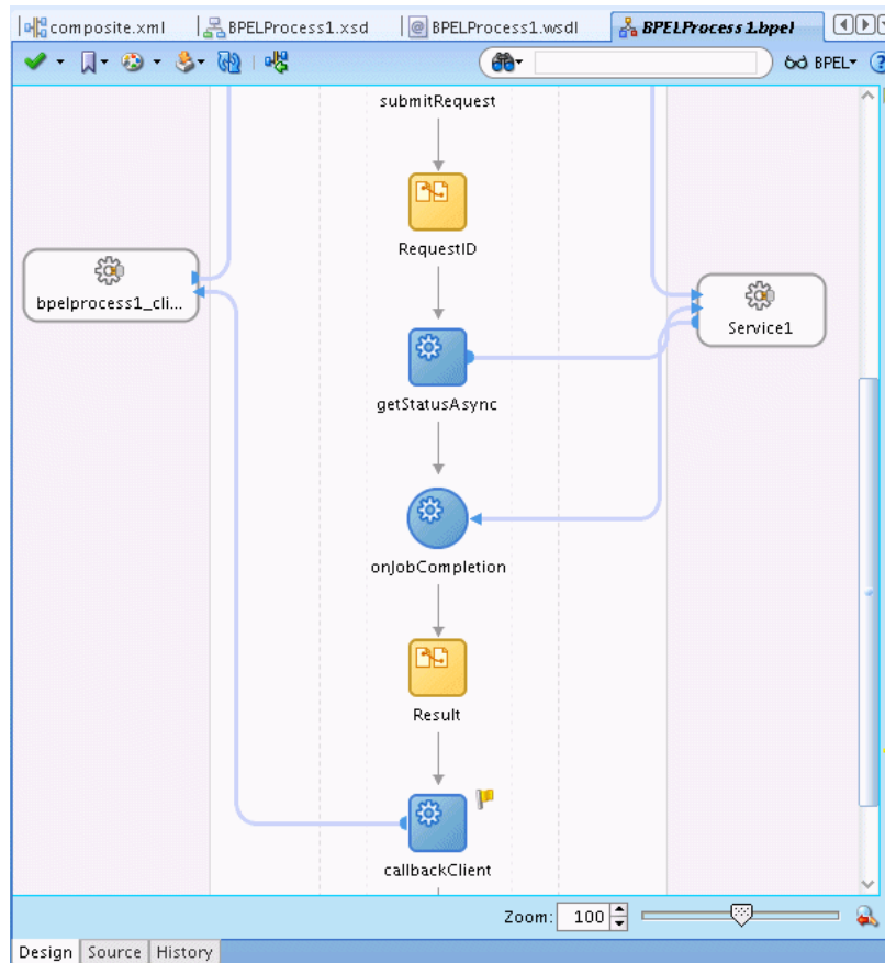
Figure 11–26 Result Assign Activity with callbackClient Invoke Activity
