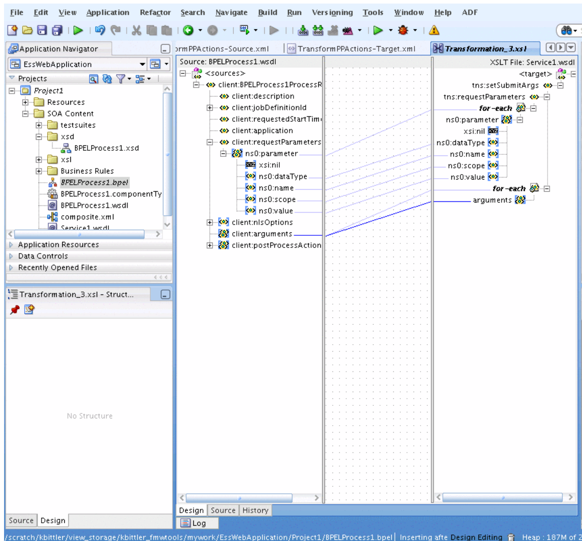
Figure 11–30 Transformation for Set Submit Arguments
