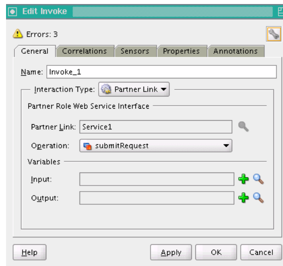
Figure 11-27 Edit Invoke Window for BPEL Activity
