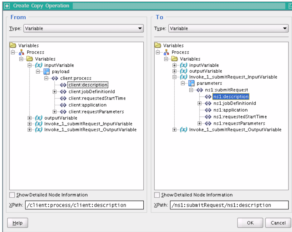
Figure 11–12 Copy Operation for Description Parameter for submitRequest
