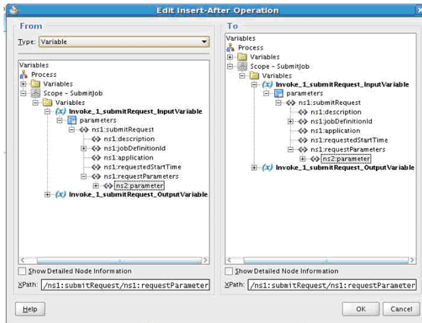
Figure 11–29 Copy with Insert-After Operation
