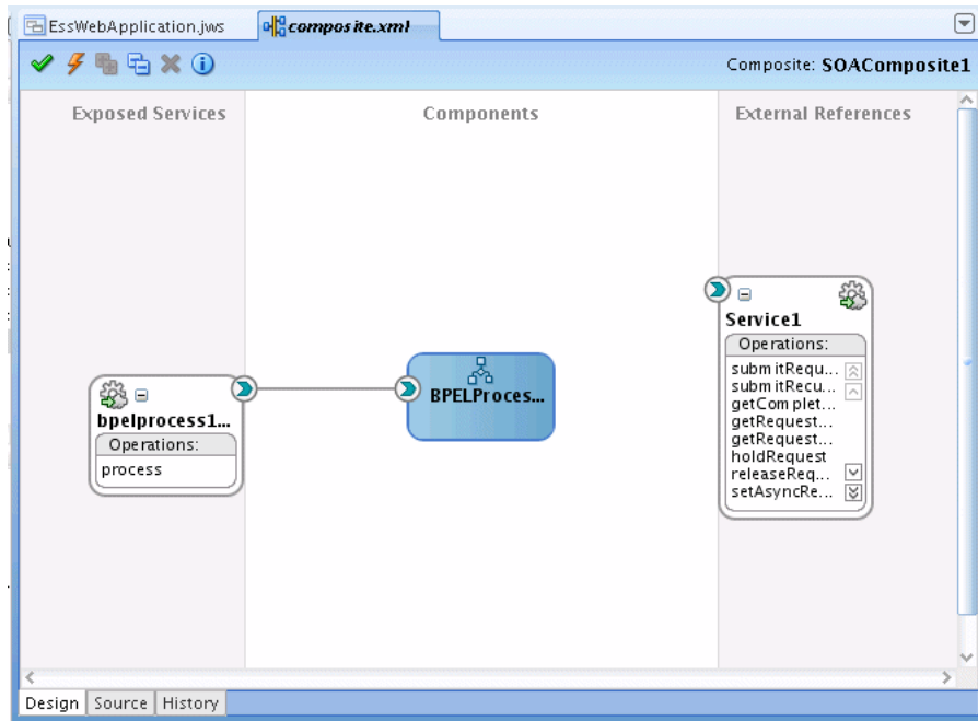
Figure 11–5 Adding a BPEL Process to the SOA Composite Application
