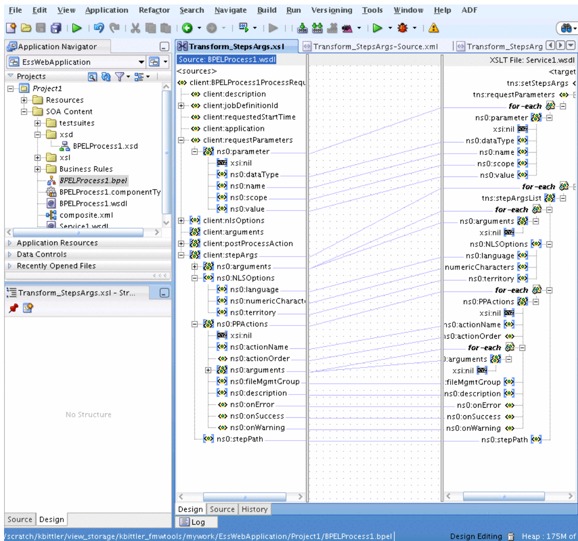
Figure 11–33 Using the Transformation for Set Step Arguments Operation
