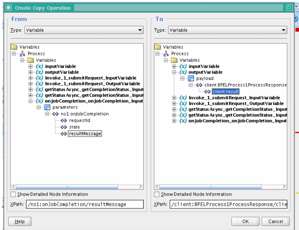
Figure 11–25 Create Copy Operation for Result
