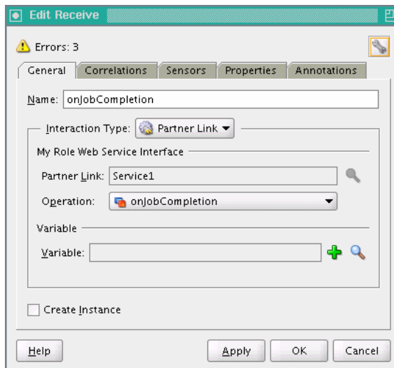
Figure 11–22 Edit Receive Window for onJobCompletion Receive Activity
