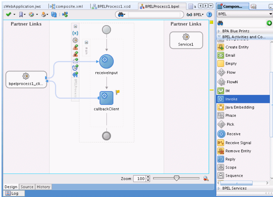
Figure 11–7 BPEL Process Before Adding Invoke Activity for ESSWebService SubmitRequest
