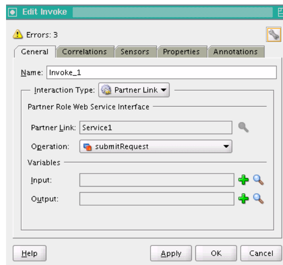
Figure 11–8 Edit Invoke Dialog for BPEL Activity
