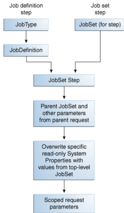
Figure 7-2 Parameter Precedence for Job Set Steps
