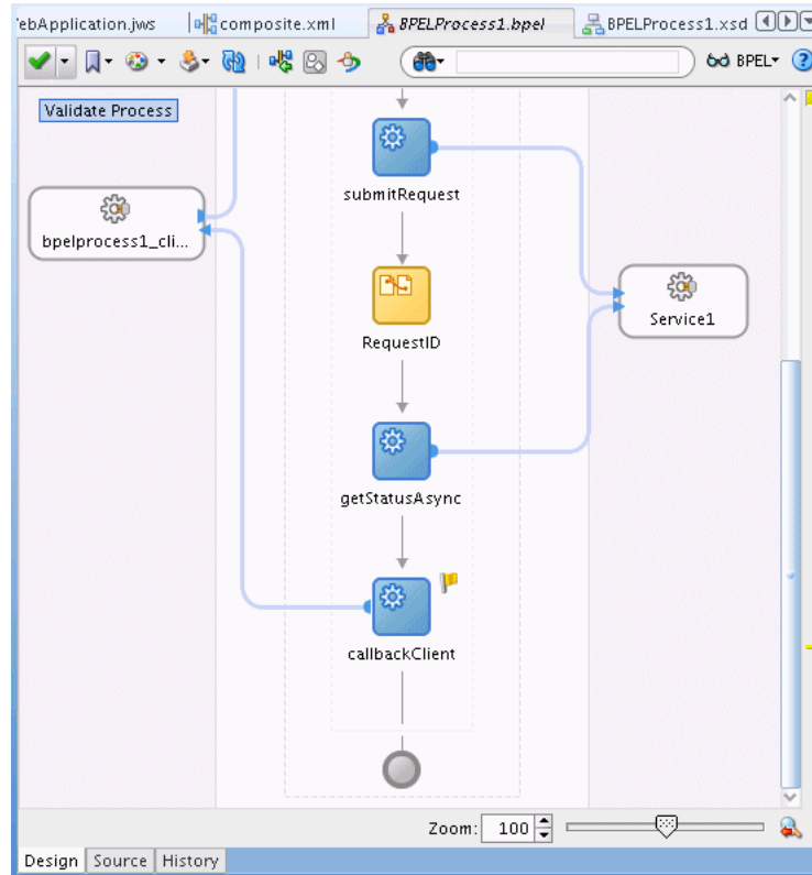
Figure 11–20 BPEL with Request ID Assign Activity Added
