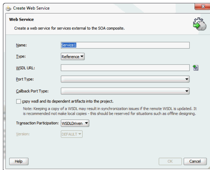
Figure 11–2 Create Web Service Dialog
