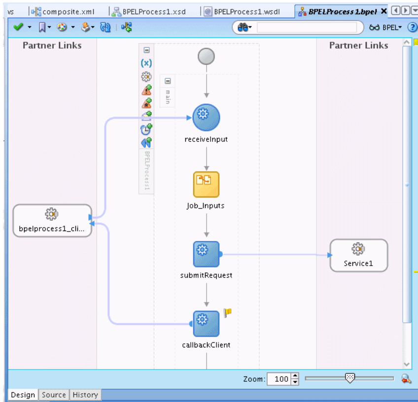
Figure 11–14 BPEL with Job_Inputs Add Activity and submitRequest Invoke
