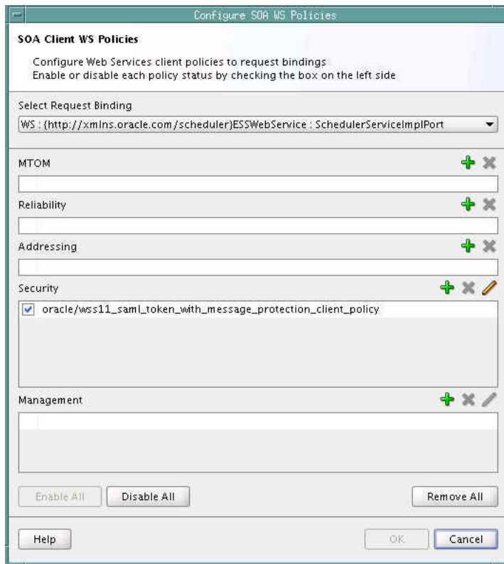
Figure 11–34 Client Security Policy for the Oracle Enterprise Scheduler Web Service
