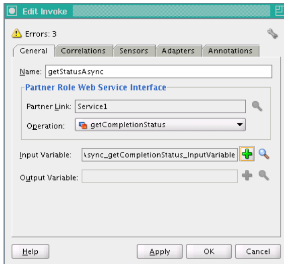
Figure 11–17 Edit Invoke Window for getStatusAsync
