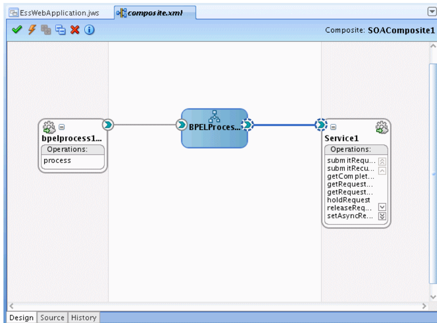
Figure 11–6 Adding A Reference to the Oracle Enterprise Scheduler Web Service in composite.xml
