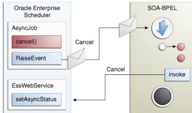
Figure 16–12 BPEL Handling Cancellation
