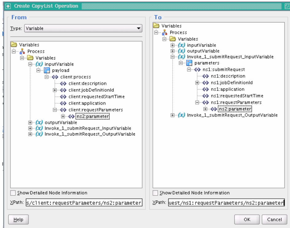
Figure 11–13 CopyList Operation for Request Parameters
