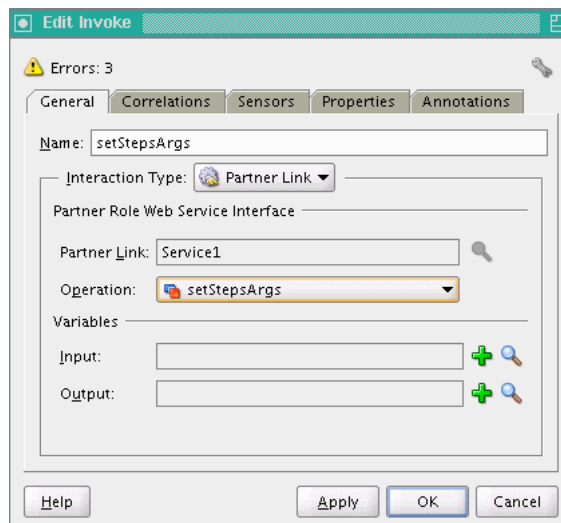
Figure 11–32 Set Step Arguments Operation
