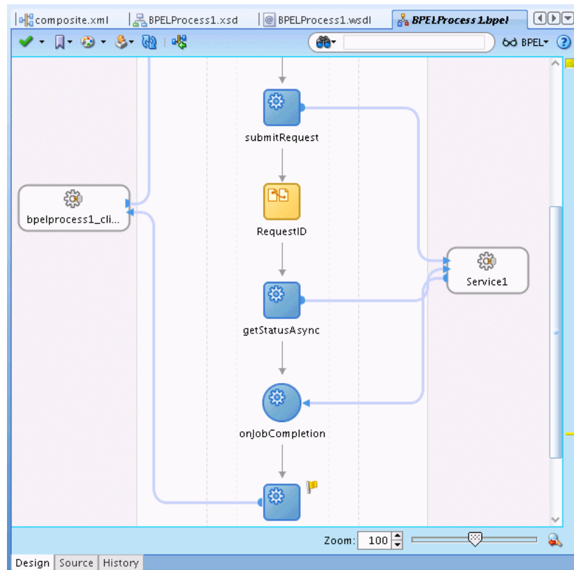
Figure 11–23 Adding the onJobCompletion Receive Activity
