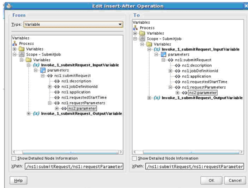
Figure 11–15 Using Insert-After to Clone Parameters
