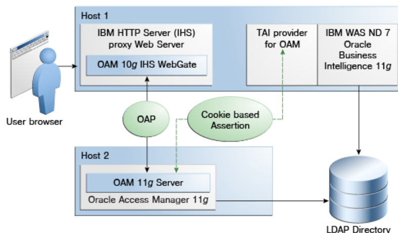
Figure 10–2 Components and Process Flow with OAM 11g and the IAP
