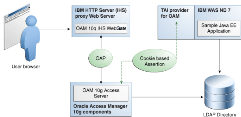
Figure 10–1 Components and Process Flow with OAM 10g (10.1.4.3) and the IAP
