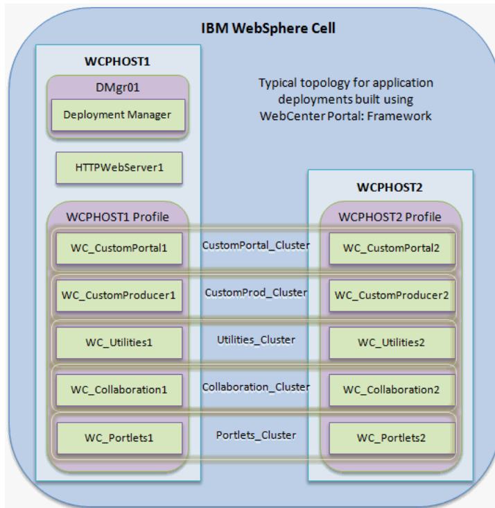
Figure 5–25 Cluster Topology - Portal Framework and Portlet Producer Applications
