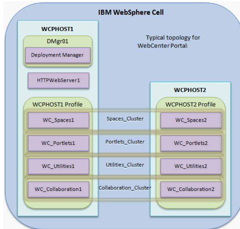
Figure 5–24 Cluster Topology - WebCenter Portal Application
