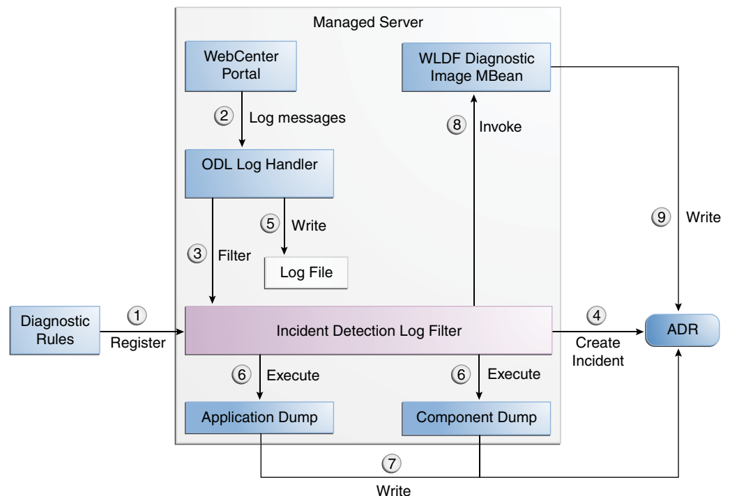
Figure 14–2 Incident Creation Generated by Incident Log Detector
