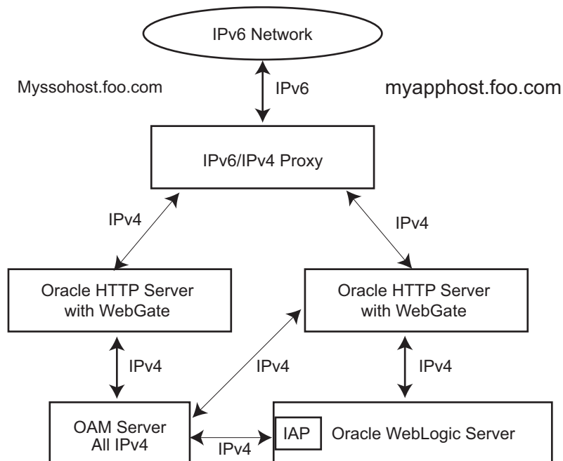
Figure 16–3 IPv6 with an Authenticating WebGate and Challenge Redirect
