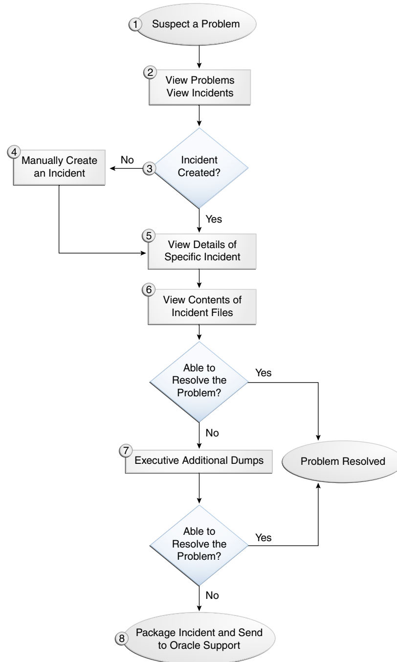
Figure 14-4 Flow for Investigating a Problem
