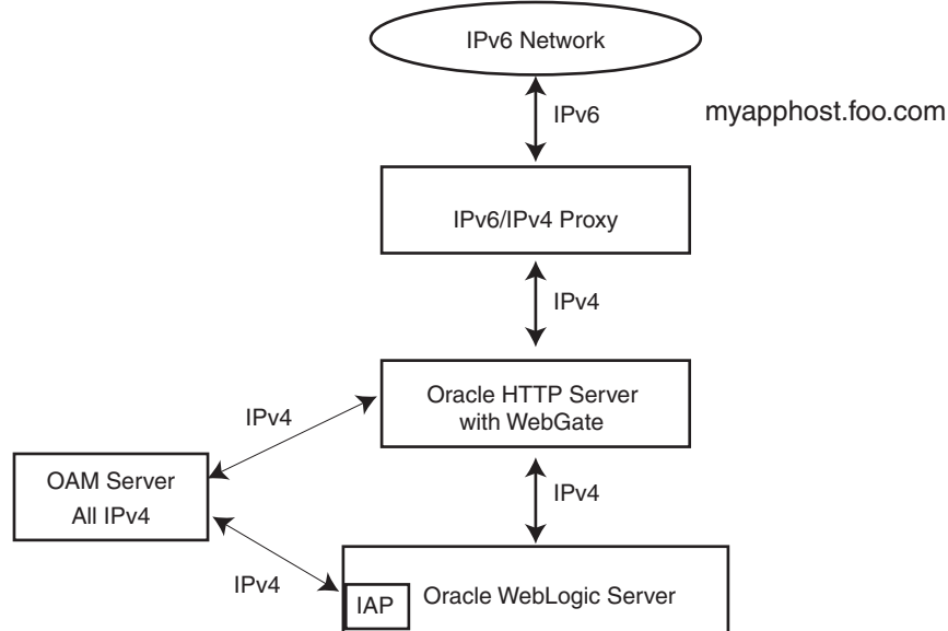
Figure 16–2 Simple Authentication with the IPv6/IPv4 Proxy
