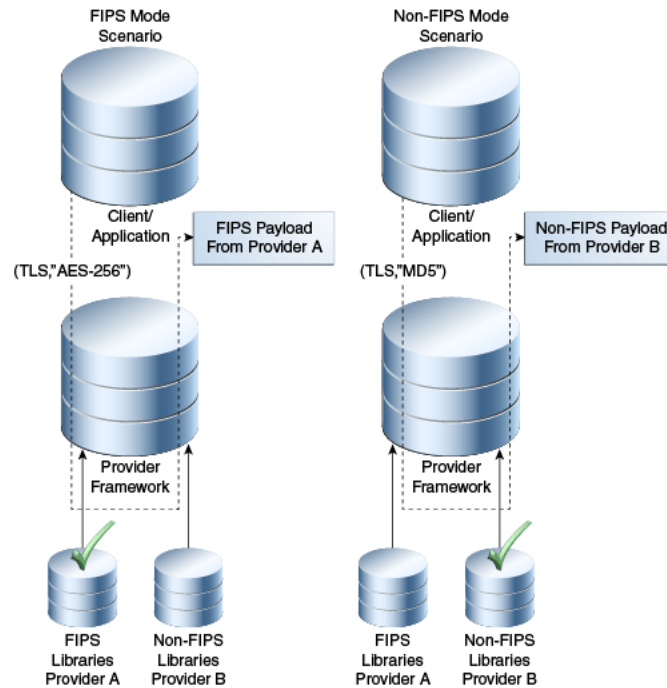
Figure 9–1 Selecting a FIPS 140 Provider
