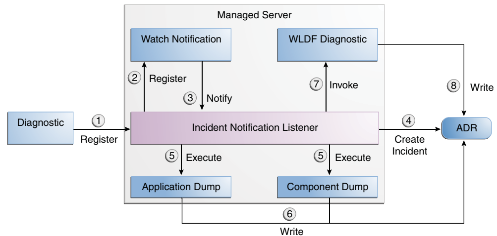
Figure 14–3 Incident Creation Generated by WLDF Watch Notification
