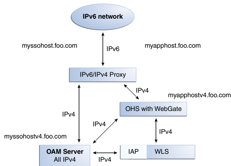
Figure 16–1 IPv6 with Oracle Access Manager and Challenge Redirect
