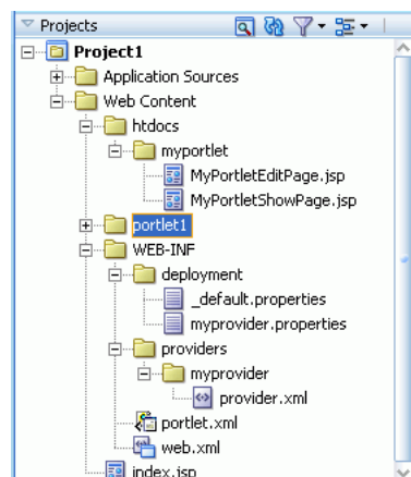
Figure 6–30 Application Navigator
