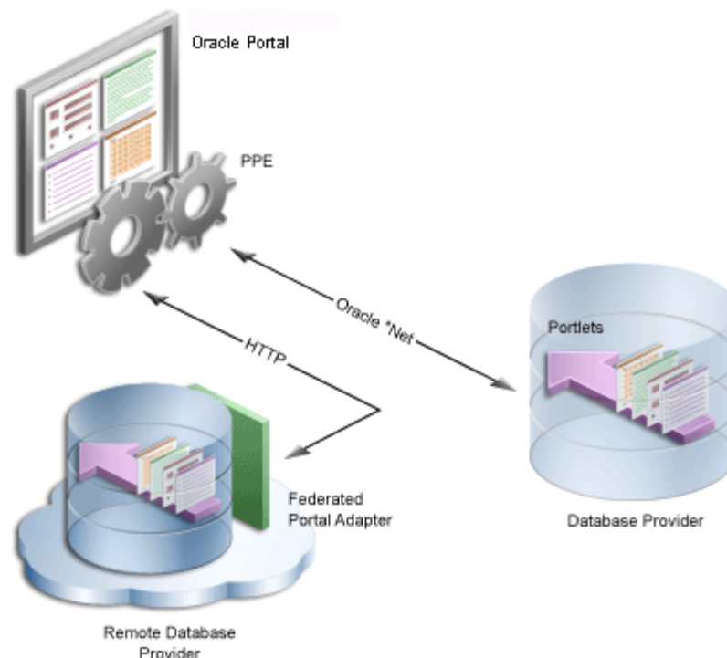
Figure 2–3 Database Providers
