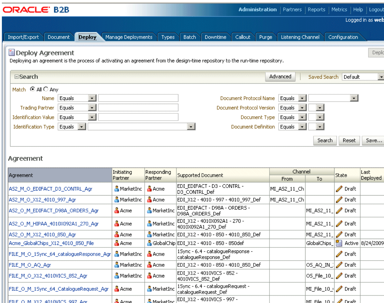
Figure 6-5 The Deploy Tab—Lists Valid Agreements
