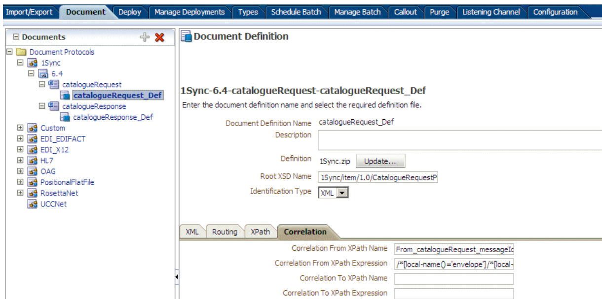
Figure 8–27 The Correlation Tab for a 1Sync Document Definition
