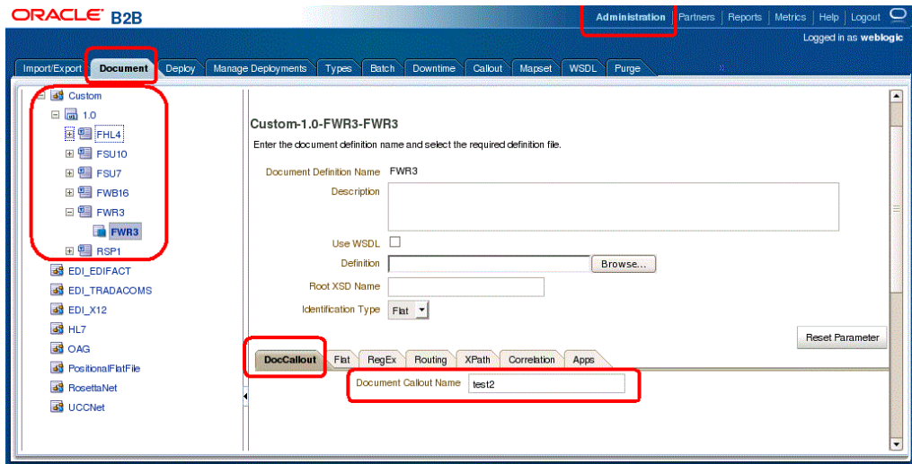
Figure 8-3 Document Definition Parameters for an DocCallout-Type Custom Document
