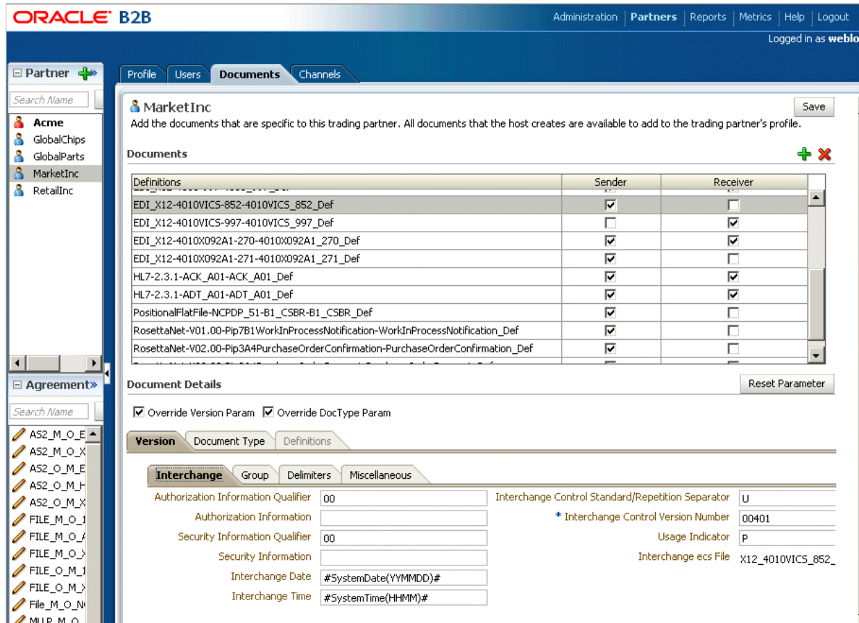
Figure 8–28 Changing Document Details
