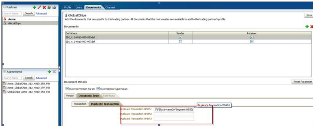
Figure 8–13 Document Type Parameters for an EDI X12 Document
