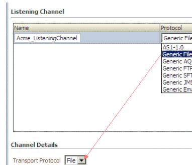
Figure 16–2 Channel Details: The Transport Protocol
