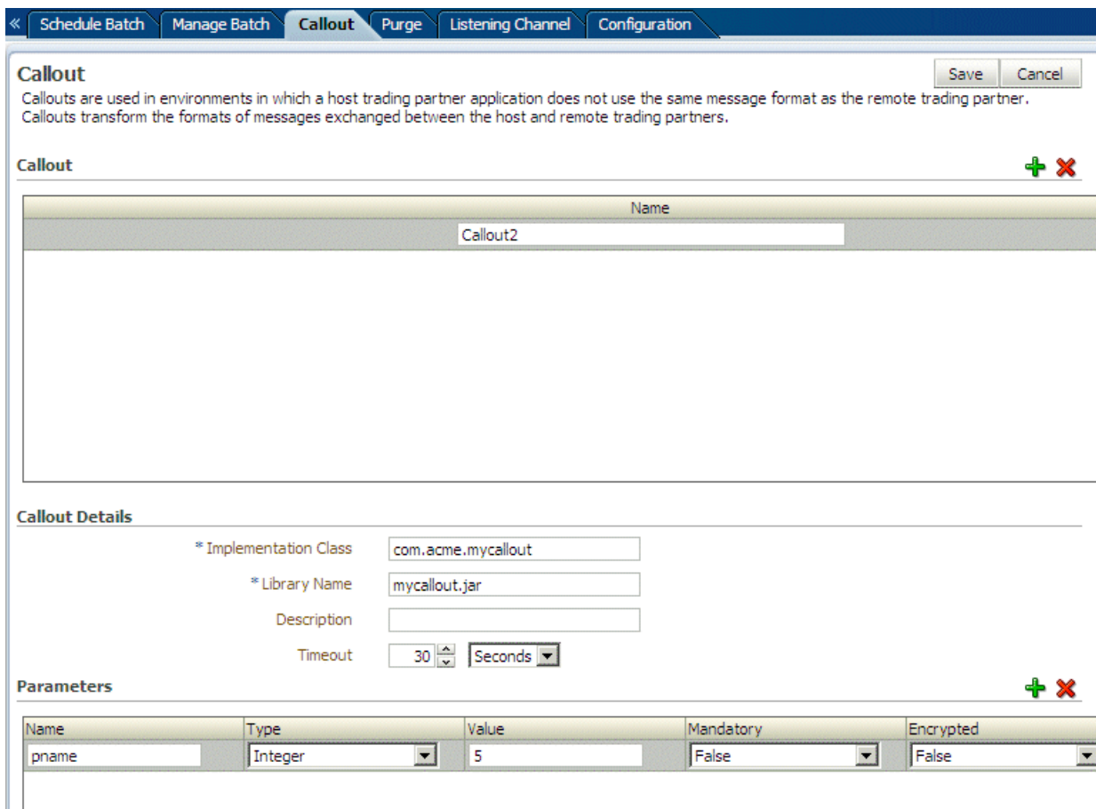
Figure 13–4 Creating a Callout
