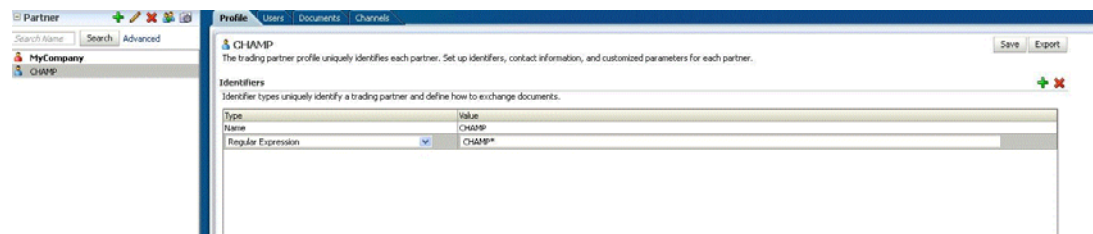
Figure 8–8 Trading Partner Profile Screen- Identifier Details
