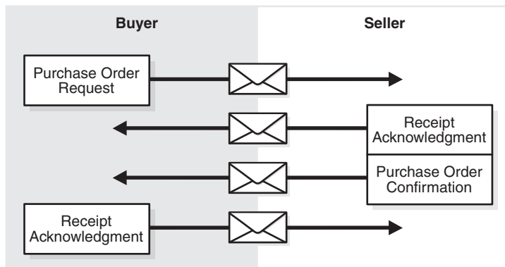
Figure 8–21 PIP 3A4 Message Exchange Between Buyer and Seller
