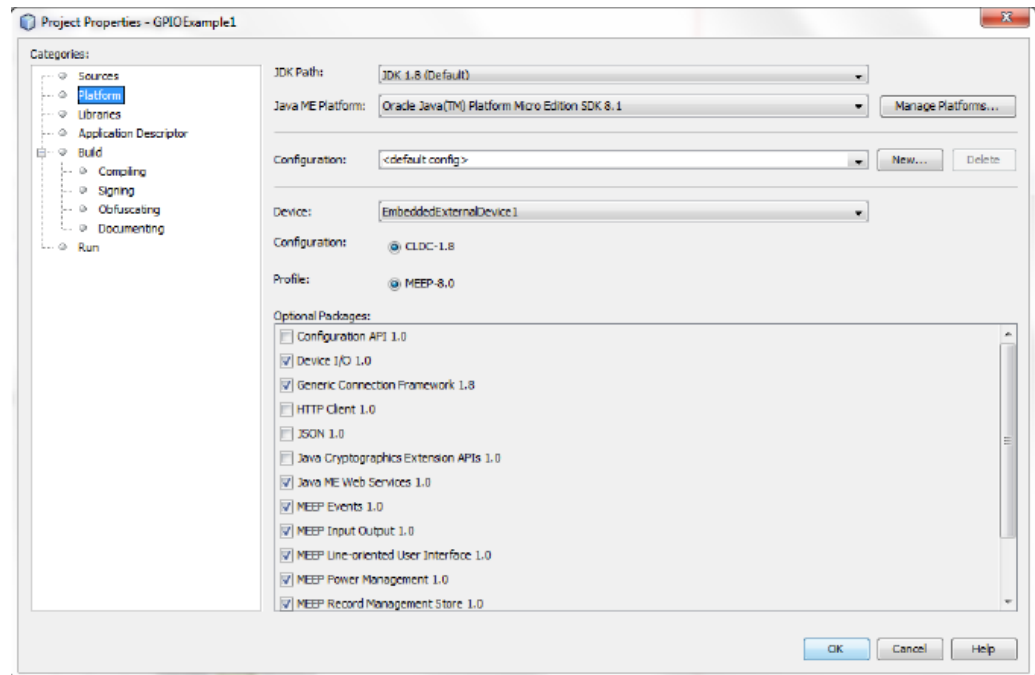
Figure 2-4 Adding a Device to Your Project
