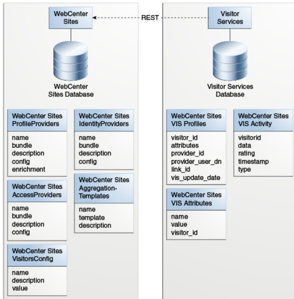
Figure 42-19 Visitor Services Data Model
