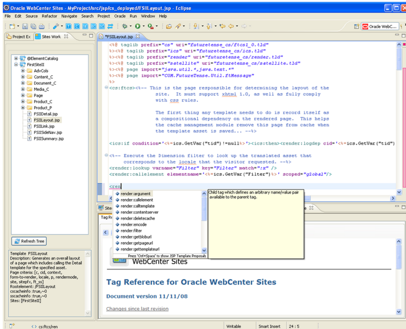
Figure 73-2 Tag and Java API Completion Feature
