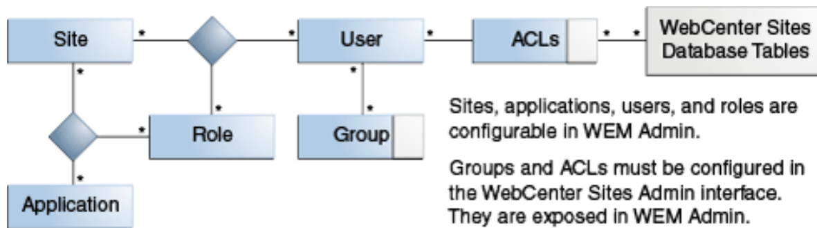
Figure 46-3 Authorization Model
