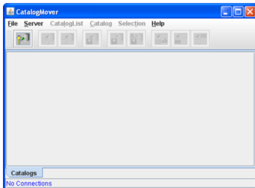
Figure 81-2 CatalogMover
