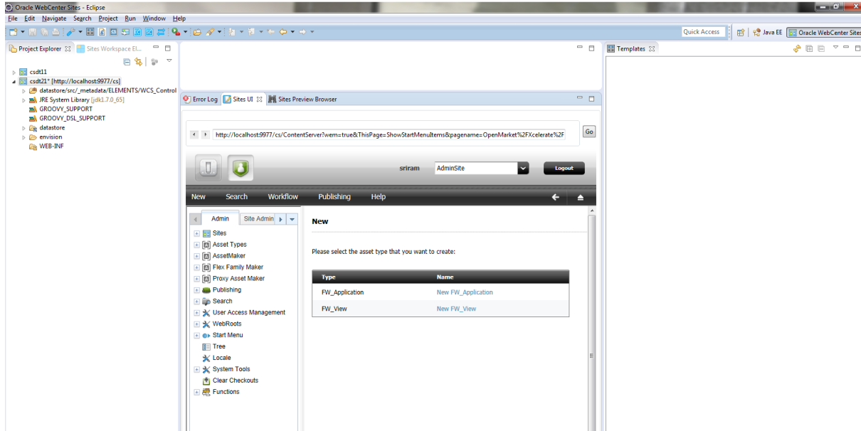
Figure 79-1 Eclipse IDE
