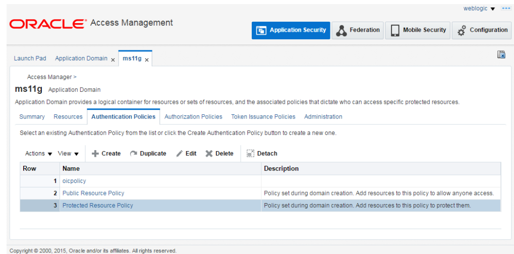
Figure 42-5 Authentication Policies
