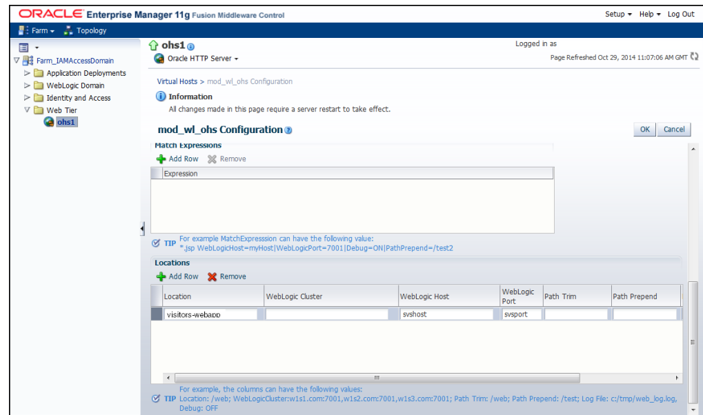
Figure 42-9 mod_wl_ohs Configuration
