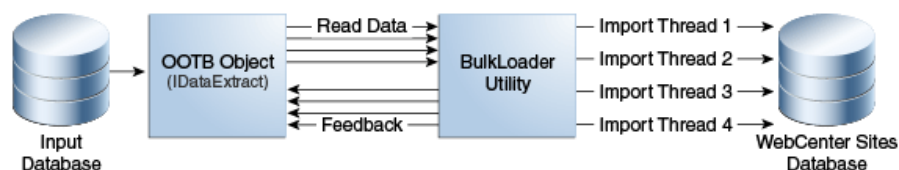
Figure 33-2 Built-in OOTB (out-of-the-box) implementation of BulkLoader
