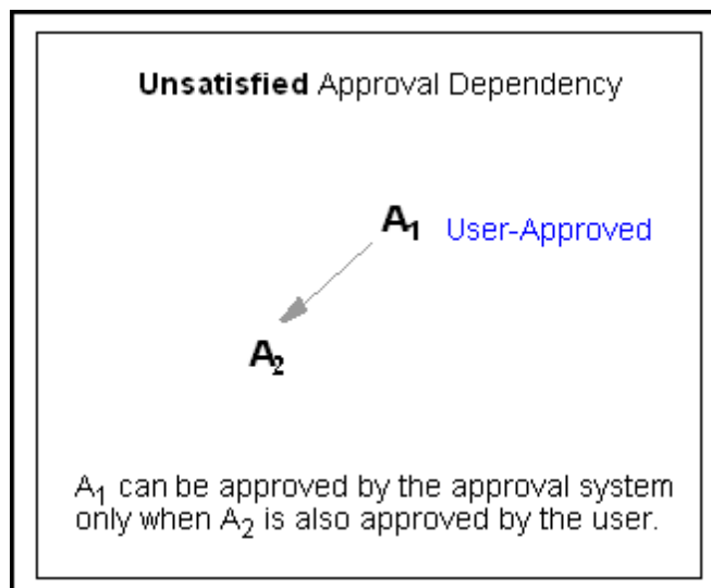
Figure 19-7 Unsatisfied Dependencies
