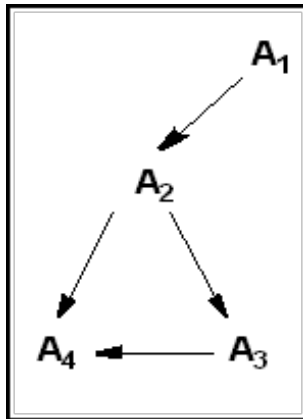
Figure 19-19 Exists/Exact Dependencies
