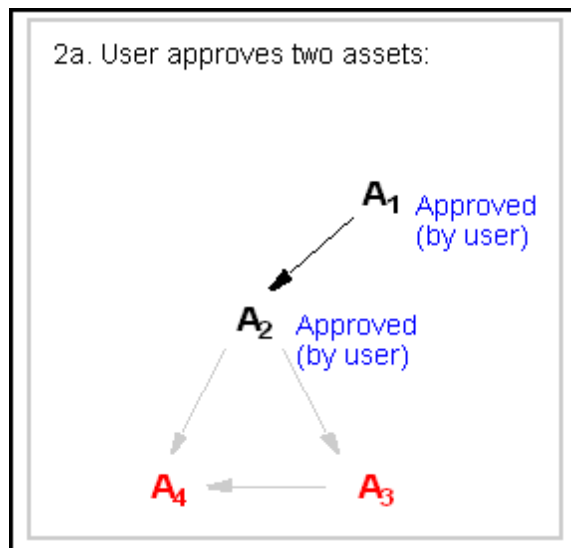
Figure 19-13 Dependency Model
