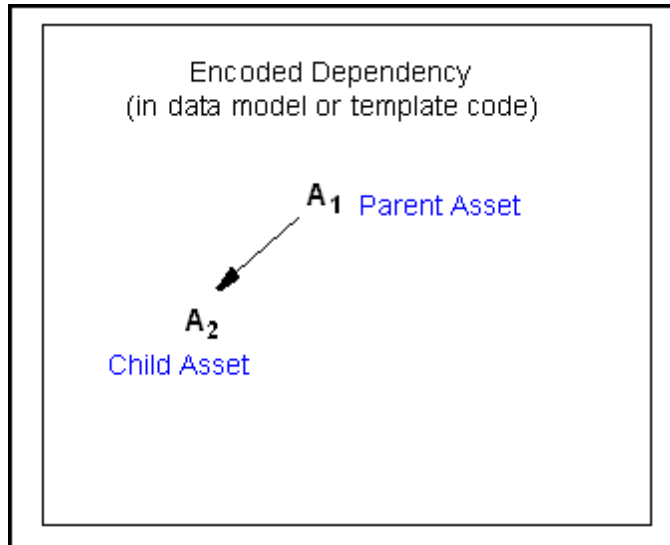
Figure 19-6 Encoded Dependencies
