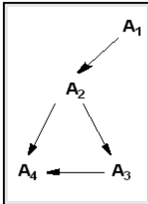
Figure 19-18 Approval Dependencies
