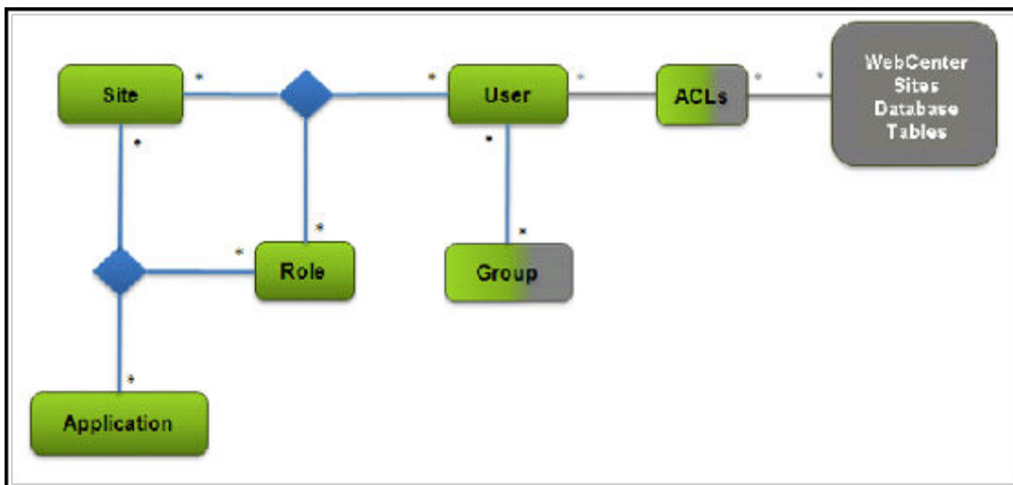
Figure 11-2 Authorization Model
