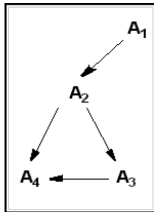
Figure 19-17 Parent-Child Relationships
