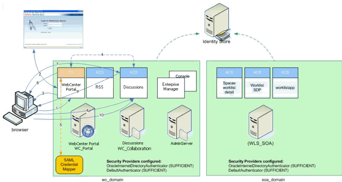
Figure 26-3 Detailed SAML Single Sign-on Components and Topology (POST Profile Configured)
