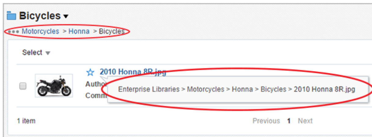
Figure 11-1 Document Context
