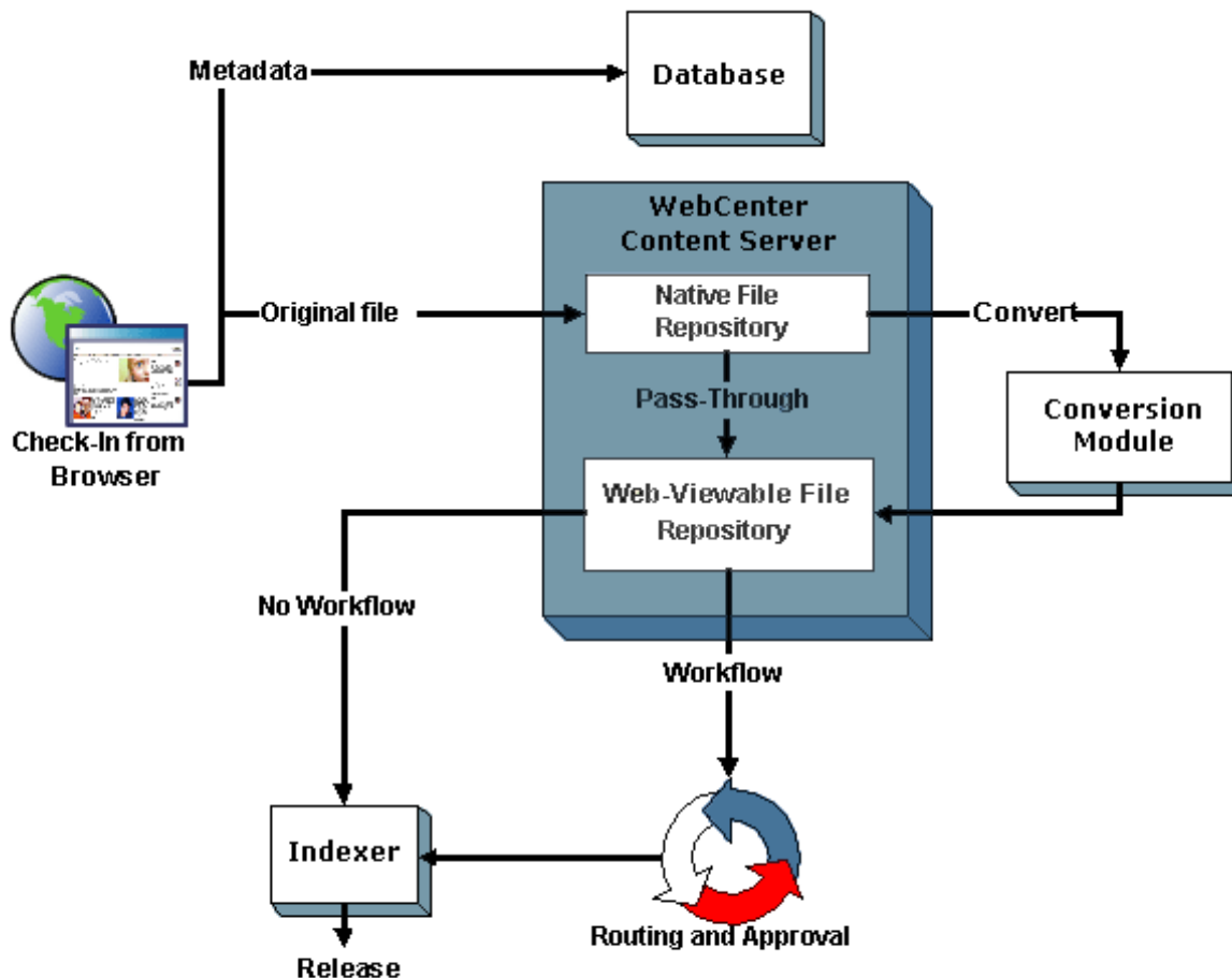
Figure 3-1 Revision Process
