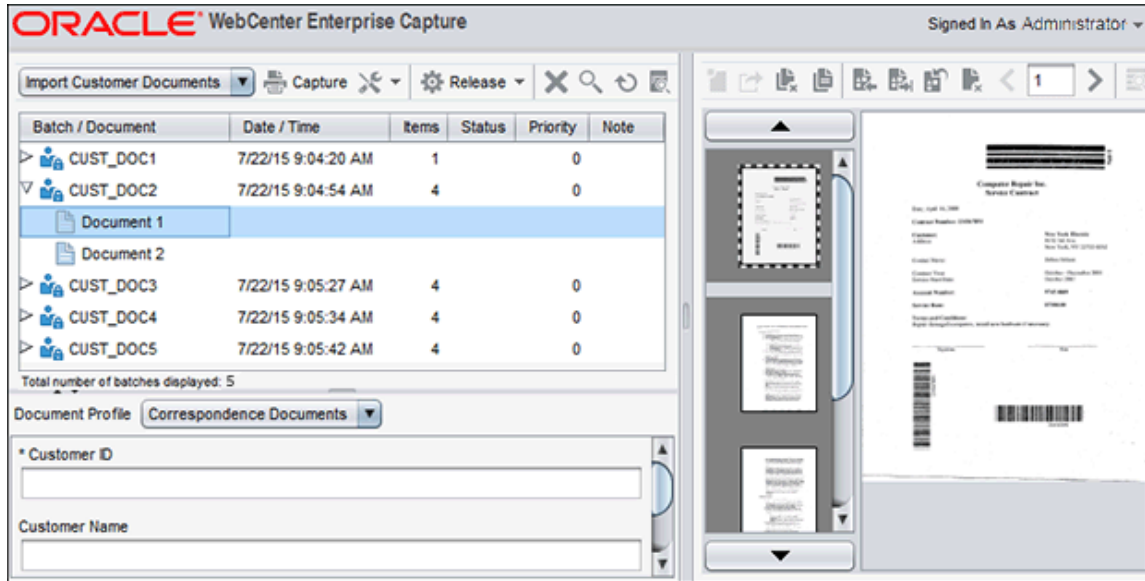
Figure 1-2 Capture Client Window Displaying Batch, Document, and Metadata Panes
