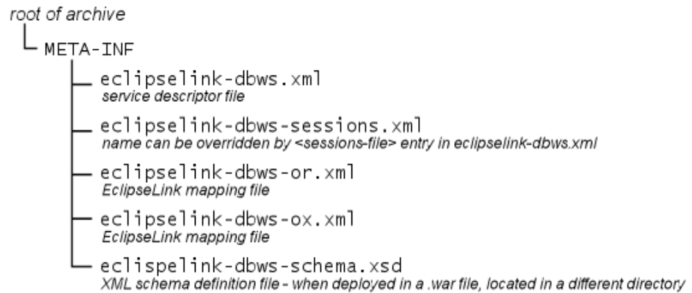
Figure 1-2 Typical EclipseLink DBWS Service Files
