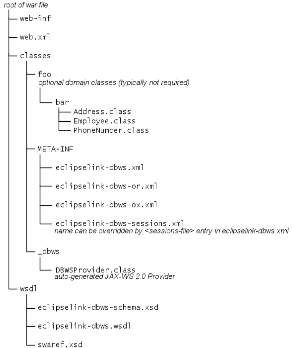
Figure 1-3 Contents of WAR File
