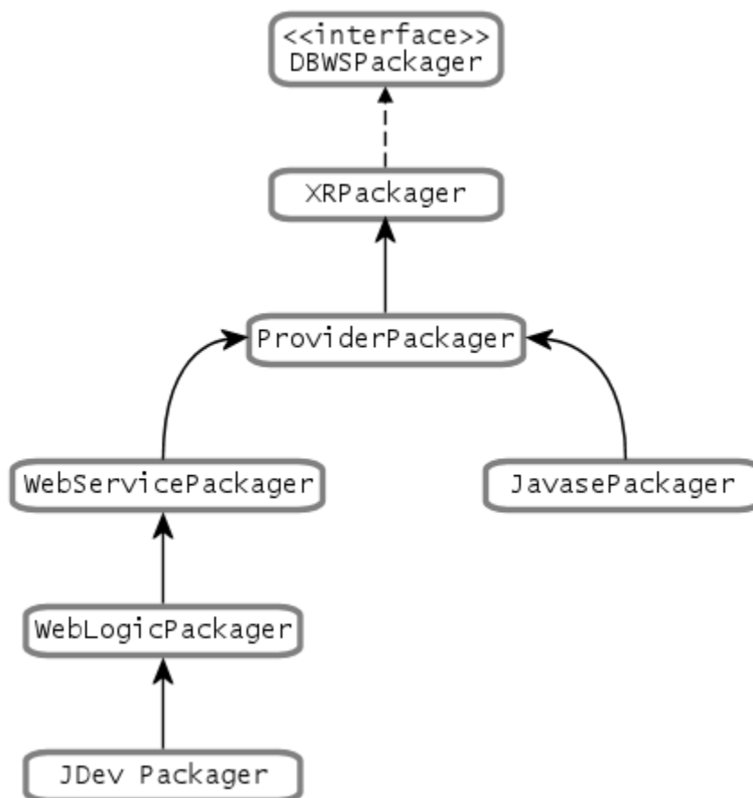
Figure 1-4 Hierarchy of Concrete Implementation
