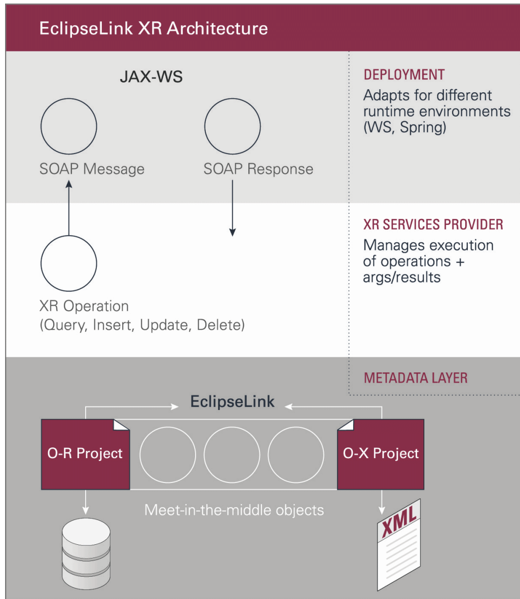
Figure 1-1 EclipseLink XR Architecture
