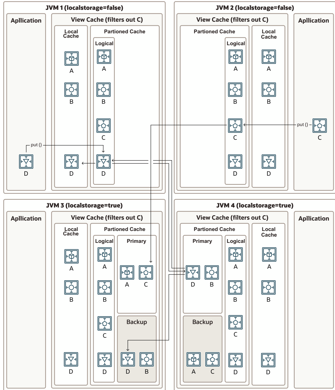
Figure 12-9 Put Operations in a View Cache
