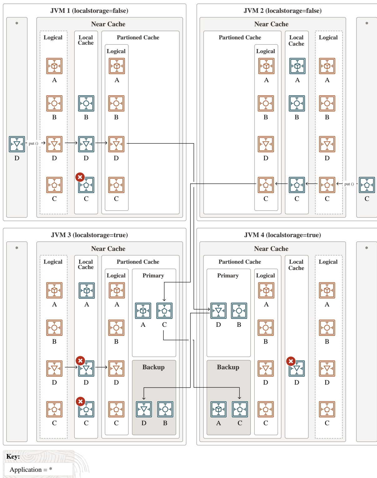
Figure 12-7 Put Operations in a Near Cache
