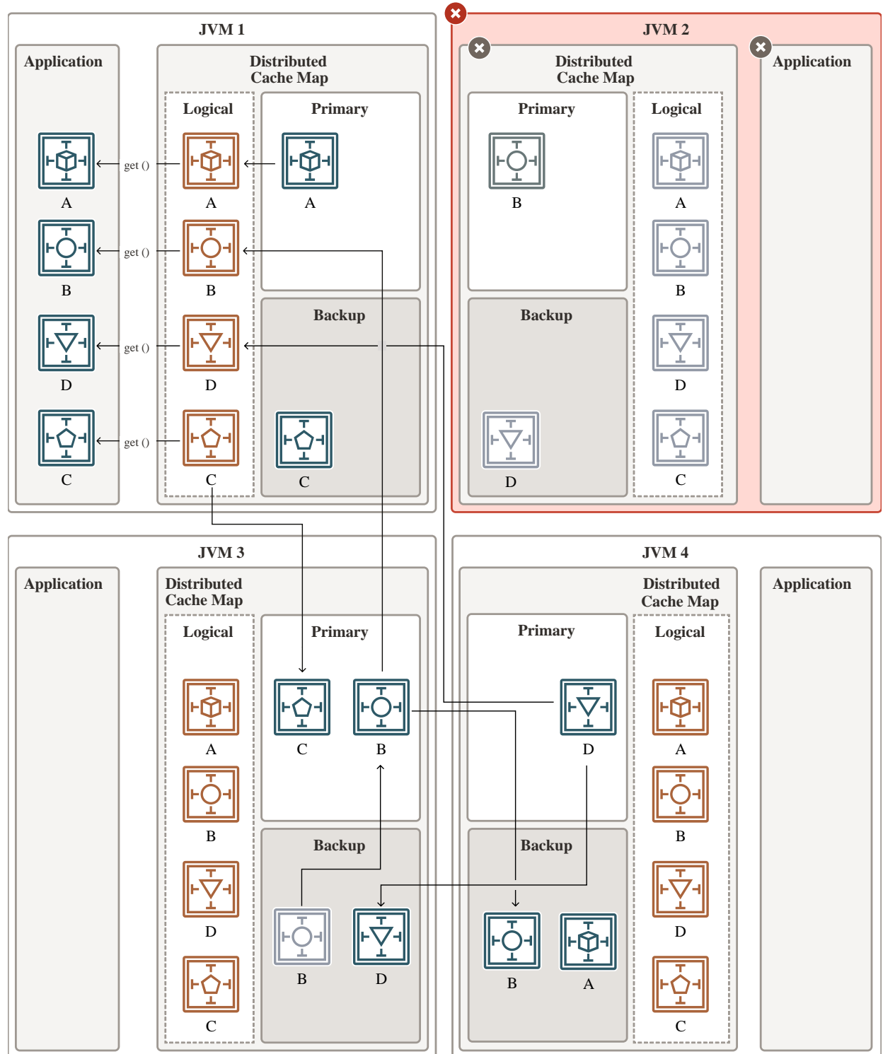
Figure 12-3 Failover in a Distributed Cache
