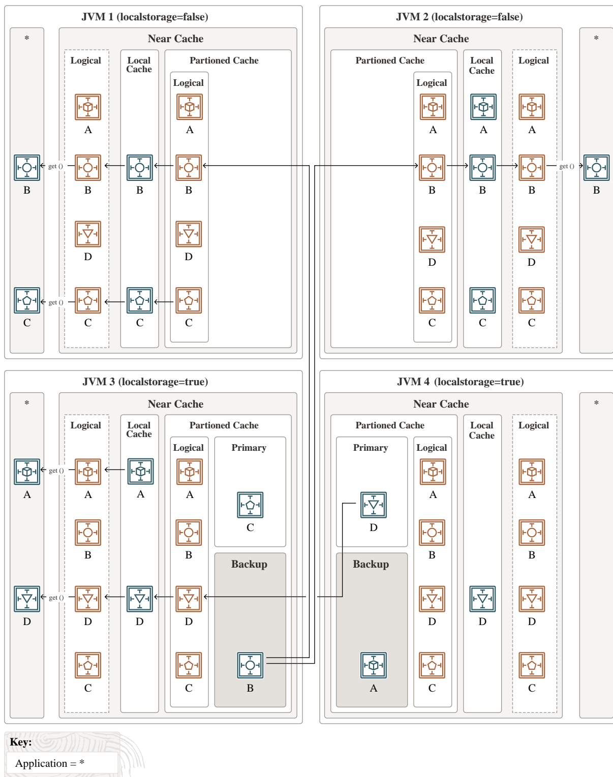
Figure 12-8 Get Operations in a Near Cache
