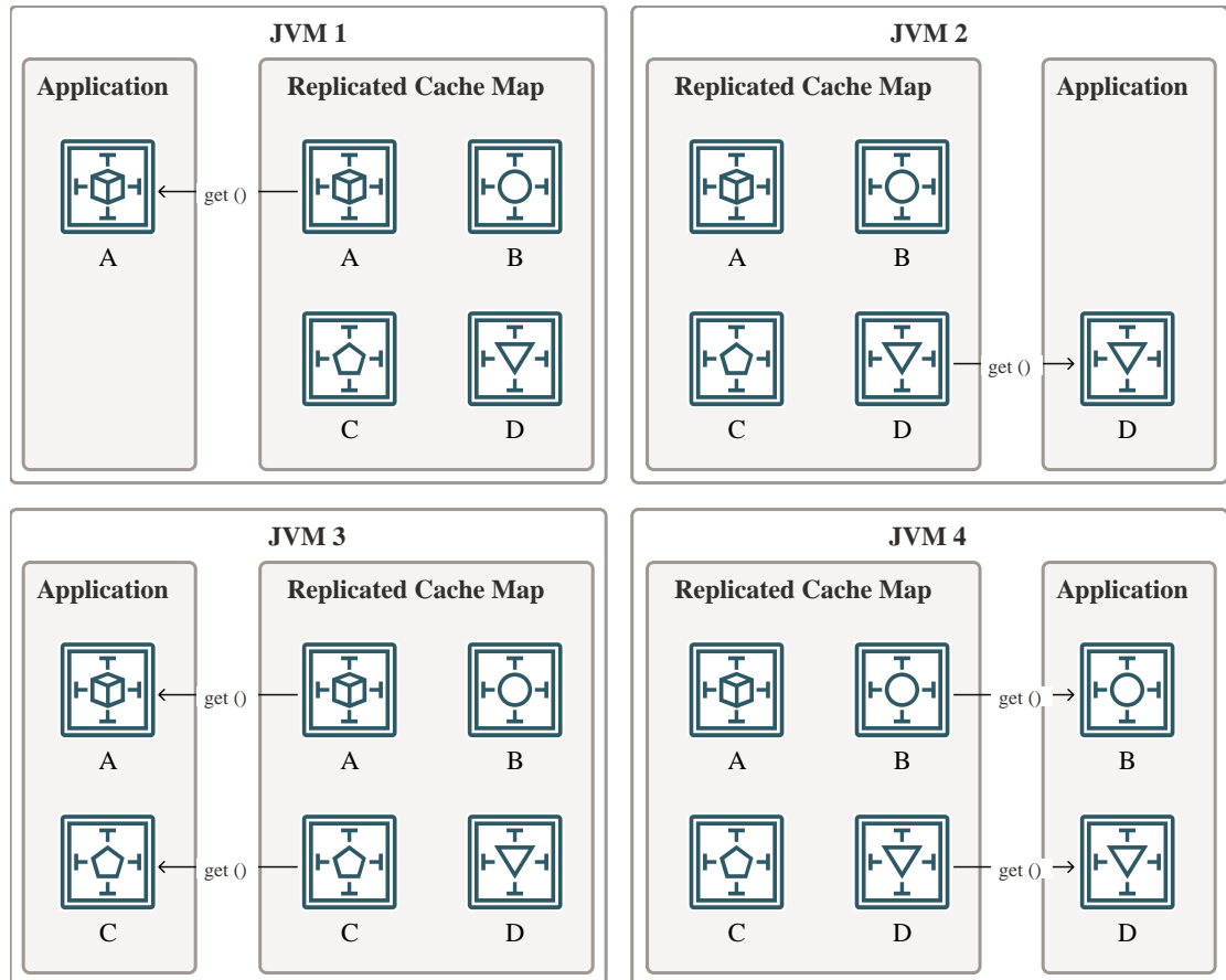
Figure 12-5 Get Operation in a Replicated Cache
