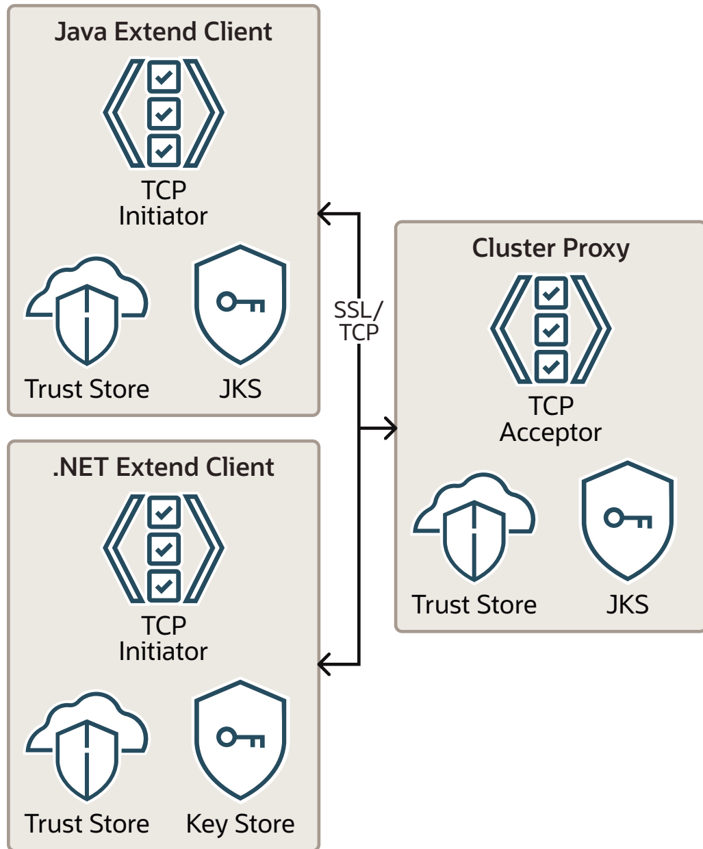
Figure 6-2 Conceptual Architecture of SSL with Oracle Coherence*Extend
