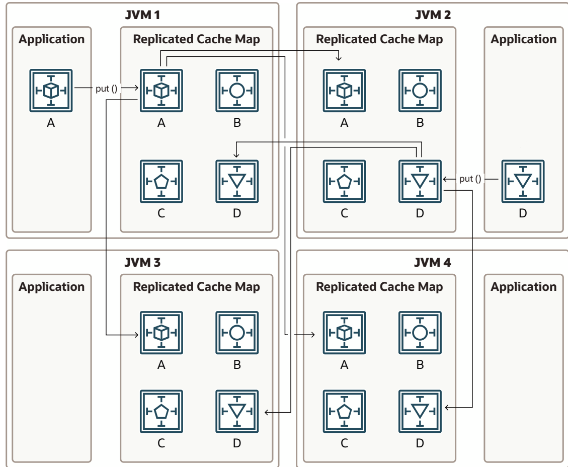
Figure 11-6 Put Operation in a Replicated Cache
