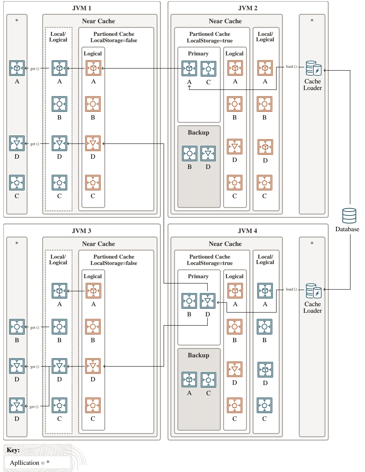
Figure 14-1 Read-Through Caching
