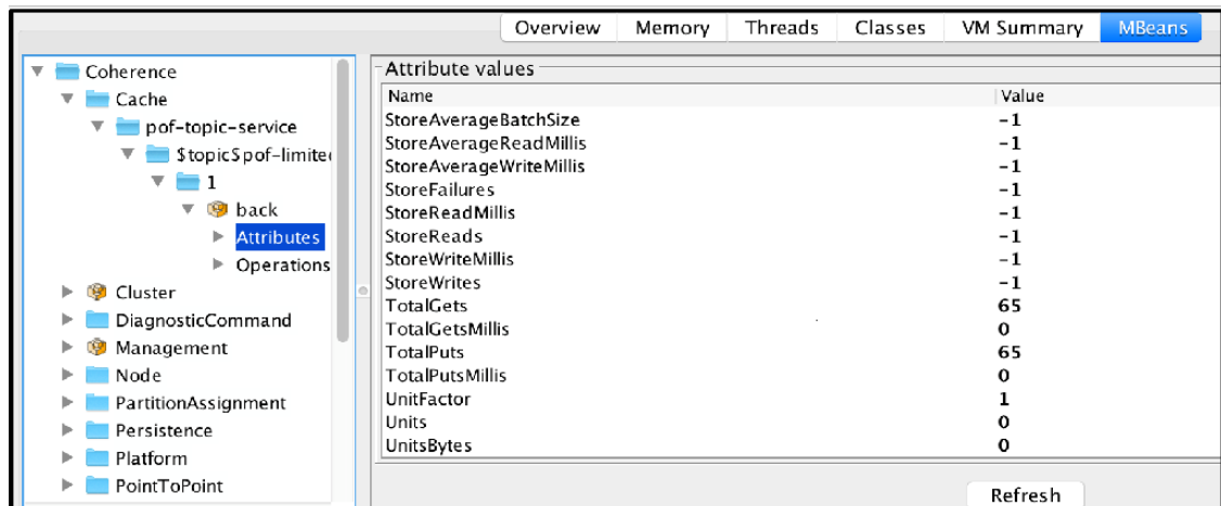
Figure 22-3 Topic pof-limited is empty and has no outstanding values to be consumed
