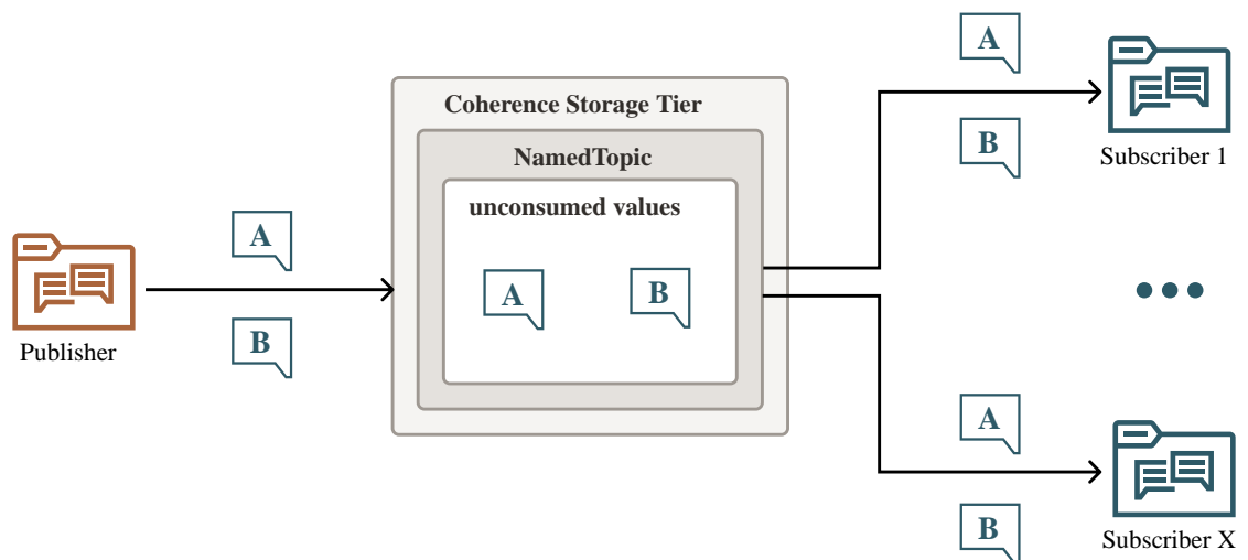
Figure 19-1 Topic Values
