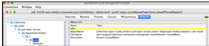
Figure 22-1 Topic pof-limited
