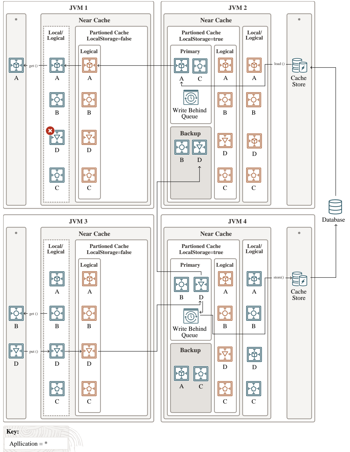
Figure 14-3 Write-Behind Caching
