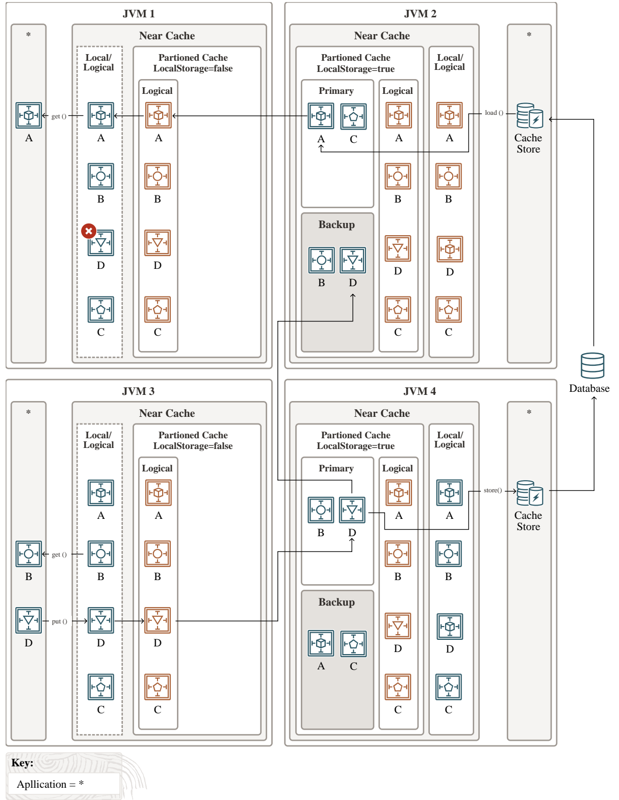
Figure 14-2 Write-Through Caching
