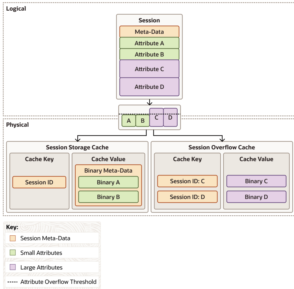
Figure 4-4 Split Session Model
