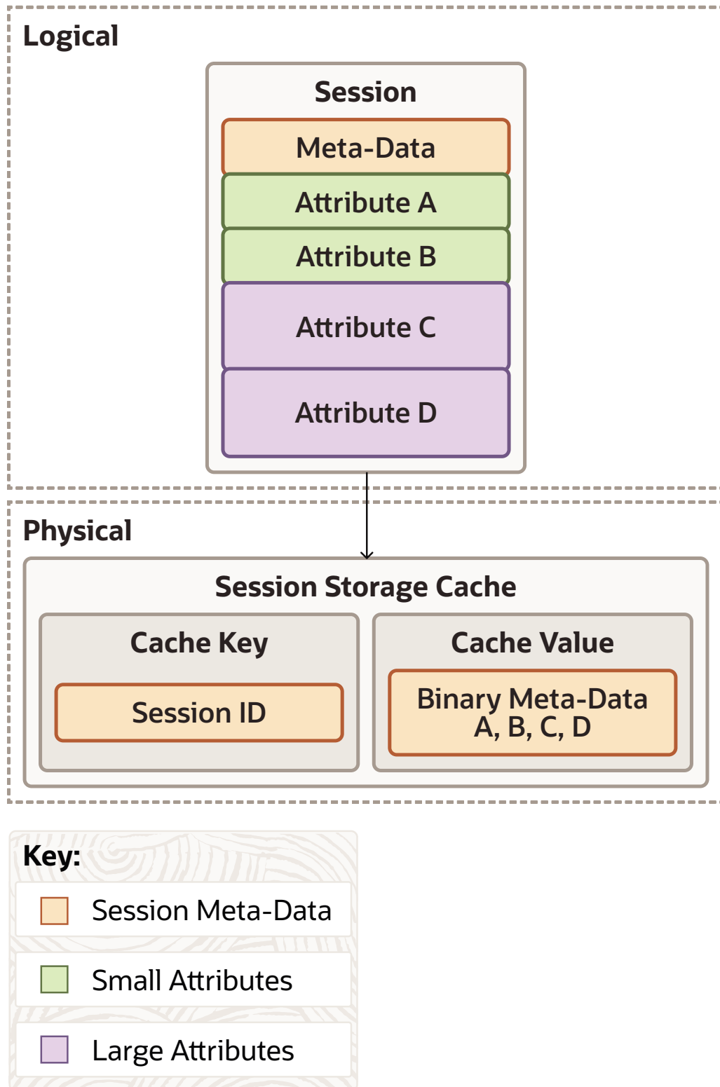
Figure 4-2 Monolithic Session Model
