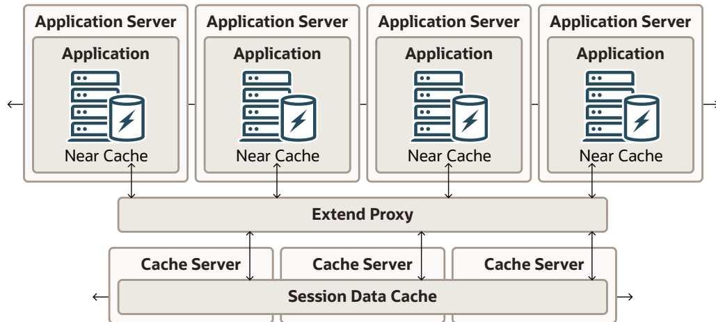
Figure 4-11 Out-of-Process with Coherence*Extend Deployment Topology
