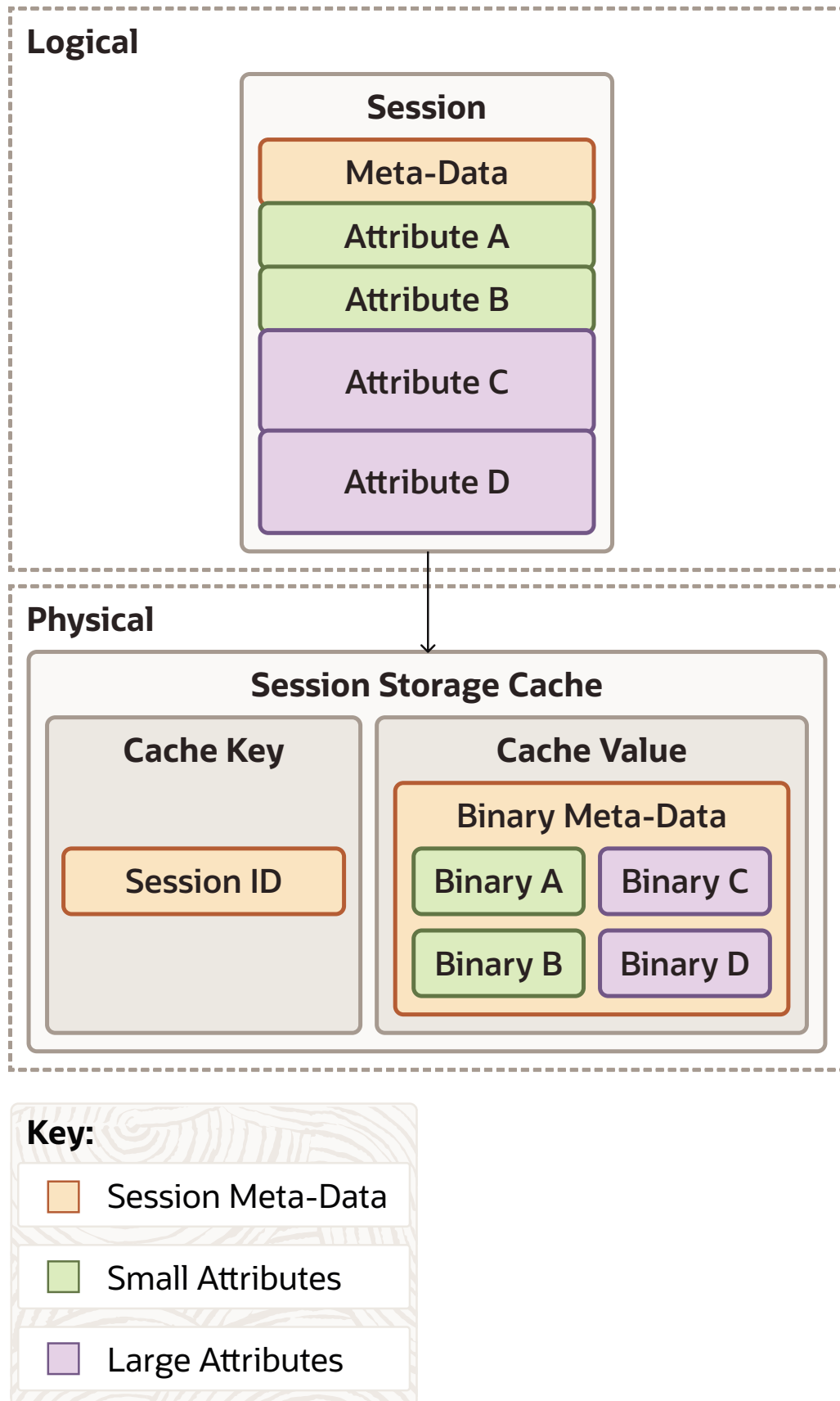
Figure 4-3 Traditional Session Model
